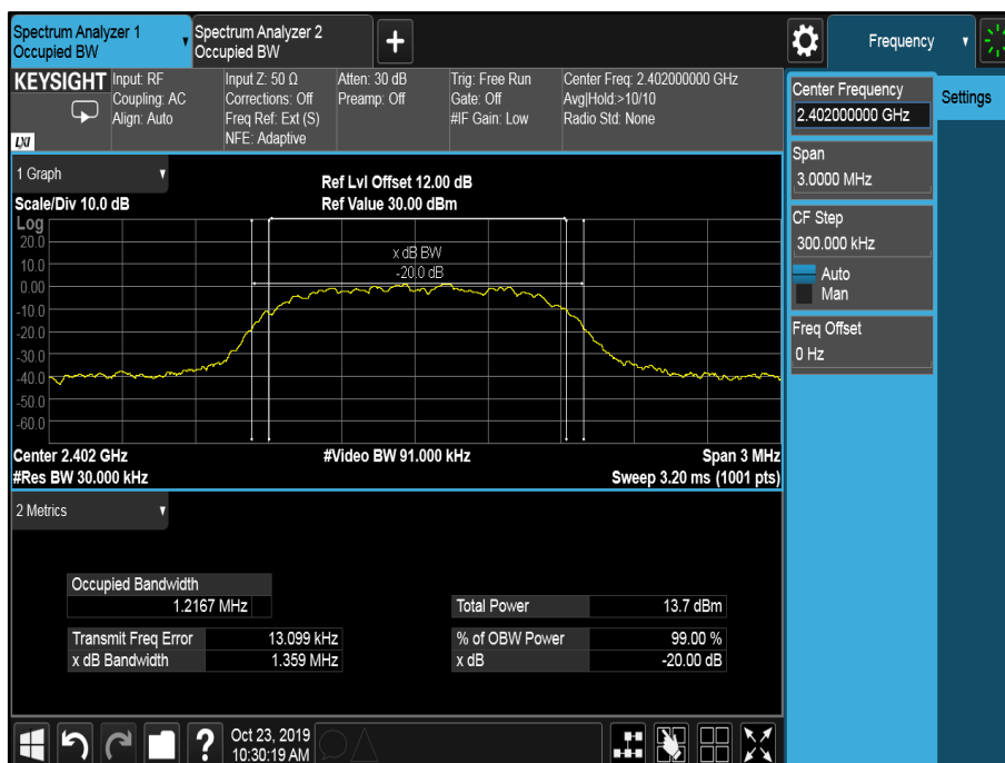
Figure 15 - 2402 MHz - 8-DPSK
