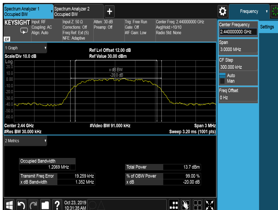
Figure 18 - 2440 MHz - 8-DPSK
