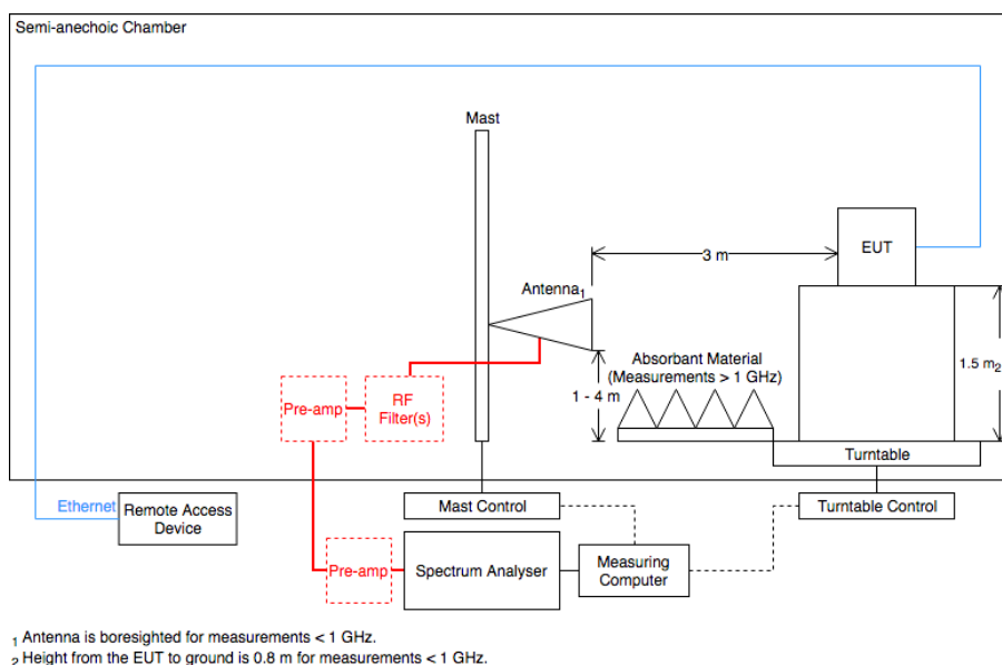
Figure 150 - Radiated Emissions Test Setup Diagram
