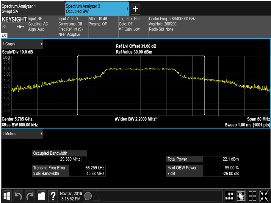
Figure 537 - 5785 MHz - 99% Occupied Bandwidth
