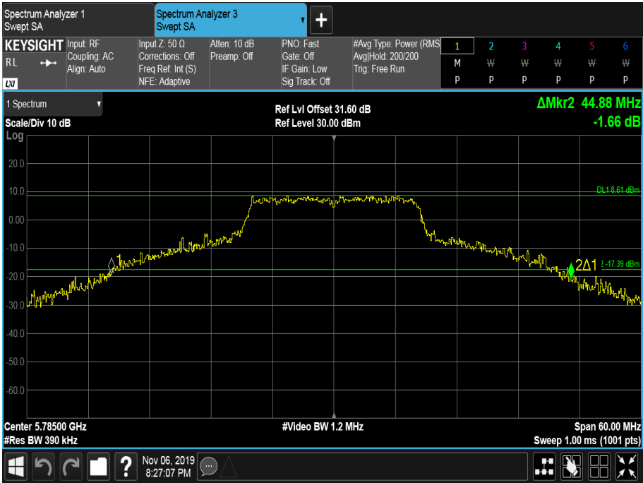
Figure 524 - 5785 MHz - 26 dB Emission Bandwidth
