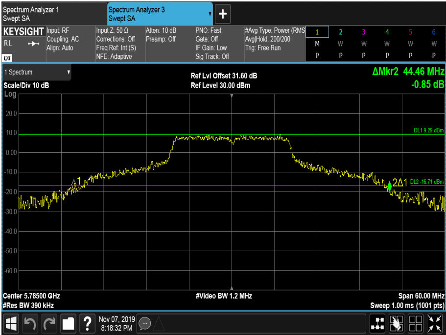
Figure 536 - 5785 MHz - 26 dB Emission Bandwidth
