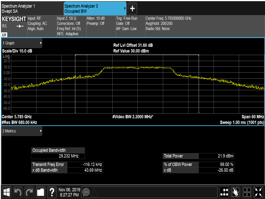
Figure 525 - 5785 MHz - 99% Occupied Bandwidth
