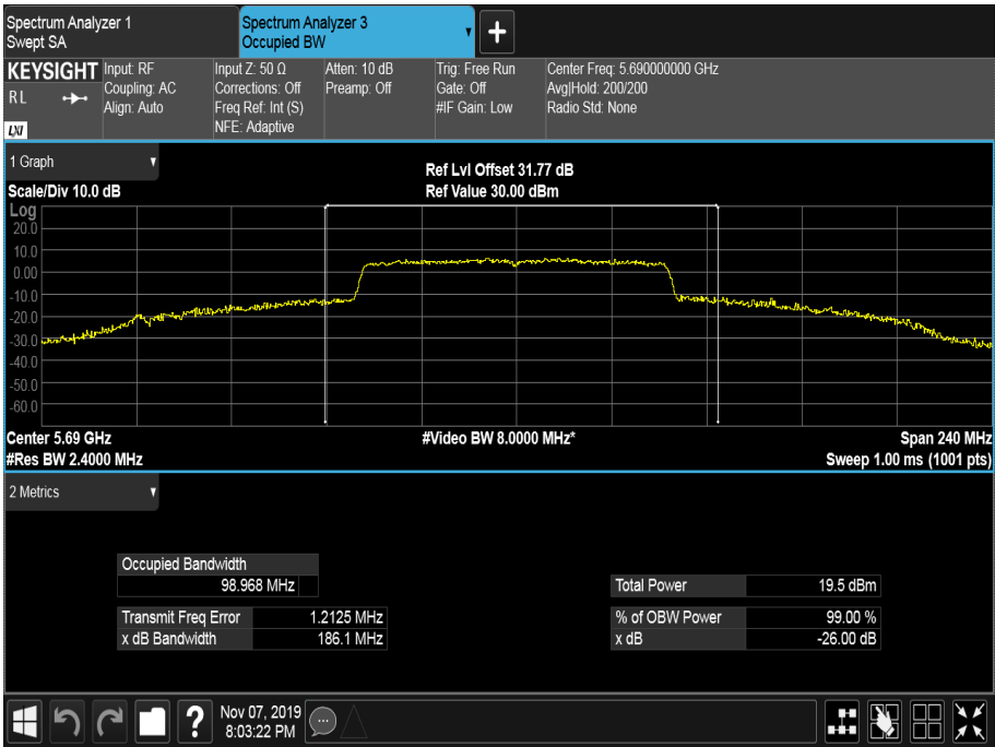
Figure 516 - 5690 MHz - 99% Occupied Bandwidth
