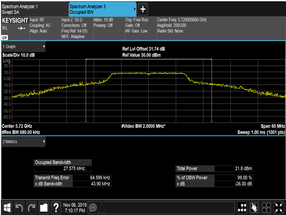
Figure 519 - 5720 MHz - 99% Occupied Bandwidth
