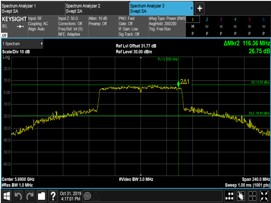
Figure 503 - 5690 MHz - 26 dB Emission Bandwidth
