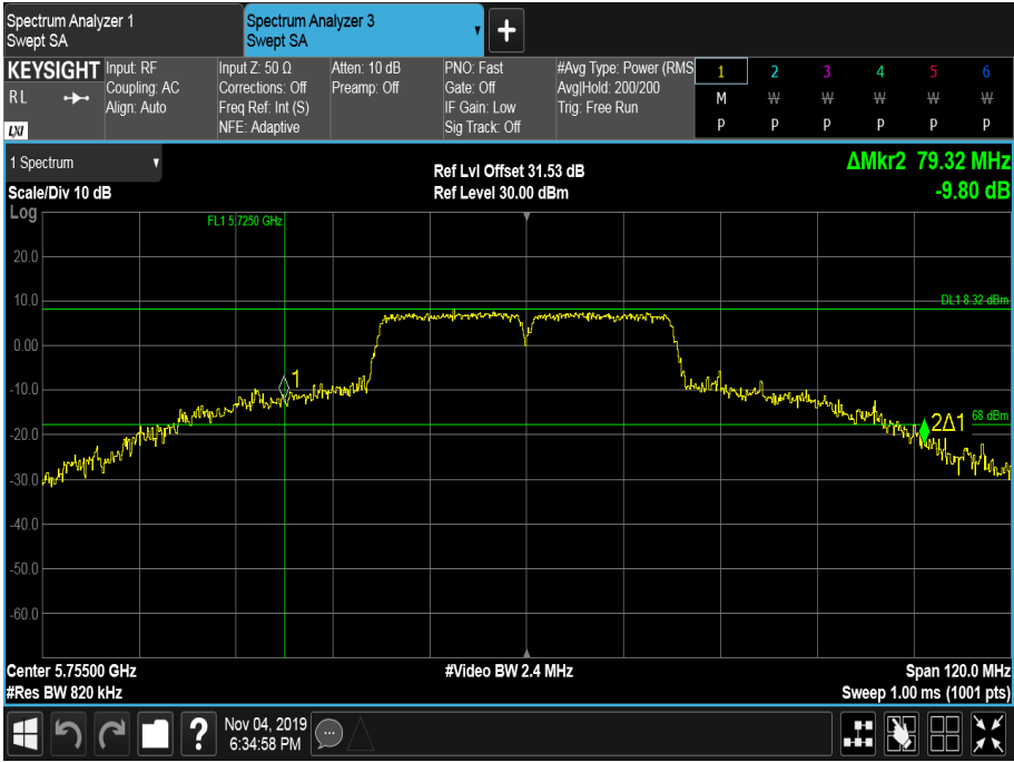
Figure 635 - 5755 MHz - 26 dB Emission Bandwidth
