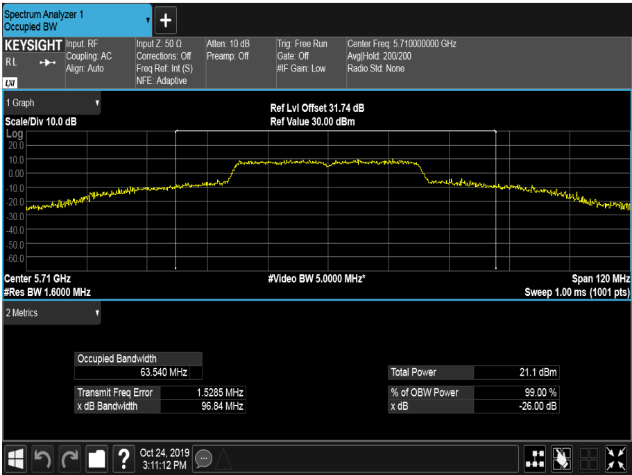
Figure 624 - 5710 MHz - 99% Occupied Bandwidth
