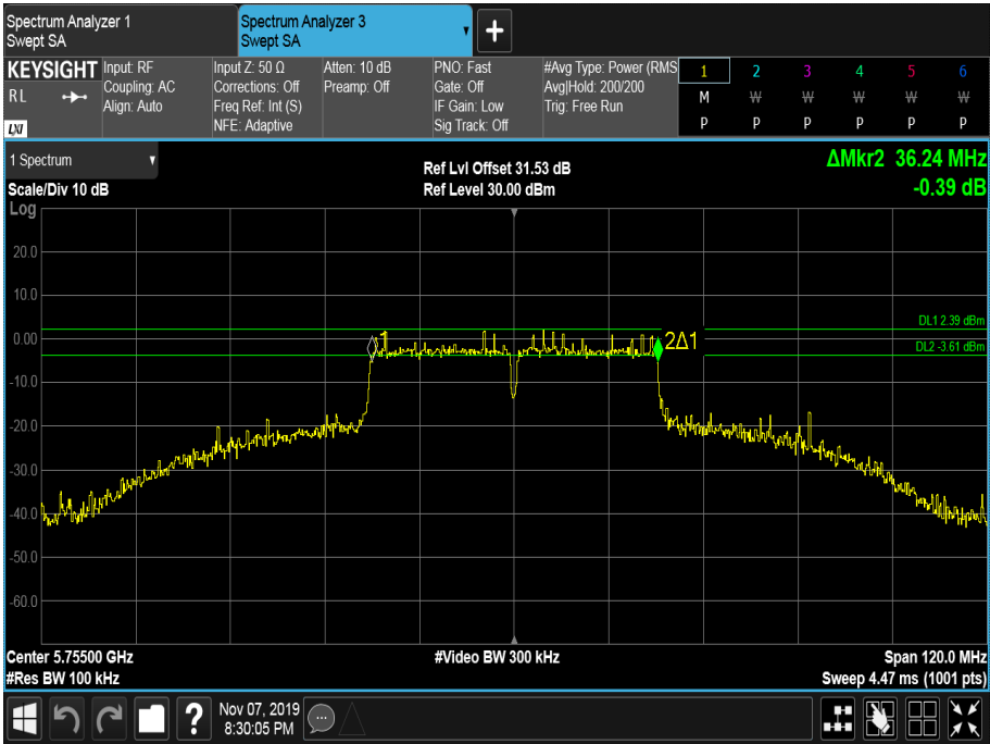
Figure 661 - 5755 MHz - 6 dB DTS Bandwidth
