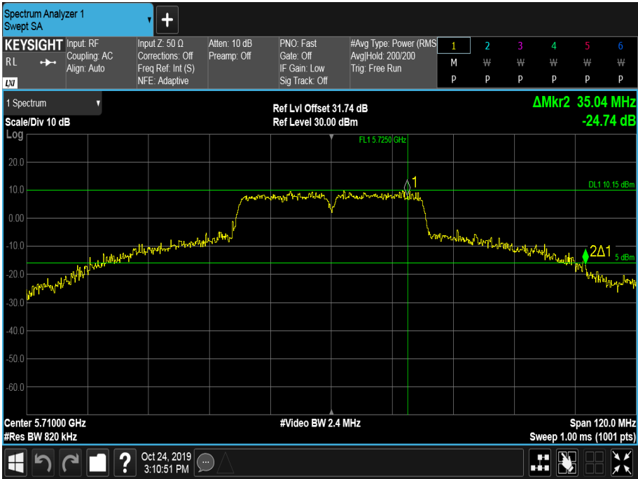
Figure 623 - 5710 MHz - 26 dB Emission Bandwidth
