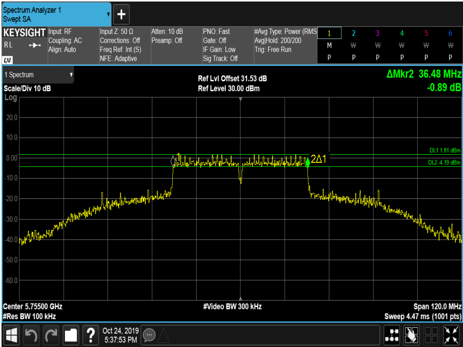
Figure 634 - 5755 MHz - 6 dB DTS Bandwidth
