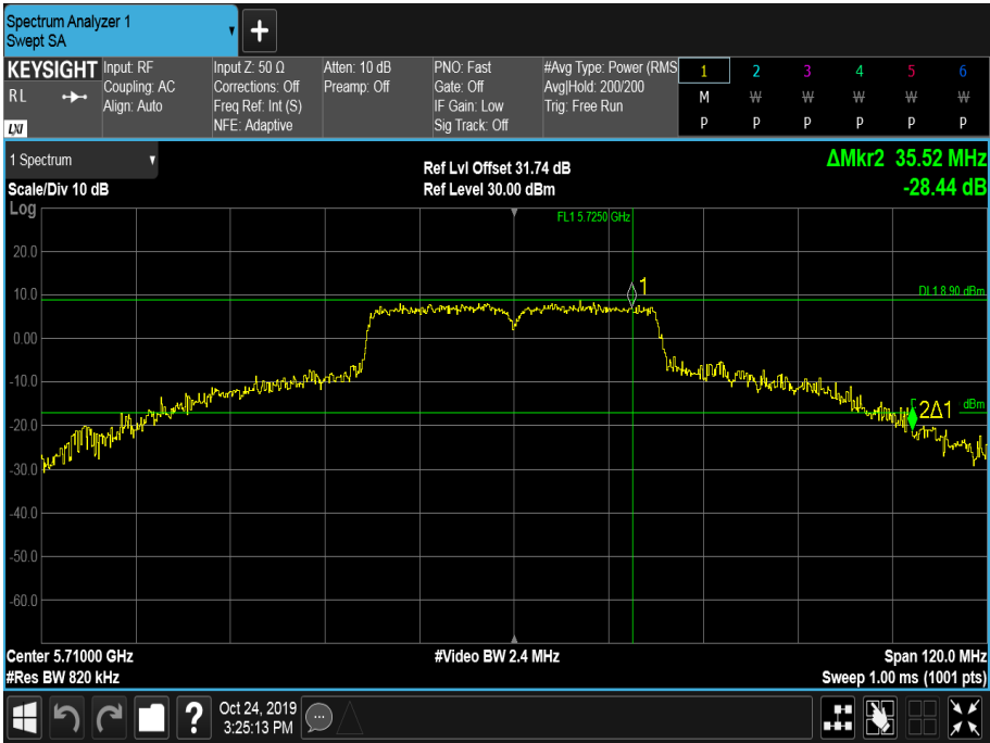
Figure 650 - 5710 MHz - 26 dB Emission Bandwidth
