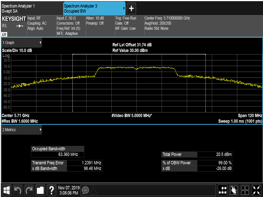
Figure 651 - 5710 MHz - 99% Occupied Bandwidth
