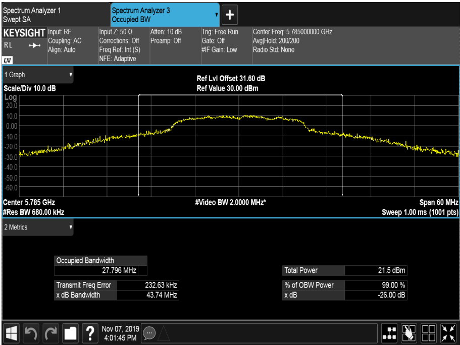
Figure 687 - 5785 MHz - 99% Occupied Bandwidth
