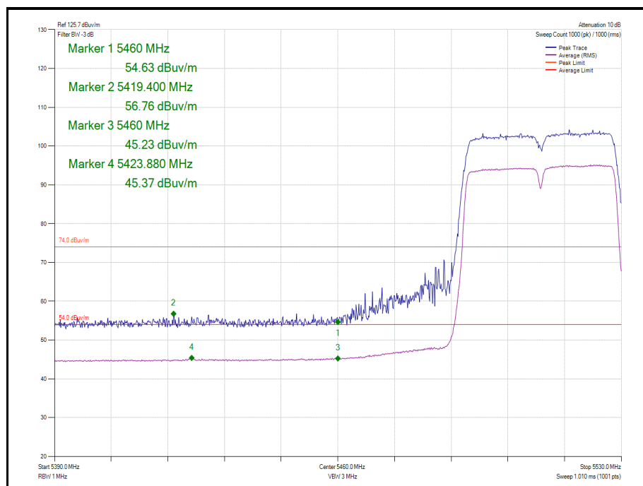
Figure 863 - 802.11n HT40 Core 1 - 5510 MHz Band Edge Frequency 5460 MHz
