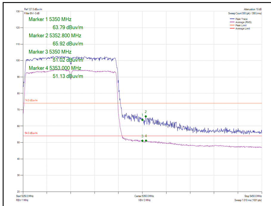
Figure 883 - 802.11ac VHT80 Core Aux - 5290 MHz Band Edge Frequency 5350 MHz
