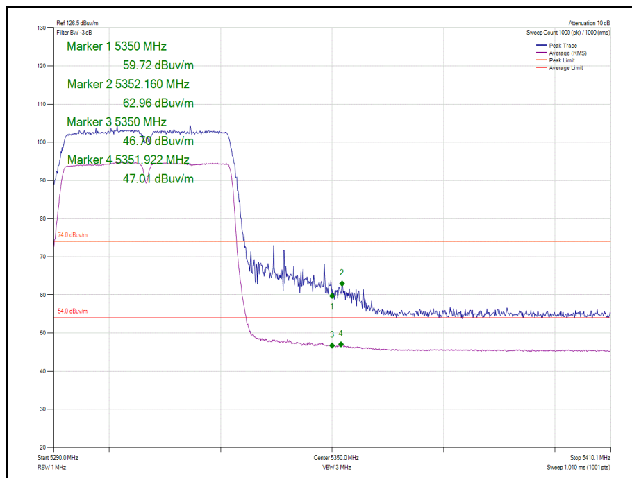
Figure 862 - 802.11n HT40 Core 1 - 5310 MHz Band Edge Frequency 5350 MHz
