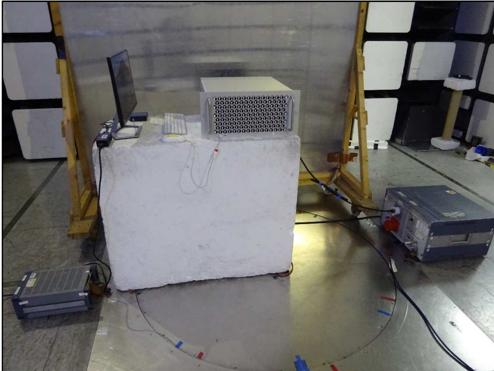
Figure 5 - Conducted Disturbance at Mains Terminals
