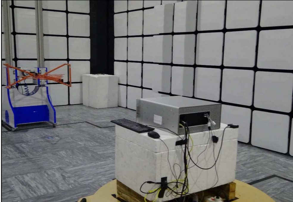
Figure 1 - Radiated Disturbance - Below 1 GHz
