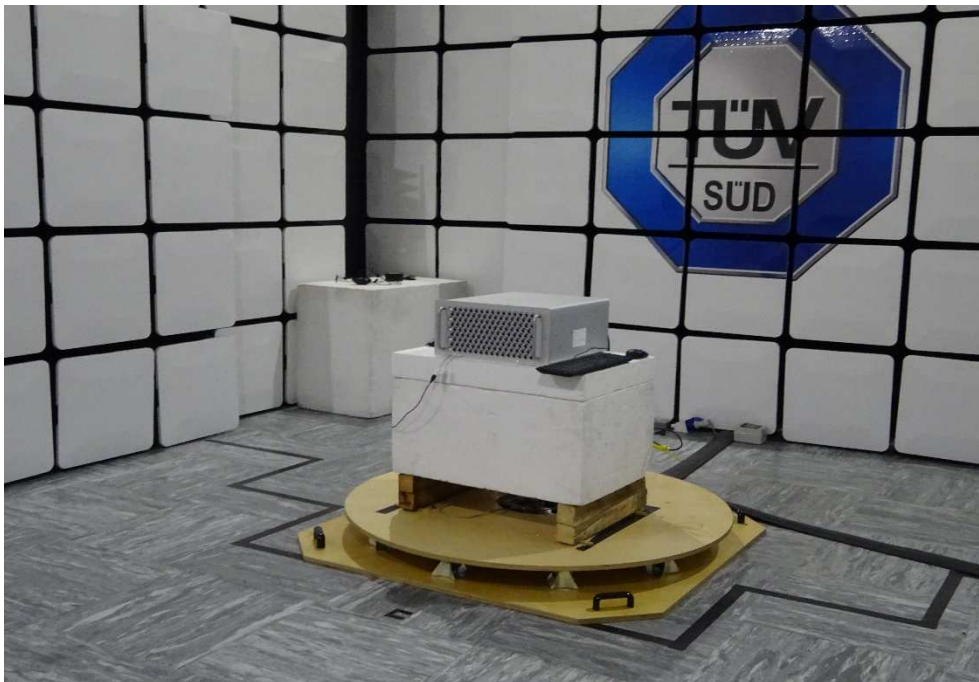
Figure 2 - Radiated Disturbance - Below 1 GHz
