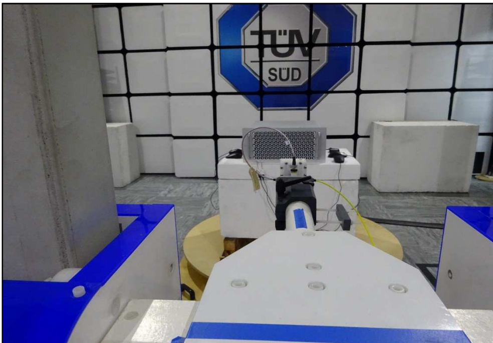
Figure 3 Radiated Disturbance - Above 1 GHz
