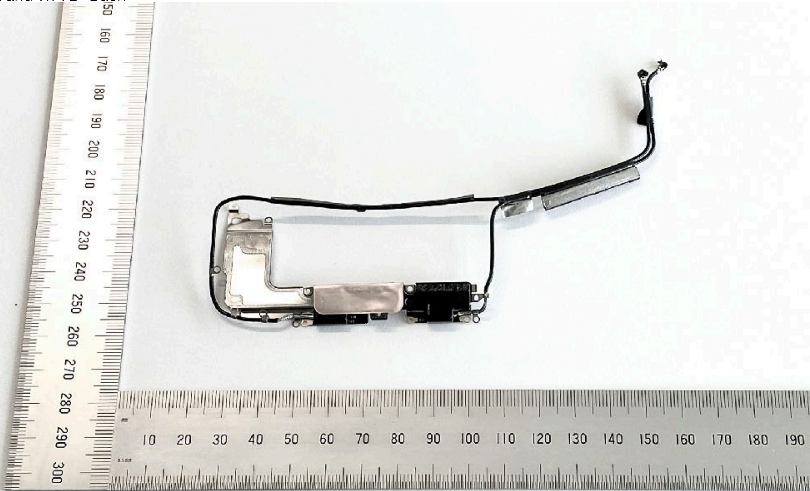
A2316 WiFi/BT Antenna WF7A and WF7B- Back
