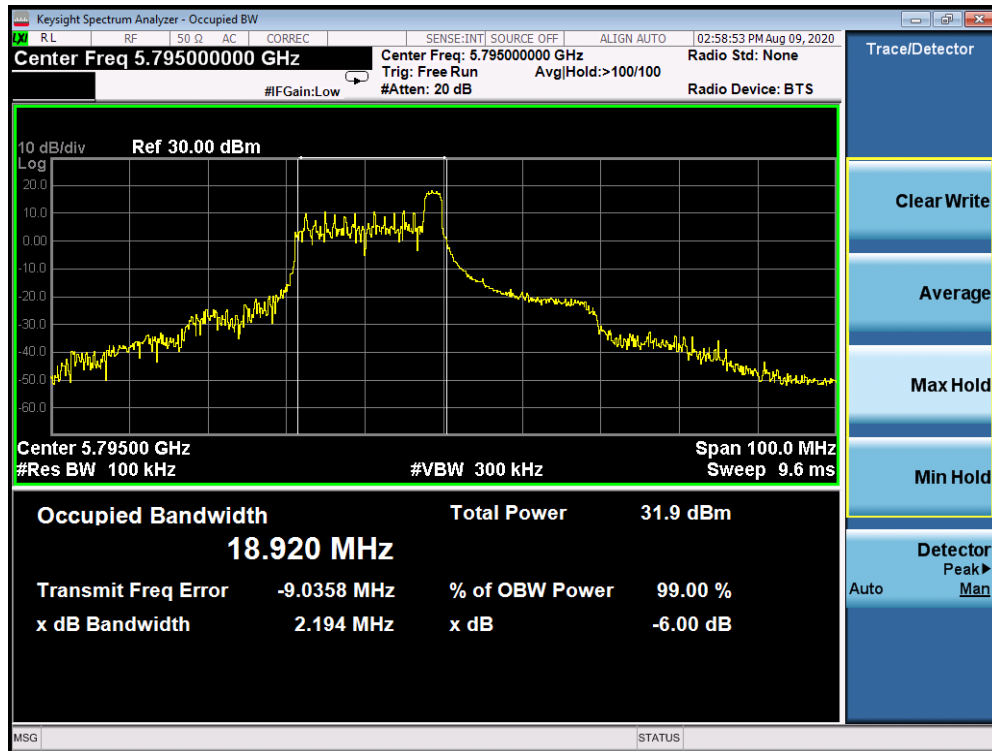
Plot 7-257. 6dB Bandwidth Plot Antenna 2b (40MHz BW 802.11ax Index 8 – RU26 (UNII Band 3) – Ch. 159)
