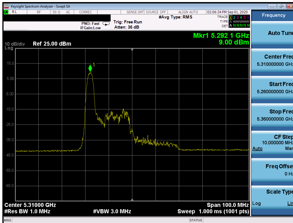
Plot 7-352. Power Spectral Density Plot Antenna 2b (40MHz BW 802.11ax Index 0 – RU26 (UNII Band 2A) – Ch. 62)
