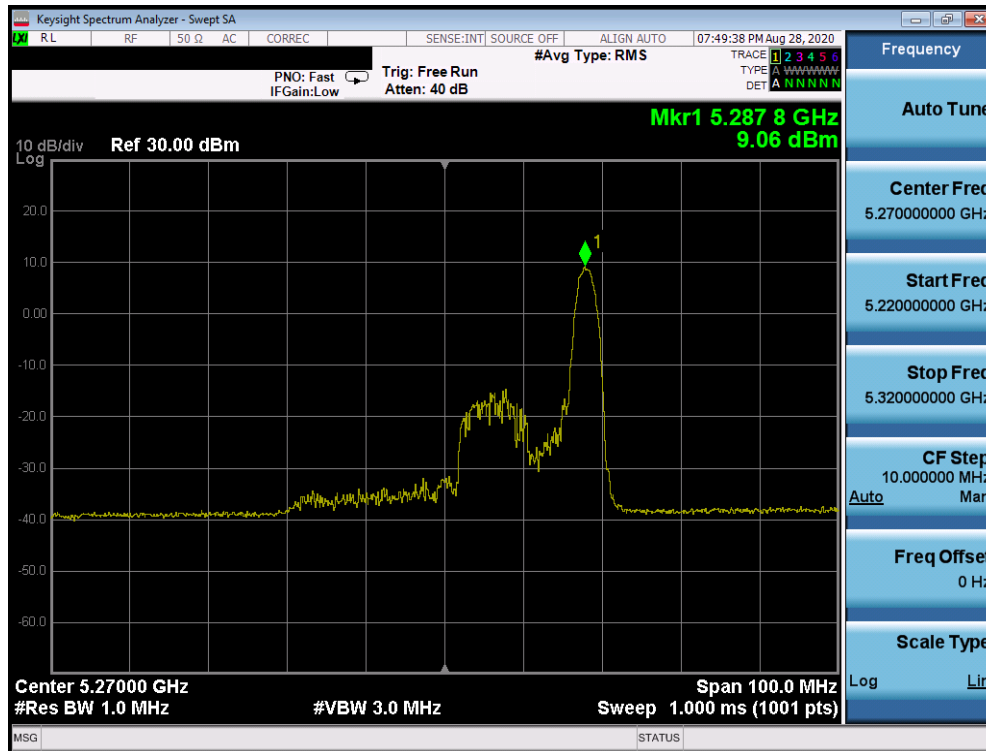
Plot 7-351. Power Spectral Density Plot Antenna 2b (40MHz BW 802.11ax Index 17 – RU26 (UNII Band 2A) – Ch. 54)
