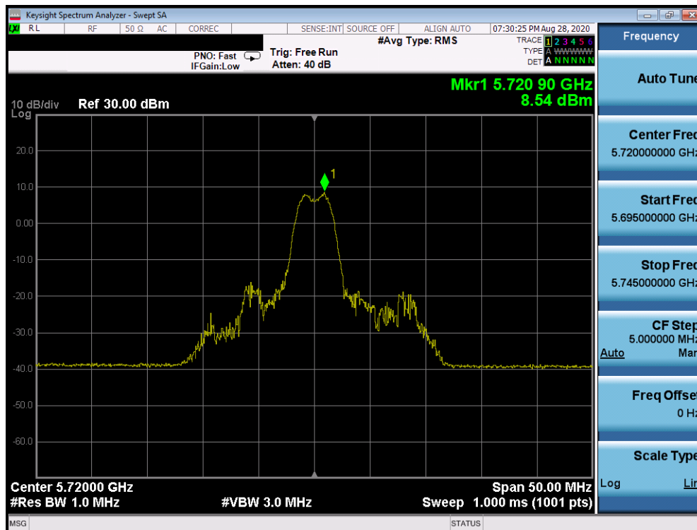
Plot 7-368. Power Spectral Density Plot Antenna 2b (20MHz BW 802.11ax Index 4 – RU26 (UNII Band 2C) – Ch. 144)
