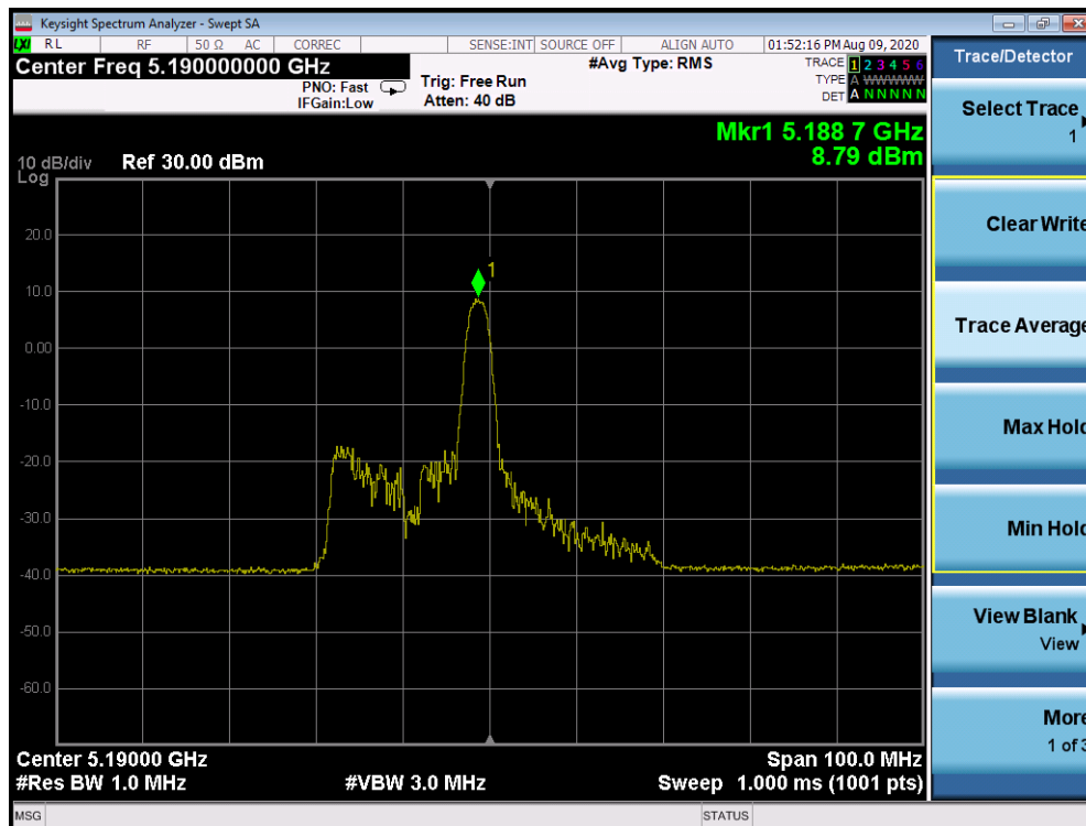
Plot 7-326. Power Spectral Density Plot Antenna 2b (40MHz BW 802.11ax Index 8 – RU26 (UNII Band 1) – Ch. 38)
