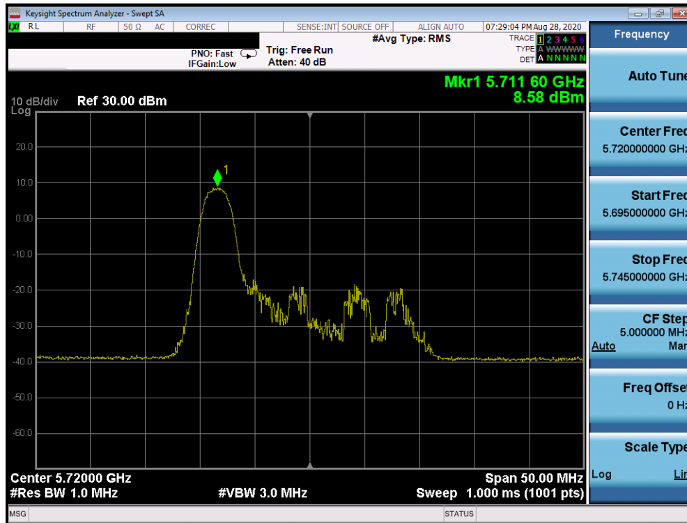
Plot 7-367. Power Spectral Density Plot Antenna 2b (20MHz BW 802.11ax Index 0 – RU26 (UNII Band 2C) – Ch. 144)
