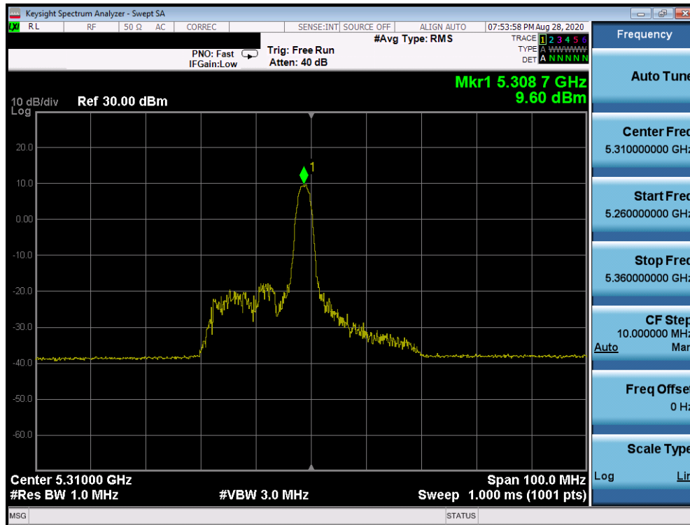
Plot 7-353. Power Spectral Density Plot Antenna 2b (40MHz BW 802.11ax Index 8 – RU26 (UNII Band 2A) – Ch. 62)
