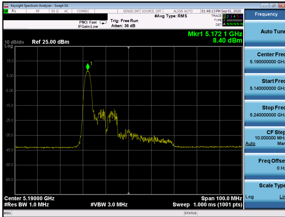
Plot 7-325. Power Spectral Density Plot Antenna 2b (40MHz BW 802.11ax Index 0 – RU26 (UNII Band 1) – Ch. 38)
