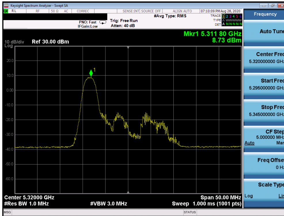
Plot 7-343. Power Spectral Density Plot Antenna 2b (20MHz BW 802.11ax Index 0 – RU26 (UNII Band 2A) – Ch. 64)
