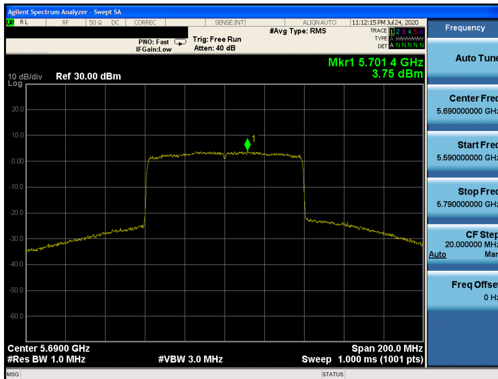
Plot 7-394. Power Spectral Density Plot Antenna 2b (80MHz BW 802.11ax – RU996 (UNII Band 2C) – Ch. 138)
