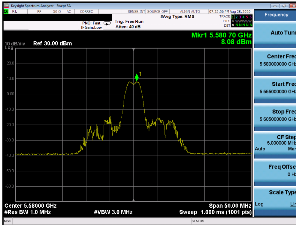
Plot 7-365. Power Spectral Density Plot Antenna 2b (20MHz BW 802.11ax Index 4 – RU26 (UNII Band 2C) – Ch. 116)
