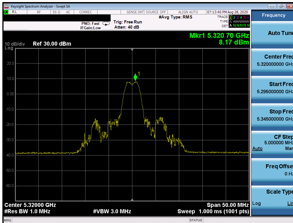
Plot 7-344. Power Spectral Density Plot Antenna 2b (20MHz BW 802.11ax Index 4 – RU26 (UNII Band 2A) – Ch. 64)
