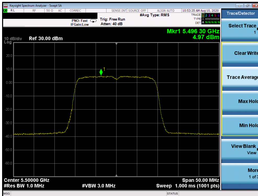
Plot 7-370. Power Spectral Density Plot Antenna 2b (20MHz BW 802.11ax– RU242 (UNII Band 2C) – Ch. 100)
