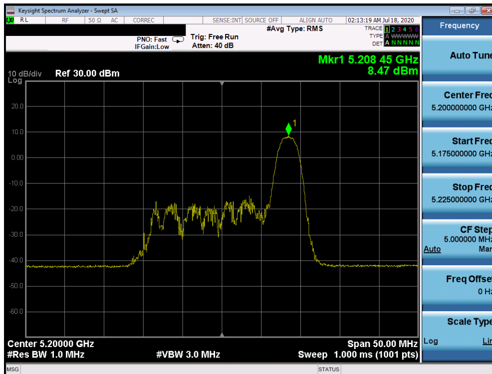
Plot 7-318. Power Spectral Density Plot Antenna 2b (20MHz BW 802.11ax Index 8– RU26 (UNII Band 1) – Ch. 40)
