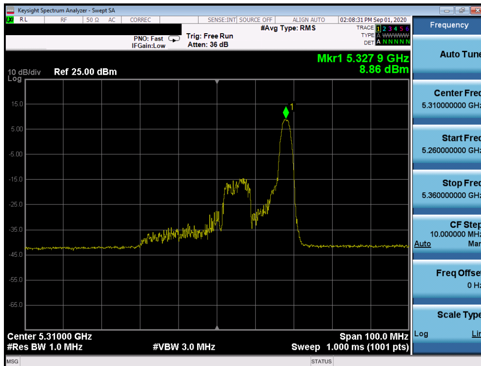
Plot 7-354. Power Spectral Density Plot Antenna 2b (40MHz BW 802.11ax Index 17 – RU26 (UNII Band 2A) – Ch. 62)
