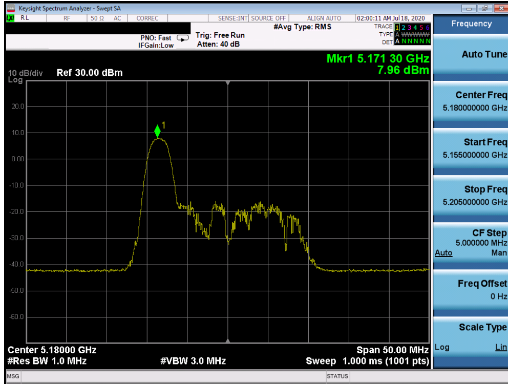
Plot 7-313. Power Spectral Density Plot Antenna 2b (20MHz BW 802.11ax Index 0 – RU26 (UNII Band 1) – Ch. 36)
