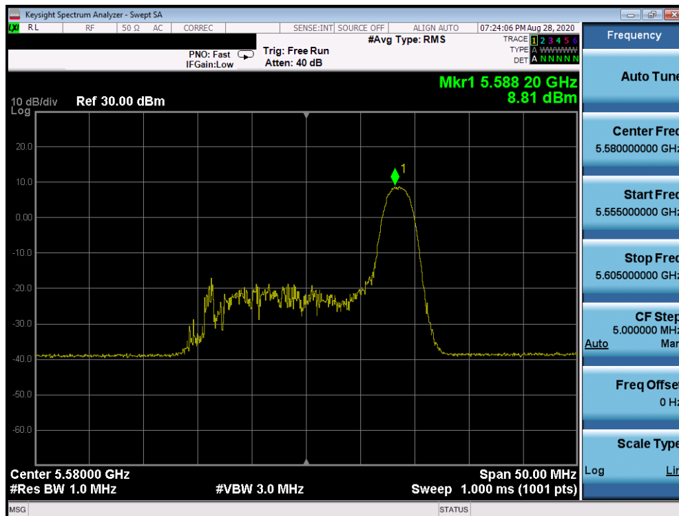
Plot 7-366. Power Spectral Density Plot Antenna 2b (20MHz BW 802.11ax Index 8– RU26 (UNII Band 2C) – Ch. 116)
