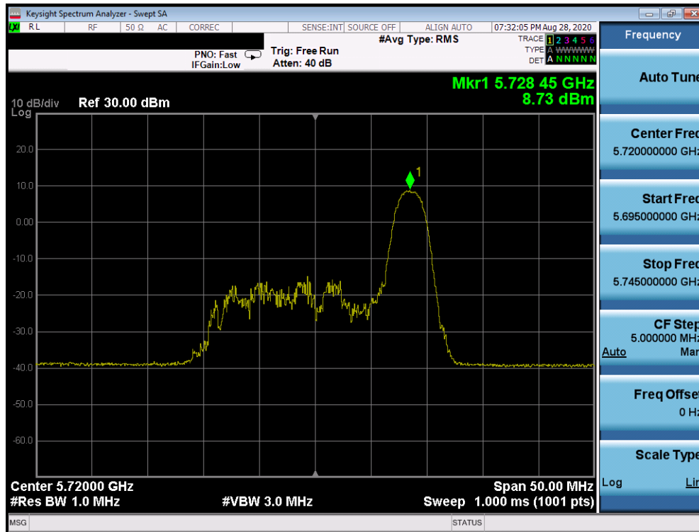
Plot 7-369. Power Spectral Density Plot Antenna 2b (20MHz BW 802.11ax Index 8 – RU26 (UNII Band 2C) – Ch. 144)
