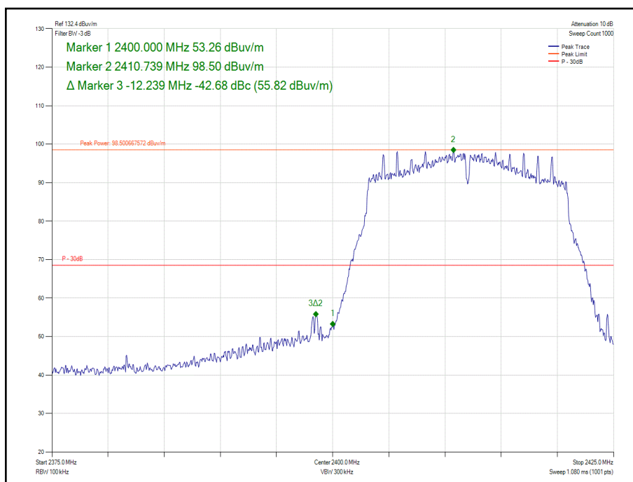
Figure 121- 802.11n HT20, Core 1- 2412 MHz Band Edge Frequency 2400 MHz
