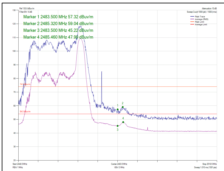
Figure 154 - 802.11ax HE20, Core 0-1, 26-8 - 2462 MHz, Band Edge Frequency 2483.5 MHz
