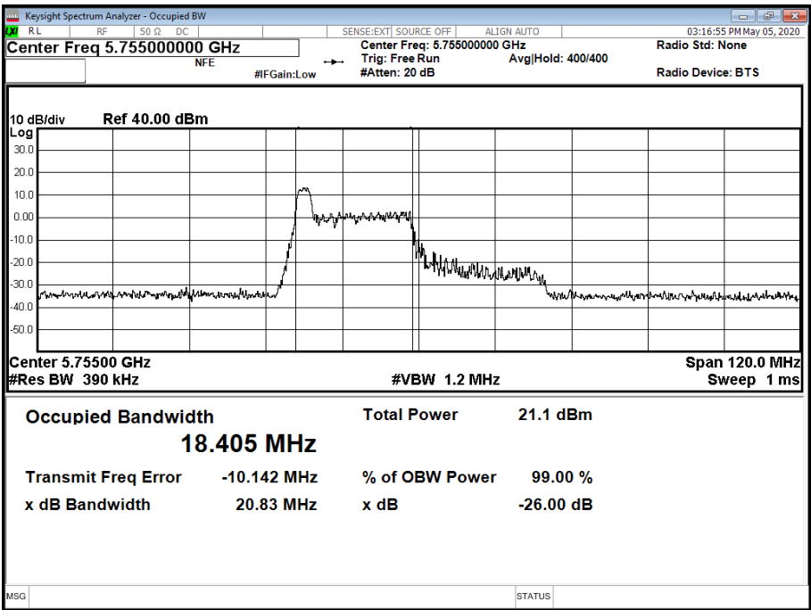
Figure 976 - 5755 MHz - 99% Occupied Bandwidth
