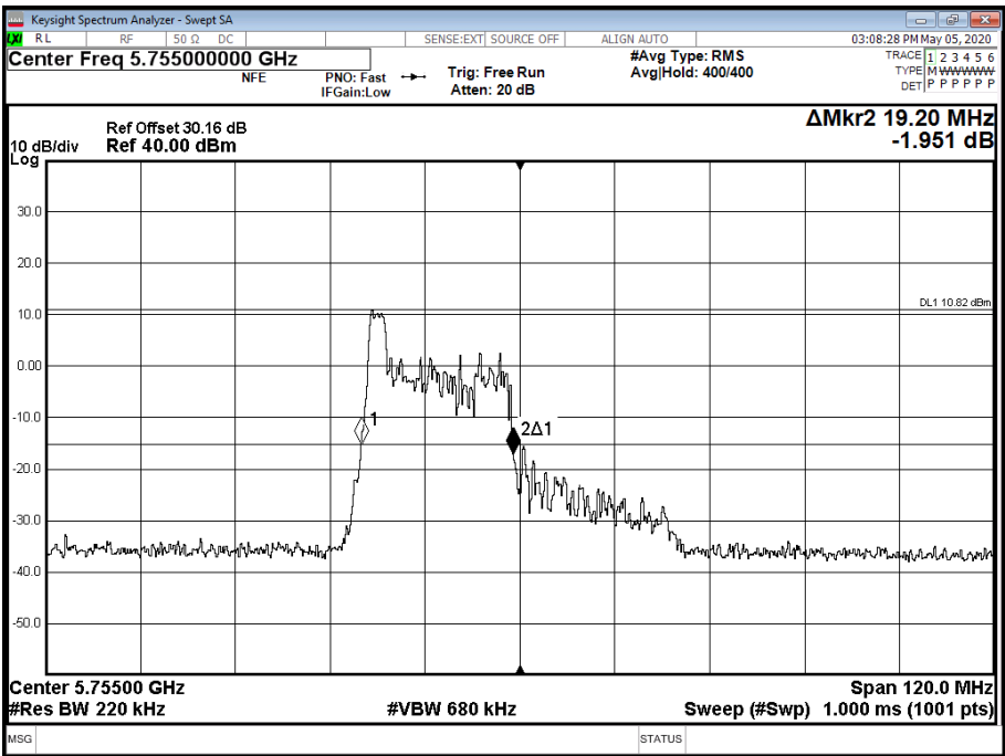
Figure 954 - 5755 MHz - 26 dB Emission Bandwidth
