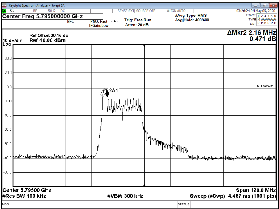
Figure 977 - 5795 MHz - 6 dB DTS Bandwidth
