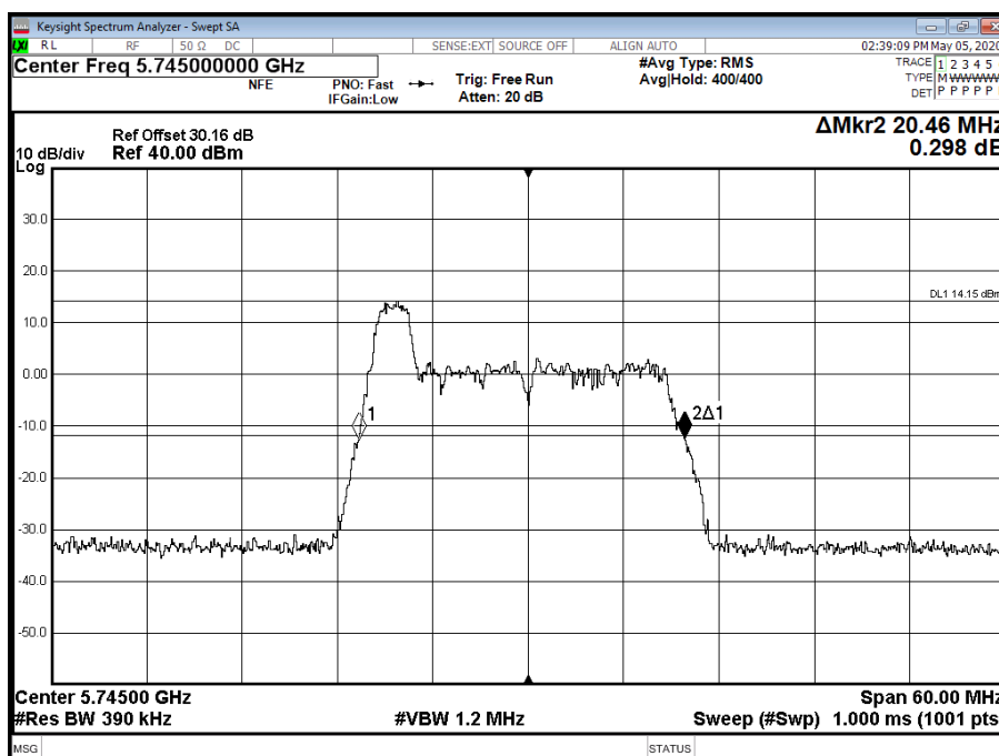
Figure 870 - 5745 MHz - 26 dB Emission Bandwidth
