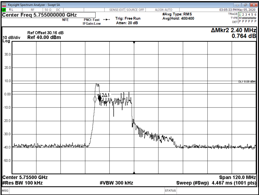
Figure 953 - 5755 MHz - 6 dB DTS Bandwidth
