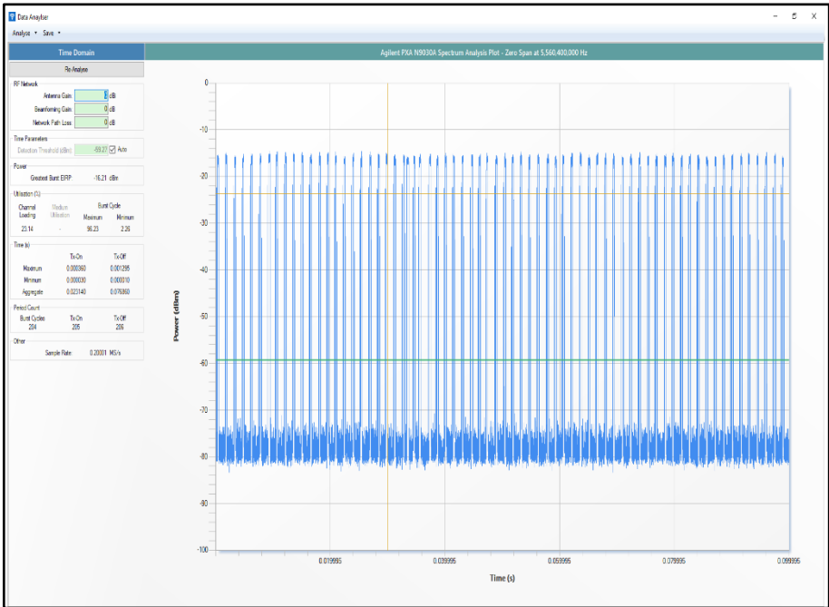
Figure 1099 - Channel Loading
