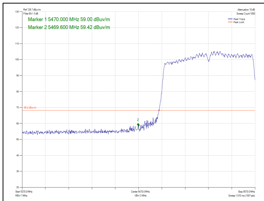
Figure 65 - 802.11ac VHT80 Core 0 - 5530 MHz Band Edge Frequency 5470 MHz
