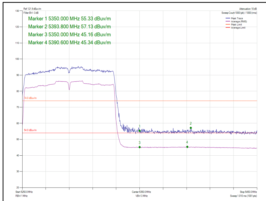
Figure 141 - 802.11ac VHT80, Core 0 - 5290 MHz Band Edge Frequency 5350 MHz
