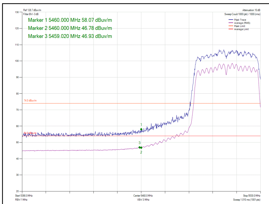
Figure 136 - 802.11n HT40 CDD, Cores 0-1 - 5510 MHz Band Edge Frequency 5460 MHz
