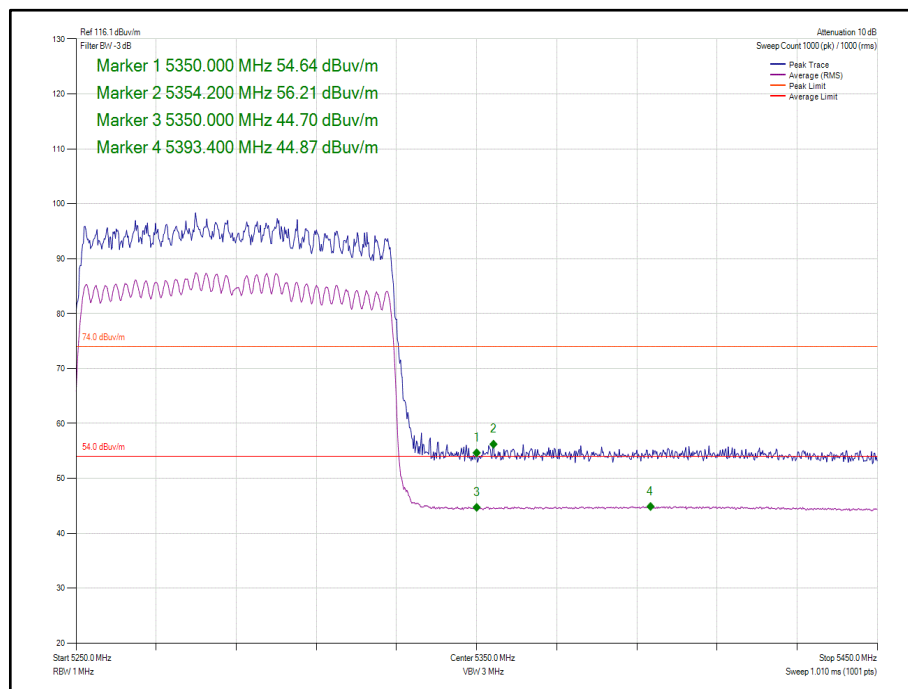
Figure 155 - 802.11ax HE80 CDD, Cores 0-1, SU - 5290 MHz Band Edge Frequency 5350 MHz
