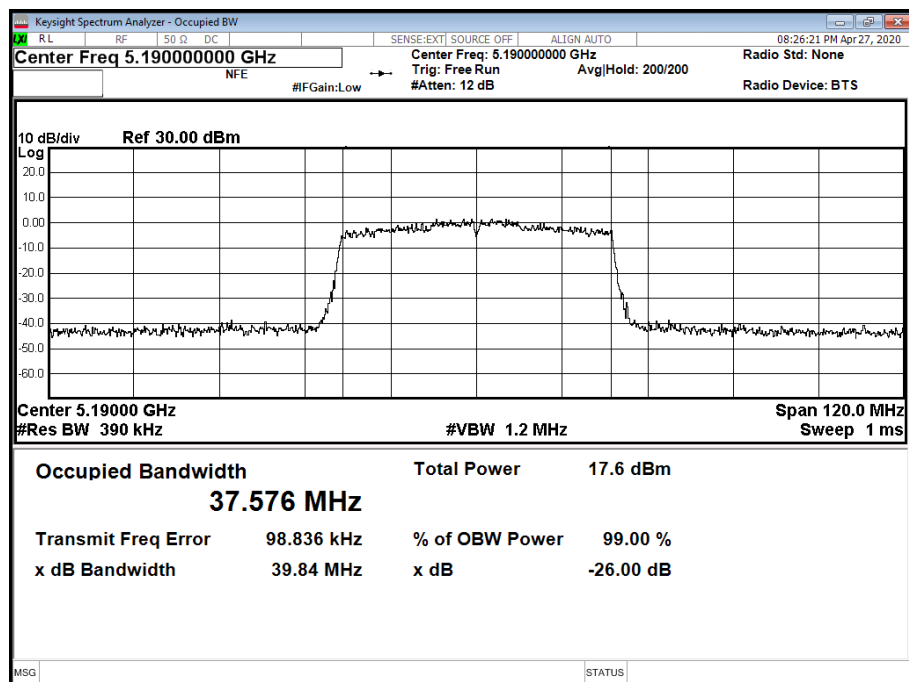
Figure 386 - 5190 MHz - 99% Occupied Bandwidth
