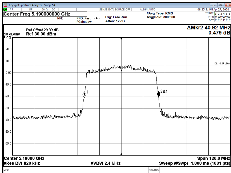
Figure 385 - 5190 MHz - 26 dB Emission Bandwidth
