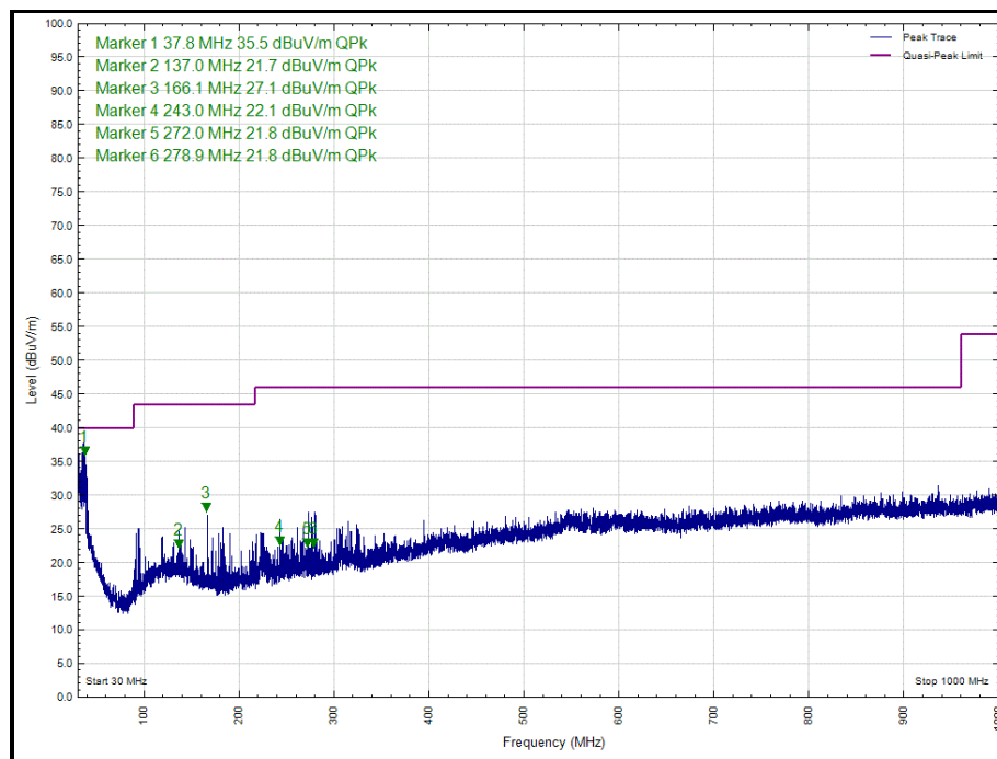
Figure 54 - Channel 17 (2440 MHz), LE1M, Core 0, 30 MHz to 1 GHz, Horizontal (Peak)
