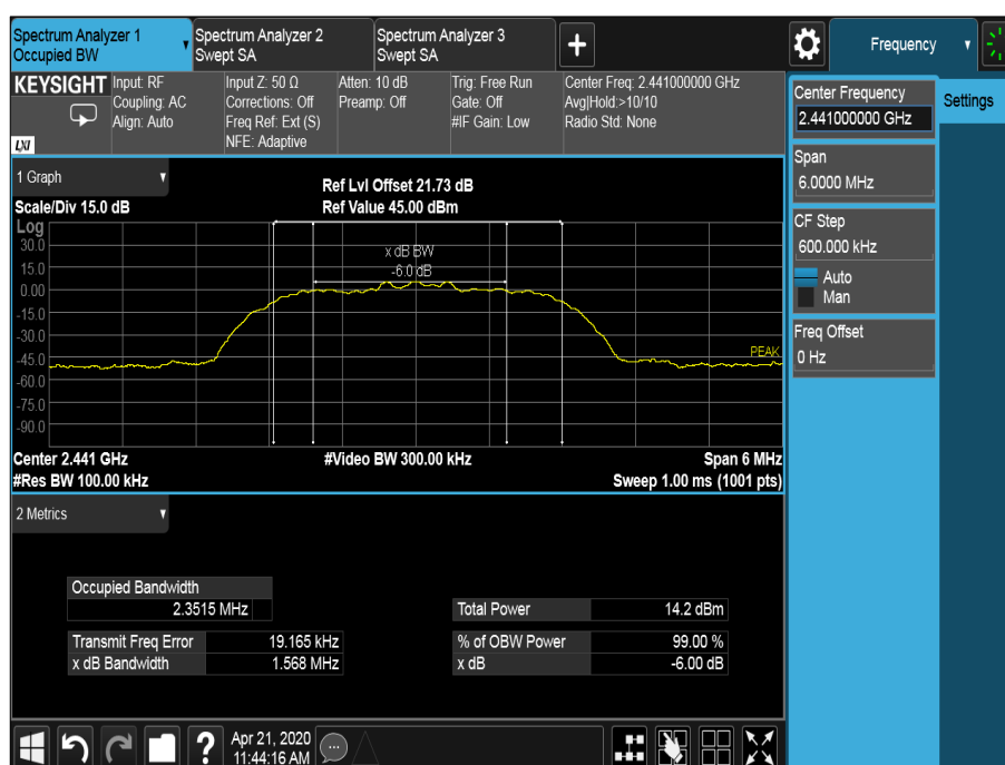
Figure 20 – 2441 MHz – Emission Bandwidth
