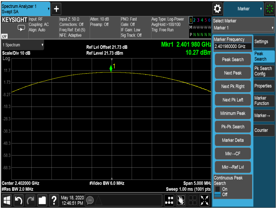
Figure 3 - 2402 MHz - Maximum Output Power, 8-DPSK
