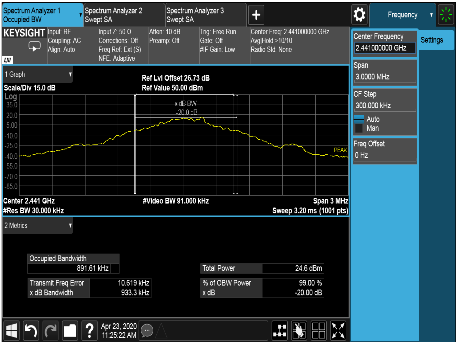
Figure 42 - 2441 MHz - GFSK
