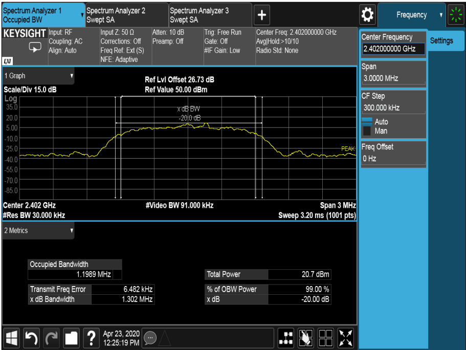
Figure 41 - 2402 MHz - 8-DPSK
