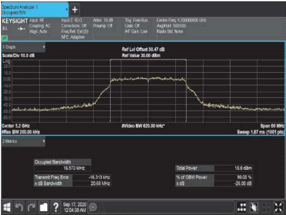
Figure 4 - 5200 MHz - 99 % Occupied Bandwidth h
