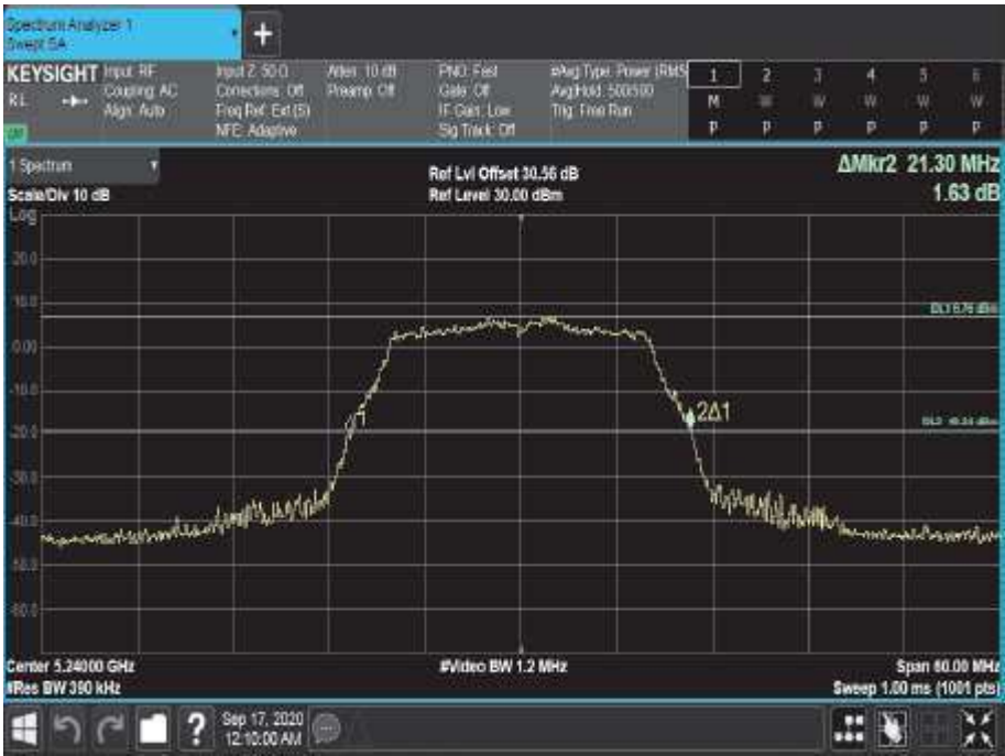
Figure 5 - 5240 MHz - 26 dB Emission Bandwidth h
