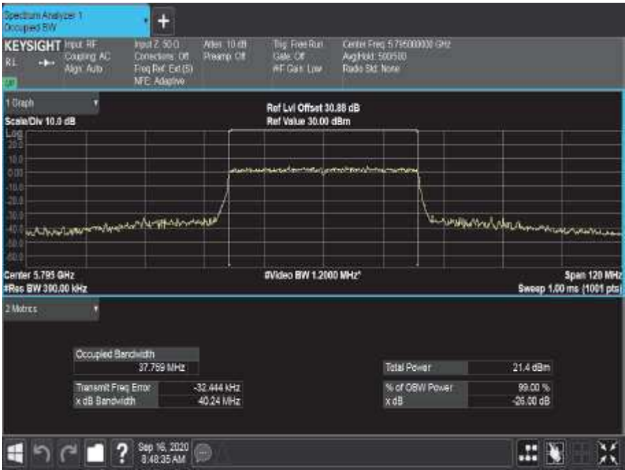
Figure 801 - 5795 MHz - 99% Occupied Bandwidth
