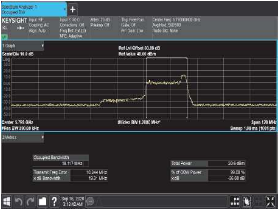
Figure 792 - 5795 MHz - 99% Occupied Bandwidth
