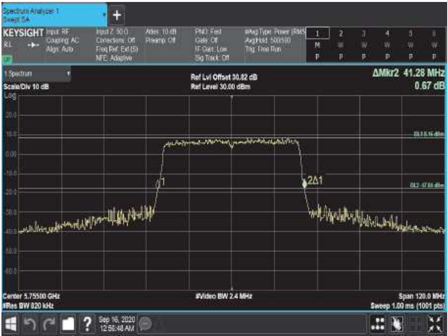
Figure 797 - 5755 MHz - 26 dB Emission Bandwidth
