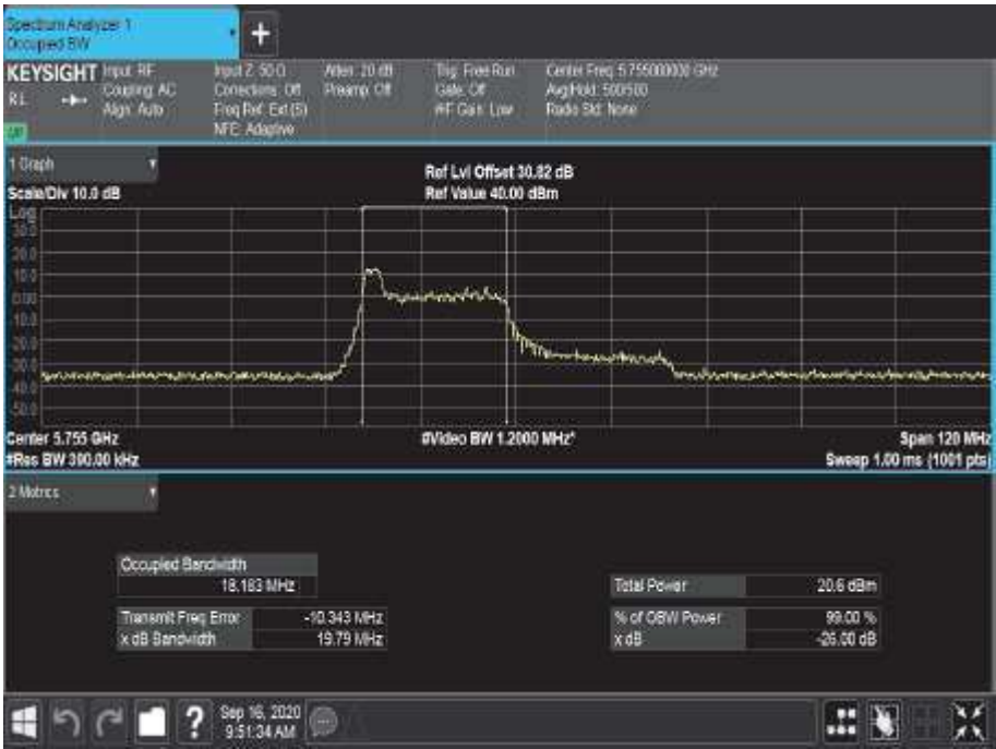
Figure 783 - 5755 MHz - 99% Occupied Bandwidth
