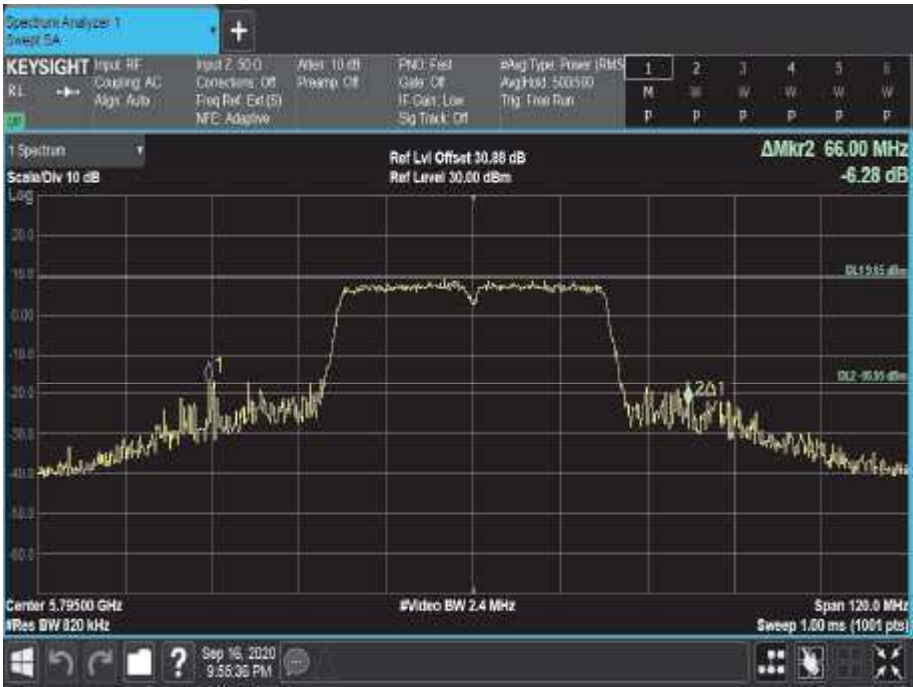
Figure 749 - 5795 MHz - 26 dB Emission Bandwidth
