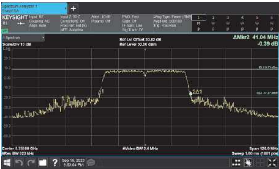
Figure 746 - 5755 MHz - 26 dB Emission Bandwidth
