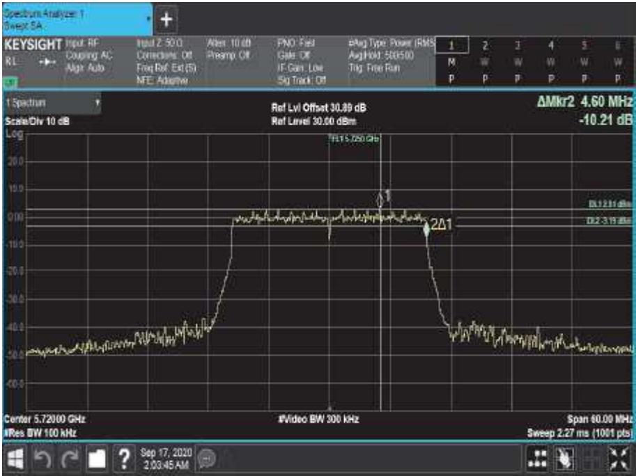
Figure 625 - 5720 MHz - 6 dB DTS Bandwidth
