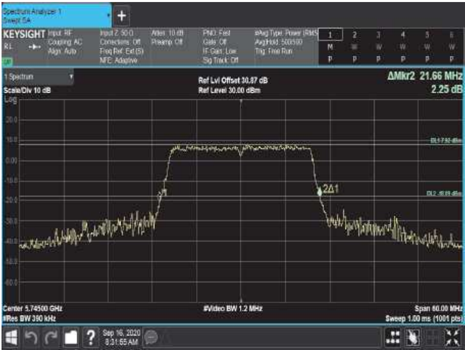
Figure 659 - 5745 MHz - 26 dB Emission Bandwidth
