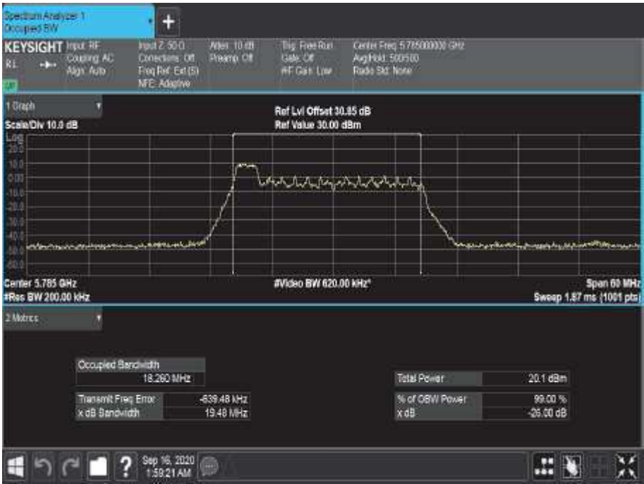
Figure 702 - 5785 MHz - 99% Occupied Bandwidth
