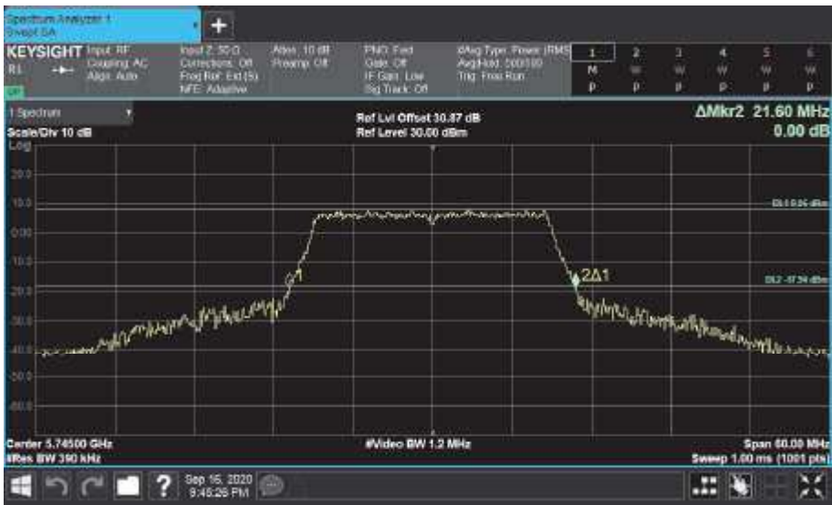
Figure 617 - 5745 MHz - 26 dB Emission Bandwidth
