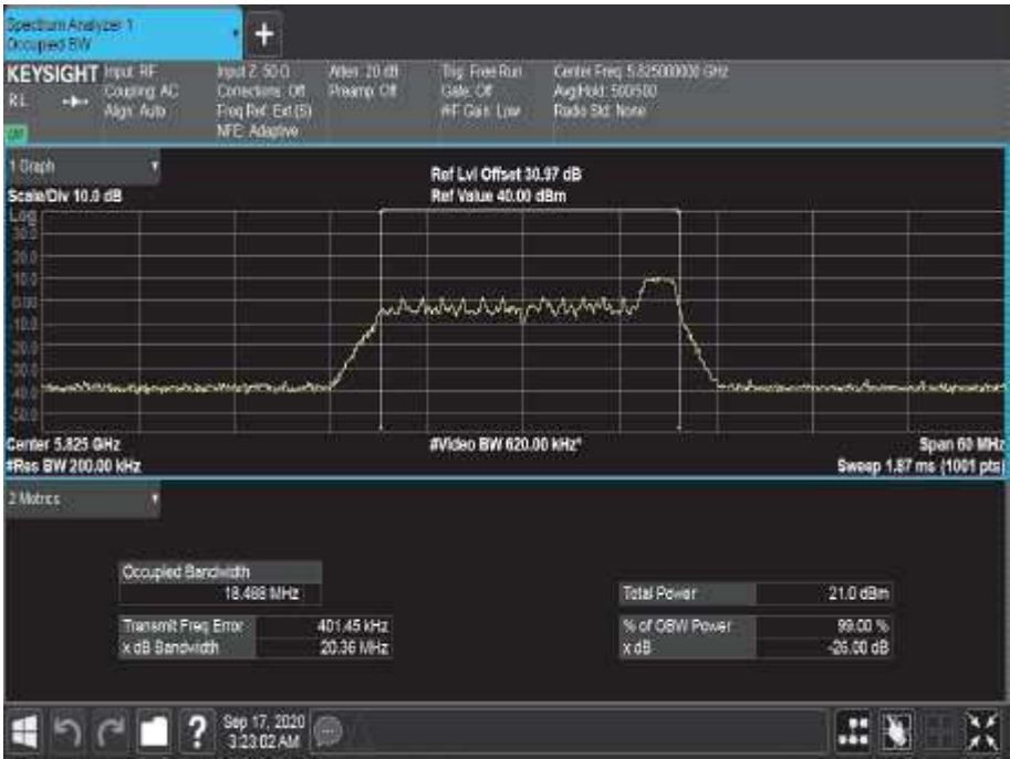
Figure 654 - 5825 MHz - 99% Occupied Bandwidth
