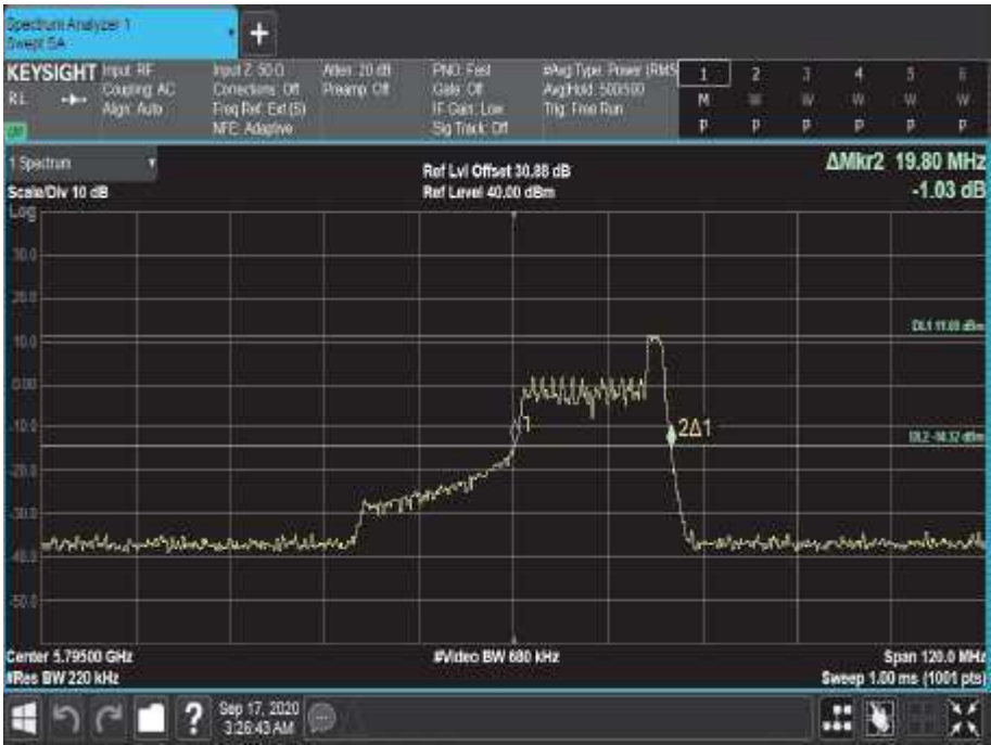
Figure 770 - 5795 MHz - 26 dB Emission Bandwidth
