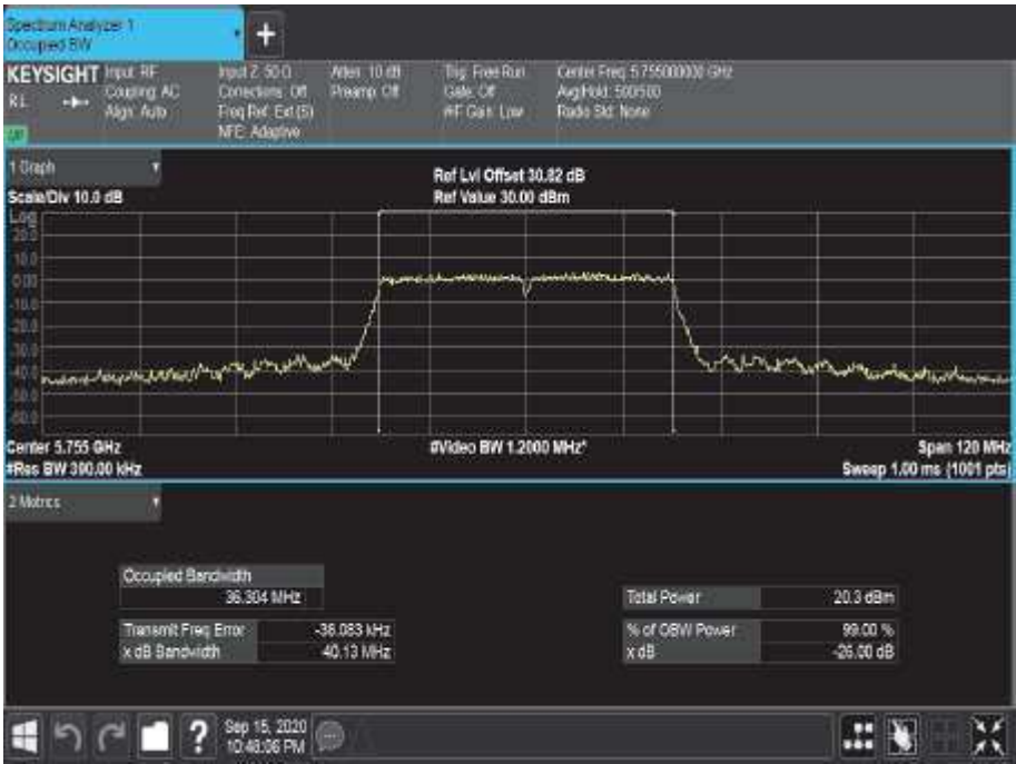
Figure 738 - 5755 MHz - 99% Occupied Bandwidth
