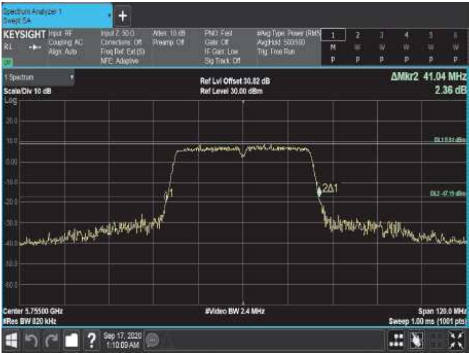
Figure 719 - 5755 MHz - 26 dB Emission Bandwidth
