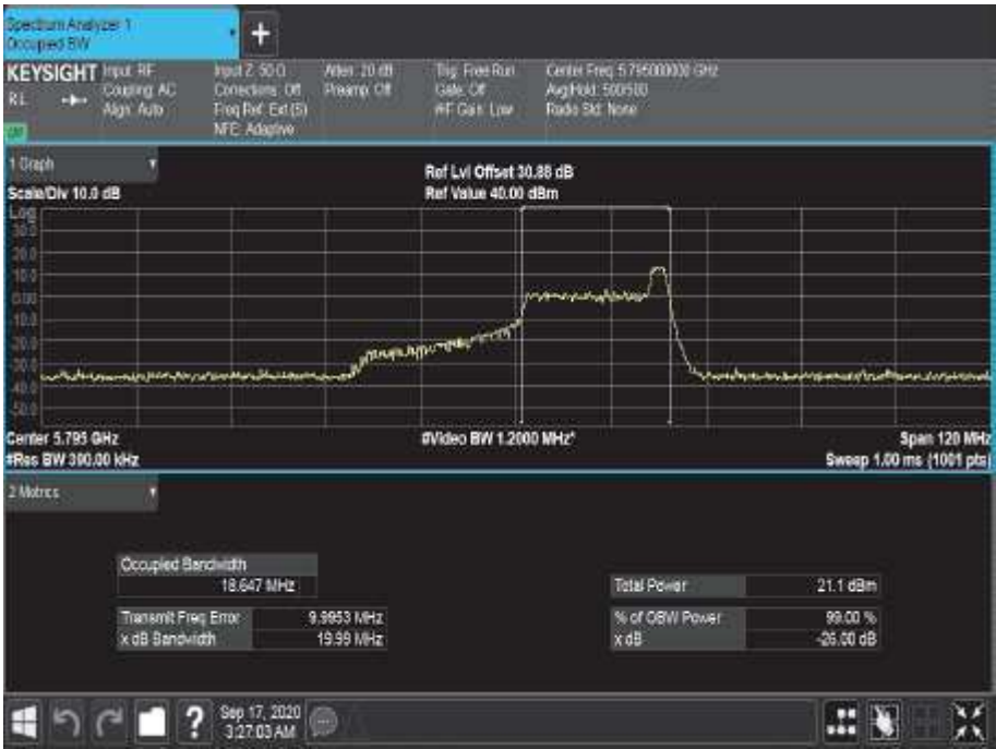
Figure 771 - 5795 MHz - 99% Occupied Bandwidth
