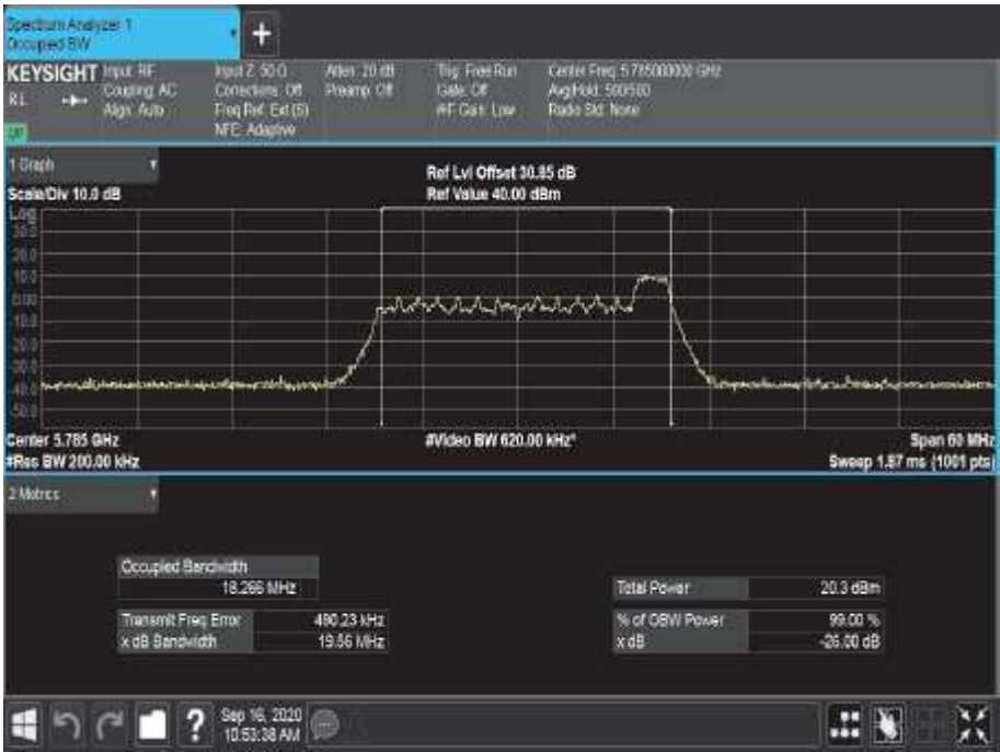
Figure 681 - 5785 MHz - 99% Occupied Bandwidth
