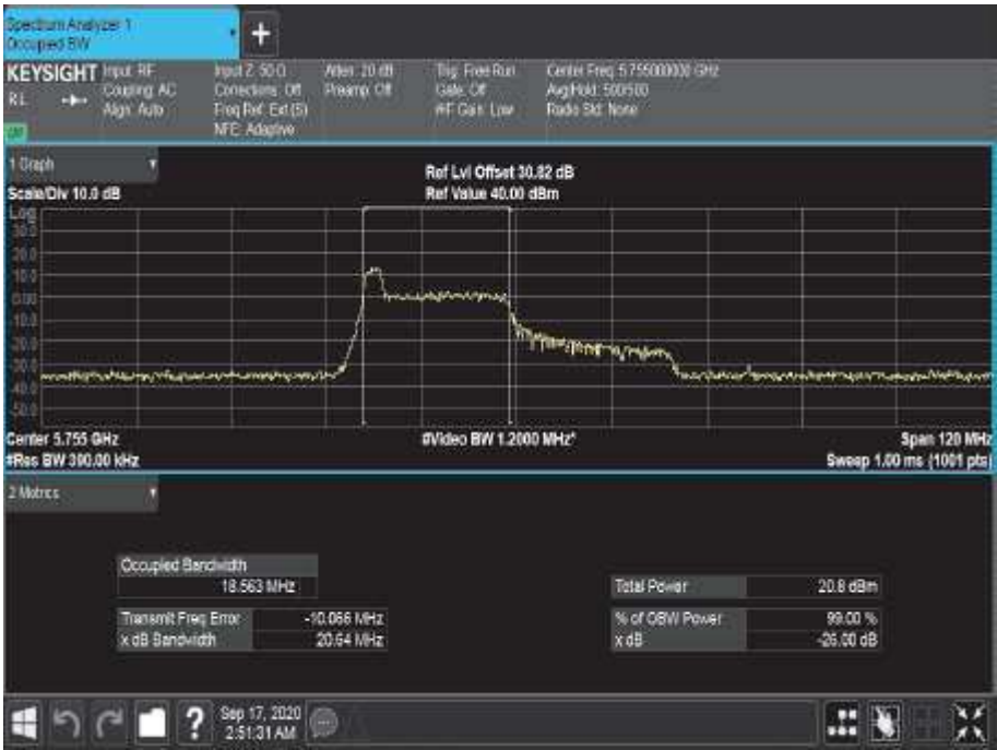
Figure 762 - 5755 MHz - 99% Occupied Bandwidth
