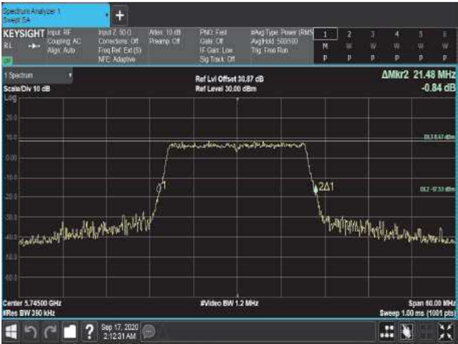
Figure 629 - 5745 MHz - 26 dB Emission Bandwidth
