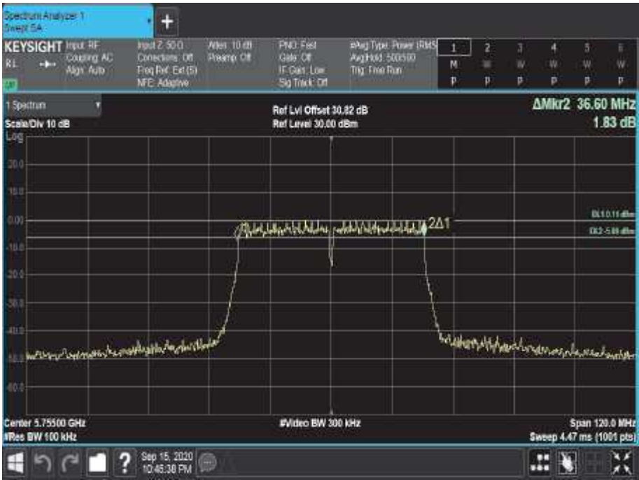
Figure 727 - 5755 MHz - 6 dB DTS Bandwidth
