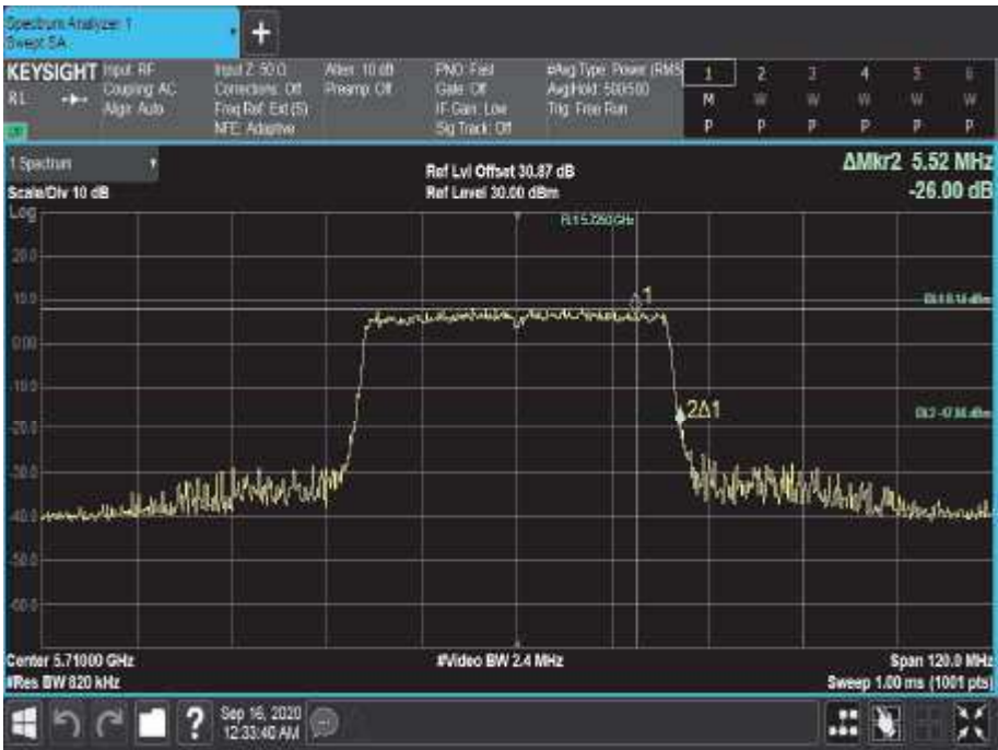
Figure 773 - 5710 MHz - 26 dB Emission Bandwidth
