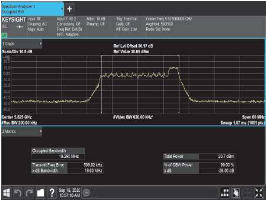
Figure 684 - 5825 MHz - 99% Occupied Bandwidth
