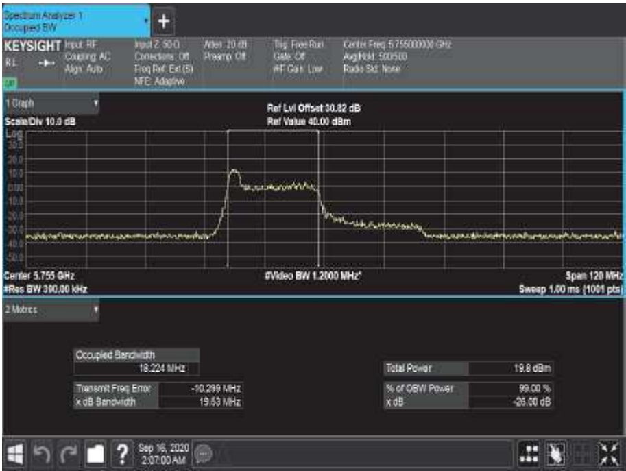
Figure 804 - 5755 MHz - 99% Occupied Bandwidth
