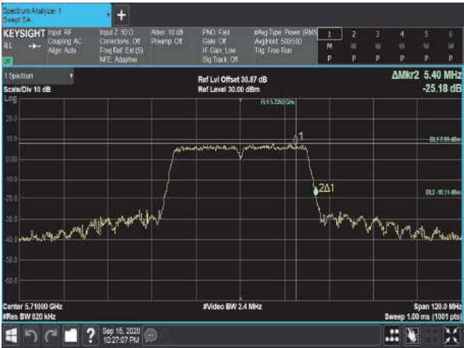
Figure 734 - 5710 MHz - 26 dB Emission Bandwidth
