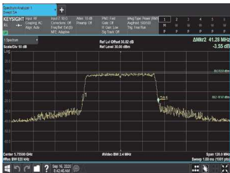
Figure 776 - 5755 MHz - 26 dB Emission Bandwidth
