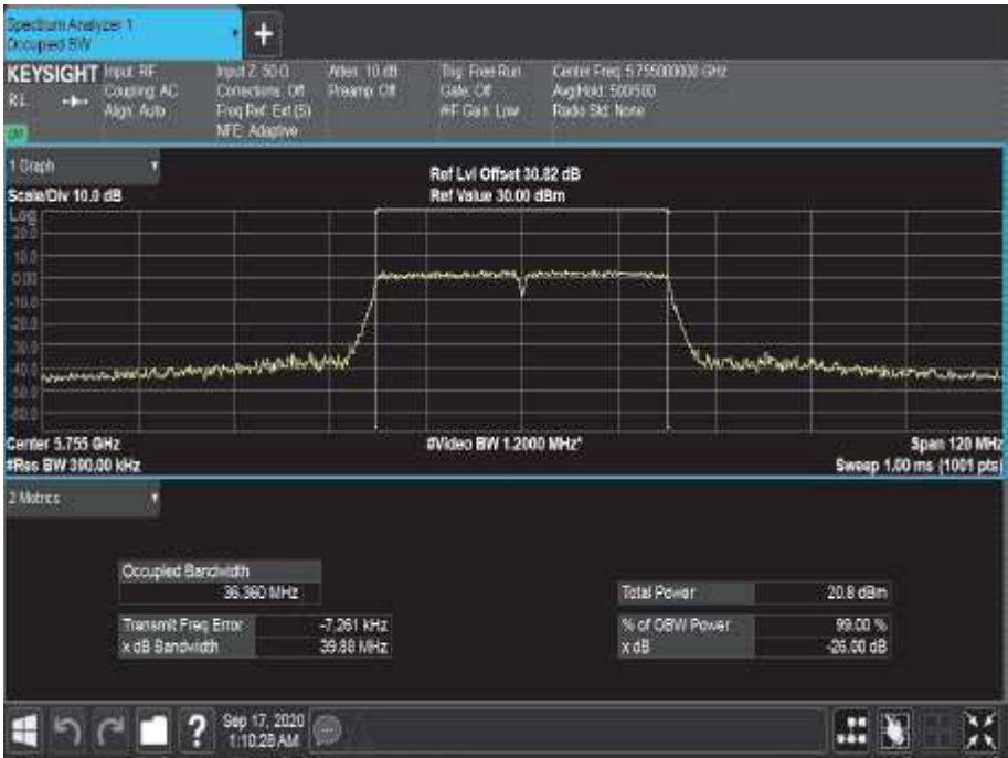
Figure 720 - 5755 MHz - 99% Occupied Bandwidth
