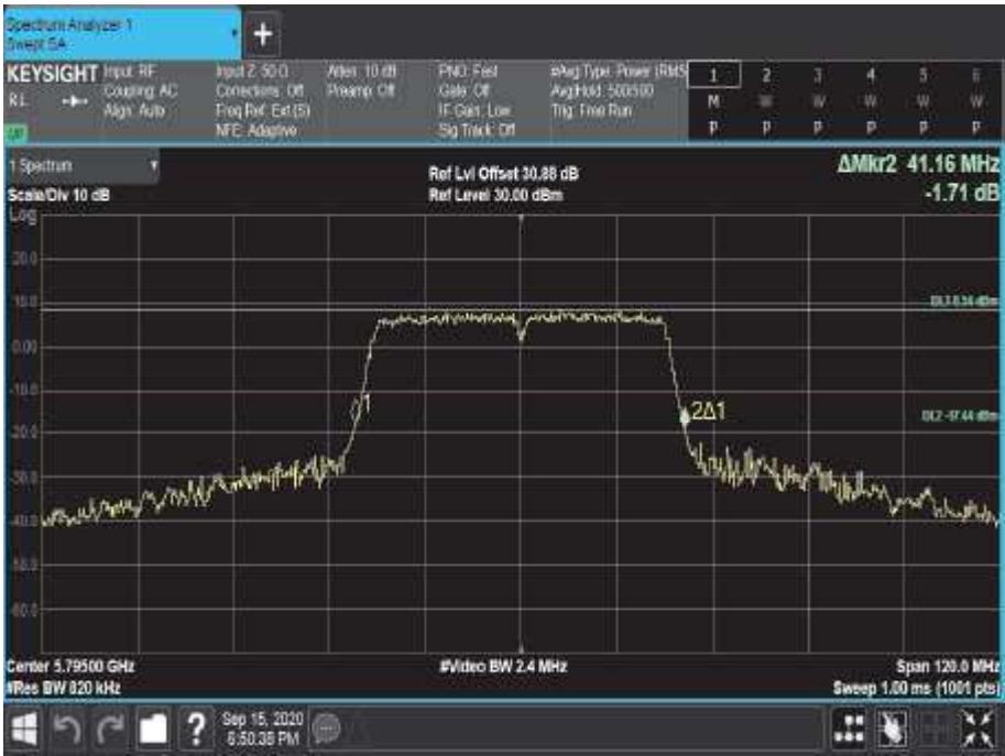
Figure 731 - 5795 MHz - 26 dB Emission Bandwidth
