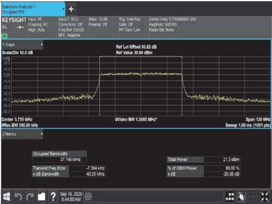
Figure 798 - 5755 MHz - 99% Occupied Bandwidth
