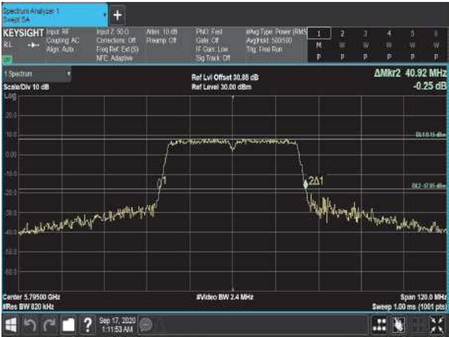
Figure 722 - 5795 MHz - 26 dB Emission Bandwidth
