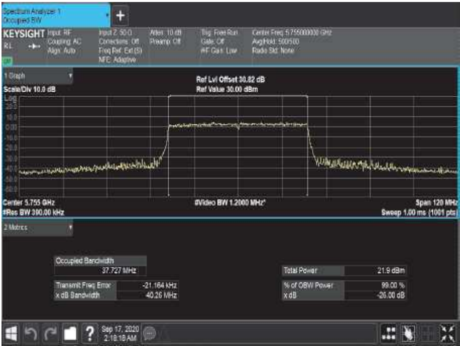
Figure 756 - 5755 MHz - 99% Occupied Bandwidth
