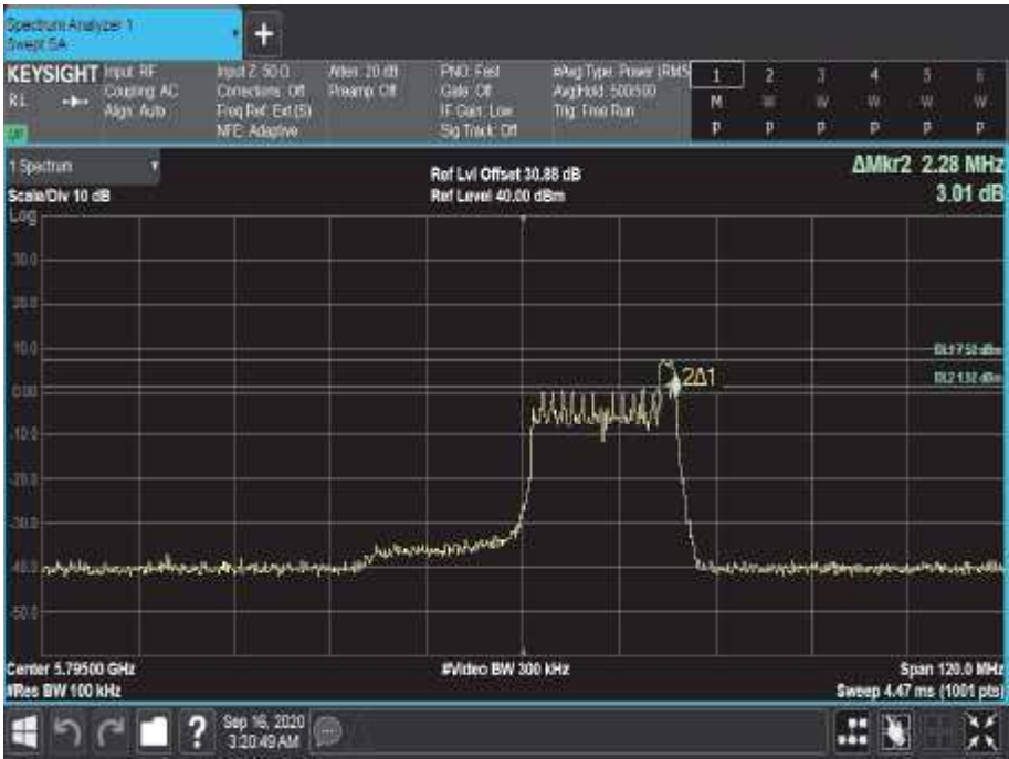
Figure 811 - 5795 MHz - 6 dB DTS Bandwidth
