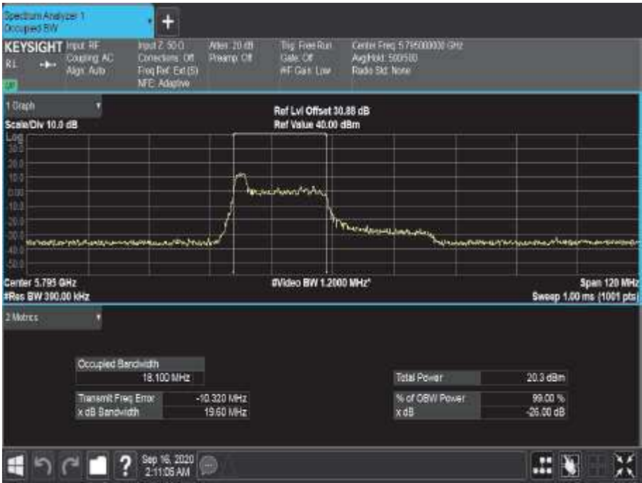
Figure 807 - 5795 MHz - 99% Occupied Bandwidth
