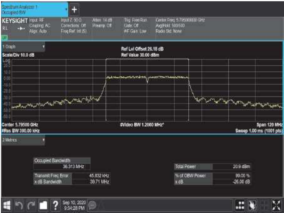
Figure 741 - 5795 MHz - 99% Occupied Bandwidth
