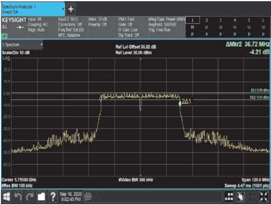
Figure 745 - 5755 MHz - 6 dB DTS Bandwidth
