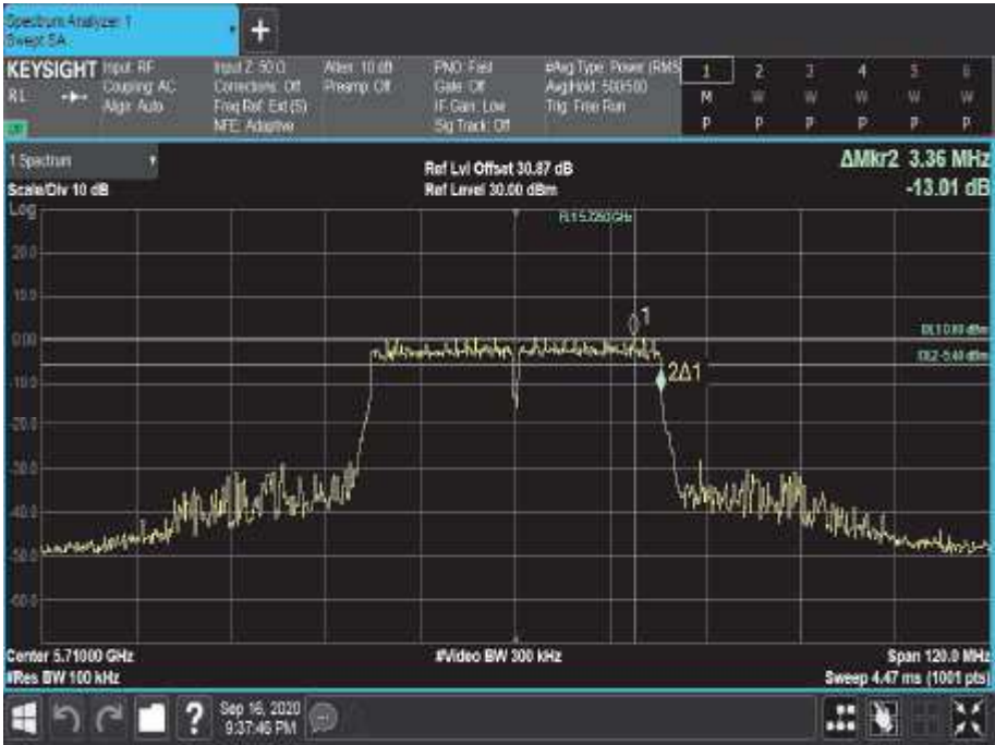
Figure 742 - 5710 MHz - 6 dB DTS Bandwidth
