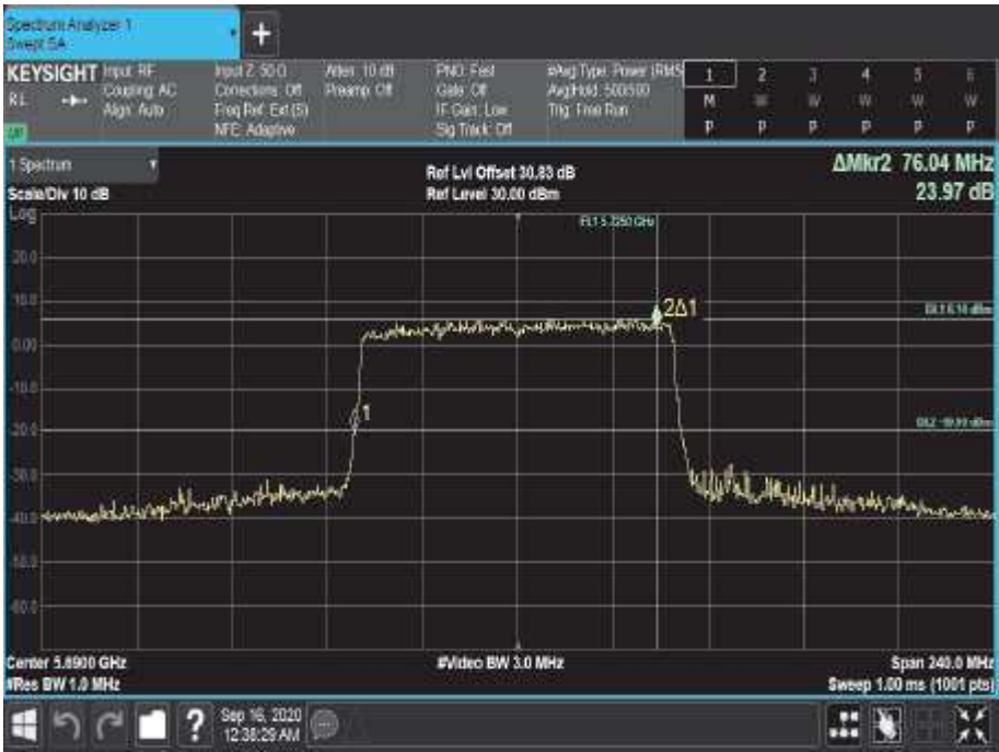
Figure 575 - 5690 MHz - 26 dB Emission Bandwidth
