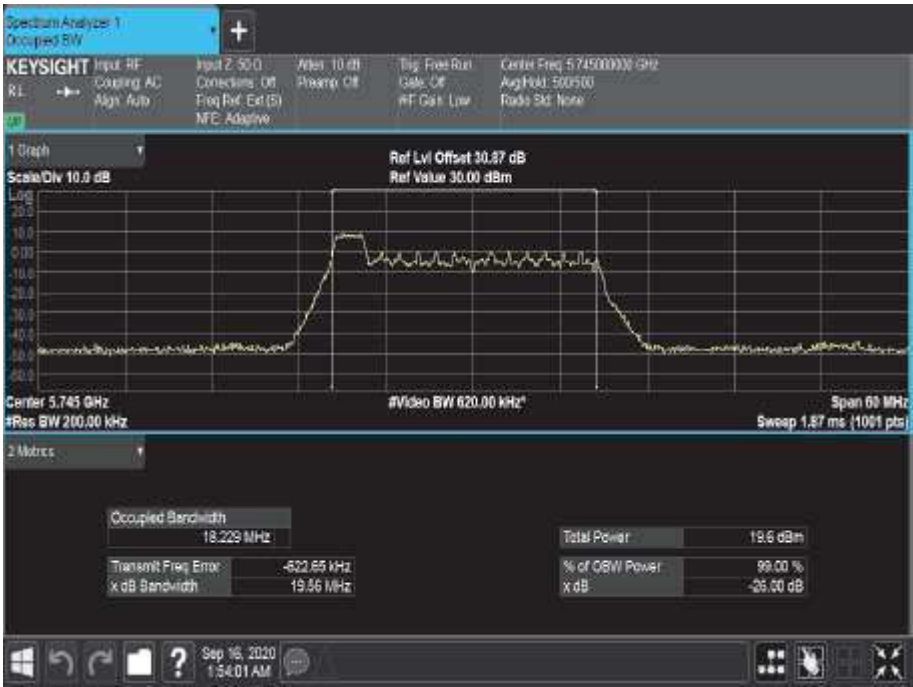
Figure 669 - 5745 MHz - 99% Occupied Bandwidth
