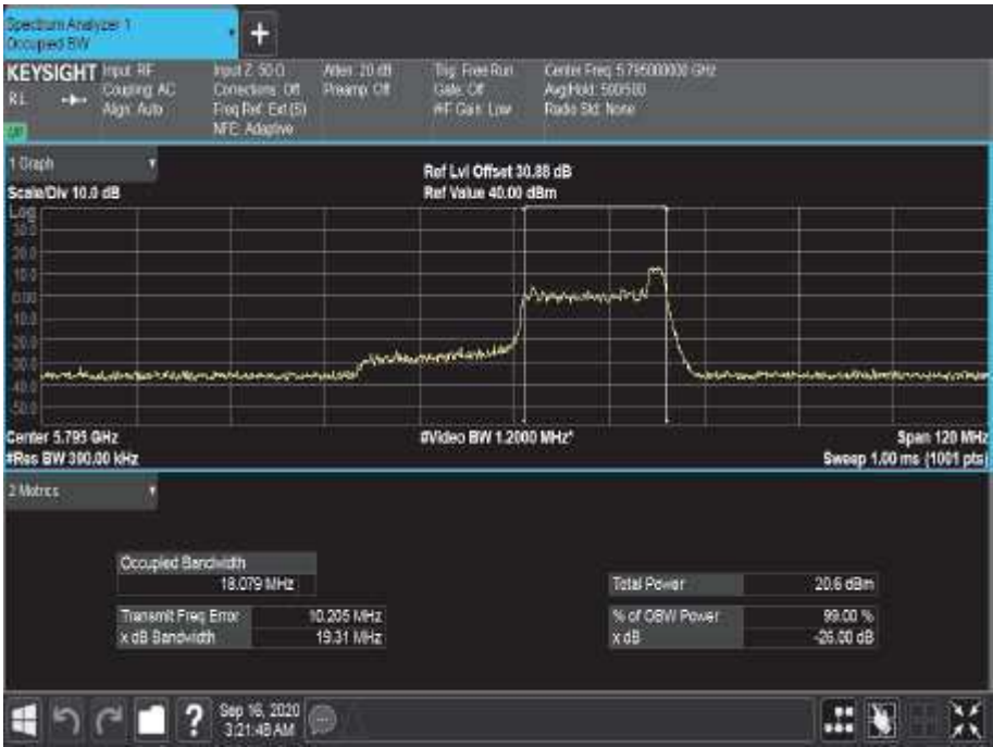
Figure 813 - 5795 MHz - 99% Occupied Bandwidth
