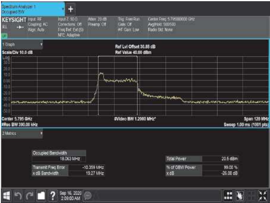
Figure 786 - 5795 MHz - 99% Occupied Bandwidth
