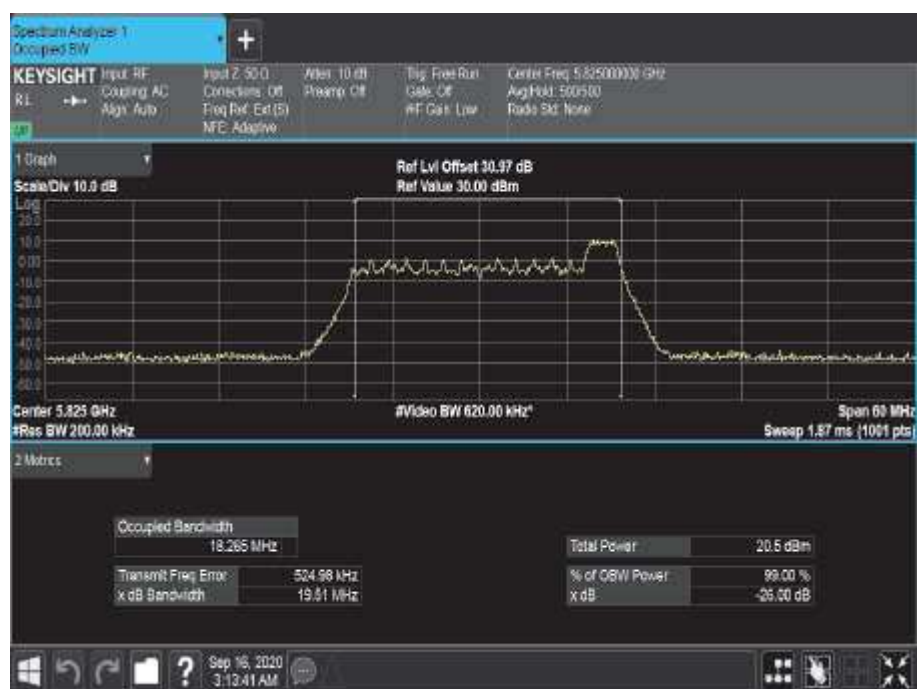
Figure 714 - 5825 MHz - 99% Occupied Bandwidth
