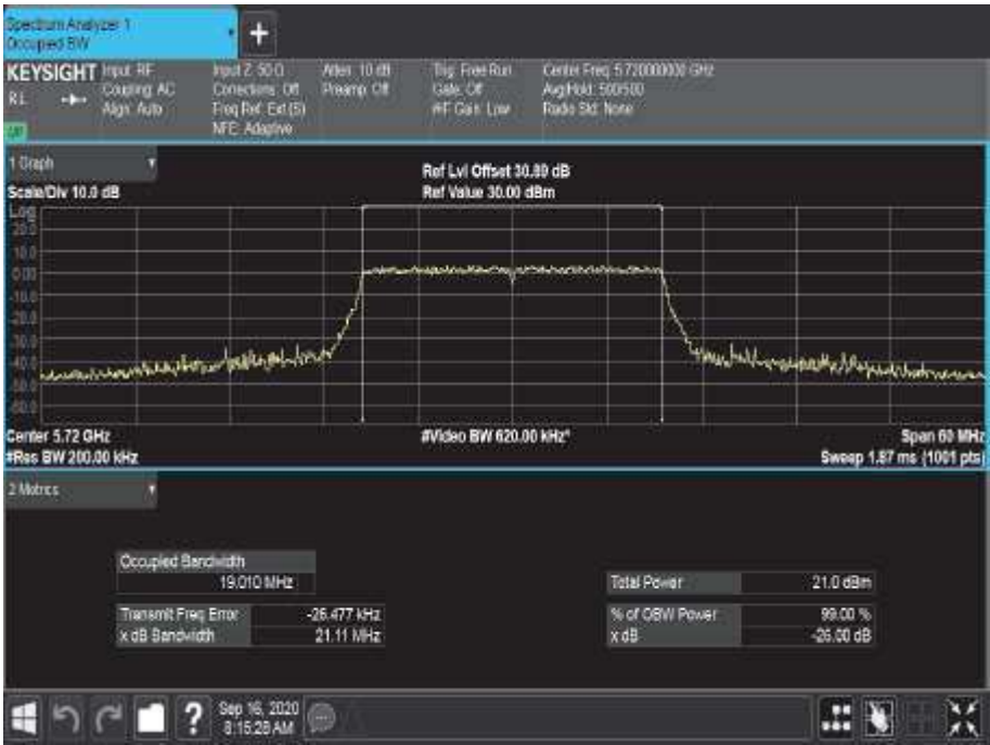
Figure 657 - 5720 MHz - 99% Occupied Bandwidth
