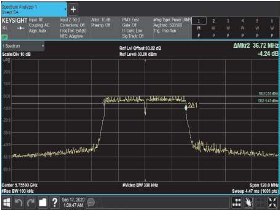
Figure 718 - 5755 MHz - 6 dB DTS Bandwidth
