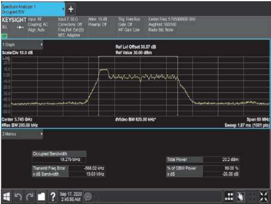
Figure 639 - 5745 MHz - 99% Occupied Bandwidth
