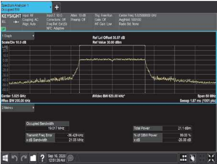
Figure 666 - 5825 MHz - 99% Occupied Bandwidth
