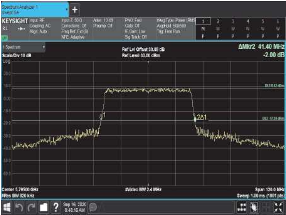
Figure 800 - 5795 MHz - 26 dB Emission Bandwidth
