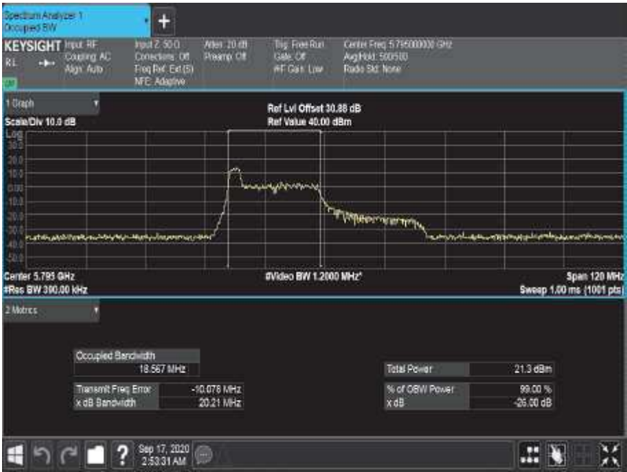
Figure 765 - 5795 MHz - 99% Occupied Bandwidth
