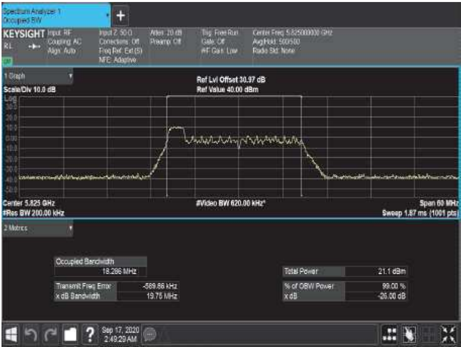
Figure 645 - 5825 MHz - 99% Occupied Bandwidth
