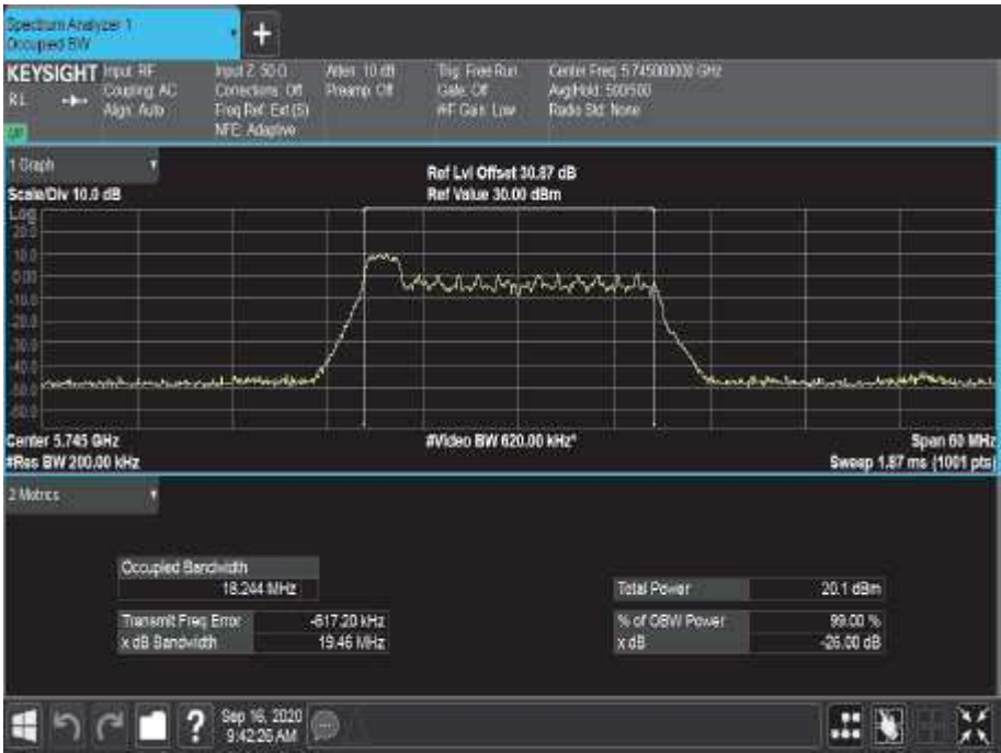
Figure 699 - 5745 MHz - 99% Occupied Bandwidth
