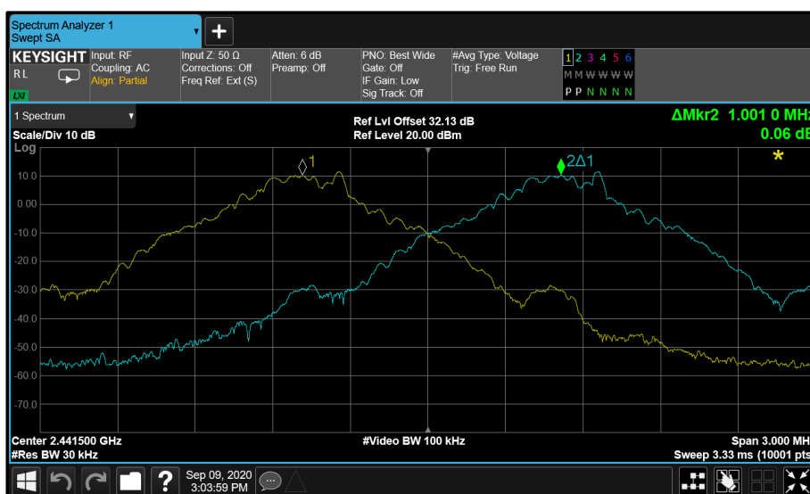
Figure 6 - GFSK - 2441 MHz (CH 39)
