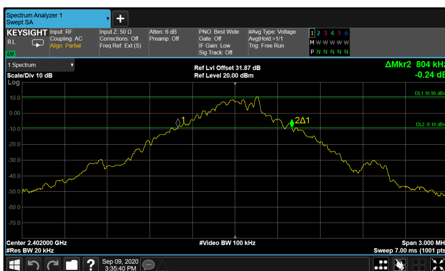
Figure 48 - Core 0 GFSK 2402 MHz (CH0)
