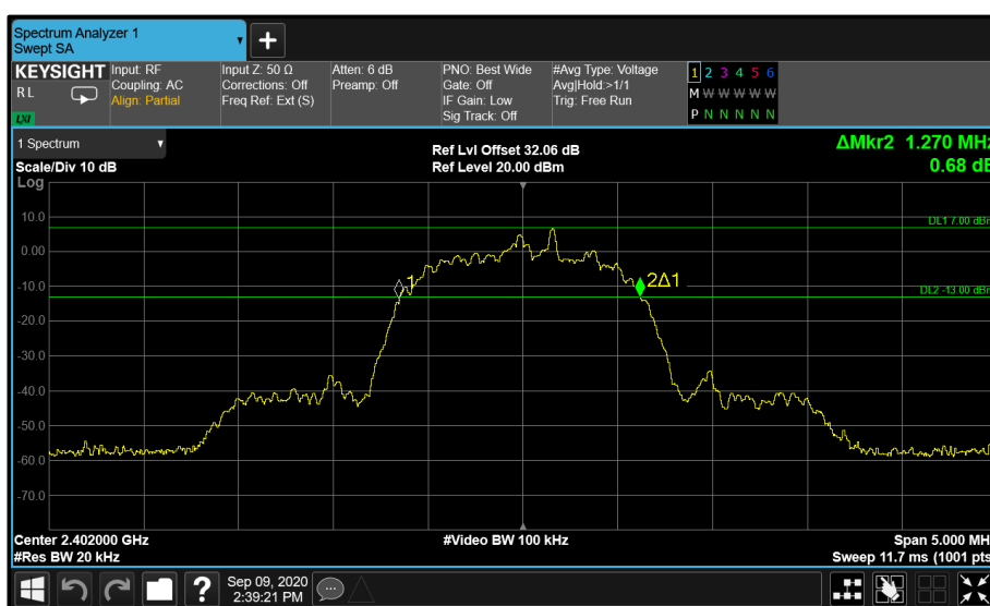
Figure 35 - Core 1 8-DPSK 2402 MHz (CH0)
