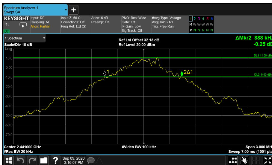
Figure 13 - Core 1 GFSK 2441 MHz (CH39)
