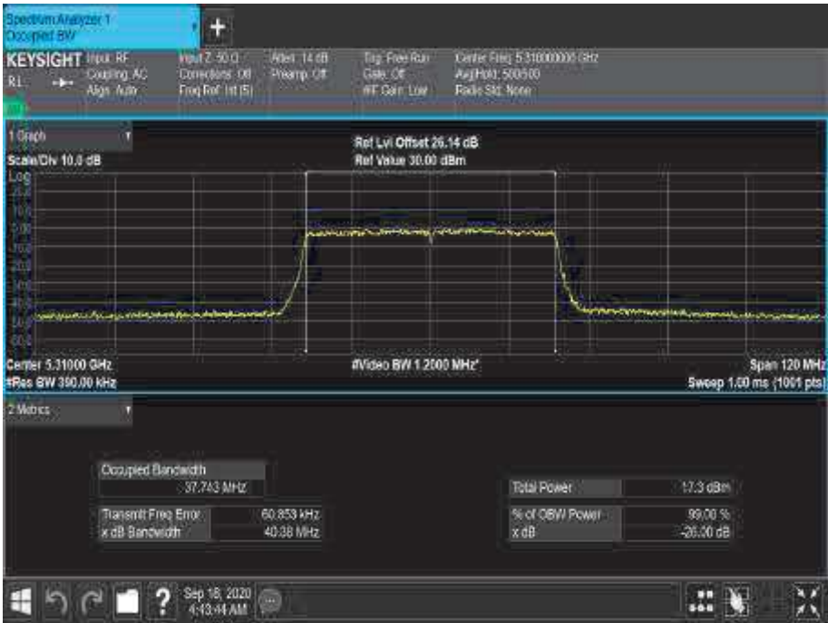
Figure 252 - 5310 MHz - 99% Occupied Bandwidth
