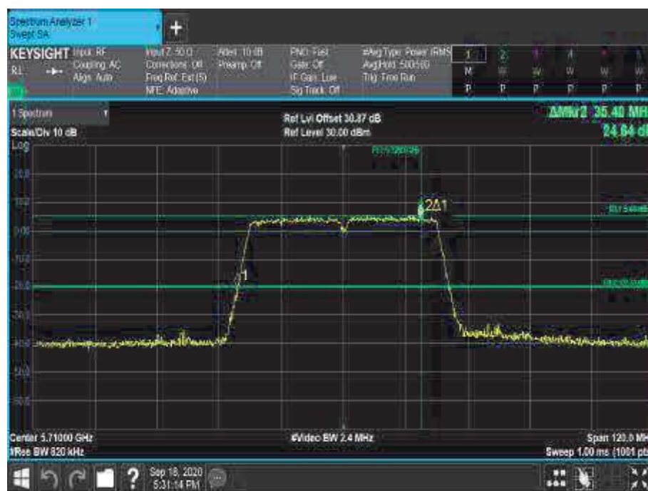
Figure 365 - 5710 MHz - 26 dB Emission Bandwidth
