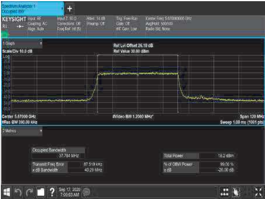
Figure 388 - 5670 MHz - 99% Occupied Bandwidth
