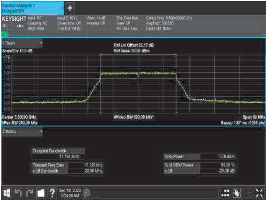
Figure 288 - 5500 MHz - 99% Occupied Bandwidth
