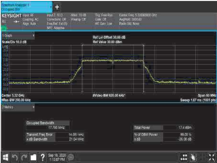
Figure 210 - 5320 MHz - 99% Occupied Bandwidth
