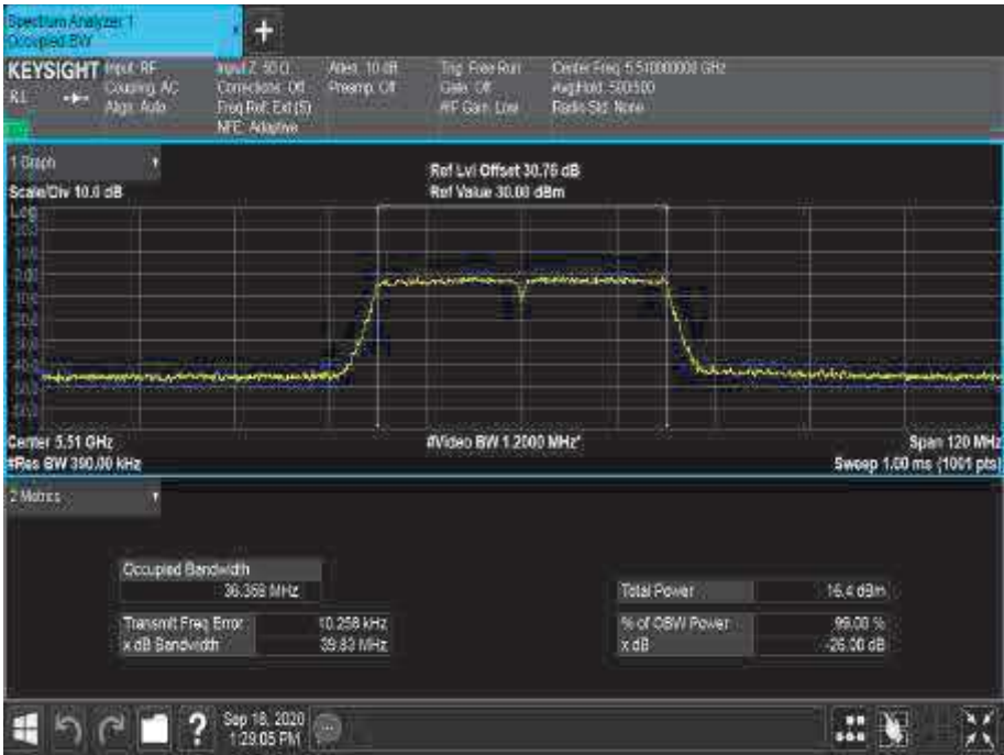
Figure 360 - 5510 MHz - 99% Occupied Bandwidth
