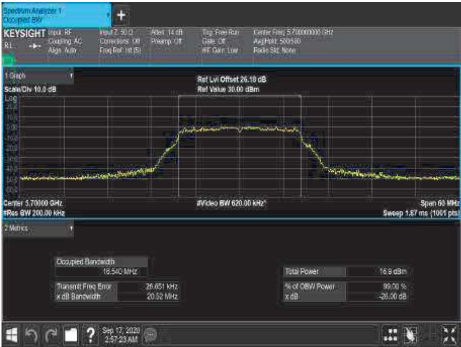
Figure 276 - 5700 MHz - 99% Occupied Bandwidth
