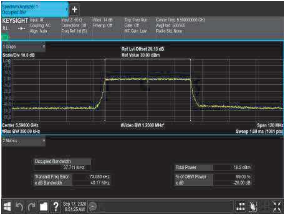
Figure 370 - 5590 MHz - 99% Occupied Bandwidth
