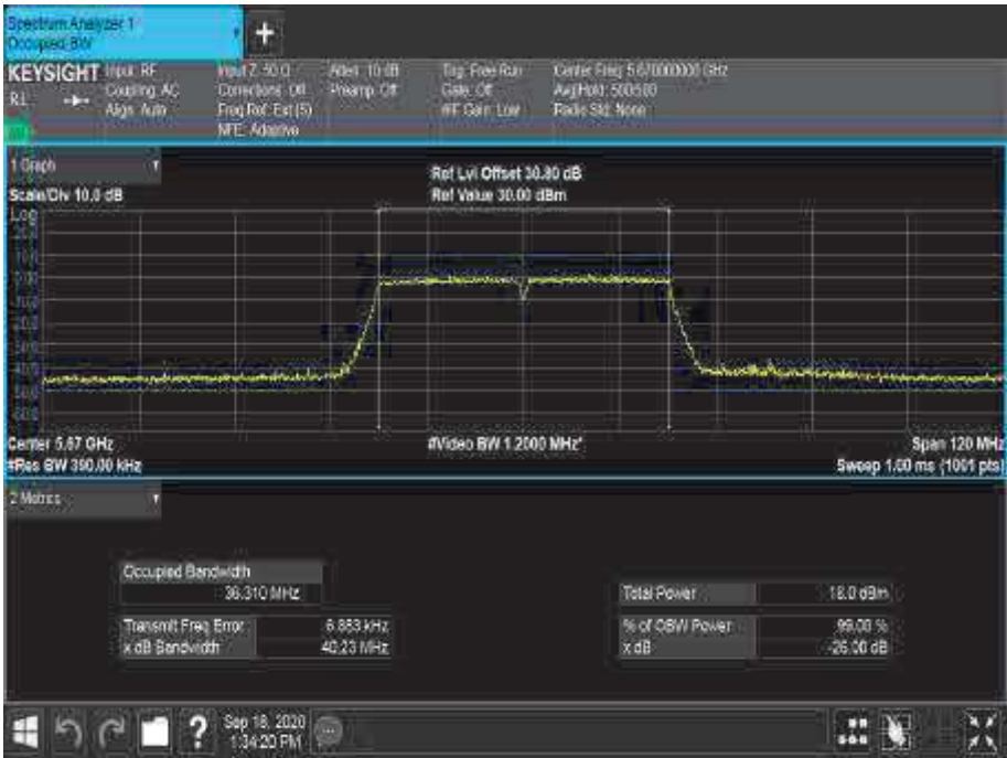
Figure 364 - 5670 MHz - 99% Occupied Bandwidth
