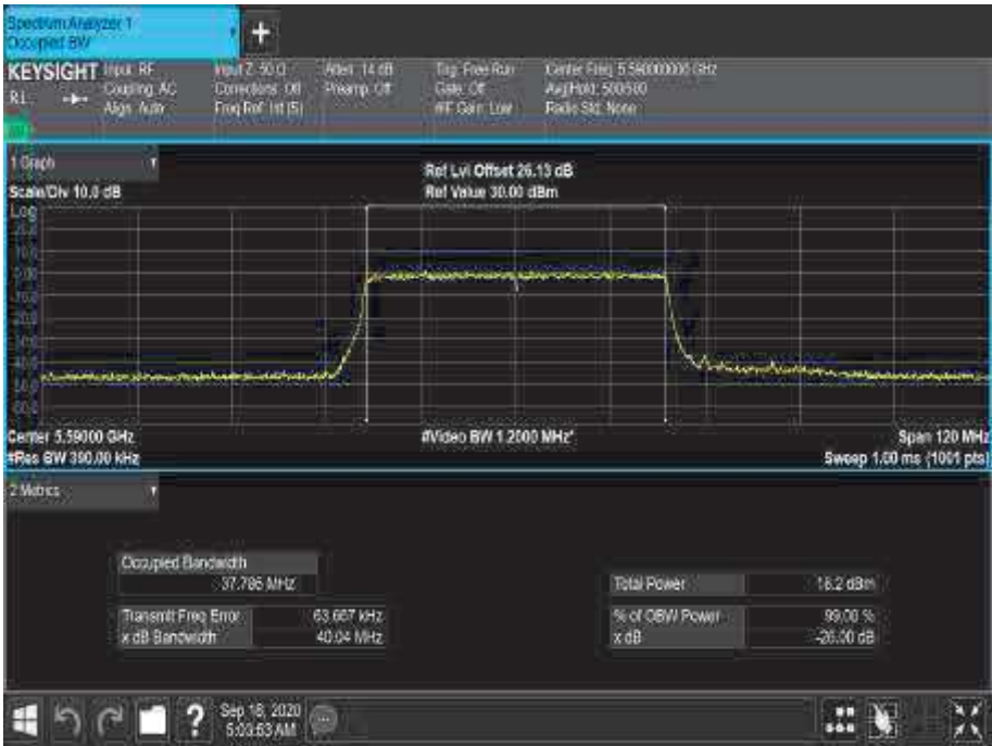
Figure 386 - 5590 MHz - 99% Occupied Bandwidth
