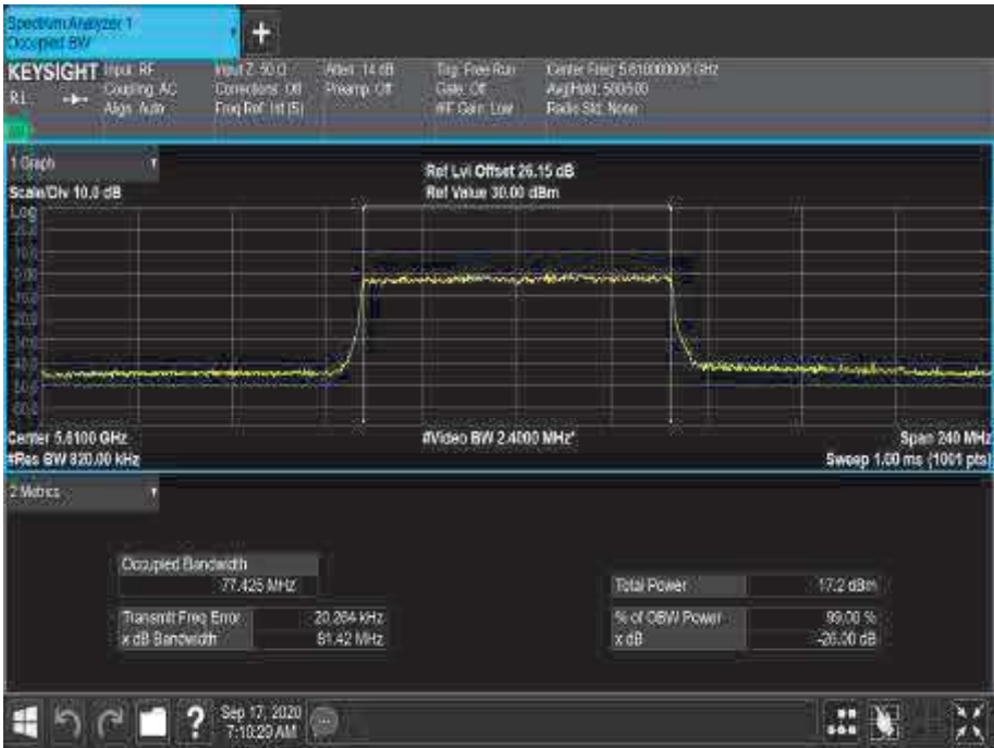
Figure 430 - 5610 MHz - 99% Occupied Bandwidth
