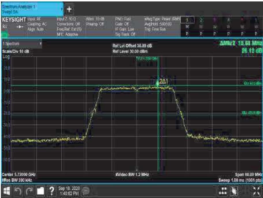
Figure 309 - 5720 MHz - 26 dB Emission Bandwidth
