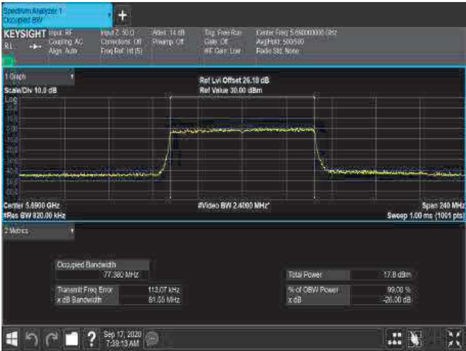
Figure 432 - 5690 MHz - 99% Occupied Bandwidth
