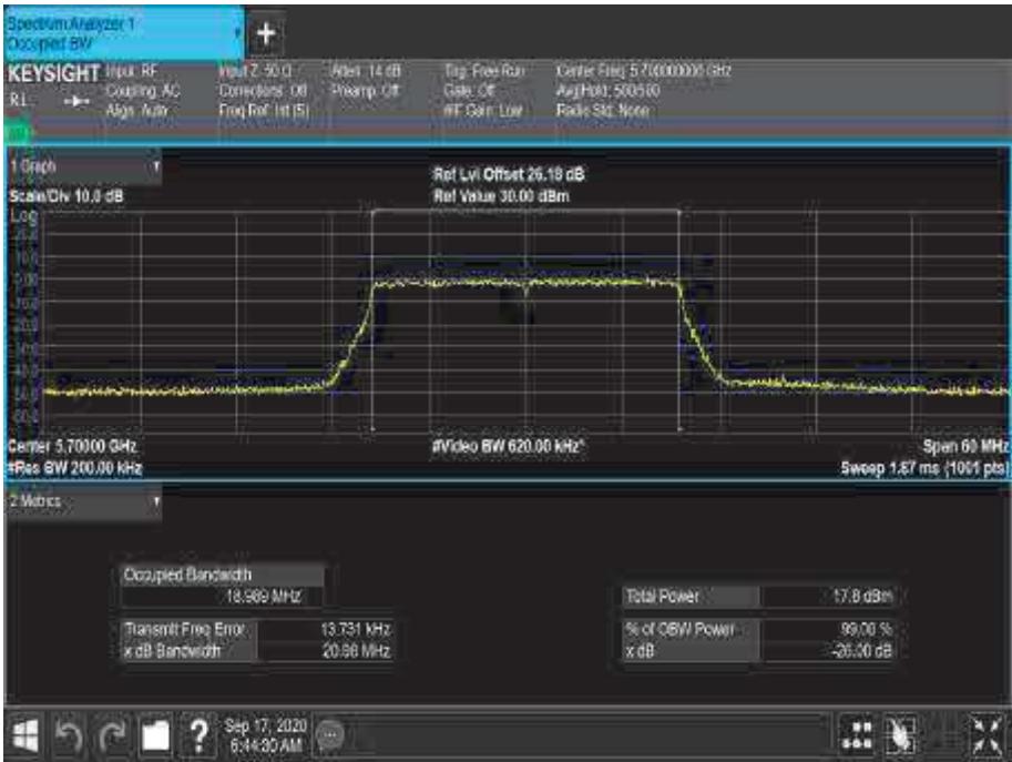
Figure 332 - 5700 MHz - 99% Occupied Bandwidth
