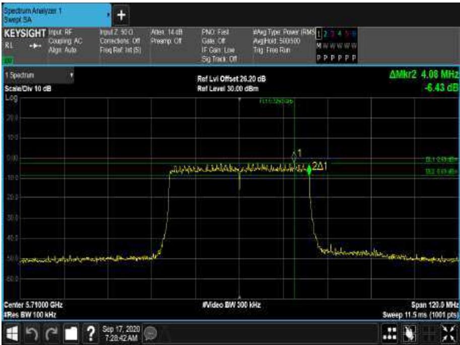
Figure 607 - 5710 MHz - 6 dB DTS Bandwidth
