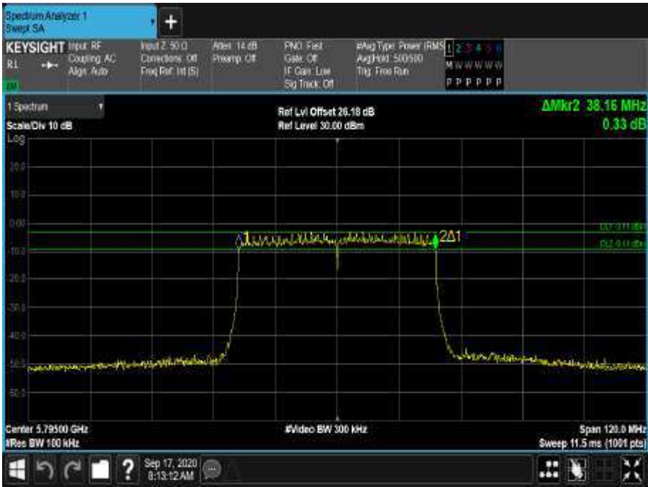
Figure 613 - 5795 MHz - 6 dB DTS Bandwidth
