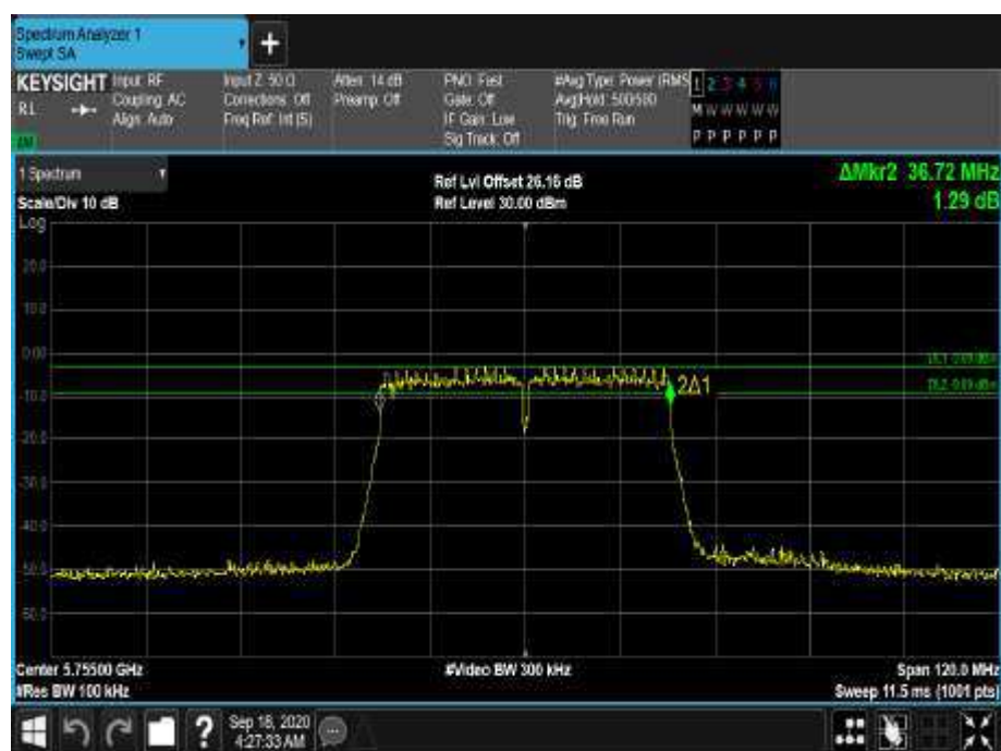
Figure 592 - 5755 MHz - 6 dB DTS Bandwidth
