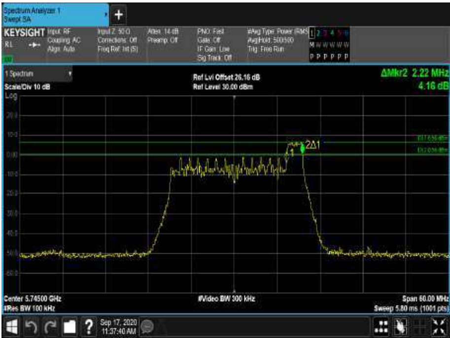
Figure 502 - 5745 MHz - 6 dB DTS Bandwidth
