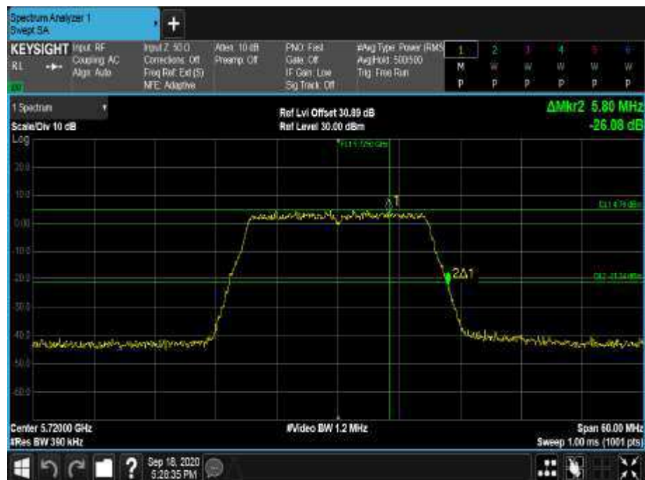
Figure 470 - 5720 MHz - 26 dB Emission Bandwidth
