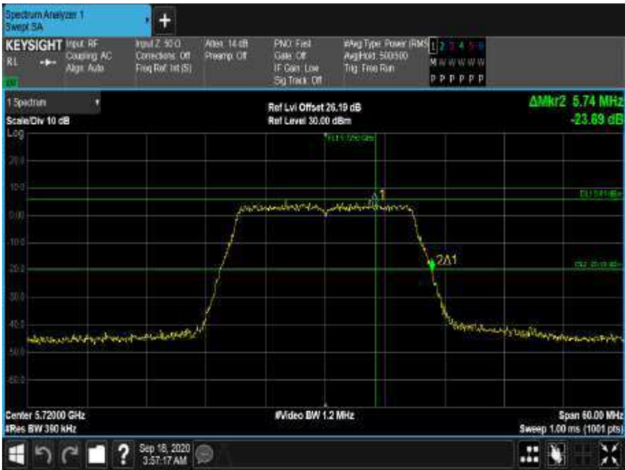
Figure 446 - 5720 MHz - 26 dB Emission Bandwidth
