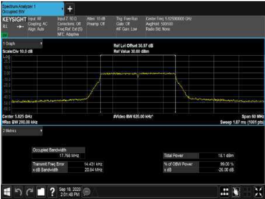
Figure 480 - 5825 MHz - 99% Occupied Bandwidth
