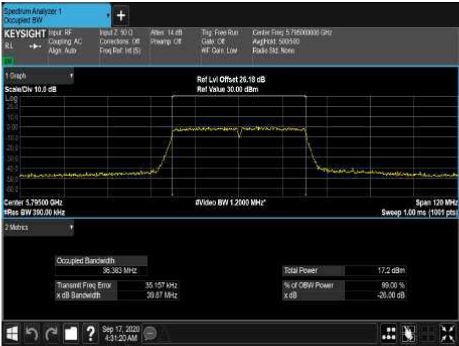
Figure 579 - 5795 MHz - 99% Occupied Bandwidth
