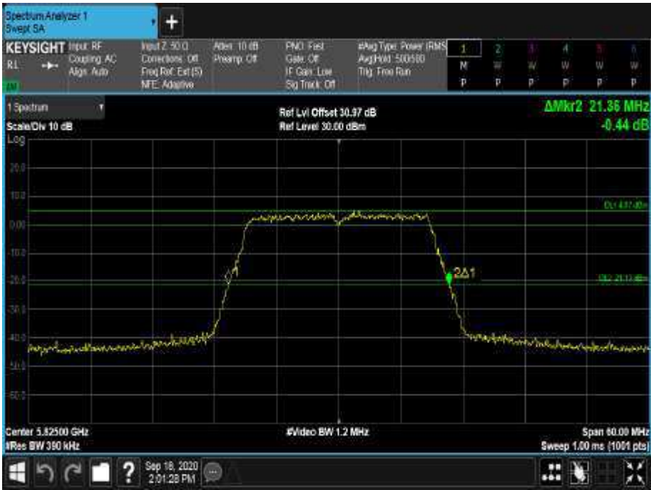
Figure 479 - 5825 MHz - 26 dB Emission Bandwidth
