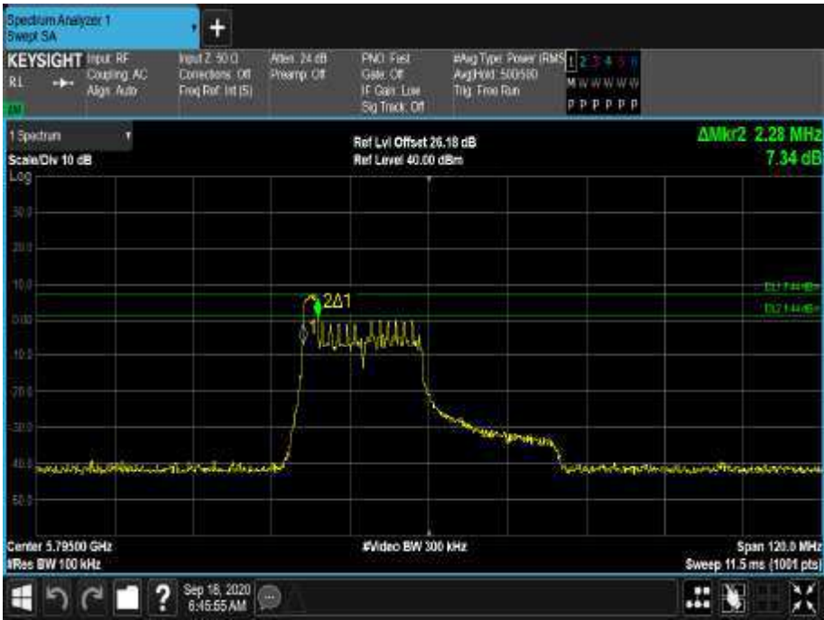
Figure 640 - 5795 MHz - 6 dB DTS Bandwidth
