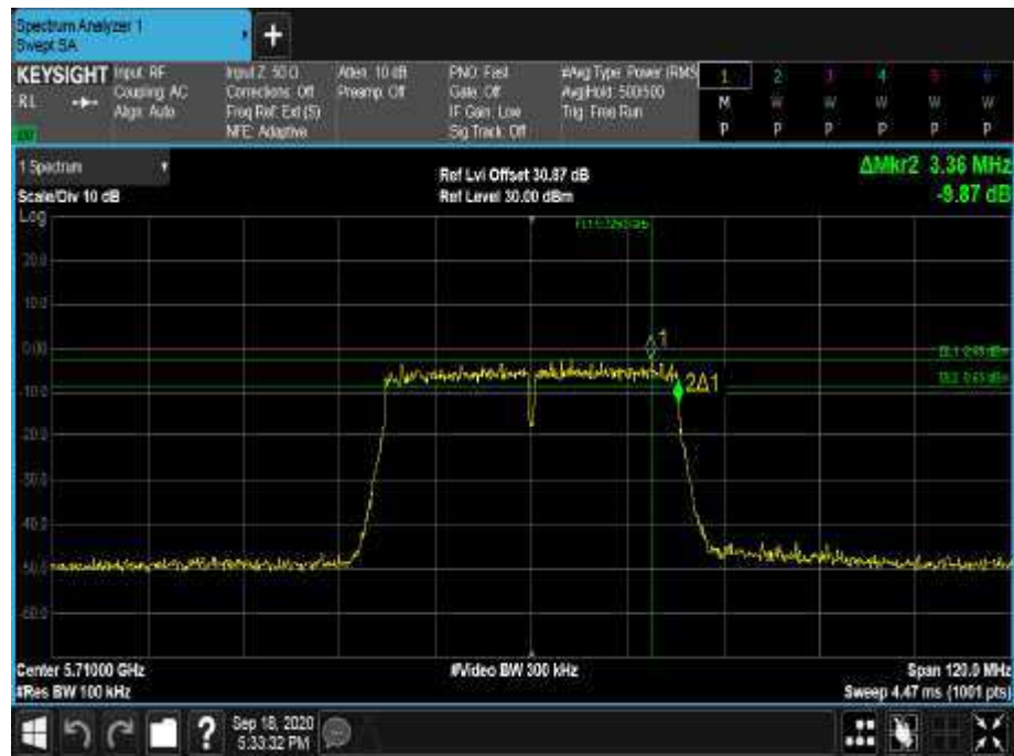
Figure 598 - 5710 MHz - 6 dB DTS Bandwidth
