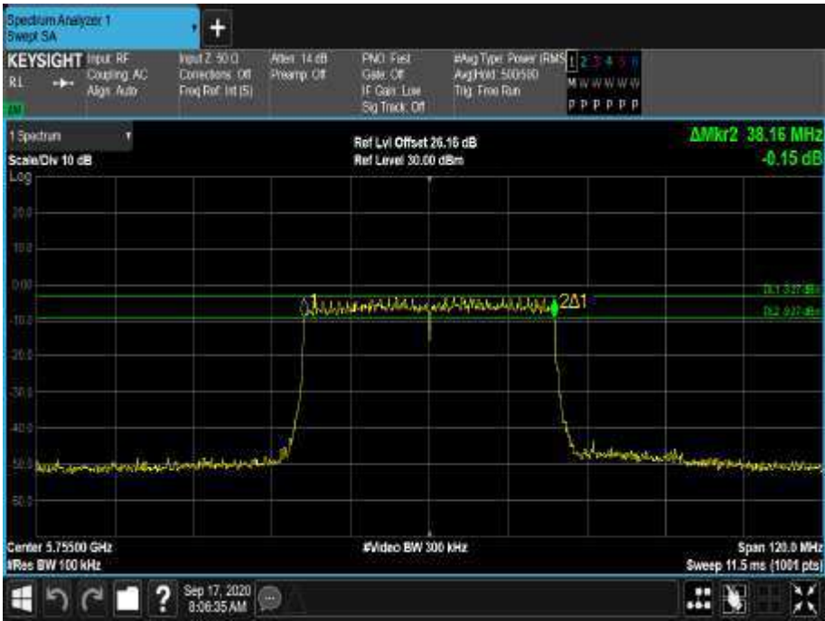
Figure 610 - 5755 MHz - 6 dB DTS Bandwidth
