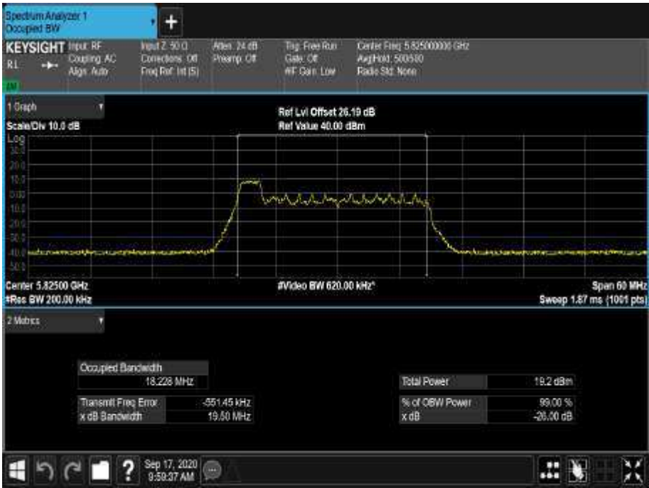
Figure 501 - 5825 MHz - 99% Occupied Bandwidth
