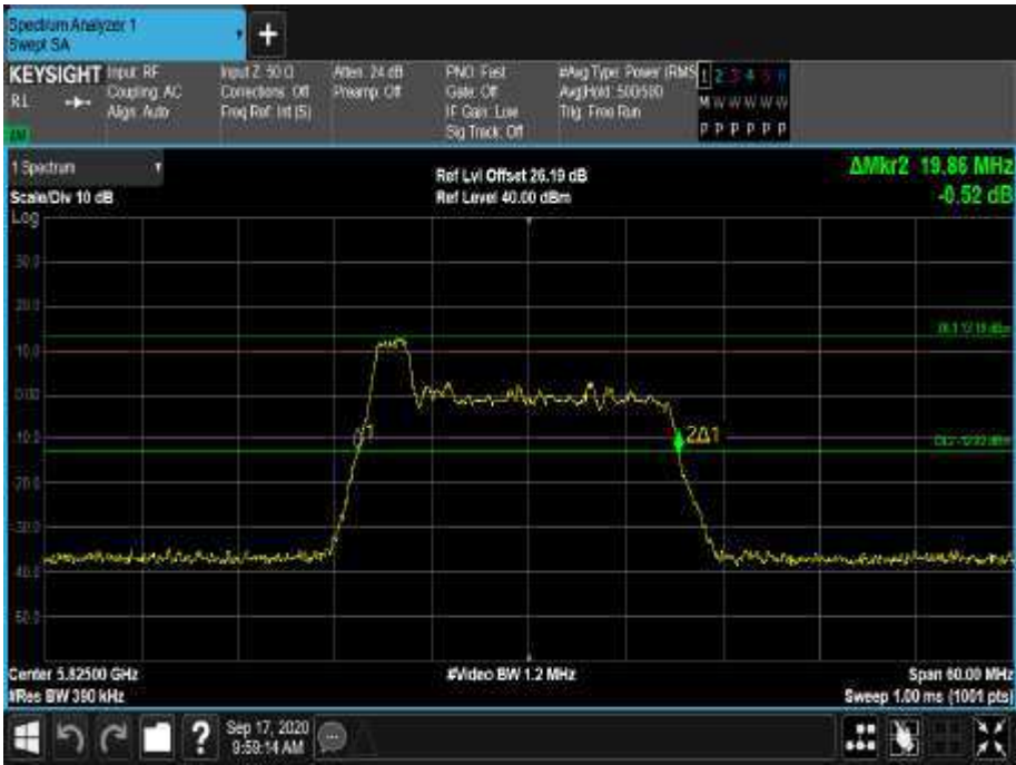
Figure 500 - 5825 MHz - 26 dB Emission Bandwidth
