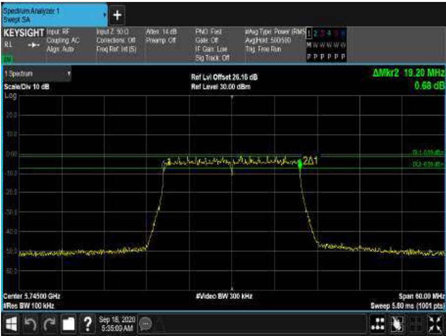
Figure 514 - 5745 MHz - 6 dB DTS Bandwidth
