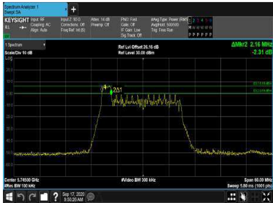
Figure 553 - 5745 MHz - 6 dB DTS Bandwidth
