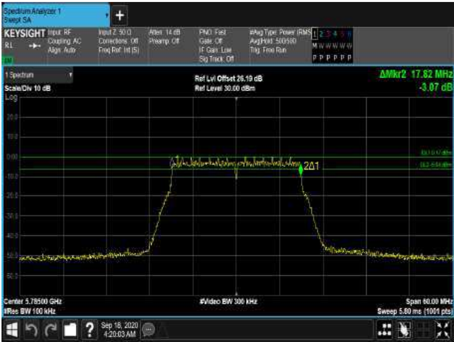
Figure 463 - 5785 MHz - 6 dB DTS Bandwidth
