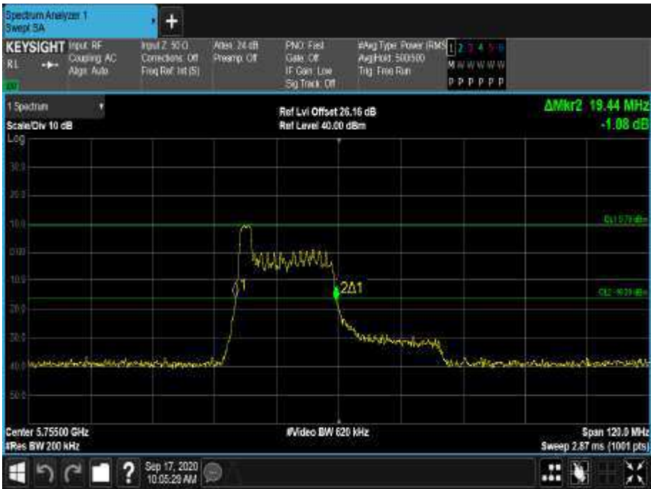
Figure 617 - 5755 MHz - 26 dB Emission Bandwidth
