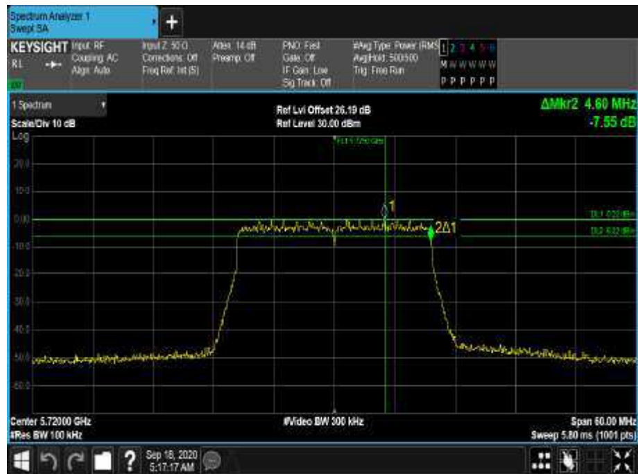
Figure 511 - 5720 MHz - 6 dB DTS Bandwidth
