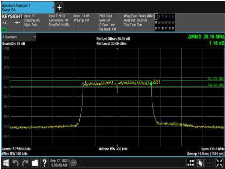
Figure 631 - 5755 MHz - 6 dB DTS Bandwidth
