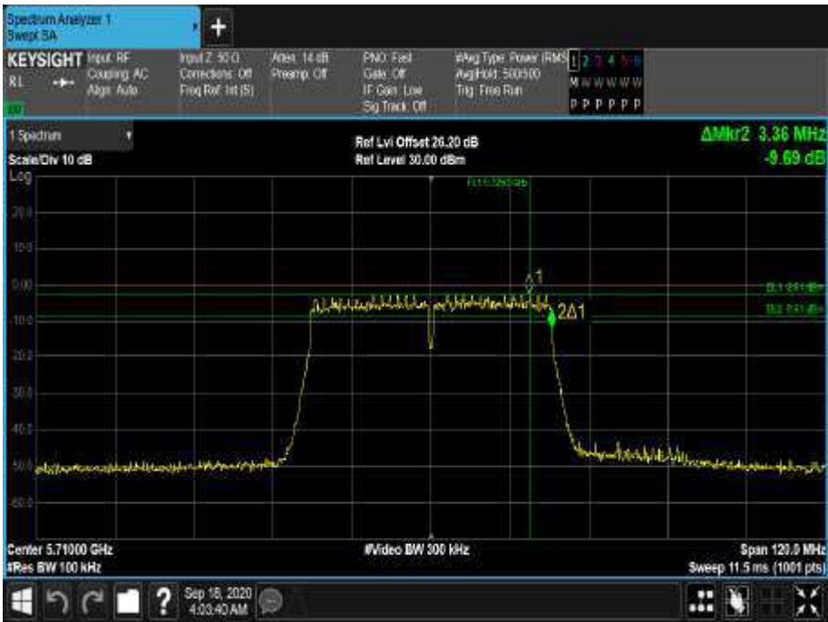
Figure 580 - 5710 MHz - 6 dB DTS Bandwidth
