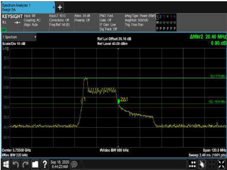
Figure 659 - 5755 MHz - 26 dB Emission Bandwidth
