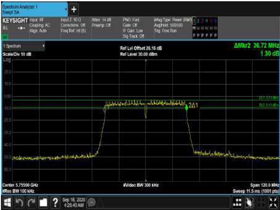
Figure 583 - 5755 MHz - 6 dB DTS Bandwidth
