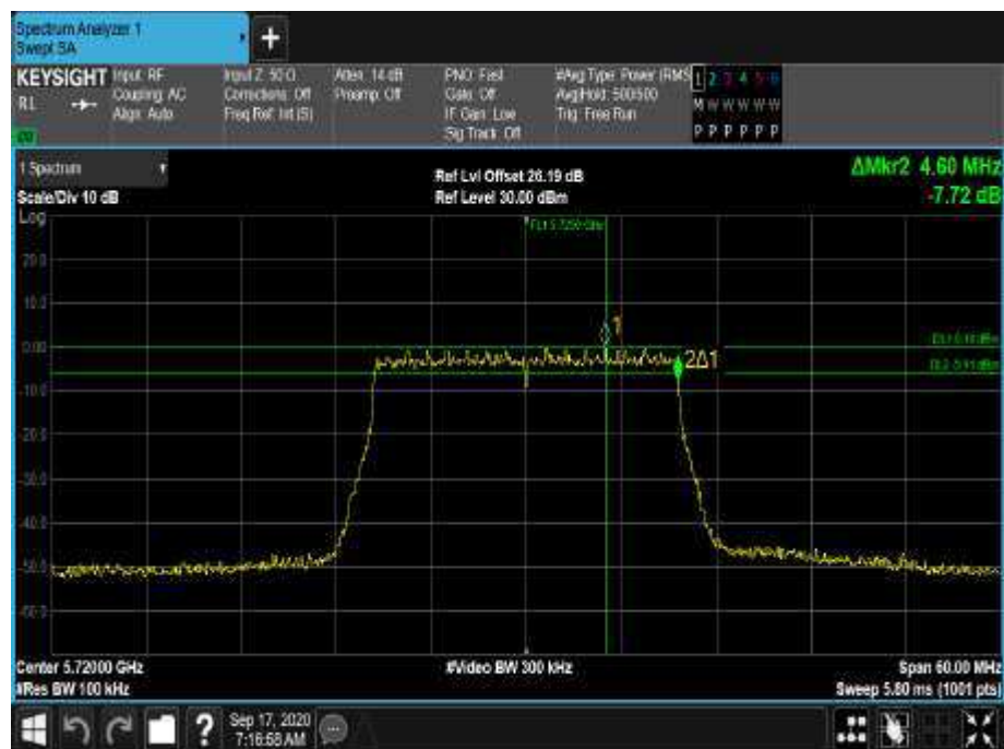
Figure 481 - 5720 MHz - 6 dB DTS Bandwidth
