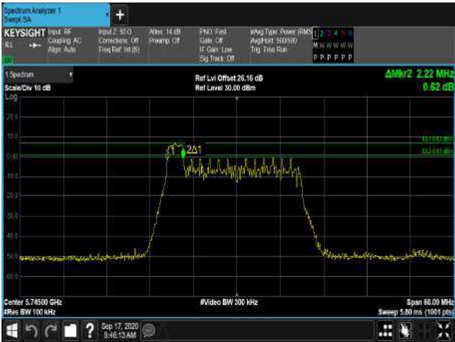
Figure 493 - 5745 MHz - 6 dB DTS Bandwidth
