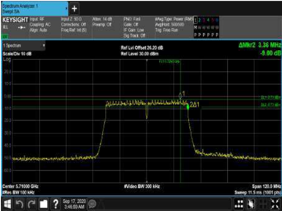
Figure 571 - 5710 MHz - 6 dB DTS Bandwidth
