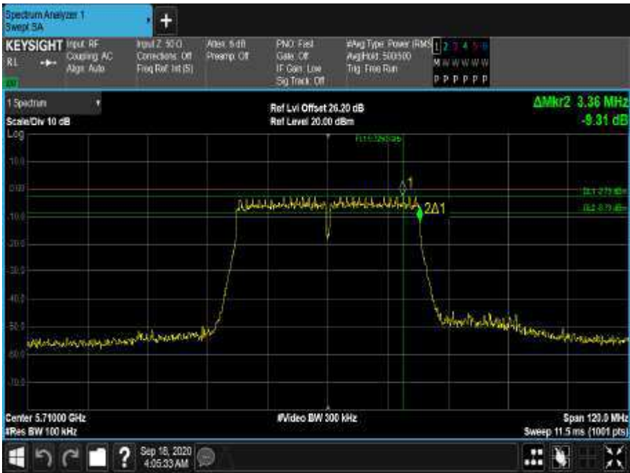
Figure 589 - 5710 MHz - 6 dB DTS Bandwidth
