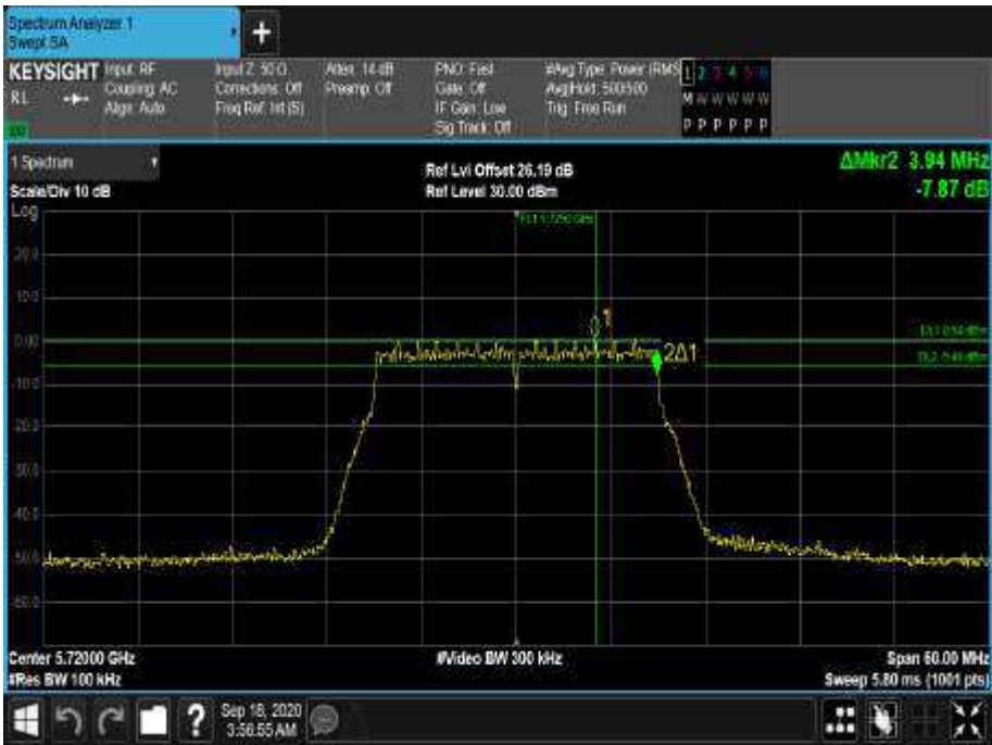
Figure 445 - 5720 MHz - 6 dB DTS Bandwidth
