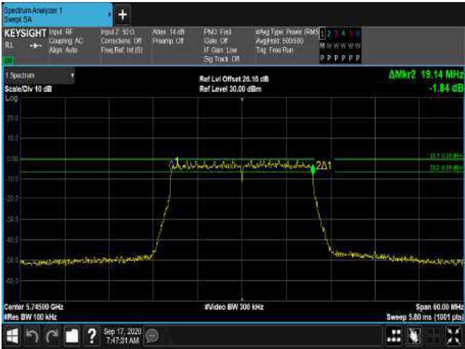
Figure 484 - 5745 MHz - 6 dB DTS Bandwidth
