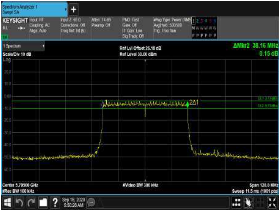
Figure 634 - 5795 MHz - 6 dB DTS Bandwidth
