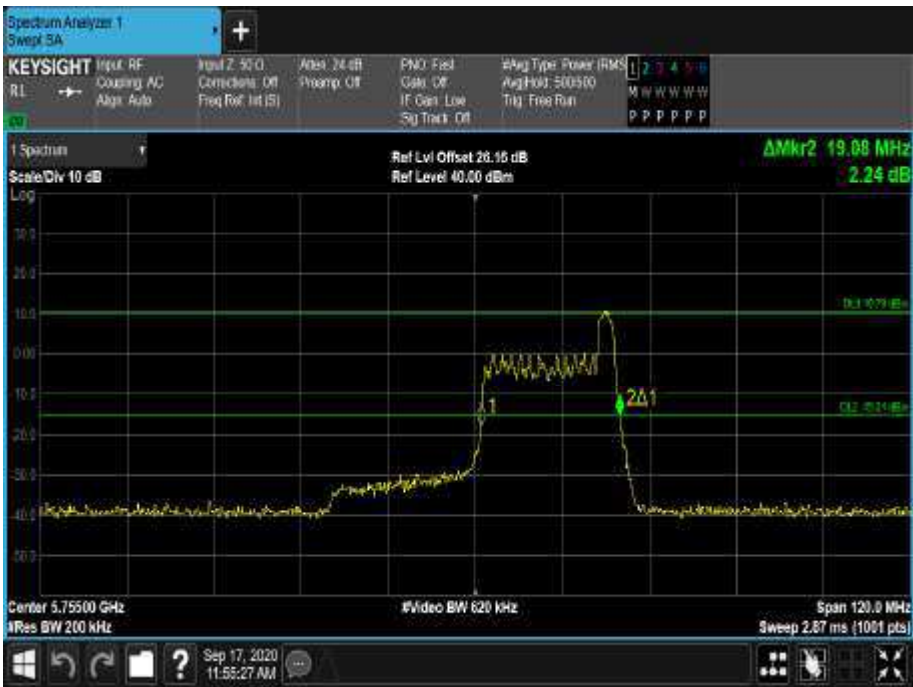
Figure 623 - 5755 MHz - 26 dB Emission Bandwidth
