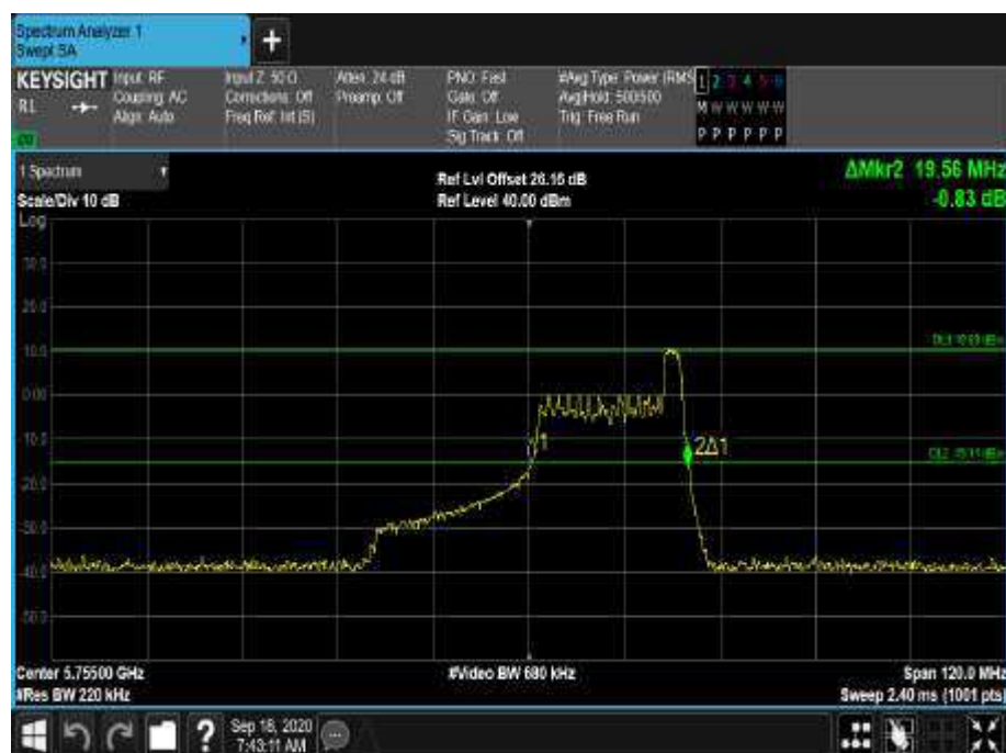
Figure 665 - 5755 MHz - 26 dB Emission Bandwidth
