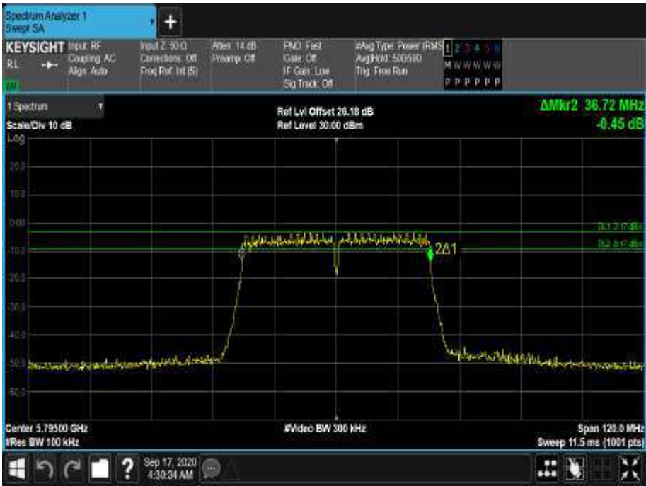
Figure 577 - 5795 MHz - 6 dB DTS Bandwidth
