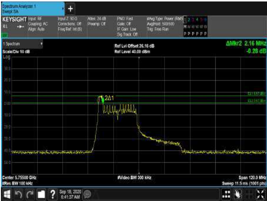
Figure 637 - 5755 MHz - 6 dB DTS Bandwidth
