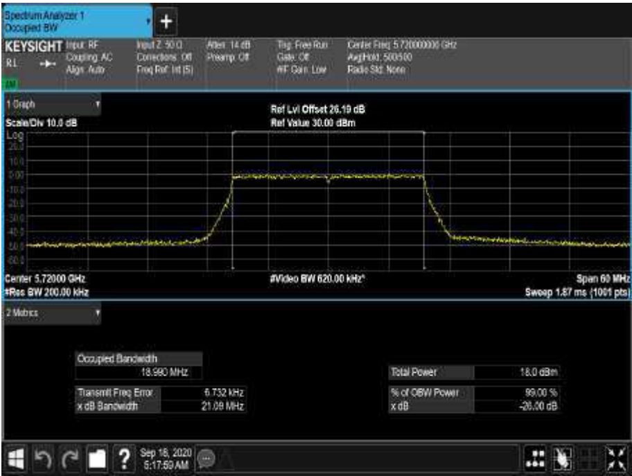
Figure 513 - 5720 MHz - 99% Occupied Bandwidth
