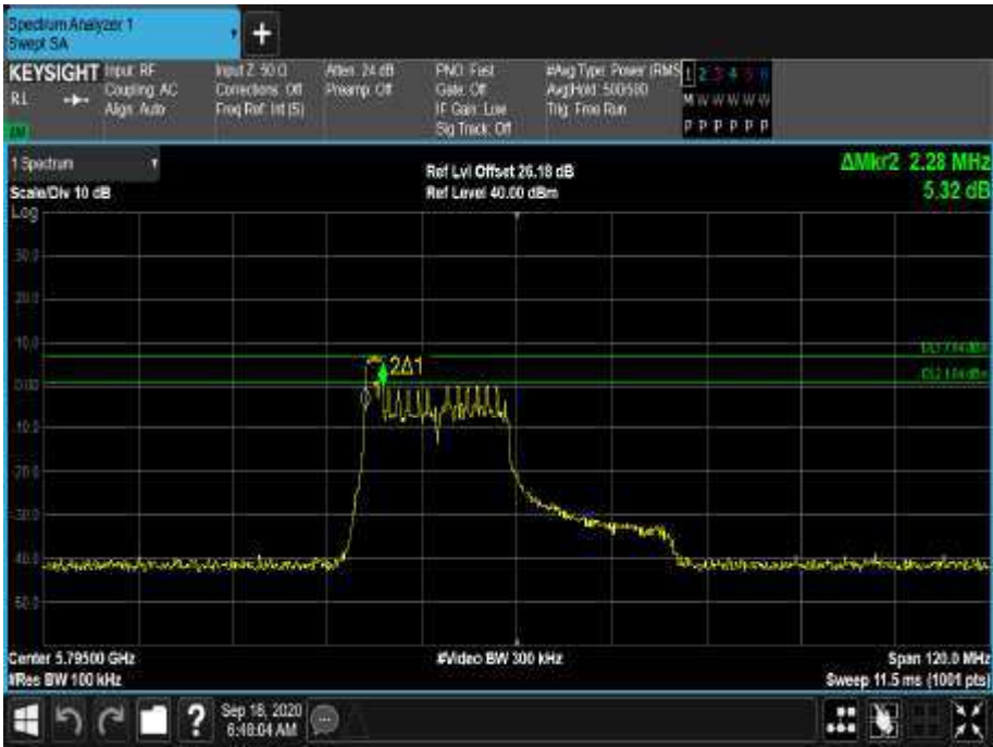
Figure 661 - 5795 MHz - 6 dB DTS Bandwidth
