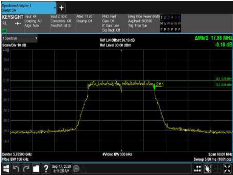
Figure 439 - 5785 MHz - 6 dB DTS Bandwidth
