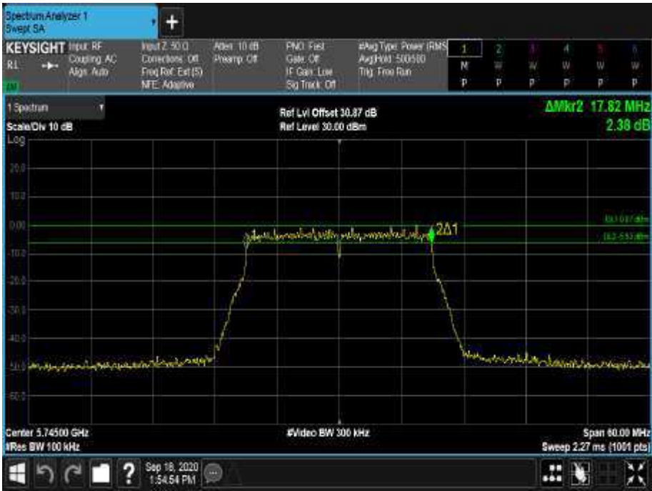
Figure 472 - 5745 MHz - 6 dB DTS Bandwidth
