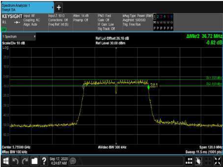
Figure 574 - 5755 MHz - 6 dB DTS Bandwidth
