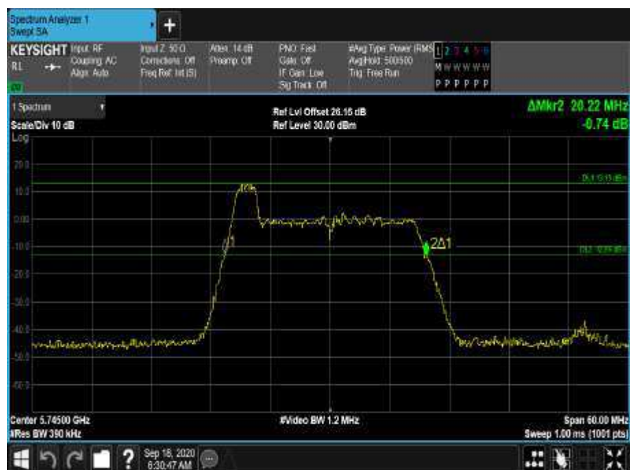
Figure 524 - 5745 MHz - 26 dB Emission Bandwidth
