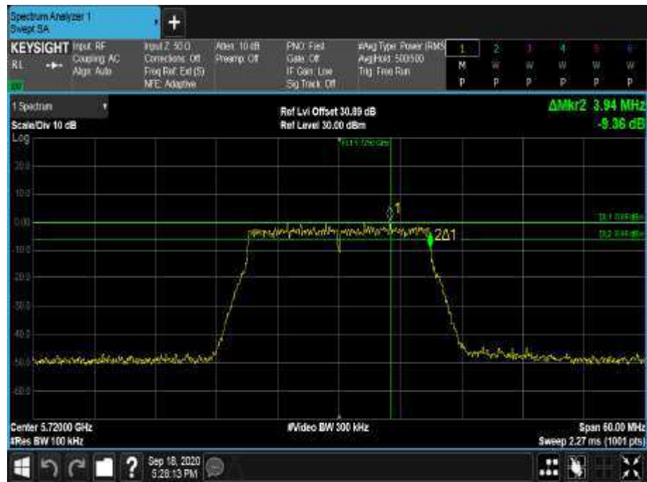
Figure 469 - 5720 MHz - 6 dB DTS Bandwidth
