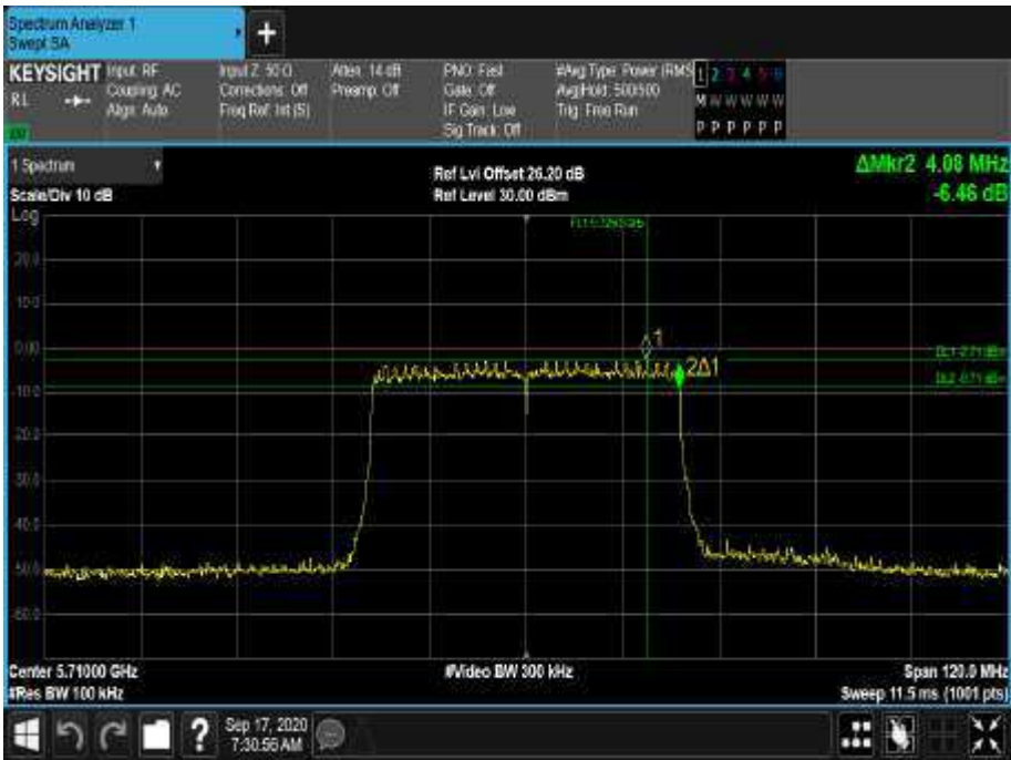
Figure 628 - 5710 MHz - 6 dB DTS Bandwidth
