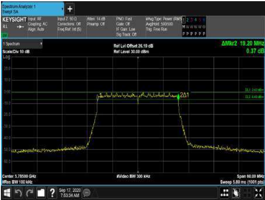
Figure 487 - 5785 MHz - 6 dB DTS Bandwidth
