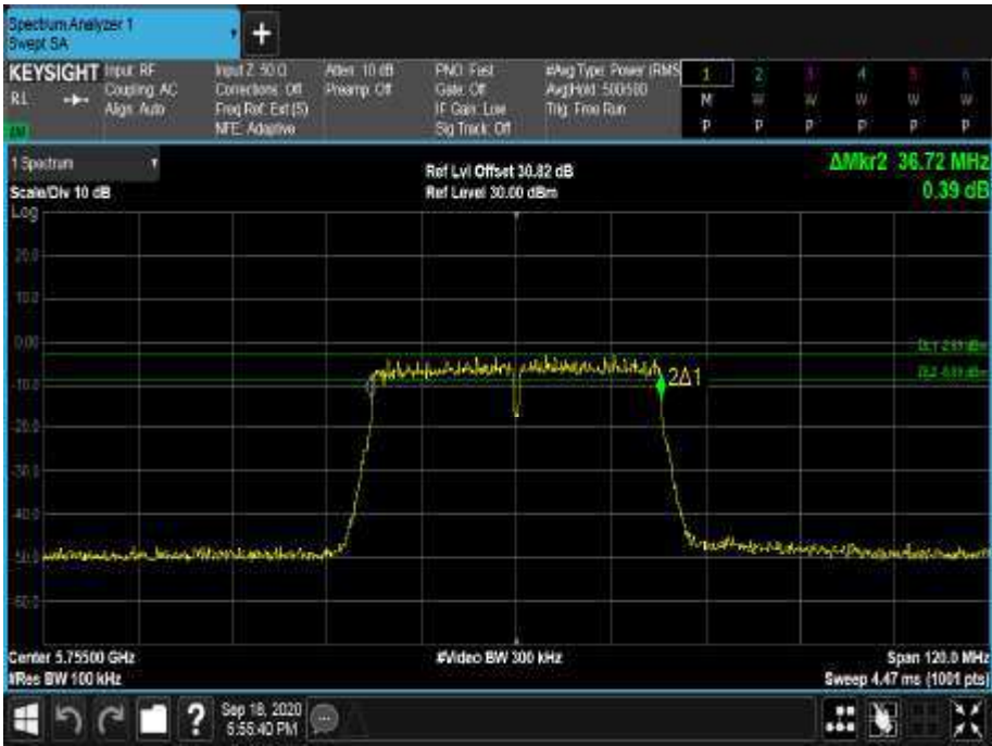
Figure 601 - 5755 MHz - 6 dB DTS Bandwidth
