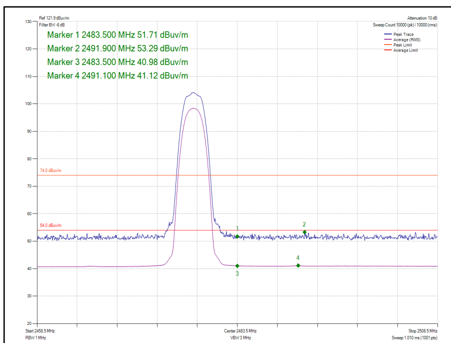
Figure 124 - Core 1 - Static - \pi/4 DQPSK /HDR4 - 2478 MHz - Band Edge Frequency 2483.5 MHz
