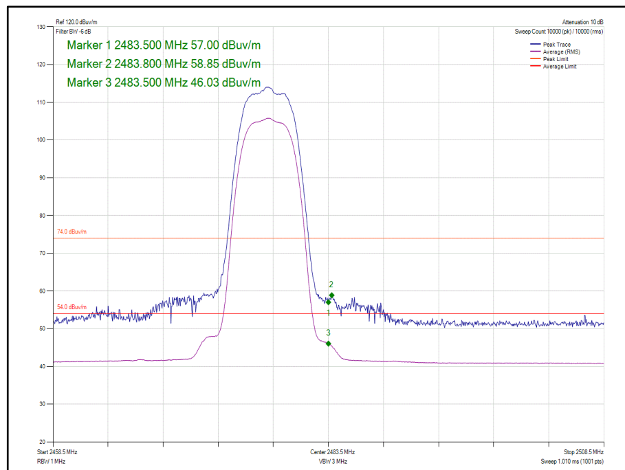
Figure 144 - Core 0-1 - Static - \pi/4 DQPSK /HDR8 - 2478 MHz - Band Edge Frequency 2483.5 MHz
