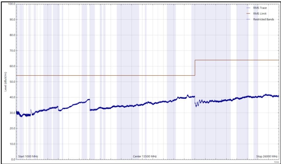
Figure 161 - 2402 MHz (CH0), LE1M, iPA, Core 1, 1 GHz to 26 GHz, Horizontal (rms)
