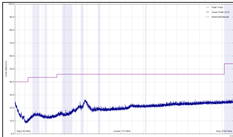
Figure 164 - 2440 MHz (CH17), LE1M, iPA, Core 1, 30 MHz to 1 GHz, Horizontal (Peak)
