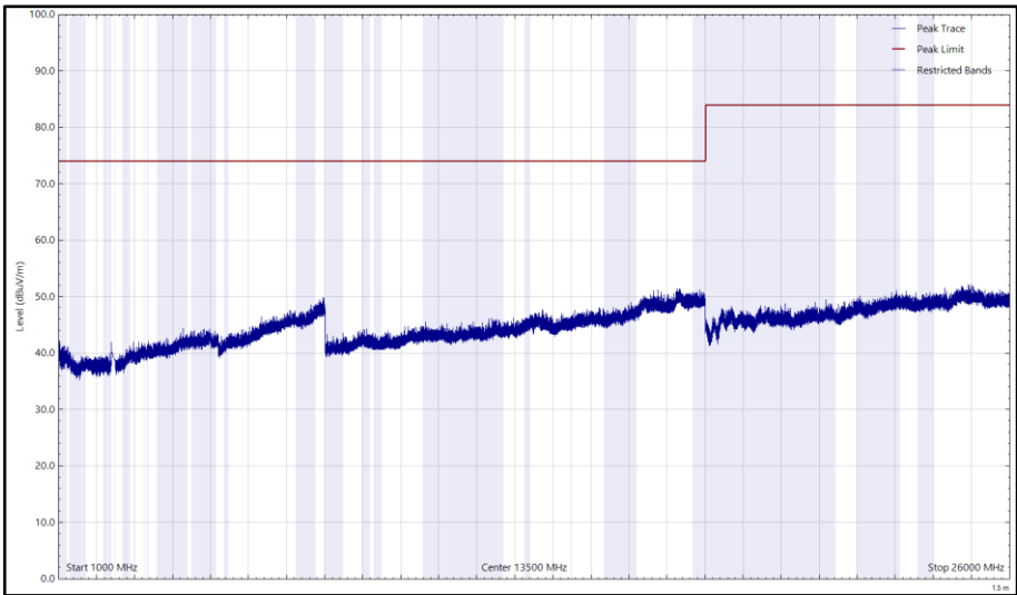
Figure 160 - 2402 MHz (CH0), LE1M, iPA, Core 1, 1 GHz to 26 GHz, Horizontal (Peak)
