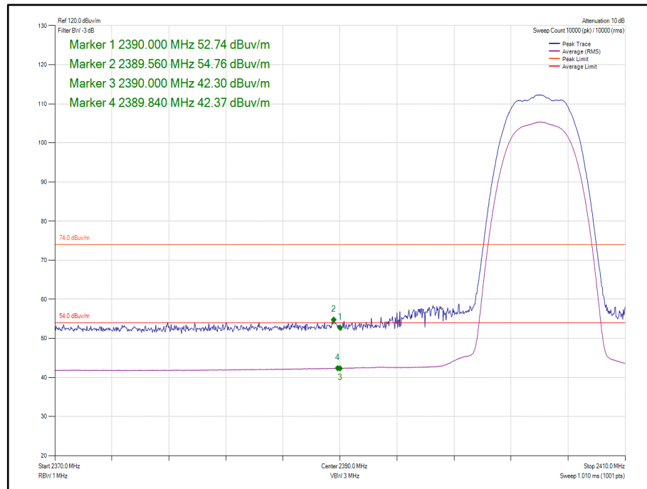
Figure 143- Core 0-1 - Static - \pi/4 DQPSK /HDR8 - 2404 MHz - Band Edge Frequency 2390.0 MHz
