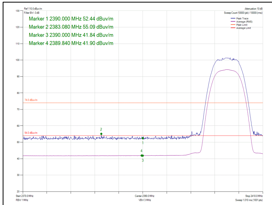
Figure 139- Core 0 - Static - \pi/4 DQPSK /HDR8 - 2404 MHz - Band Edge Frequency 2390.0 MHz
