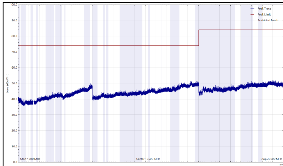
Figure 156 - 2480 MHz (CH39), LE1M, iPA, Core 0, 1 GHz to 26 GHz, Horizontal (Peak)
