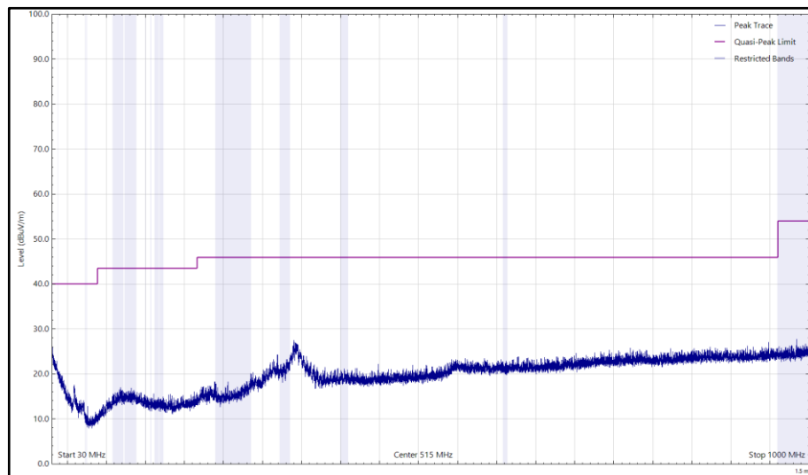
Figure 150 - 2440 MHz (CH17), LE1M, iPA, Core 0, 30 MHz to 1 GHz, Horizontal (Peak)
