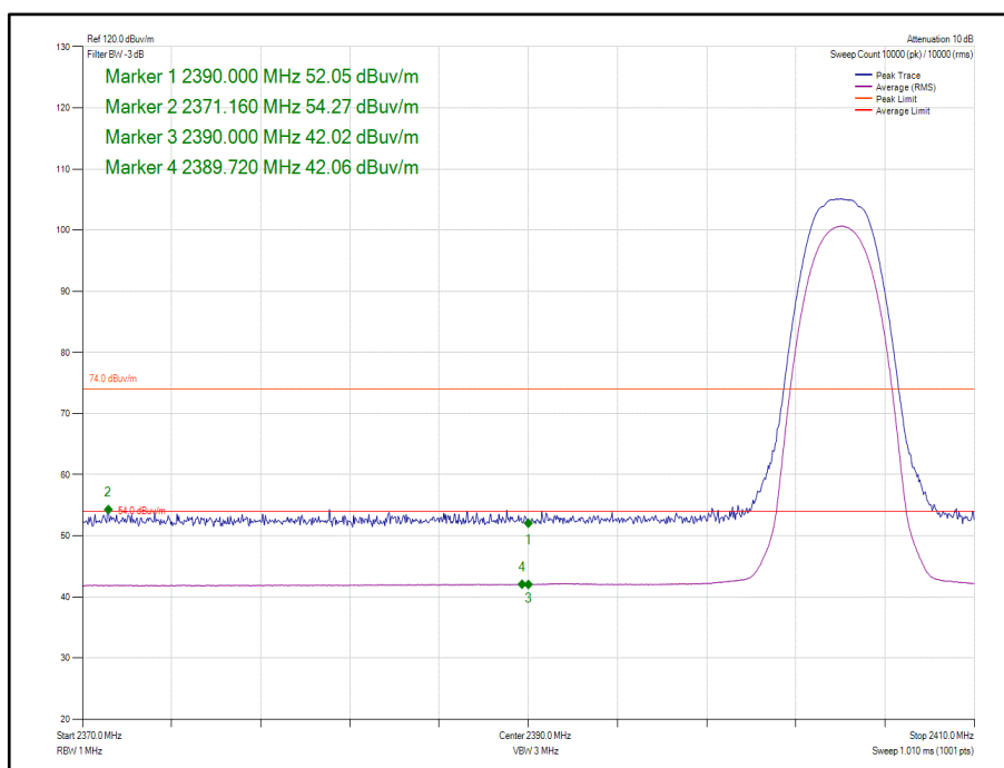
Figure 123 - Core 1 - Static - \pi/4 DQPSK /HDR4 - 2404 MHz - Band Edge Frequency 2390.0 MHz
