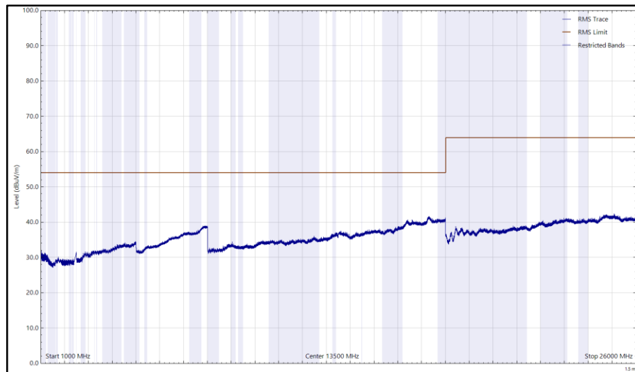
Figure 157 - 2480 MHz (CH39), LE1M, iPA, Core 0, 1 GHz to 26 GHz, Horizontal (rms)
