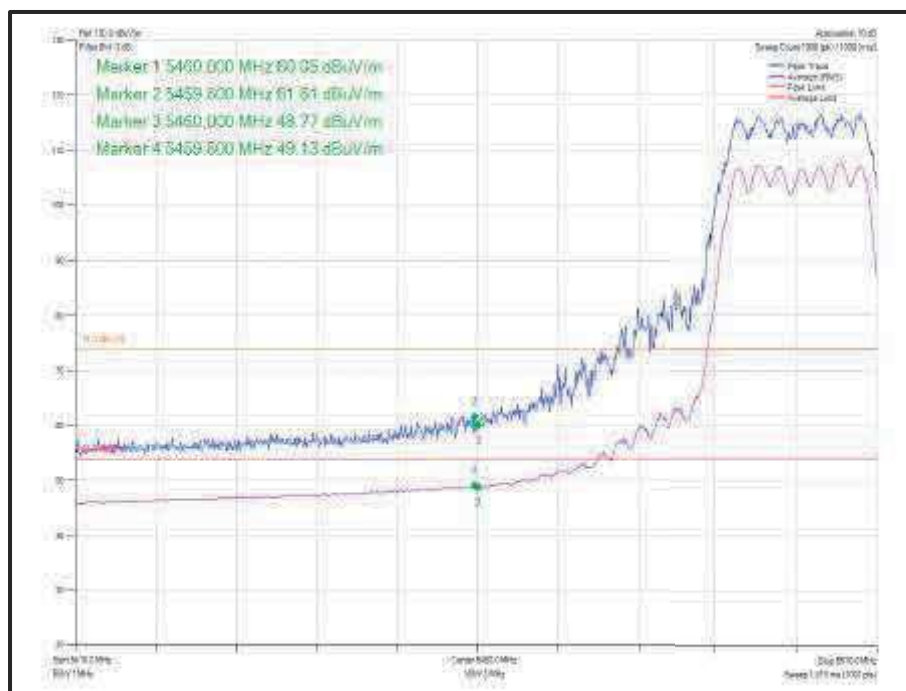
Figure 866 - 802.11n HT20 CDD, Cores 0-1 - 5500 MHz Band Edge Frequency 5460 MHz
