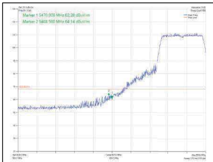
Figure 731 - 802.11n HT20, Core 1 - 5 500 MHz Band Edge Frequency 5470 MHz
