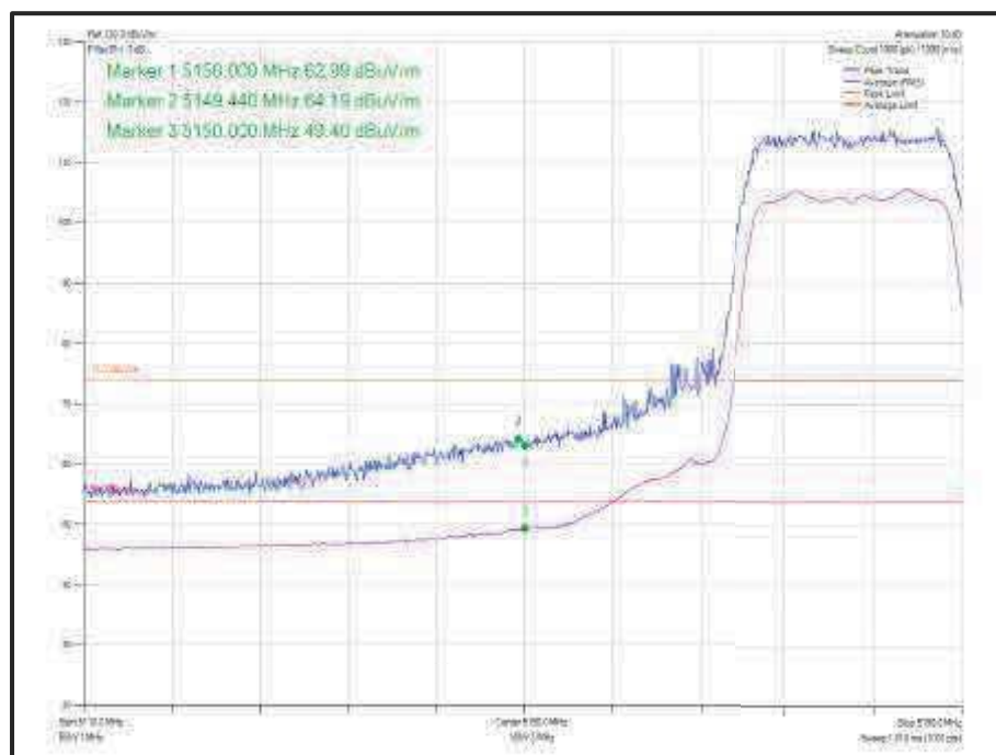
Figure 855 - 802.11n HT20 SDM, Cores 0-1 - 5180 MHz Band Edge Frequency 5150 MHz
