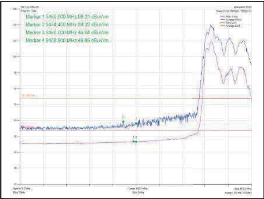
Figure 871 - 802.11ax HE20 SDM, Cores 0-1, 26-0 - 5500 MHz Band Edge Frequency 5460 MHz
