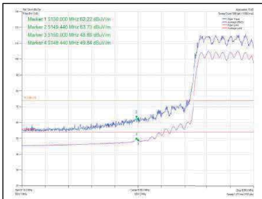
Figure 856 - 802.11ax HE20 CDD, Cores 0-1 SU - 5180 MHz Band Edge Frequency 5150 MHz
