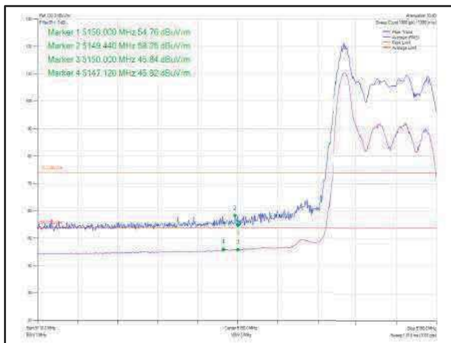
Figure 857 - 802.11ax HE20 CDD, Cores 0-1, 26-0 - 5180 MHz Band Edge Frequency 5150 MHz
