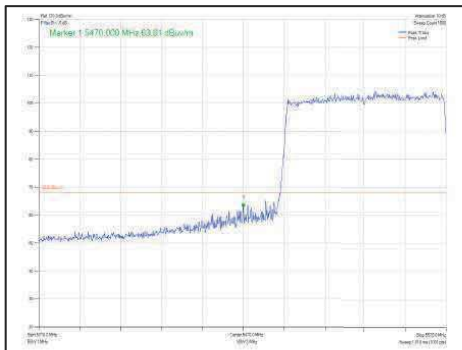
Figure 810 - 802.11ax HE80 Core 1 SU - 5530 MHz Band Edge Frequency 5470 MHz
