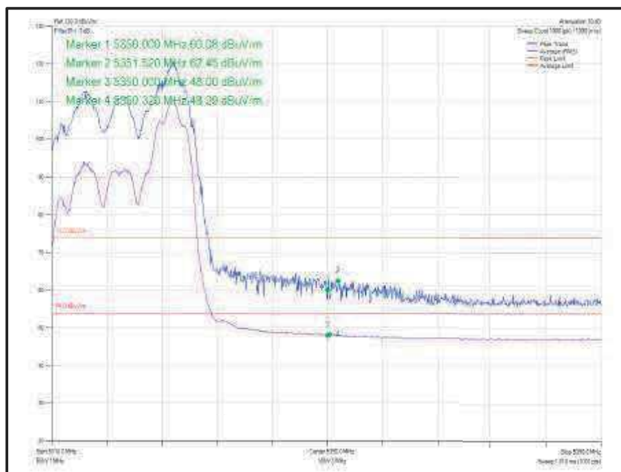
Figure 863 - 802.11ax HE20 CDD, Cores 0-1, 52-40 - 5320 MHz Band Edge Frequency 5350 MHz
