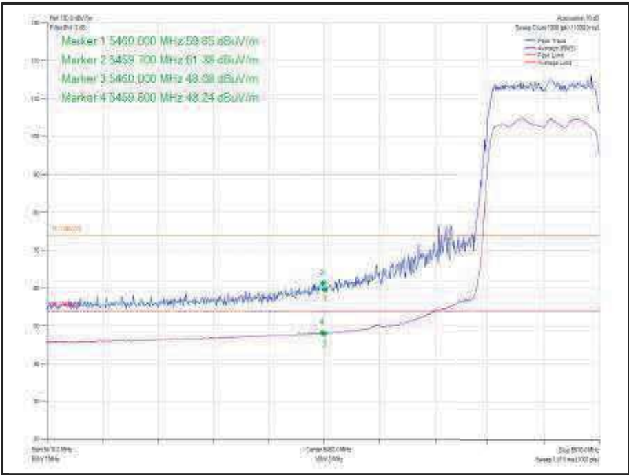
Figure 870 - 802.11ax HE20 SDM, Cores 0-1, SU- 5500 MHz Band Edge Frequency 5460 MHz
