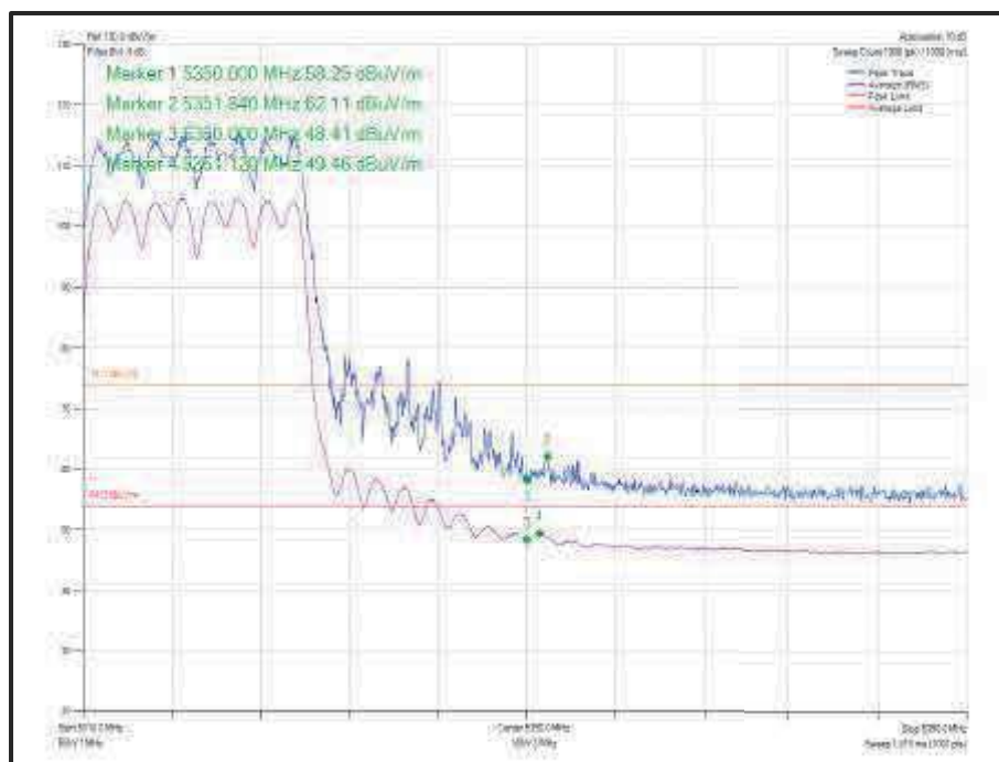
Figure 862 - 802.11ax HE20 CDD, Cores 0-1, SU - 5320 MHz Band Edge Frequency 5350 MHz
