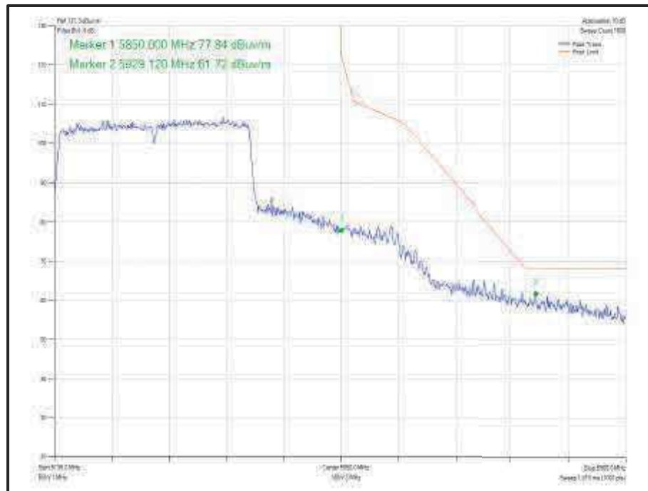
Figure 809 - 802.11ac VHT80 Core 1 - 5775 MHz Band Edge Frequency 5850 MHz
