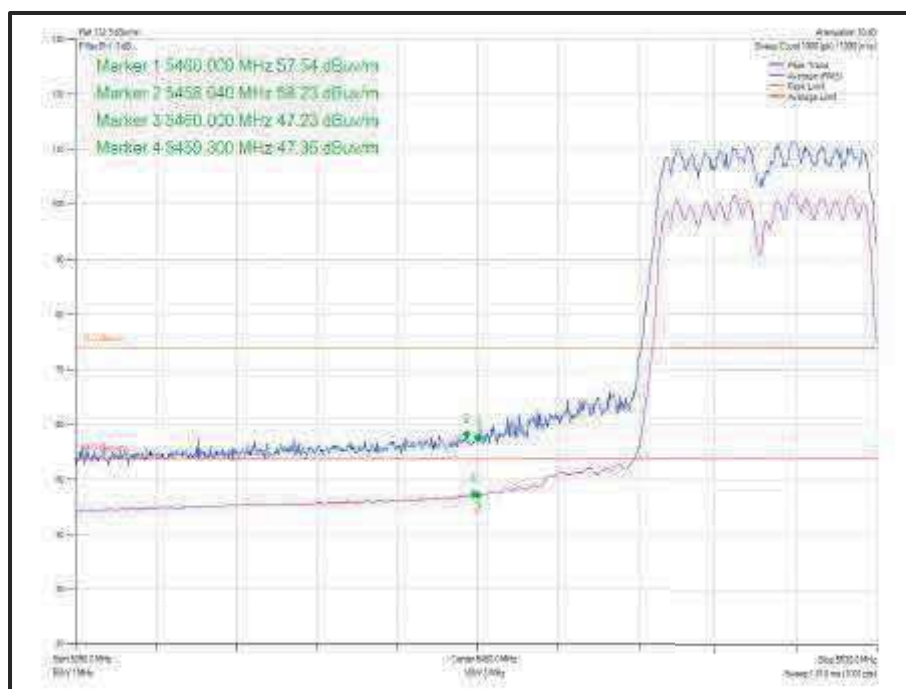
Figure 893 - 802.11n HT40 CDD, Cores 0-1 - 5510 MHz Band Edge Frequency 5460 MHz
