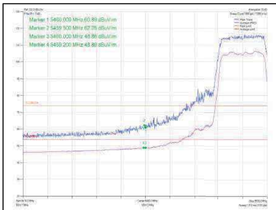
Figure 867 - 802.11n HT20 SDM, Cores 0-1 - 5500 MHz Band Edge Frequency 5460 MHz
