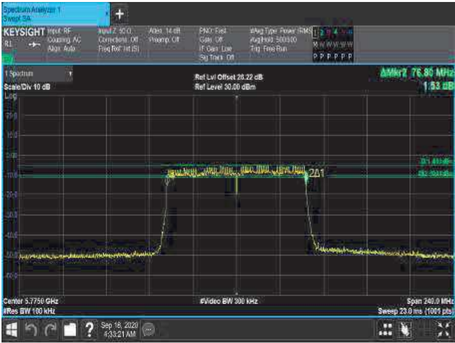
Figure 679 - 5775 MHz - 6 dB DTS Bandwidth
