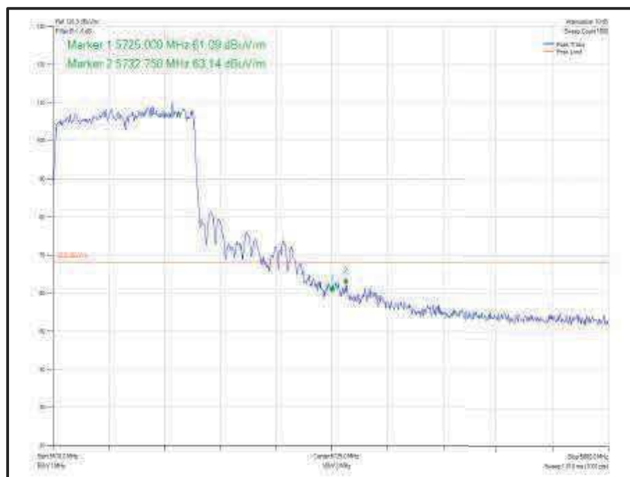
Figure 825 - 802.11ac VHT80 SDM, Cores 0-1 - 5610 MHz Band Edge Frequency 5725 MHz
