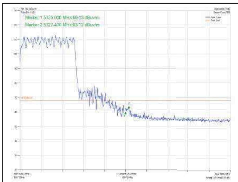
Figure 790 - 802.11ax HE40 CDD, Cores 0-1, SU - 5670 MHz Band Edge Frequency 5725 MHz
