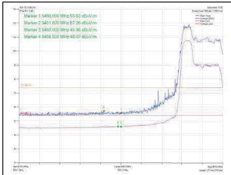
Figure 853 - 802.11ax HE20, Core 1, 52-37 - 5500 MHz, Band Edge Frequency 5460 MHz
