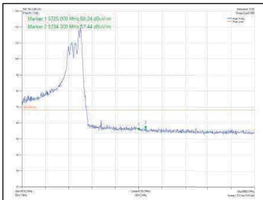
Figure 827 - 802.11ax HE80 CDD, Cores 0-1, 52-52 - 5610 MHz Band Edge Frequency 5725 MHz
