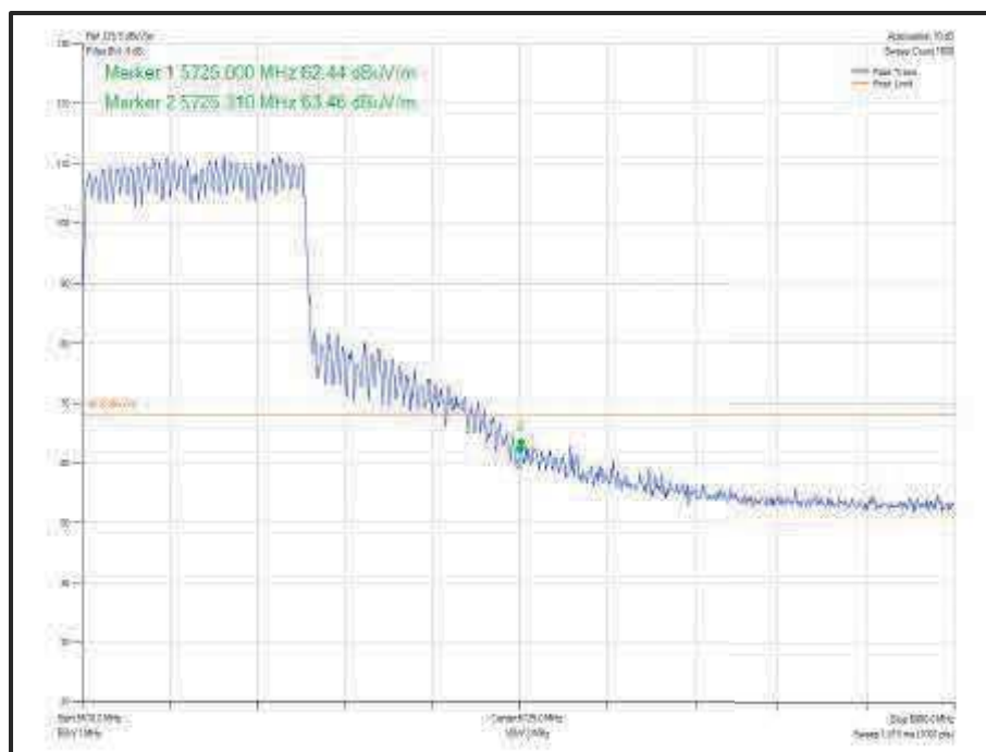
Figure 826 - 802.11ax HE80 CDD, Cores 0-1, SU - 5610 MHz Band Edge Frequency 5725 MHz
