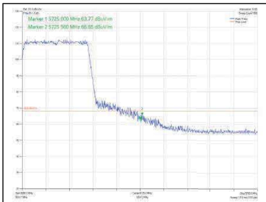
Figure 753 - 802.11n HT20 SDM, Cores 0-1 - 5700 MHz Band Edge Frequency 5725 MHz
