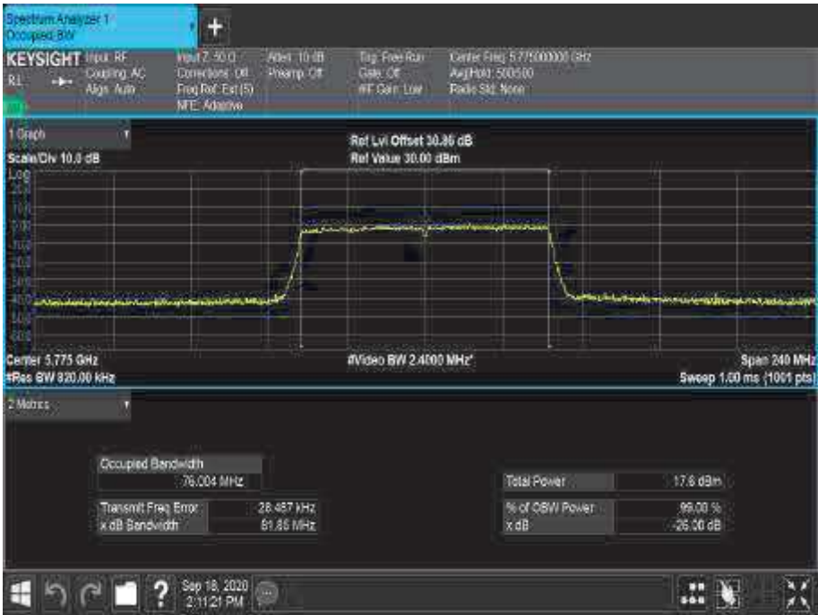
Figure 693 - 5775 MHz - 99% Occupied Bandwidth
