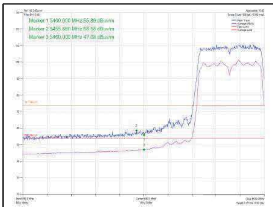
Figure 894 - 802.11n HT40 SDM, Cores 0-1 - 5510 MHz Band Edge Frequency 5460 MHz
