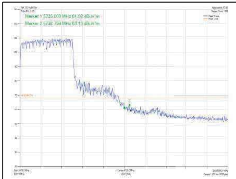
Figure 824 - 802.11ac VHT80 CDD, Cores 0-1 - 5610 MHz Band Edge Frequency 5725 MHz
