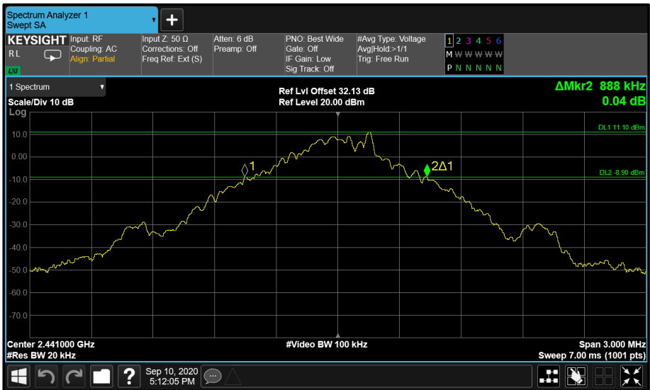
Figure 12 - Core 1 GFSK 2441 MHz (CH39)
