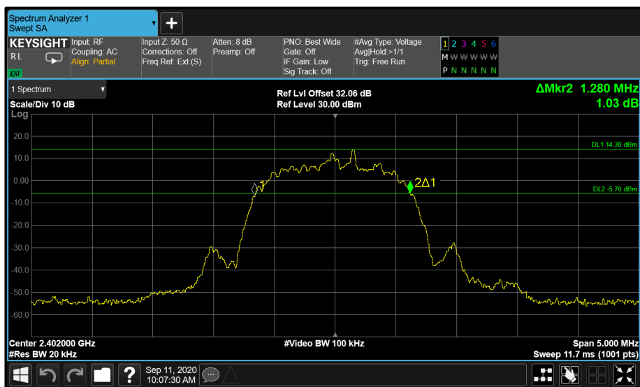
Figure 44 - Core 1 8-DPSK 2402 MHz (CH0)
