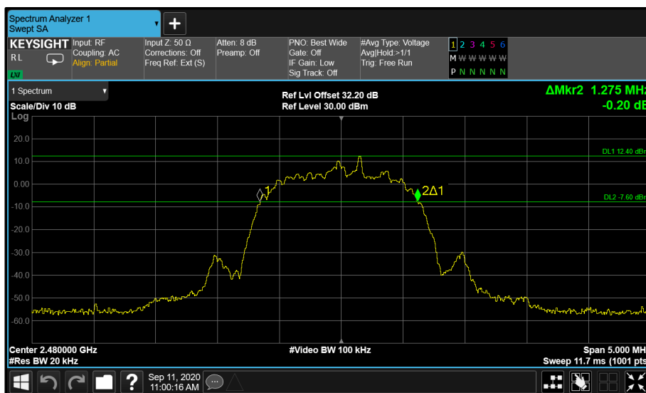
Figure 63 - Core 1 8-DPSK 2480 MHz (CH78)
