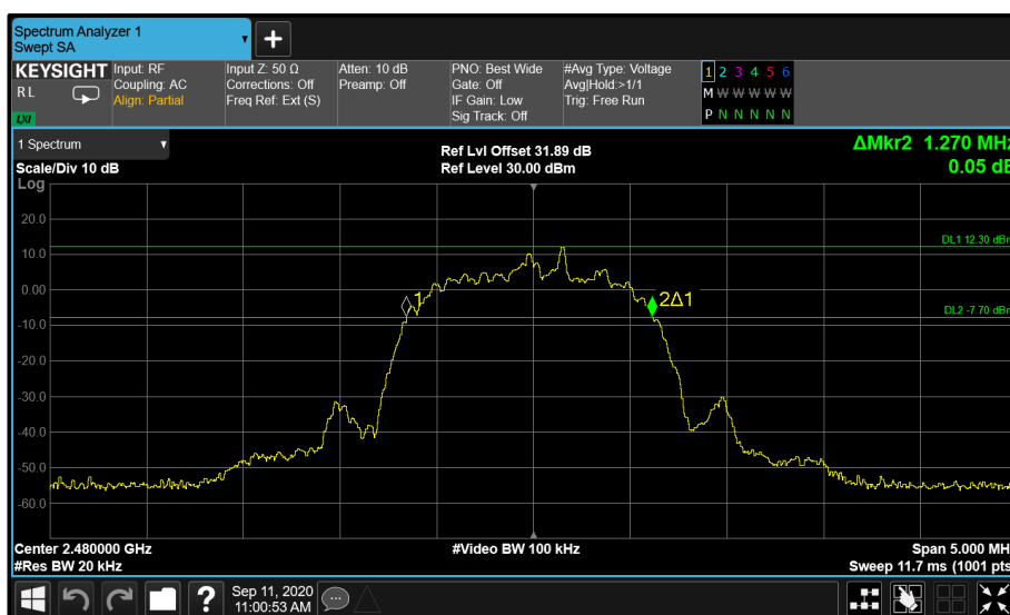
Figure 64 - Core 0 8-DPSK 2480 MHz (CH78)
