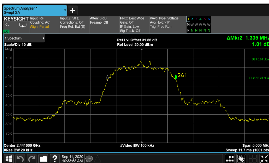
Figure 29 - Core 0 \pi/4 DQPSK 2441 MHz (CH39)
