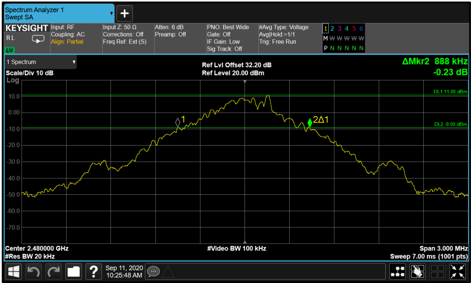
Figure 24 - Core 1 GFSK 2480 MHz (CH78)
