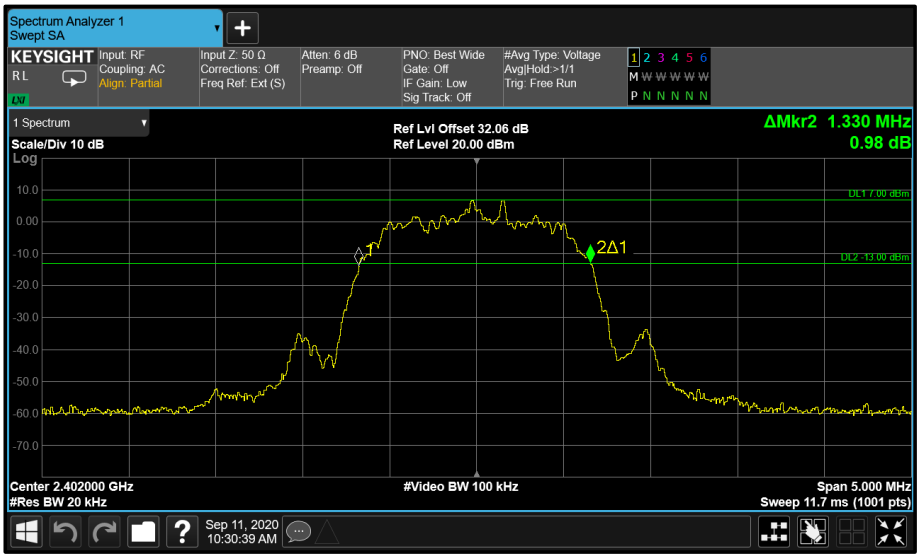
Figure 26 - Core 1 \pi/4 DQPSK 2402 MHz (CH0)
