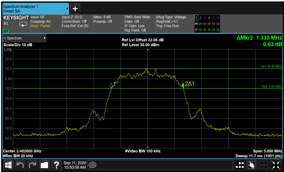
Figure 53 - Core 1 \pi/4 DQPSK 2402 MHz (CH0)
