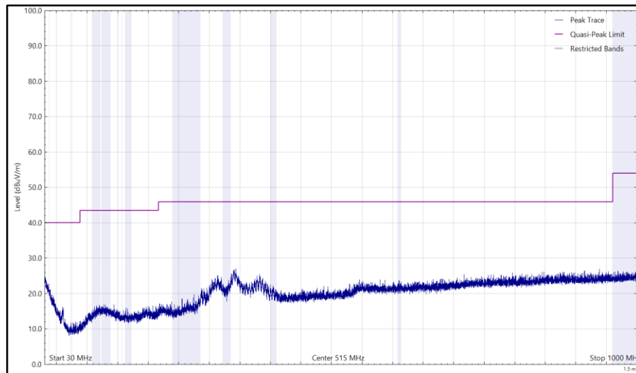
Figure 134 - 2437 MHz (CH6), 802.11b, Core 1, 30 MHz to 1 GHz, Horizontal (Peak)
