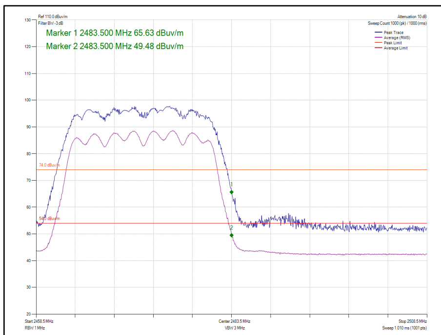
Figure 92 - 802.11n HT20, Core 0-1 - 2472 MHz, Band Edge Frequency 2483.5 MHz
