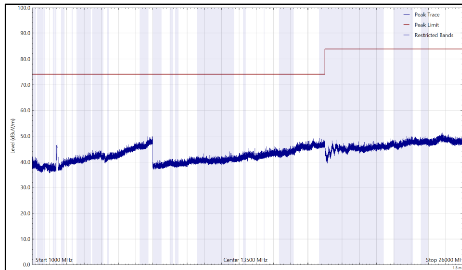
Figure 121 - 2437 MHz (CH6), 802.11b, Core 0, 1 GHz to 26 GHz, Horizontal (Peak)
