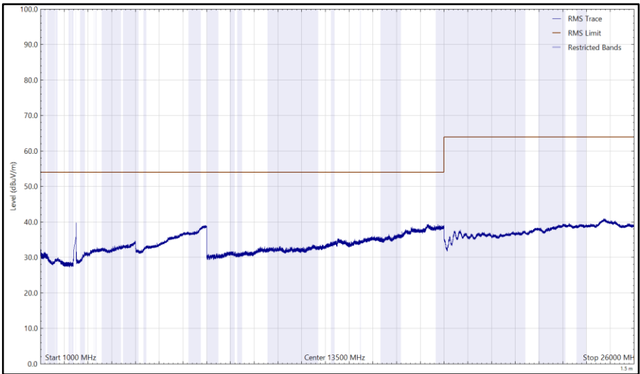
Figure 141 - 2472 MHz (CH13), 802.11b, Core 1, 1 GHz to 26 GHz, Horizontal (RMS)
