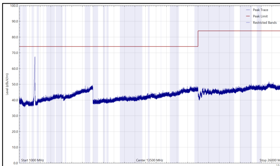
Figure 154 - 2472 MHz (CH13), HE20, RU26-0, Core 0 + Core 1, 1 GHz to 26 GHz, Horizontal (Peak)
