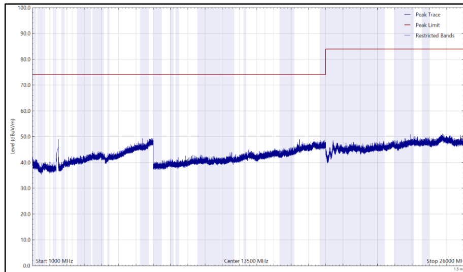
Figure 126 - 2472 MHz (CH13), 802.11b, Core 0, 1 GHz to 26 GHz, Horizontal (Peak)
