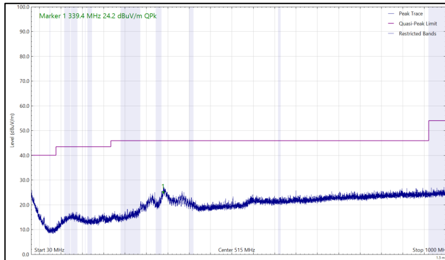
Figure 148 - 2437 MHz (CH6), HE20, RU26-0, Core 0 + Core 1, 30 MHz to 1 GHz, Horizontal (Peak)
