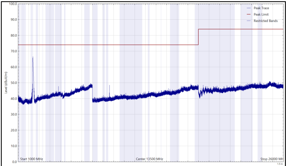
Figure 146 - 2412 MHz (CH1), HE20, RU26-0, Core 0 + Core 1, 1 GHz to 26 GHz, Vertical (Peak)
