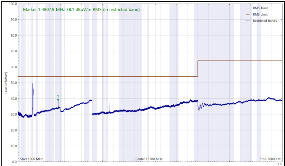
Figure 147 - 2412 MHz (CH1), HE20, RU26-0, Core 0 + Core 1, 1 GHz to 26 GHz, Vertical (RMS)
