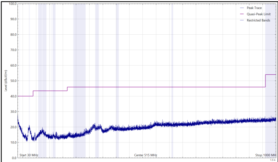
Figure 137 - 2437 MHz (CH6), 802.11b, Core 1, 30 MHz to 1 GHz, Vertical (Peak)
