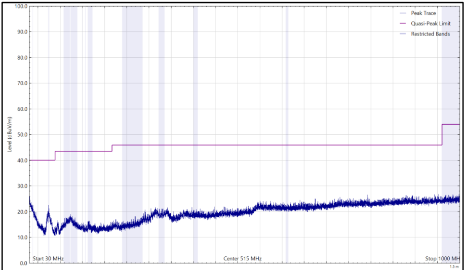
Figure 151 - 2437 MHz (CH6), HE20, RU26-0, Core 0 + Core 1, 30 MHz to 1 GHz, Vertical (Peak)
