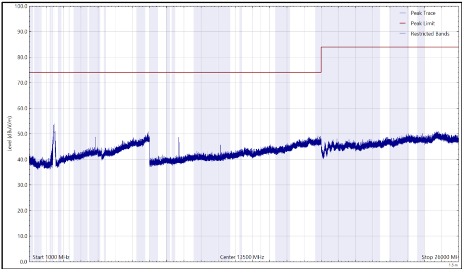
Figure 152 - 2437 MHz (CH6), HE20, RU26-0, Core 0 + Core 1, 1 GHz to 26 GHz, Vertical (Peak)
