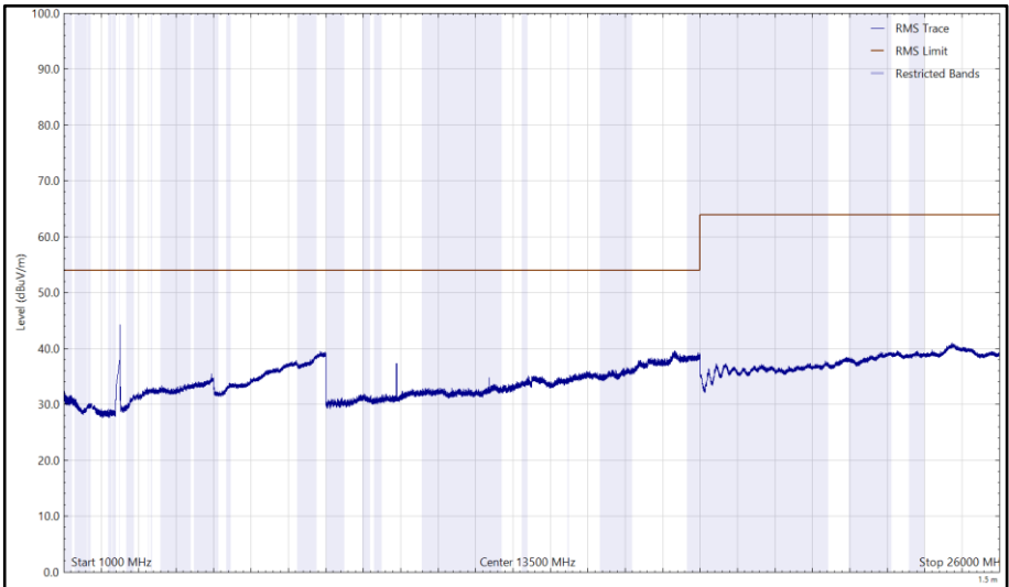
Figure 143 - 2472 MHz (CH13), 802.11b, Core 1, 1 GHz to 26 GHz, Vertical (RMS)
