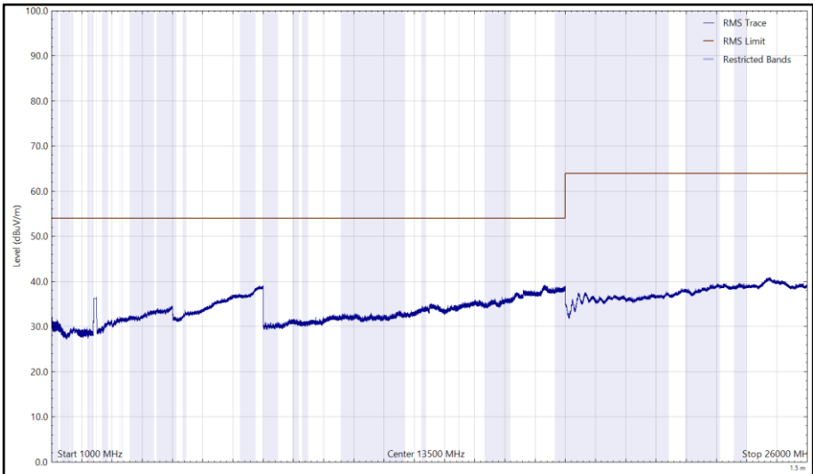
Figure 136 - 2437 MHz (CH6), 802.11b, Core 1, 1 GHz to 26 GHz, Horizontal (RMS)
