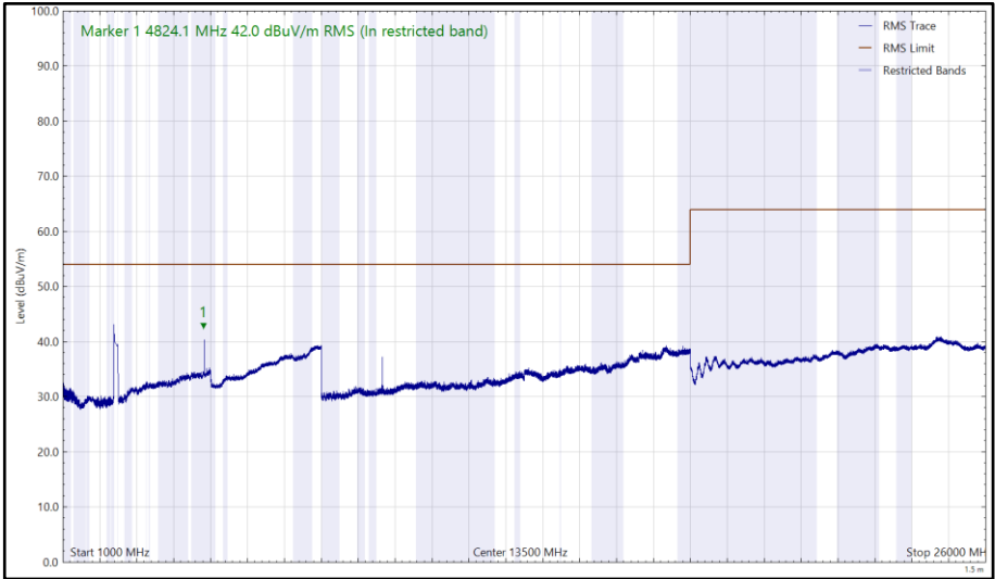
Figure 133 - 2412 MHz (CH1), 802.11b, Core 1, 1 GHz to 26 GHz, Vertical (RMS)
