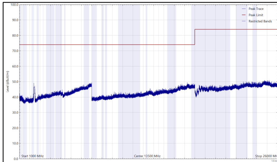
Figure 149 - 2437 MHz (CH6), HE20, RU26-0, Core 0 + Core 1, 1 GHz to 26 GHz, Horizontal (Peak)
