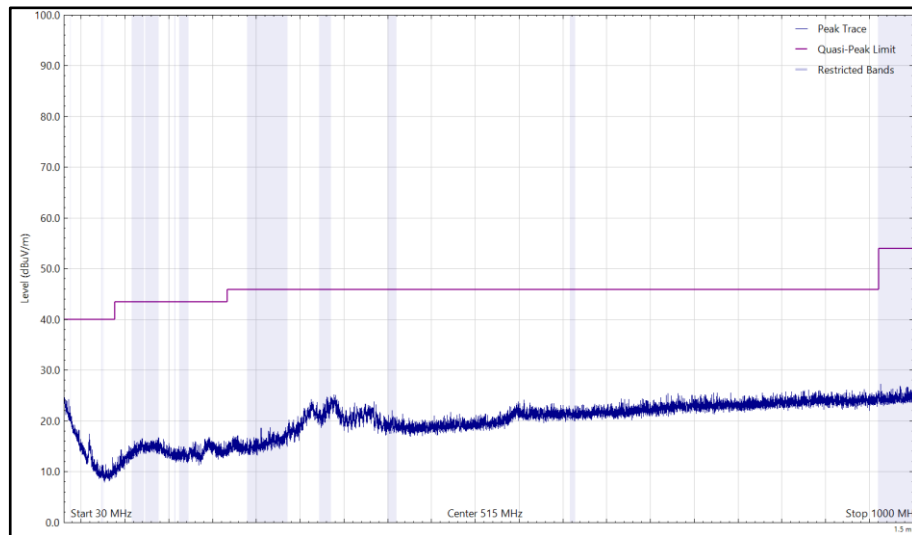
Figure 120 - 2437 MHz (CH6), 802.11b, Core 0, 30 MHz to 1 GHz, Horizontal (Peak)
