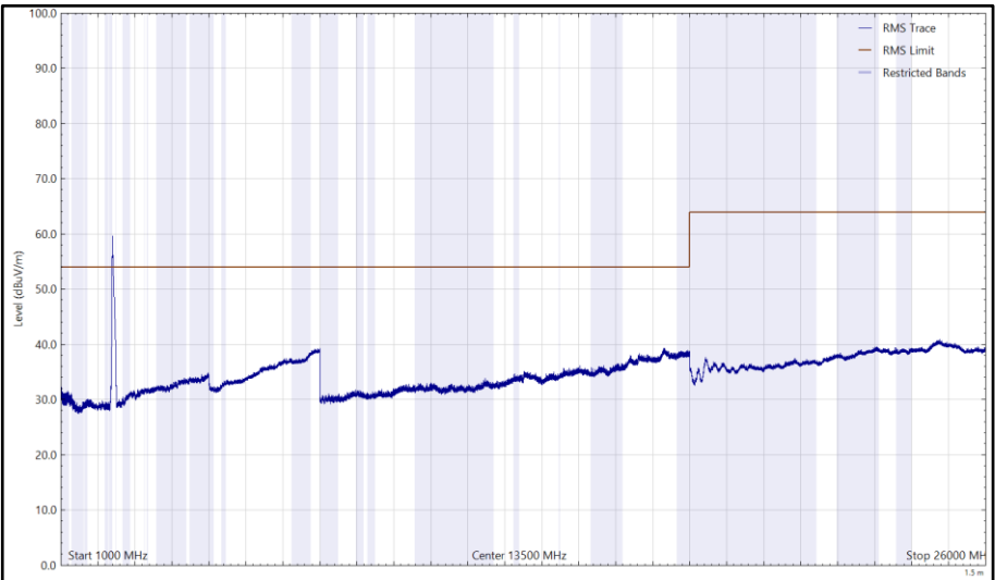
Figure 103 - 2412 MHz (CH1), HT20, CDD, Core 0 + Core 1, 1 GHz to 26 GHz, Horizontal (RMS)
