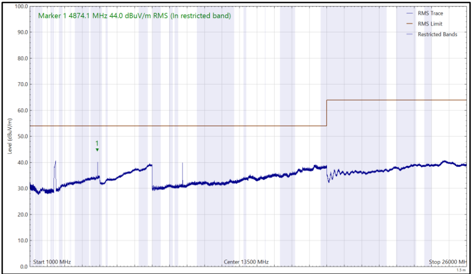
Figure 125 - 2437 MHz (CH6), 802.11b, Core 0, 1 GHz to 26 GHz, Vertical (RMS)
