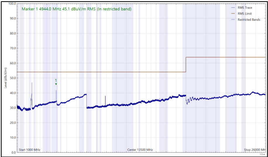
Figure 129 - 2472 MHz (CH13), 802.11b, Core 0, 1 GHz to 26 GHz, Vertical (RMS)
