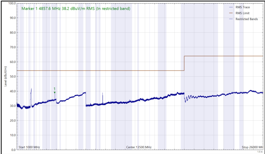
Figure 153 - 2437 MHz (CH6), HE20, RU26-0, Core 0 + Core 1, 1 GHz to 26 GHz, Vertical (RMS)
