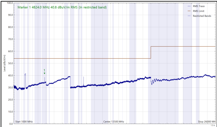
Figure 119 - 2412 MHz (CH1), 802.11b, Core 0, 1 GHz to 26 GHz, Vertical (RMS)
