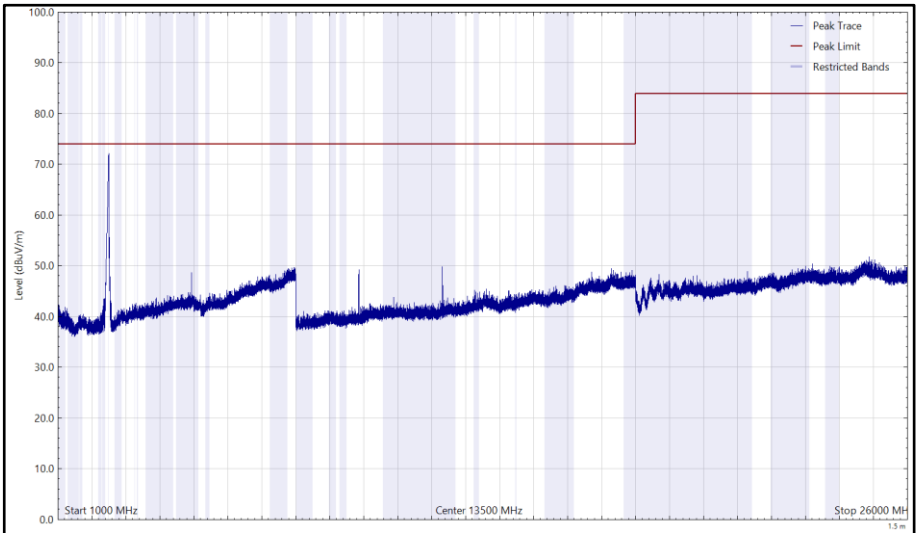
Figure 156 - 2472 MHz (CH13), HE20, RU26-0, Core 0 + Core 1, 1 GHz to 26 GHz, Vertical (Peak)
