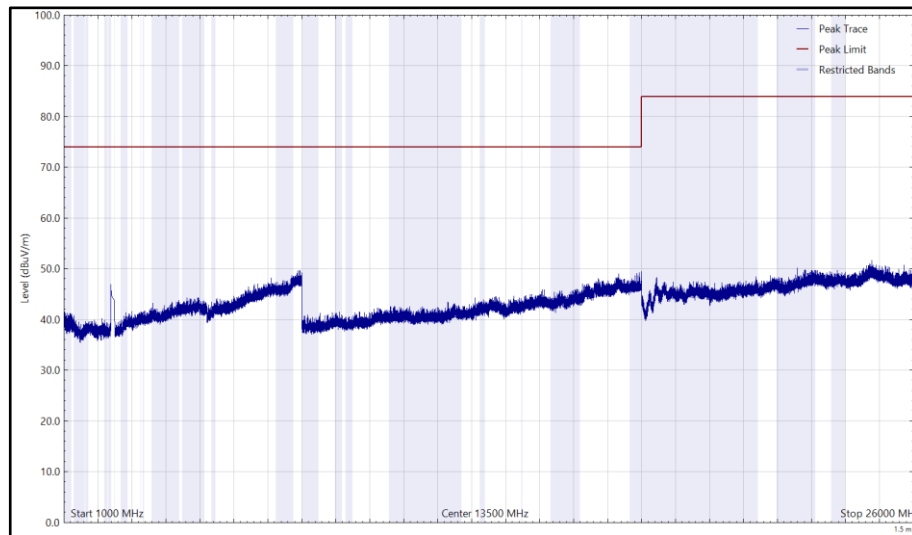
Figure 130 - 2412 MHz (CH1), 802.11b, Core 1, 1 GHz to 26 GHz, Horizontal (Peak)
