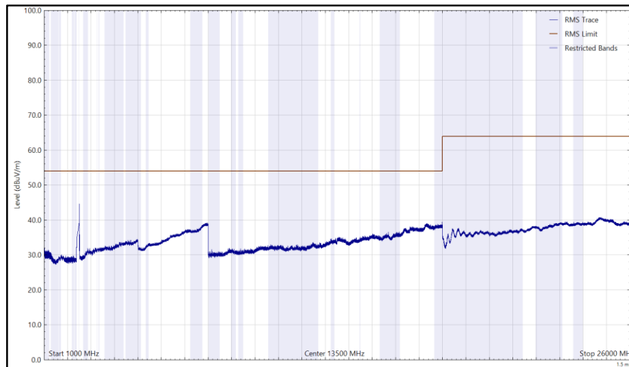
Figure 127 - 2472 MHz (CH13), 802.11b, Core 0, 1 GHz to 26 GHz, Horizontal (RMS)
