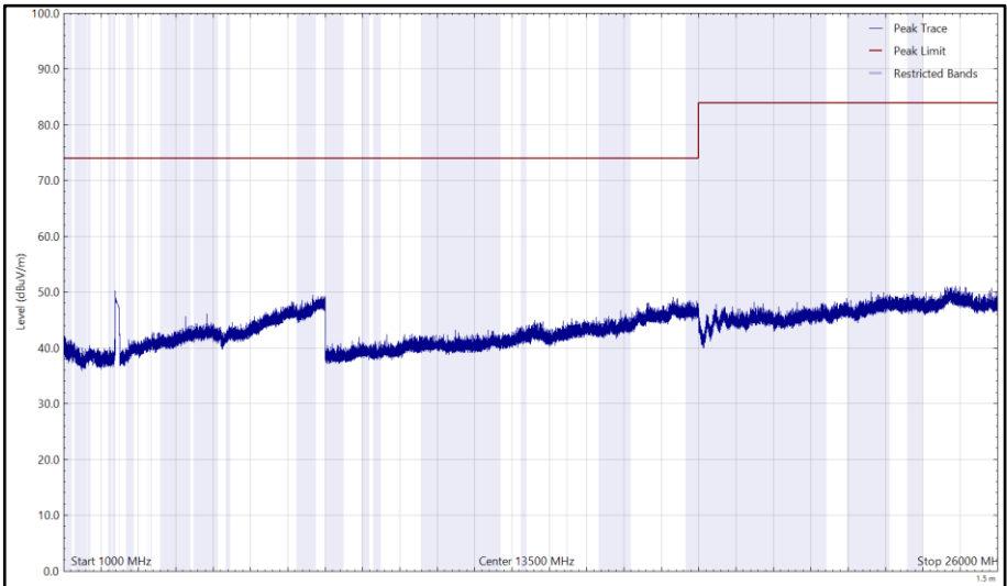
Figure 132 - 2412 MHz (CH1), 802.11b, Core 1, 1 GHz to 26 GHz, Vertical (Peak)
