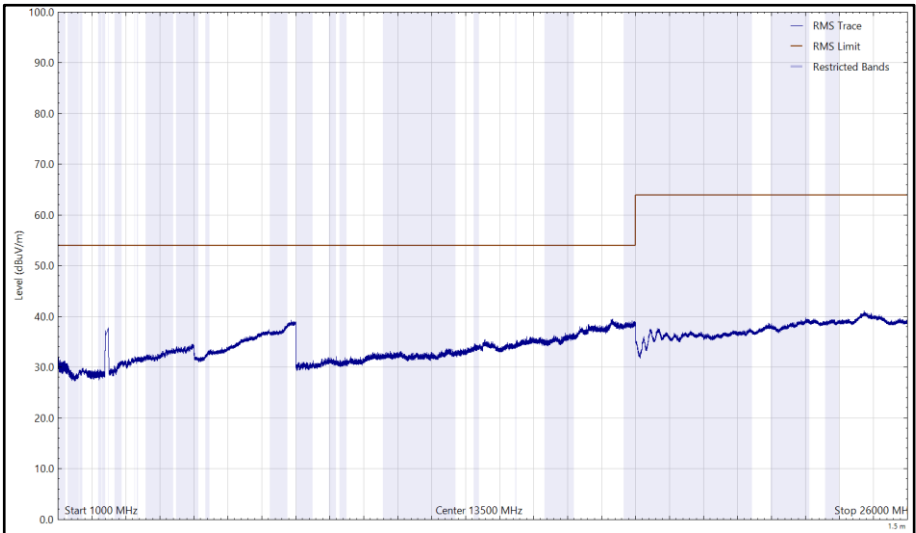
Figure 150 - 2437 MHz (CH6), HE20, RU26-0, Core 0 + Core 1, 1 GHz to 26 GHz, Horizontal (RMS)
