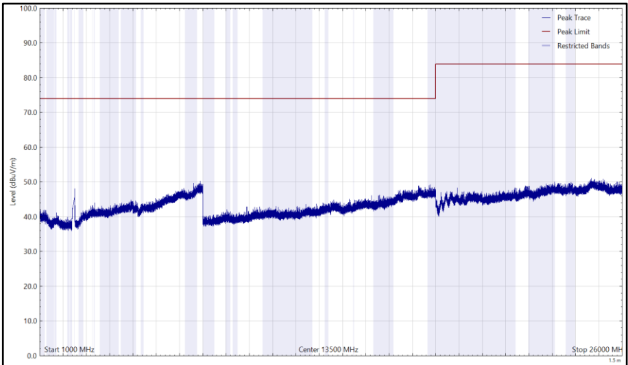
Figure 142 - 2472 MHz (CH13), 802.11b, Core 1, 1 GHz to 26 GHz, Vertical (Peak)
