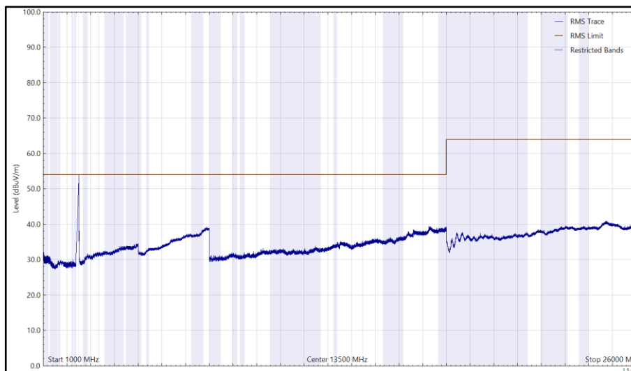
Figure 155 - 2472 MHz (CH13), HE20, RU26-0, Core 0 + Core 1, 1 GHz to 26 GHz, Horizontal (RMS)
