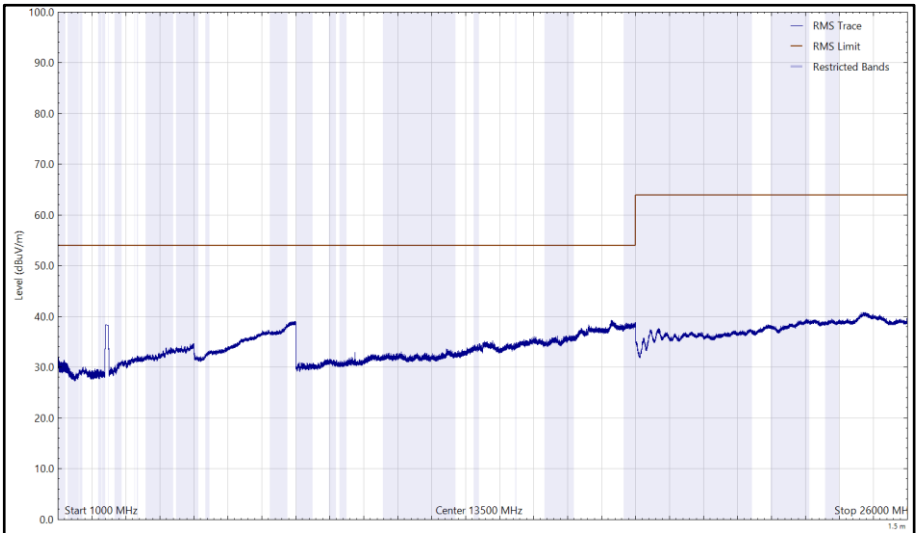
Figure 122 - 2437 MHz (CH6), 802.11b, Core 0, 1 GHz to 26 GHz, Horizontal (RMS)
