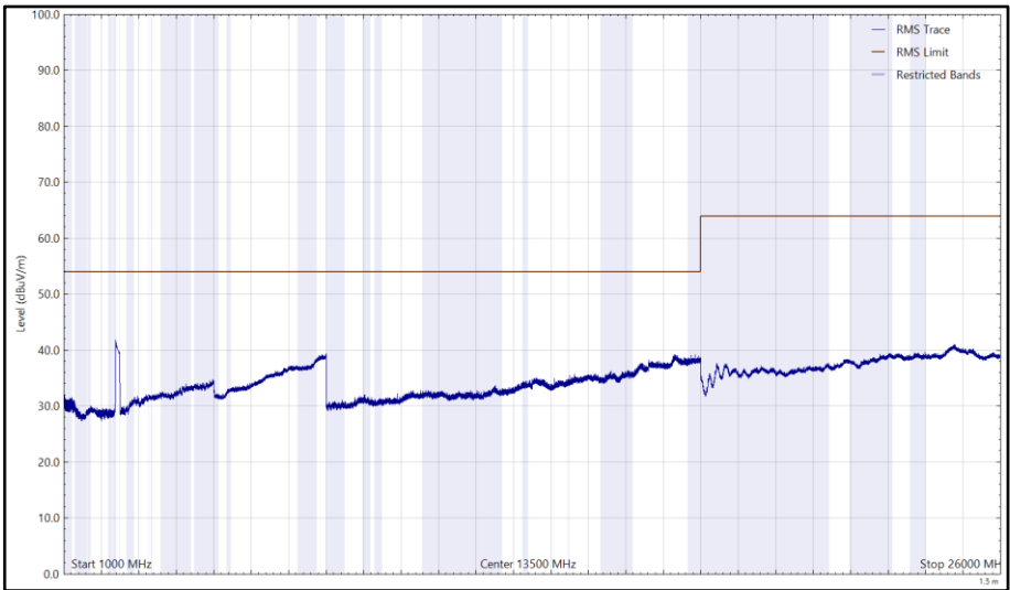
Figure 117 - 2412 MHz (CH1), 802.11b, Core 0, 1 GHz to 26 GHz, Horizontal (RMS)
