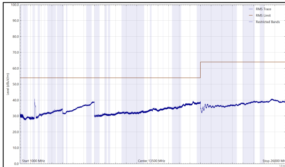
Figure 131 - 2412 MHz (CH1), 802.11b, Core 1, 1 GHz to 26 GHz, Horizontal (RMS)
