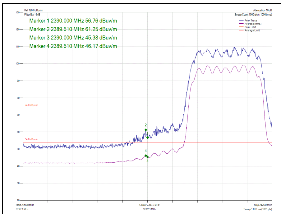
Figure 93 - 802.11ax HE20, Core 0-1, SU - 2412 MHz, Band Edge Frequency 2390 MHz
