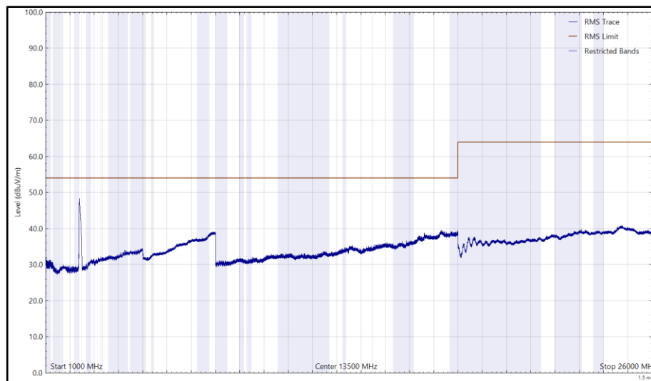
Figure 145 - 2412 MHz (CH1), HE20, RU26-0, Core 0 + Core 1, 1 GHz to 26 GHz, Horizontal (RMS)
