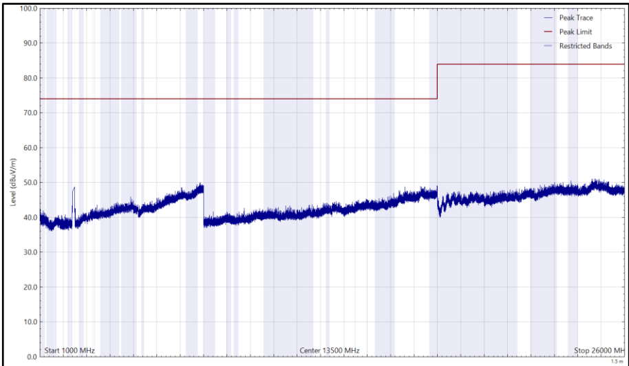
Figure 138 - 2437 MHz (CH6), 802.11b, Core 1, 1 GHz to 26 GHz, Vertical (Peak)
