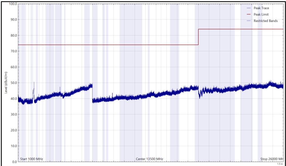
Figure 128 - 2472 MHz (CH13), 802.11b, Core 0, 1 GHz to 26 GHz, Vertical (Peak)
