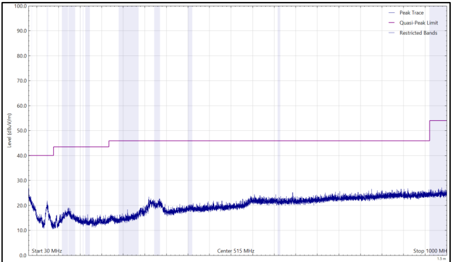
Figure 123 - 2437 MHz (CH6), 802.11b, Core 0, 30 MHz to 1 GHz, Vertical (Peak)
