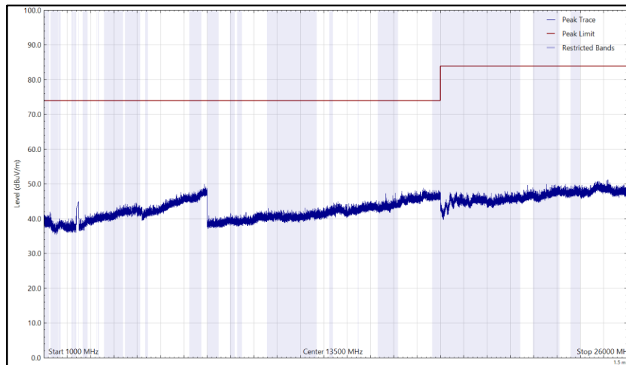
Figure 135 - 2437 MHz (CH6), 802.11b, Core 1, 1 GHz to 26 GHz, Horizontal (Peak)
