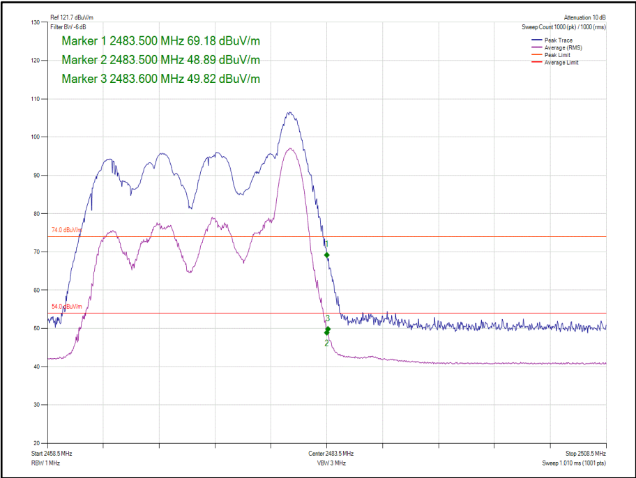
Figure 100 - 802.11ax HE20, Core 0-1, 26-8 - 2472 MHz, Band Edge Frequency 2483.5 MHz FCC 47 CFR Part 15, Limit Clause 15.209
