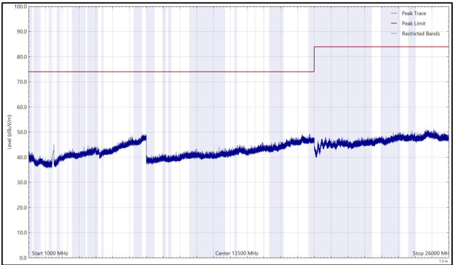
Figure 140 - 2472 MHz (CH13), 802.11b, Core 1, 1 GHz to 26 GHz, Horizontal (Peak)
