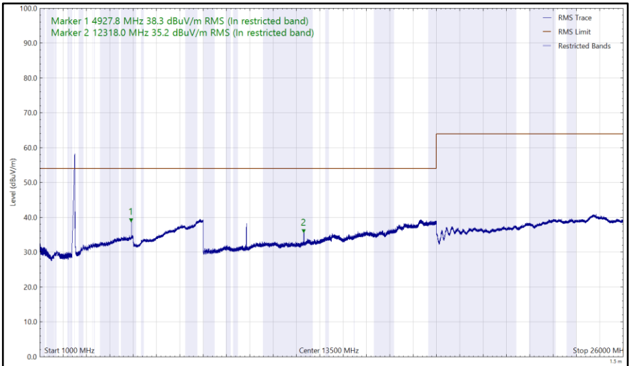
Figure 157 - 2472 MHz (CH13), HE20, RU26-0, Core 0 + Core 1, 1 GHz to 26 GHz, Vertical (RMS)
