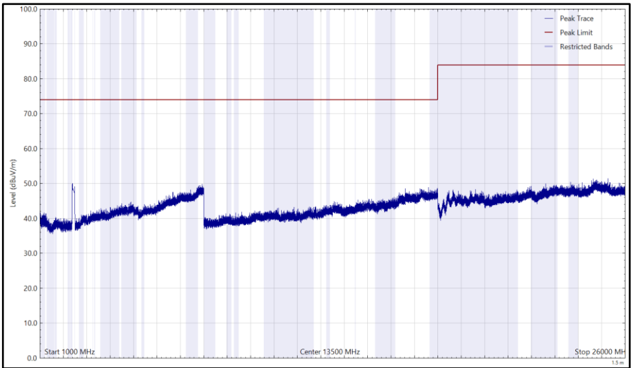
Figure 116 - 2412 MHz (CH1), 802.11b, Core 0, 1 GHz to 26 GHz, Horizontal (Peak)
