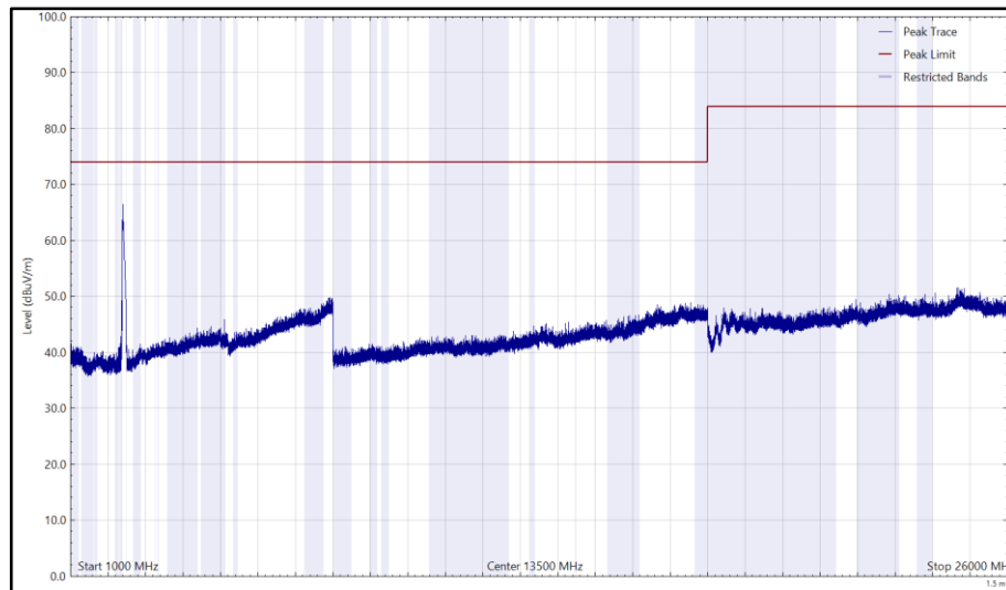
Figure 144 - 2412 MHz (CH1), HE20, RU26-0, Core 0 + Core 1, 1 GHz to 26 GHz, Horizontal (Peak)
