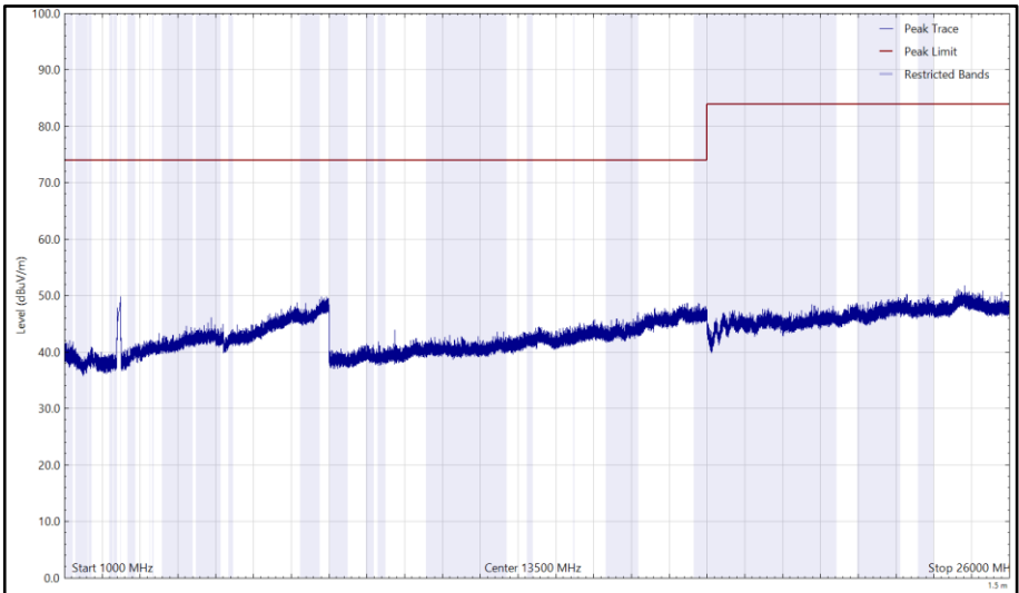
Figure 124 - 2437 MHz (CH6), 802.11b, Core 0, 1 GHz to 26 GHz, Vertical (Peak)
