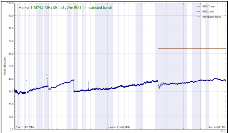
Figure 139 - 2437 MHz (CH6), 802.11b, Core 1, 1 GHz to 26 GHz, Vertical (RMS)
