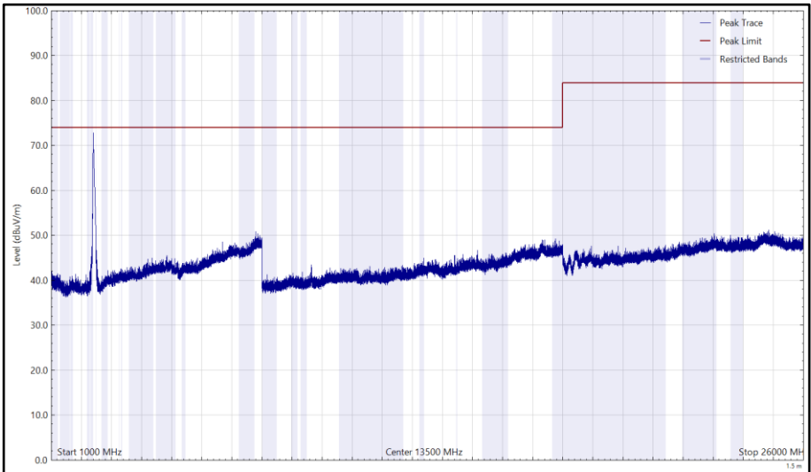
Figure 104 - 2412 MHz (CH1), HT20, CDD, Core 0 + Core 1, 1 GHz to 26 GHz, Vertical (Peak)
