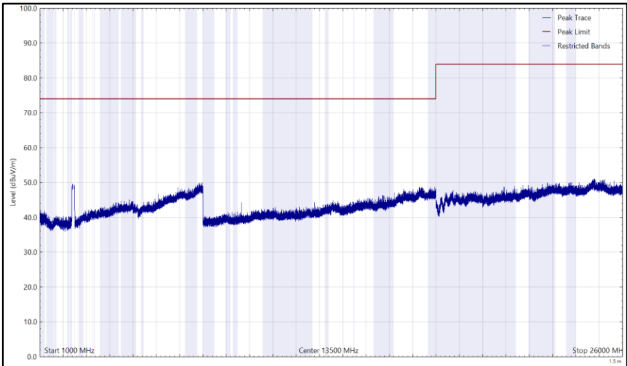
Figure 118 - 2412 MHz (CH1), 802.11b, Core 0, 1 GHz to 26 GHz, Vertical (Peak)
