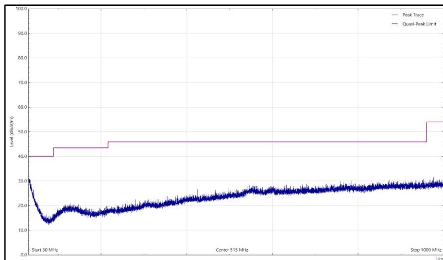
Figure 8 – 2452 MHz (CH9), HT20, CDD, Core 0 + Core 1 and 2402 MHz (CH0), DH5, ePA, Core 0, 30 MHz to 1 GHz, Horizontal, Q-Peak
