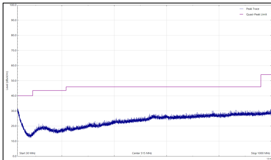
Figure 2 – 2417 MHz (CH2), HT20, CDD, Core 0 + Core 1 and 2480 MHz (CH78), DH5, ePA, Core 0, 30 MHz to 1 GHz, Horizontal, Q-Peak
