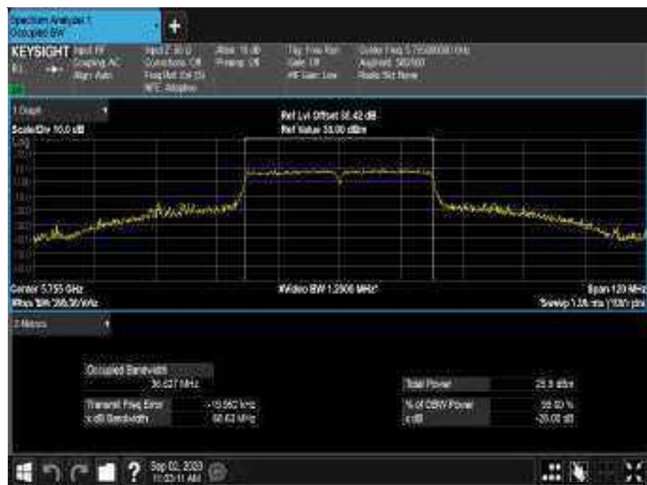
Figure 747 - 5755 MHz - 99% Occupied Bandwidth
