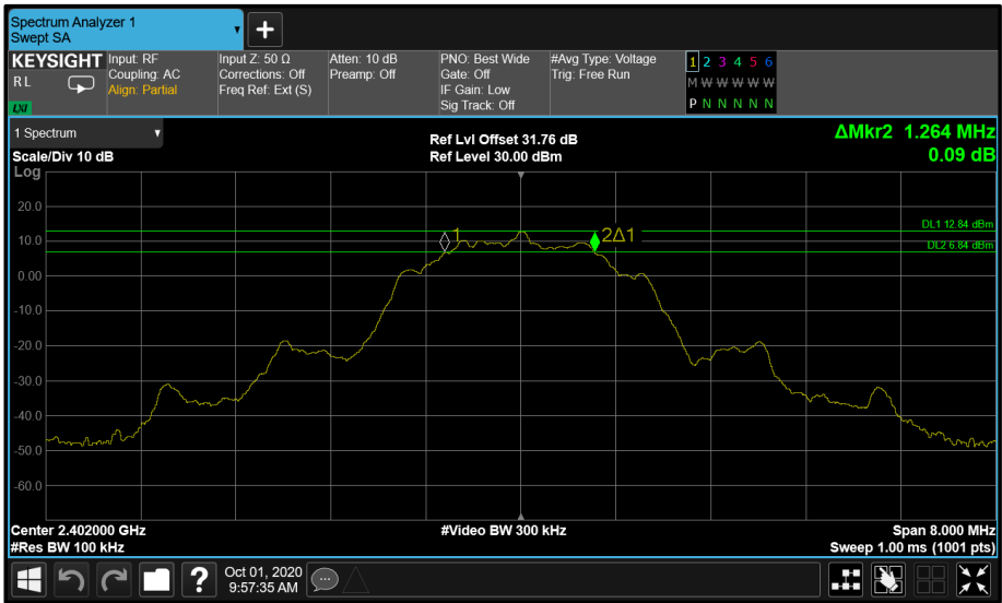
Figure 79 - Core 0 LE 2M 2402 MHz (CH0) 6dB & 99% Bandwidth
