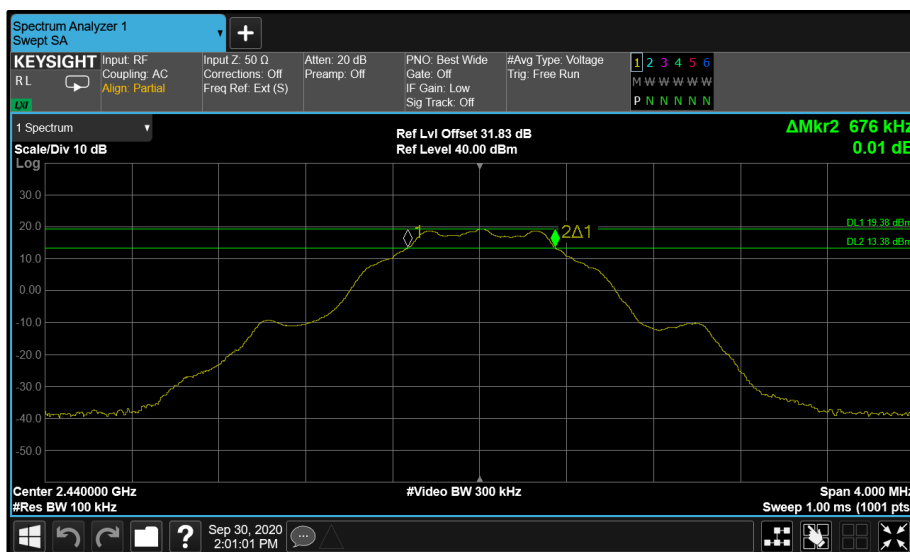
Figure 56 - Core 0 LE 1M 2440 MHz (CH19) 6dB & 99% Bandwidth
