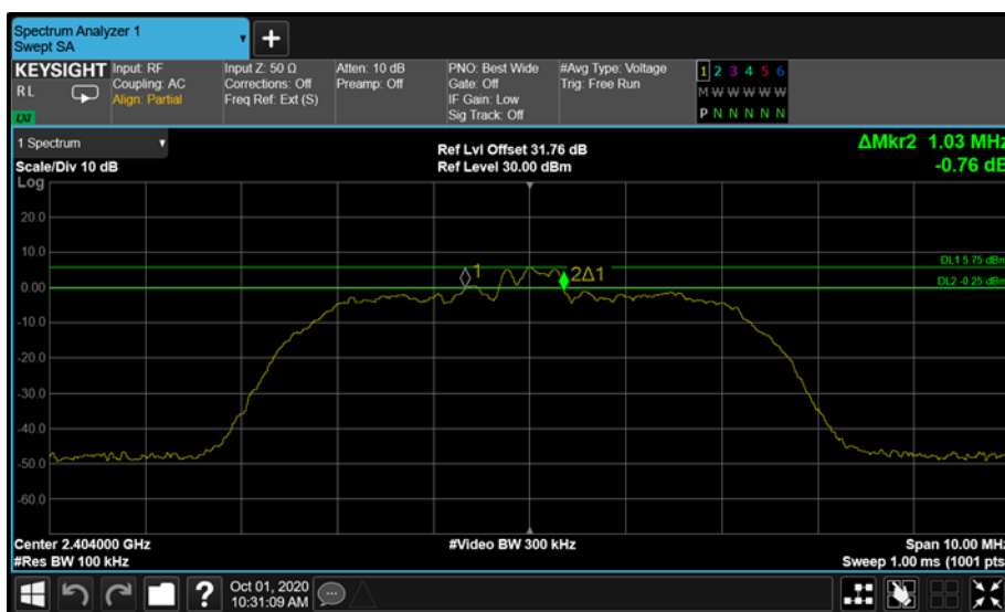
Figure 7 - Core 0 HDR8 2404 MHz (CH2) 6dB & 99% Bandwidth
