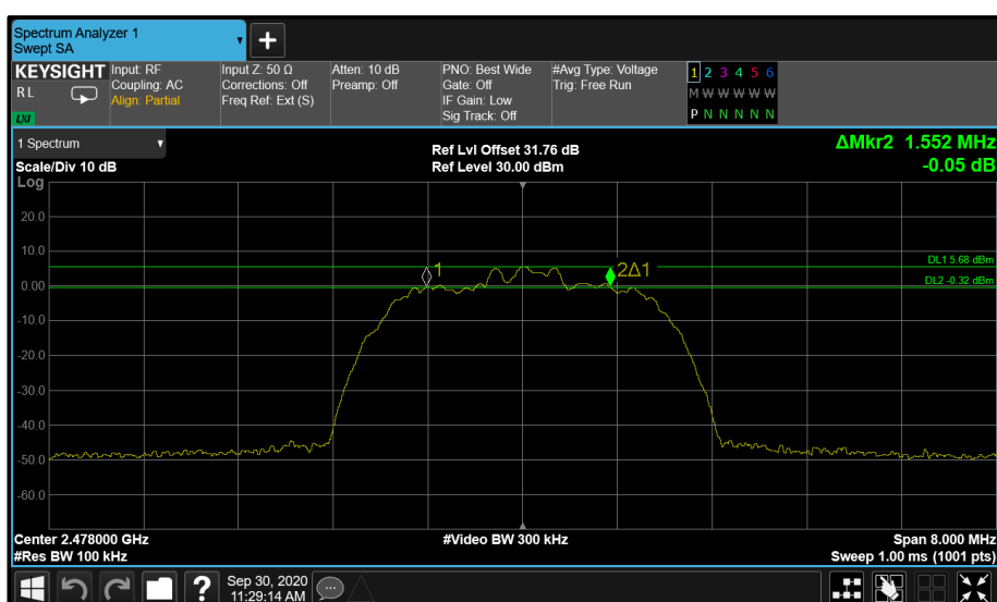
Figure 6 - Core 2 HDR4 2478 MHz (CH76) 6dB & 99% Bandwidth
