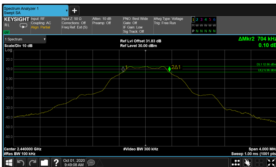
Figure 75 - Core 0 LE 1M 2440 MHz (CH19) 6dB & 99% Bandwidth
