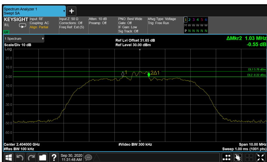
Figure 10 - Core 2 HDR8 2404 MHz (CH2) 6dB & 99% Bandwidth
