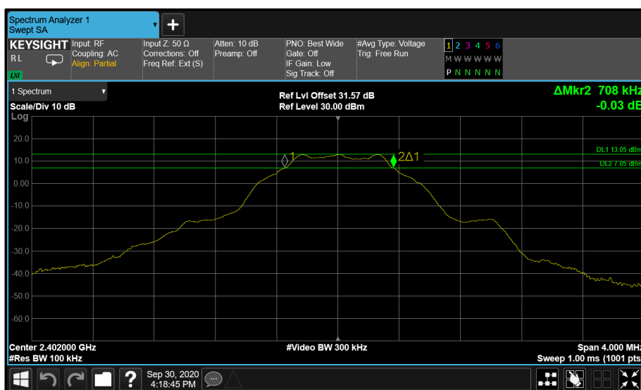
Figure 74 - Core 1 LE 1M 2402 MHz (CH0) 6dB & 99% Bandwidth
