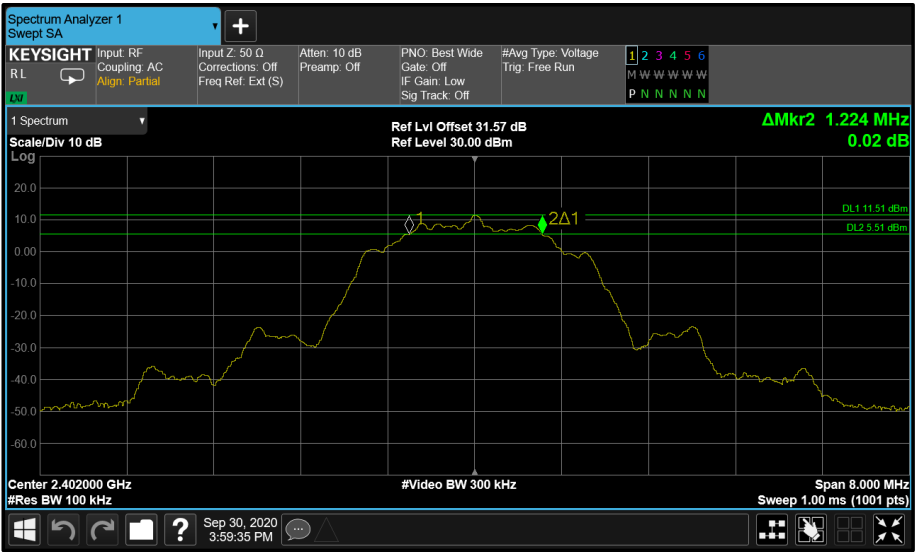
Figure 44 - Core 1 LE 2M 2402 MHz (CH0) 6dB & 99% Bandwidth
