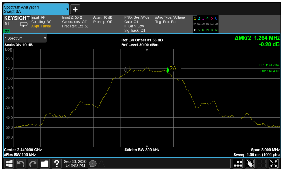
Figure 46 - Core 1 LE 2M 2440 MHz (CH19) 6dB & 99% Bandwidth
