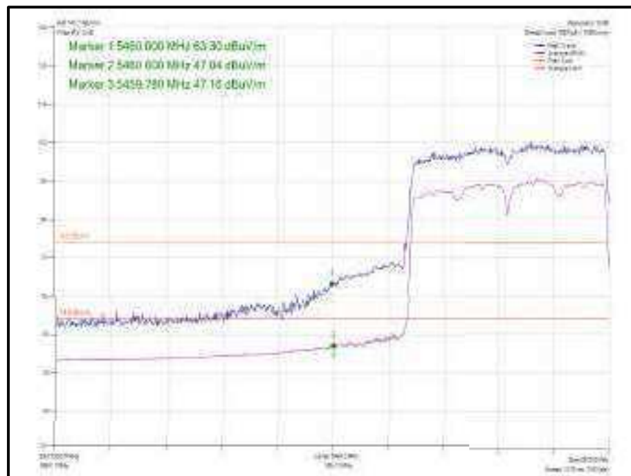
Figure 1102 - 802.11ac VHT80, Core0 - 5530 MHz Band Edge Frequency 5530 MHz
