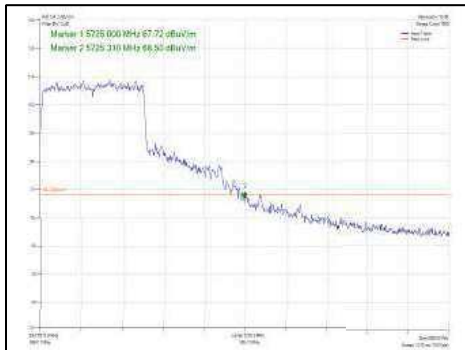
Figure 1026 - 802.11ac VHT80 SDM, Cores 0-1 - 5610 MHz Band Edge Frequency 5725 MHz
