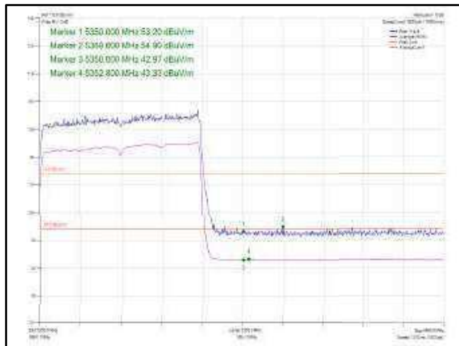
Figure 1105 - 802.11ax HE80, Core 0, SU - 5290 MHz Band Edge Frequency 5350 MHz
