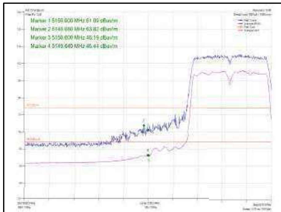
Figure 1083 - 802.11n HT40 SDM Cores 0-1 - 5190 MHz Band Edge Frequency 5150 MHz
