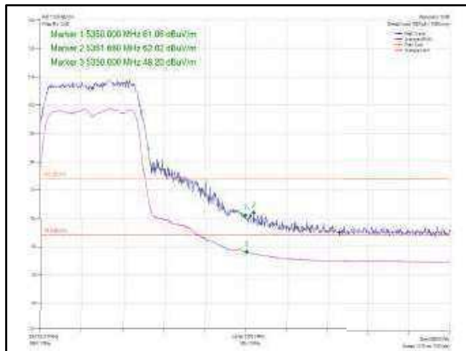
Figure 1062 - 802.11n HT20 SDM, Cores 0-1 - 5320 MHz Band Edge Frequency 5350 MHz
