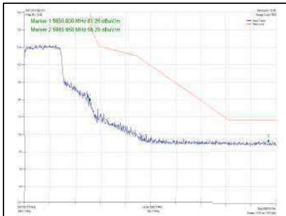
Figure 945 - 802.11ax HE20, Core 1, SU - 5825 MHz Band Edge Frequency 5850 MHz
