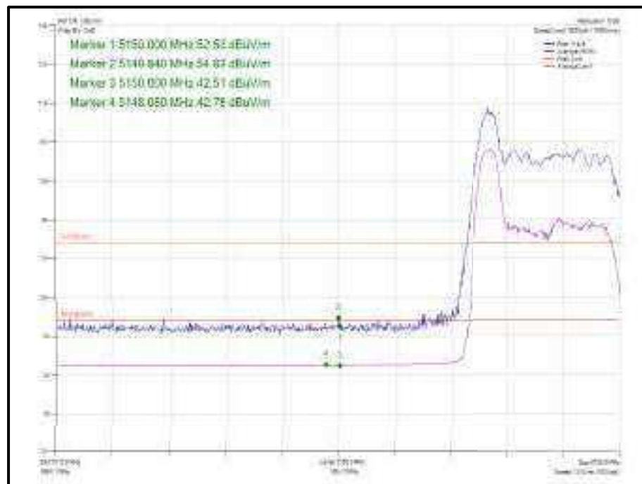
Figure 1046 - 802.11ax HE20, Core0, 26-0 - 5180 MHz, B and E dge Frequency 5150 MHz
