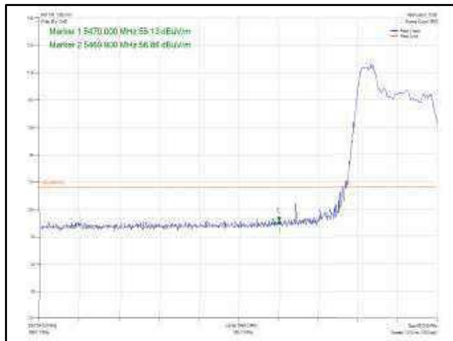
Figure 934 - 802.11 a HE20, Core 0, 52.37 - 5500 MHz Band Edge Frequency 5470 MHz
