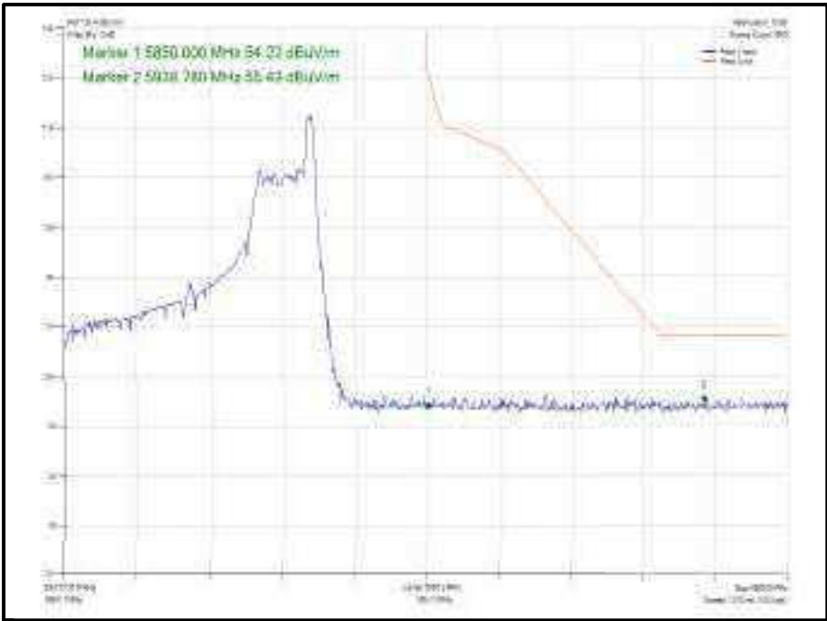
Figure 1018 - 802.11ax HE80 Core 126-36 - 5775 MHz Band Edge Frequency 5850 MHz
