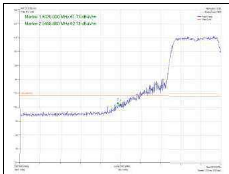
Figure 948 - 802.11 n HT20 SDM, Cores 0-1 - 5500 MHz Band Edge Frequency 5470 MHz
