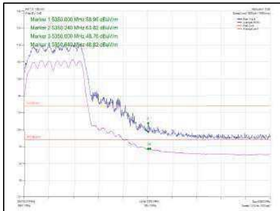
Figure 1061 - 802.11n HT20 CDD, Cores 0-1 - 5320 MHz Band Edge Frequency 5350 MHz
