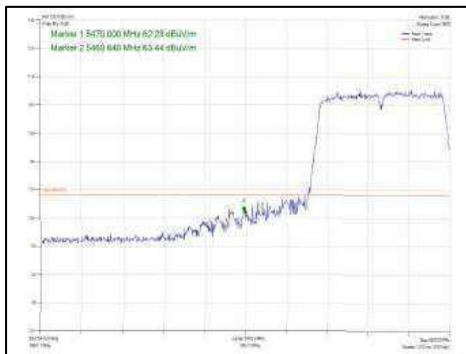
Figure 984 - 802.11 n HT40 SDM, Cores 0-1 - 5510 MHz Band Edge Frequency 5470 MHz
