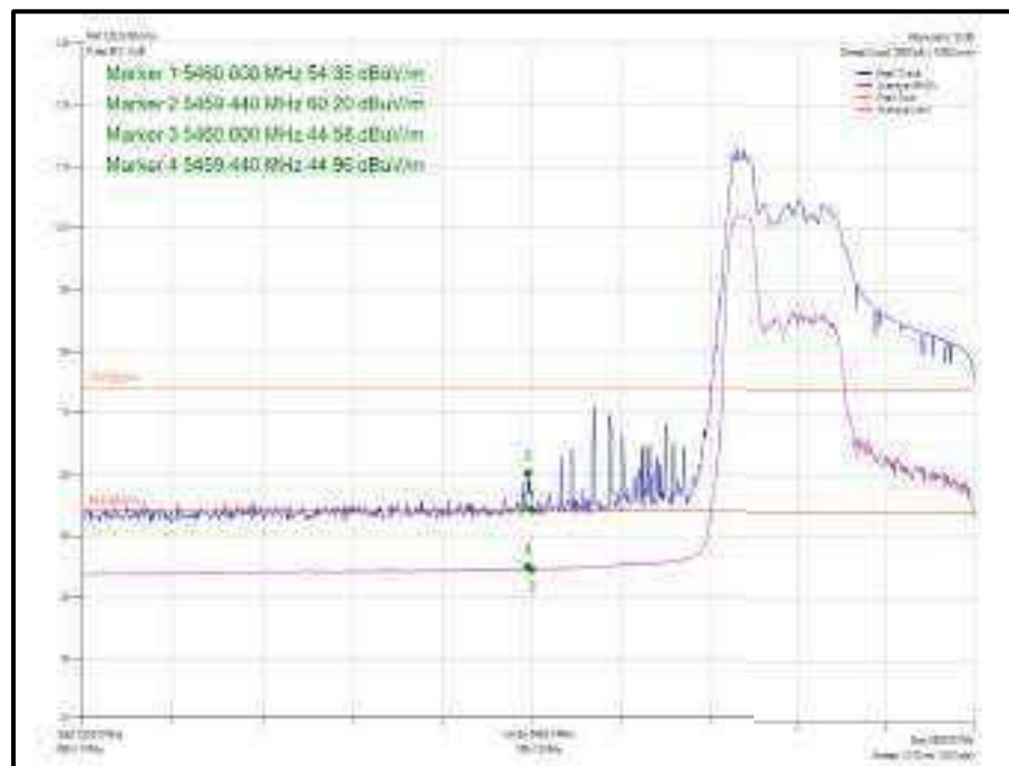
Figure 1081 - 802.11ax HE40, Core 0, 52-37- 5510 MHz Band Edge Frequency 5460 MHz
