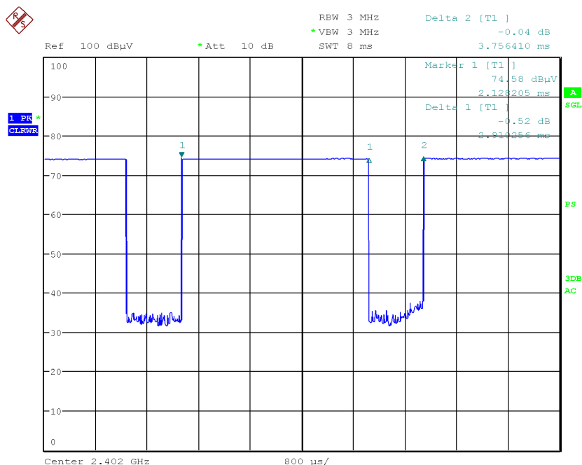
Figure 8-6 Bluetooth Transmission Plot & Duty Cycle Calculation – Antenna A Variant 2
