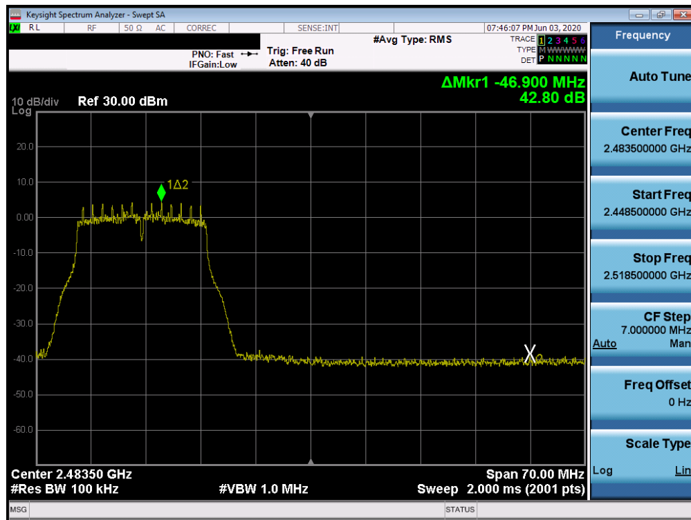
Plot 7-72. Band Edge Plot SISO CORE 1 (802.11g – Ch. 11)
