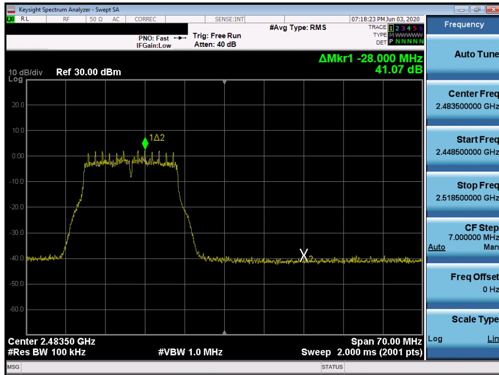
Plot 7-57. Band Edge Plot SISO CORE 0 (802.11g – Ch. 12)
