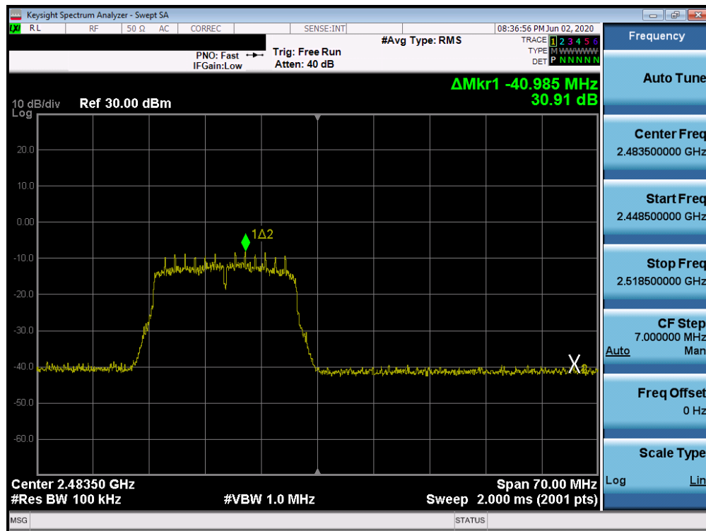
Plot 7-64. Band Edge Plot SISO CORE 0 (802.11n) (2.4GHz) – Ch. 13)
