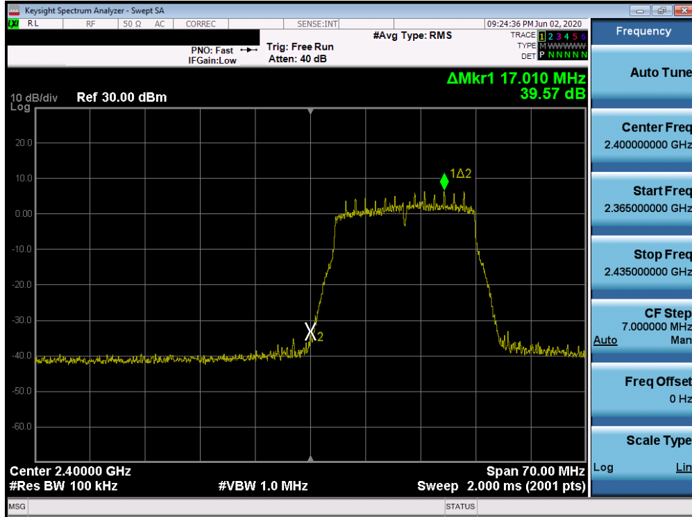
Plot 7-75. Band Edge Plot SISO CORE 1 (802.11n (2.4GHz) – Ch. 1)
