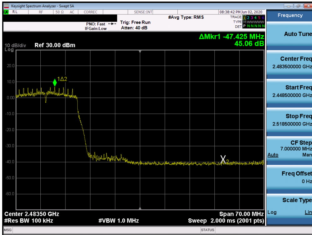
Plot 7-61. Band Edge Plot SISO CORE 0 (802.11n (2.4GHz) – Ch. 10)
