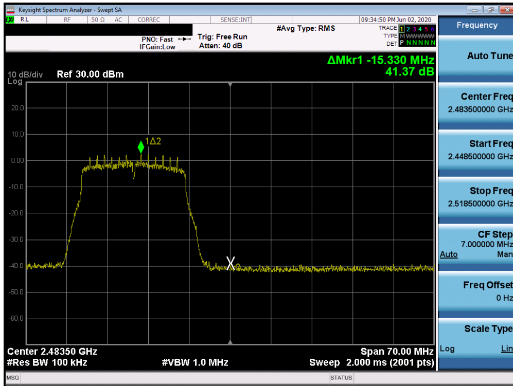
Plot 7-79. Band Edge Plot SISO CORE 1 (802.11n (2.4GHz) – Ch. 12)
