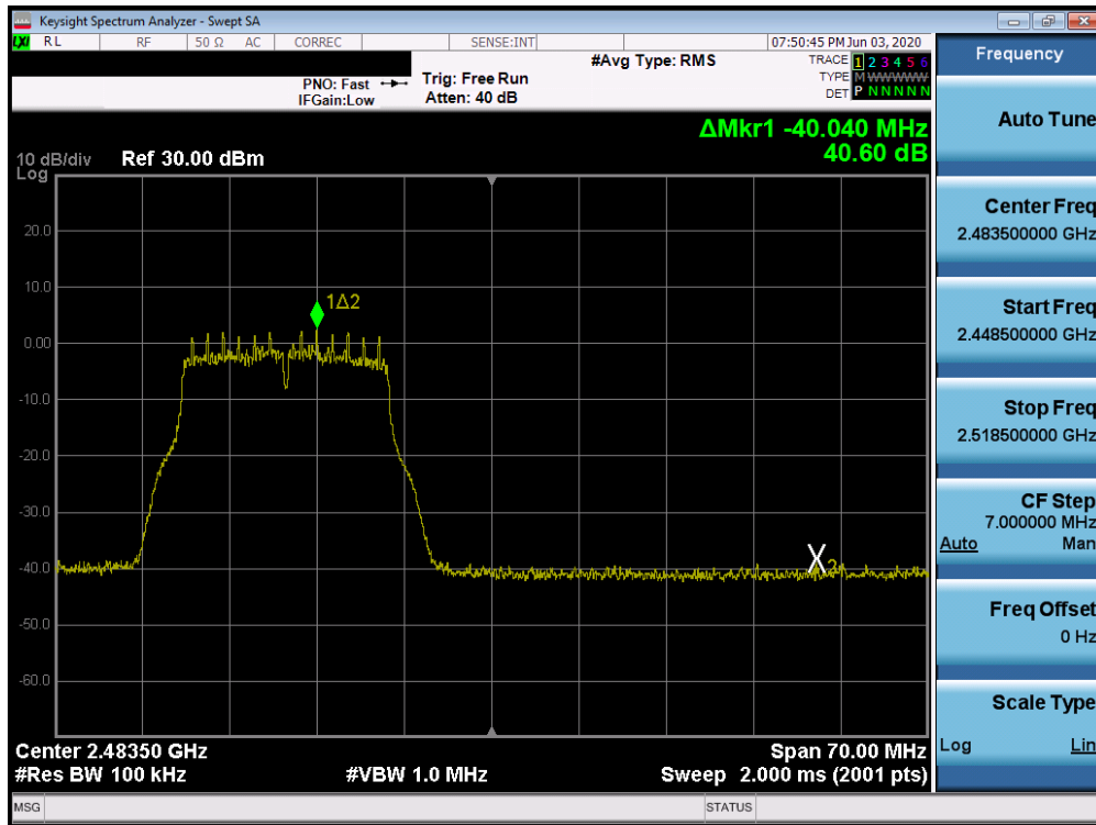
Plot 7-73. Band Edge Plot SISO CORE 1 (802.11g – Ch. 12)
