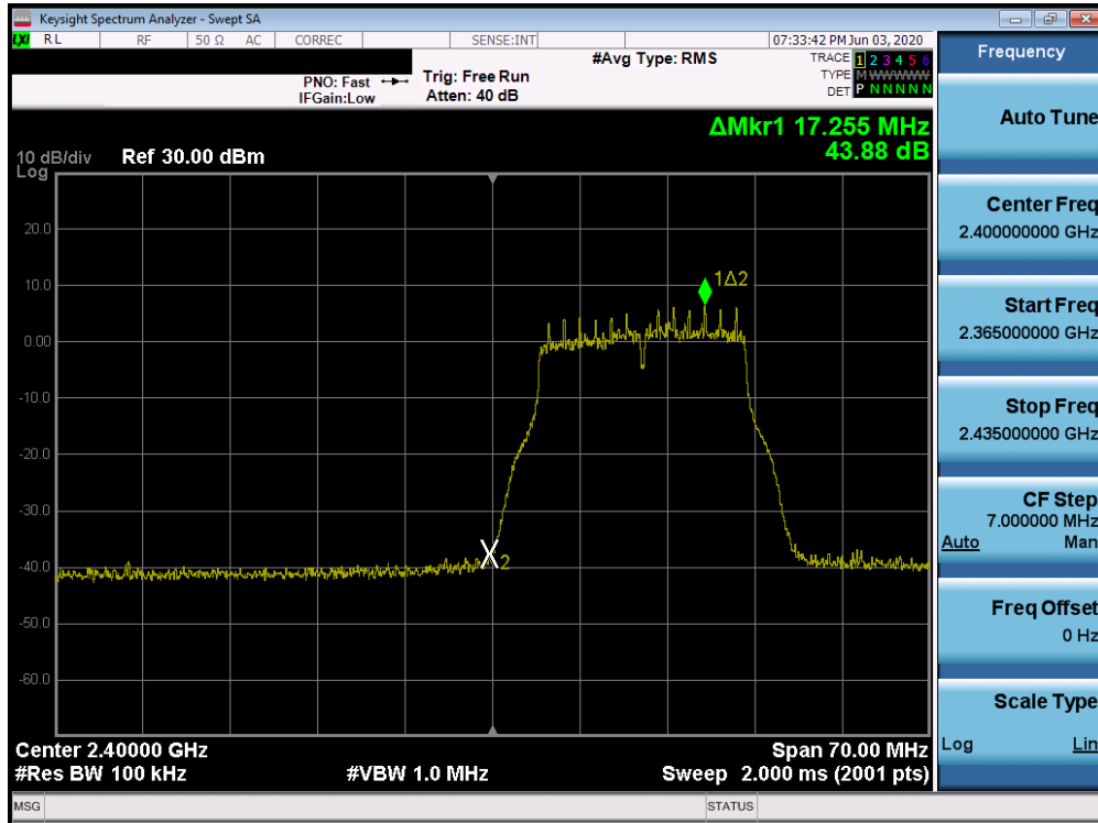
Plot 7-69. Band Edge Plot SISO CORE 1 (802.11g- Ch. 1)
