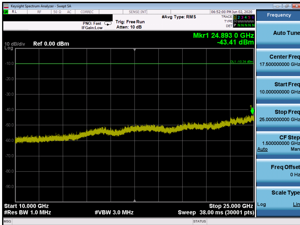
Plot 7-82. Conducted Spurious Plot SISO CORE 0 (802.11b – Ch. 1)
