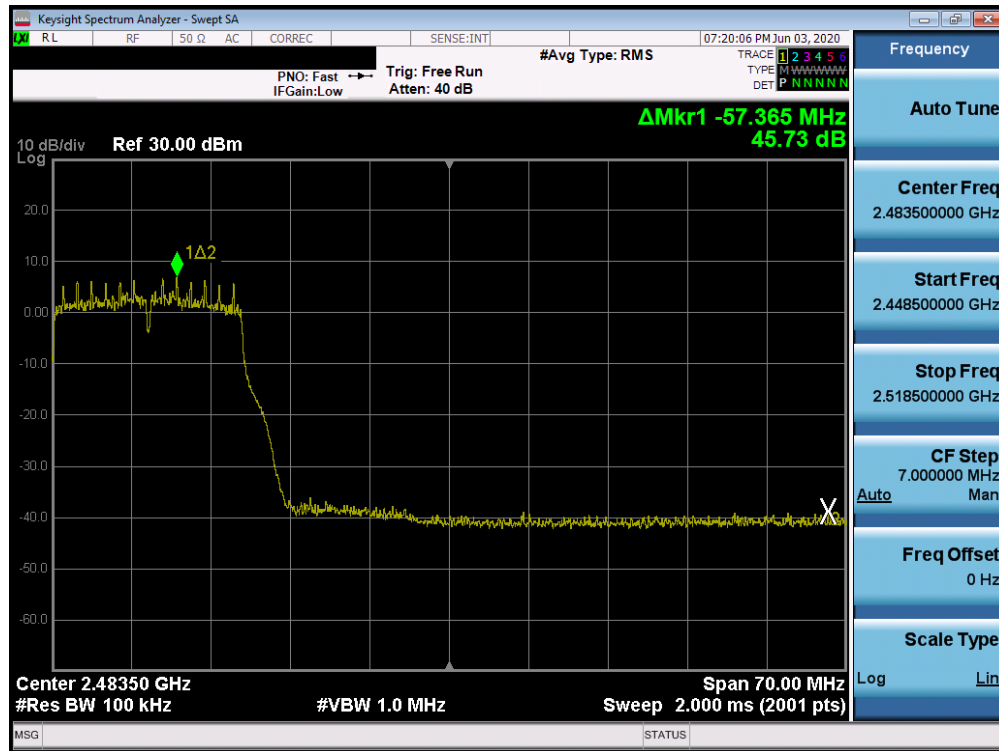
Plot 7-55. Band Edge Plot SISO CORE 0 (802.11g – Ch. 10)
