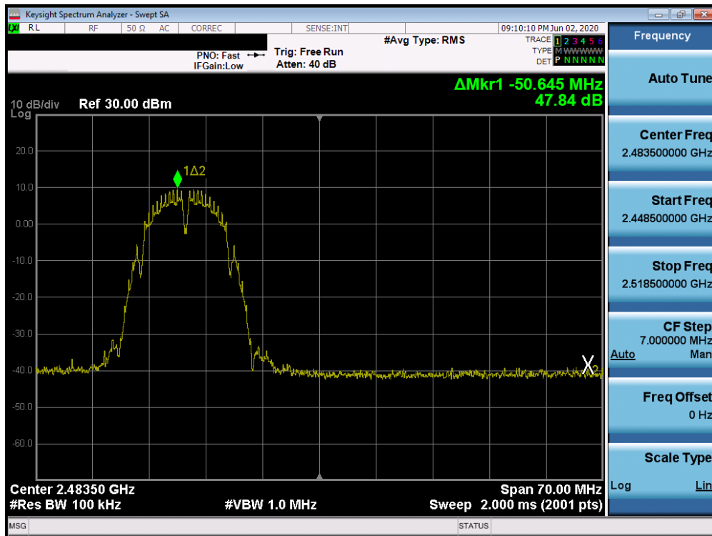
Plot 7-67. Band Edge Plot SISO CORE 1 (802.11b – Ch. 12)
