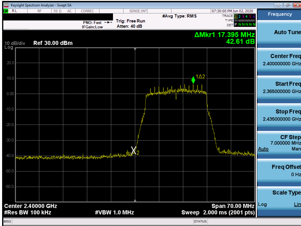
Plot 7-59. Band Edge Plot SISO CORE 0 (802.11n (2.4GHz) – Ch. 1)
