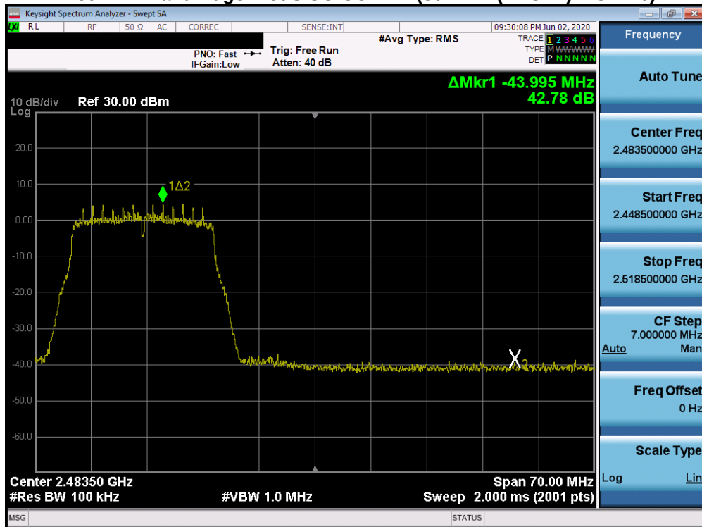
Plot 7-78. Band Edge Plot SISO CORE 1 (802.11n) (2.4GHz) - Ch. 11
