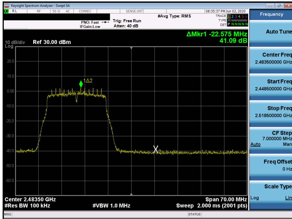
Plot 7-63. Band Edge Plot SISO CORE 0 (802.11n) (2.4GHz) – Ch. 12)
