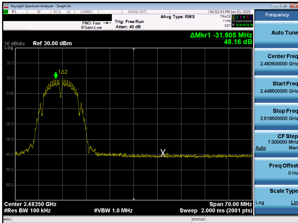
Plot 7-66. Band Edge Plot SISO CORE 1 (802.11b – Ch. 11)
