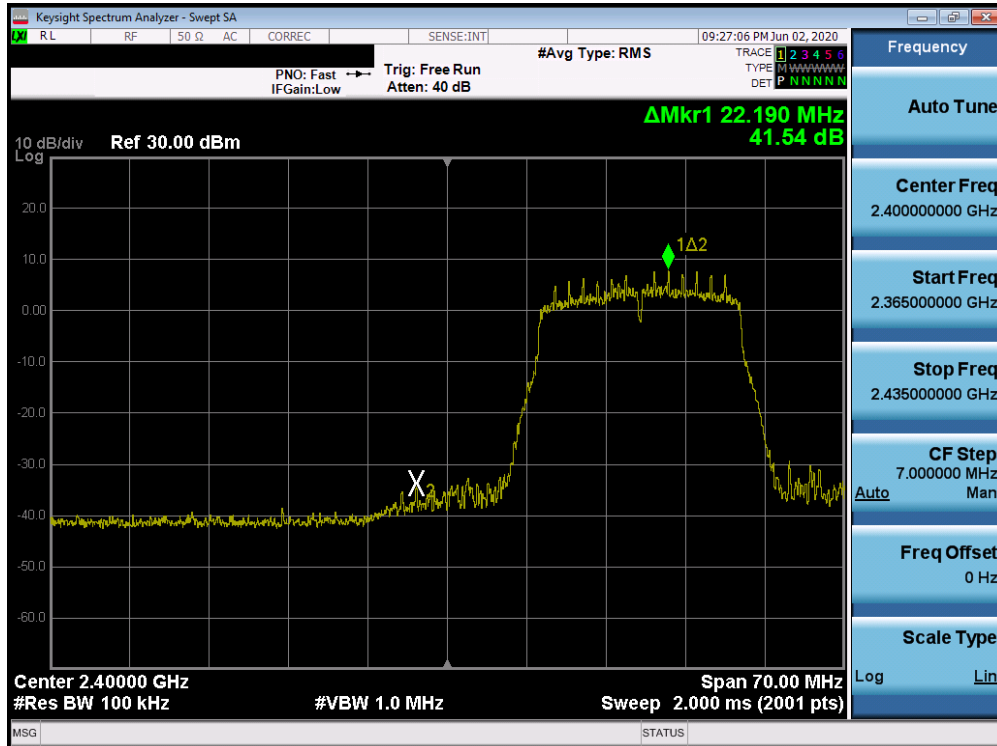
Plot 7-76. Band Edge Plot SISO CORE 1 (802.11n (2.4GHz) – Ch. 2)
