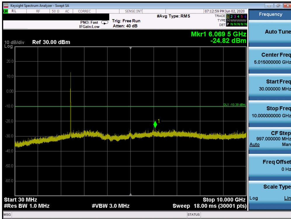
Plot 7-83. Conducted Spurious Plot SISO CORE 0 (802.11b – Ch. 6)
