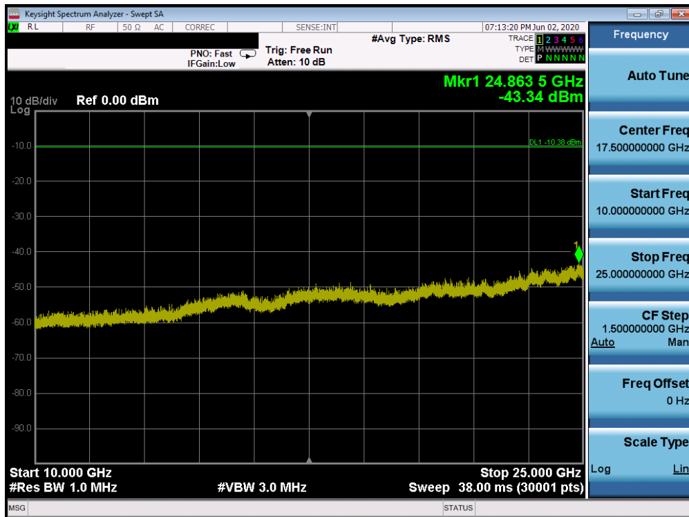
Plot 7-84. Conducted Spurious Plot SISO CORE 0 (802.11b – Ch. 6)
