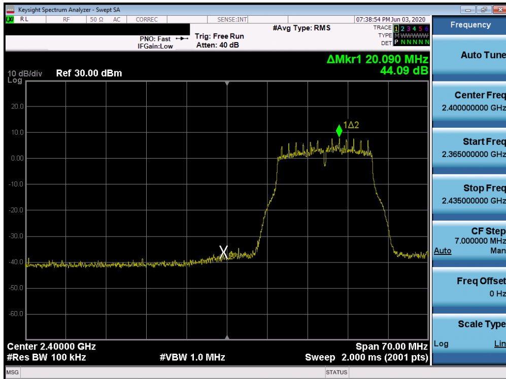
Plot 7-70. Band Edge Plot SISO CORE 1 (802.11g- Ch. 2)
