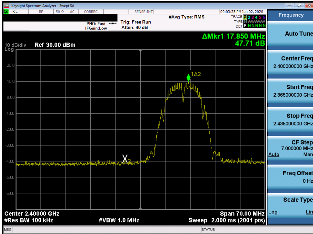
Plot 7-65. Band Edge Plot SISO CORE 1 (802.11b – Ch. 1)
