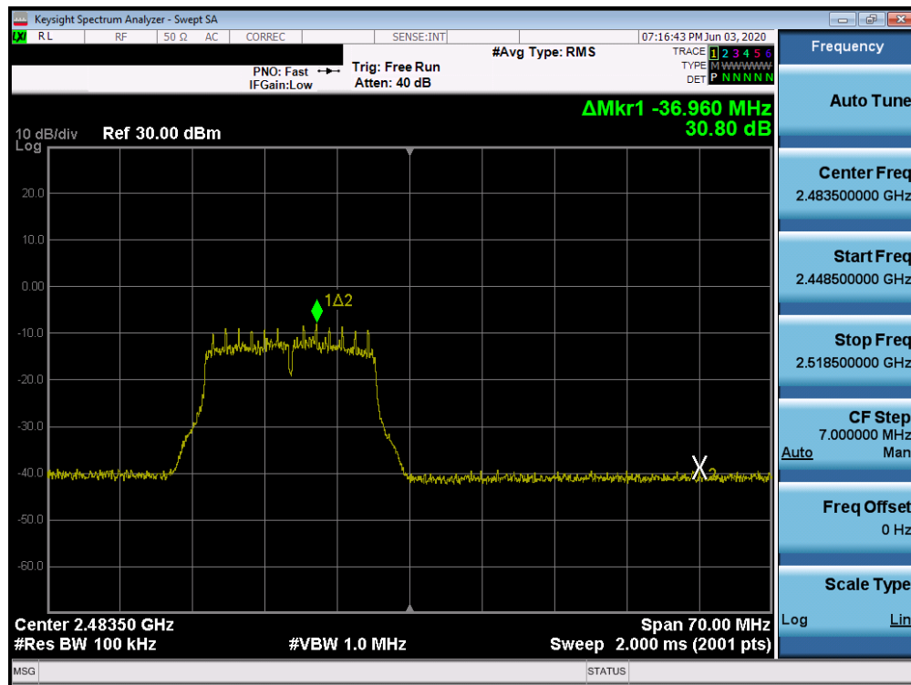
Plot 7-58. Band Edge Plot SISO CORE 0 (802.11g – Ch. 13)
