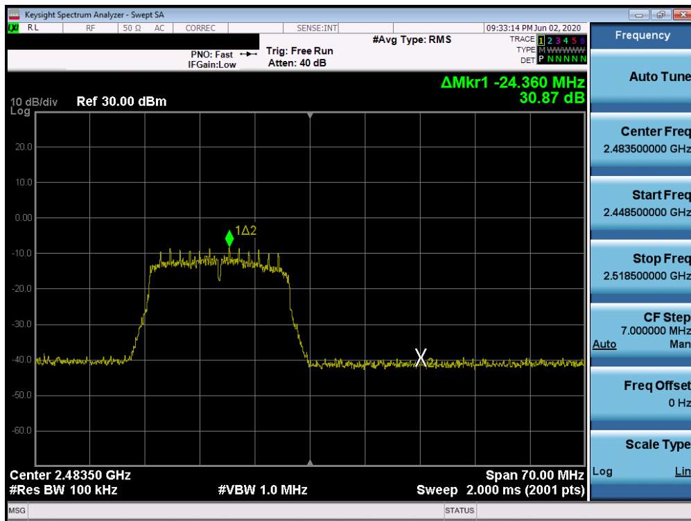
Plot 7-80. Band Edge Plot SISO CORE 1 (802.11n (2.4GHz) – Ch. 13)
