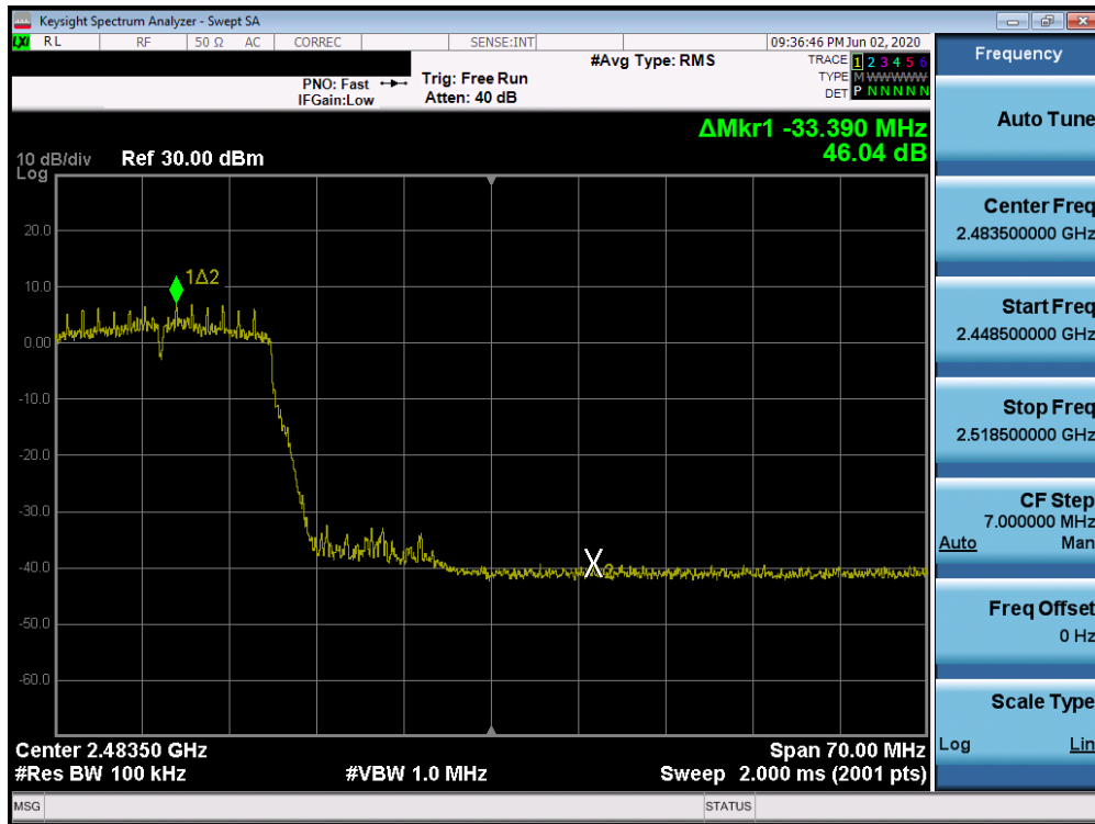
Plot 7-77. Band Edge Plot SISO CORE 1 (802.11n) (2.4GHz) - Ch. 10
