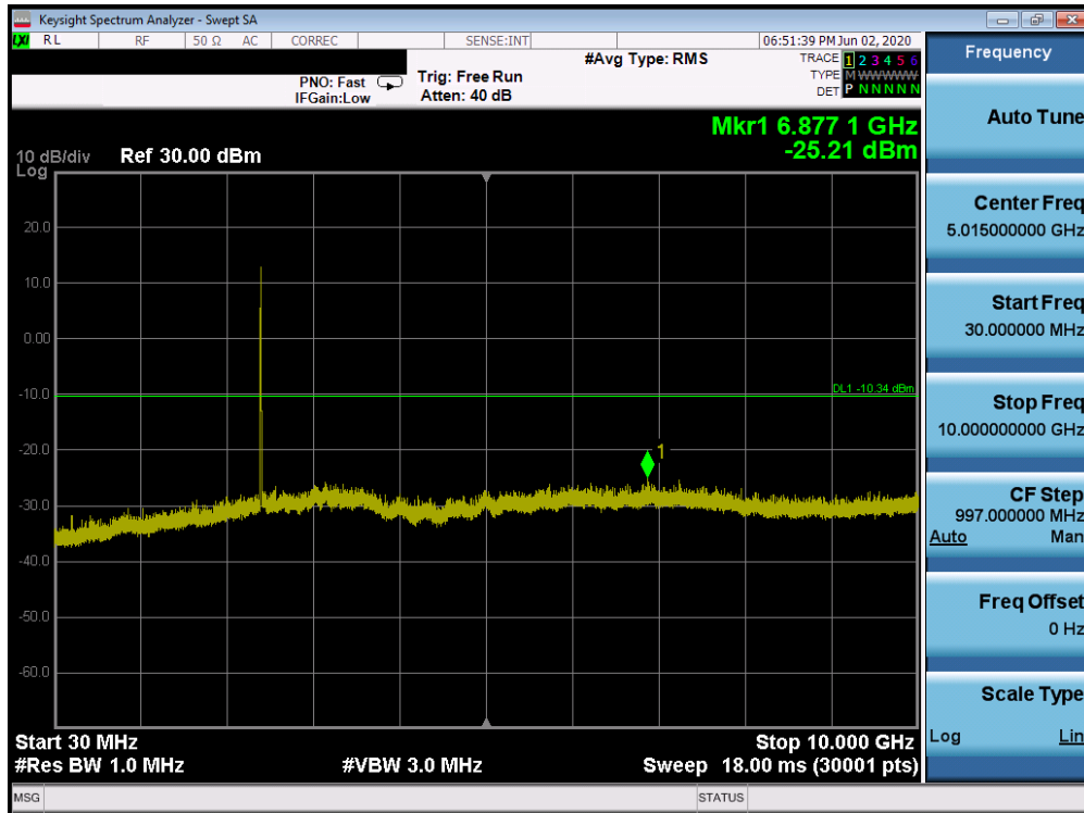
Plot 7-81. Conducted Spurious Plot SISO CORE 0 (802.11b – Ch. 1)
