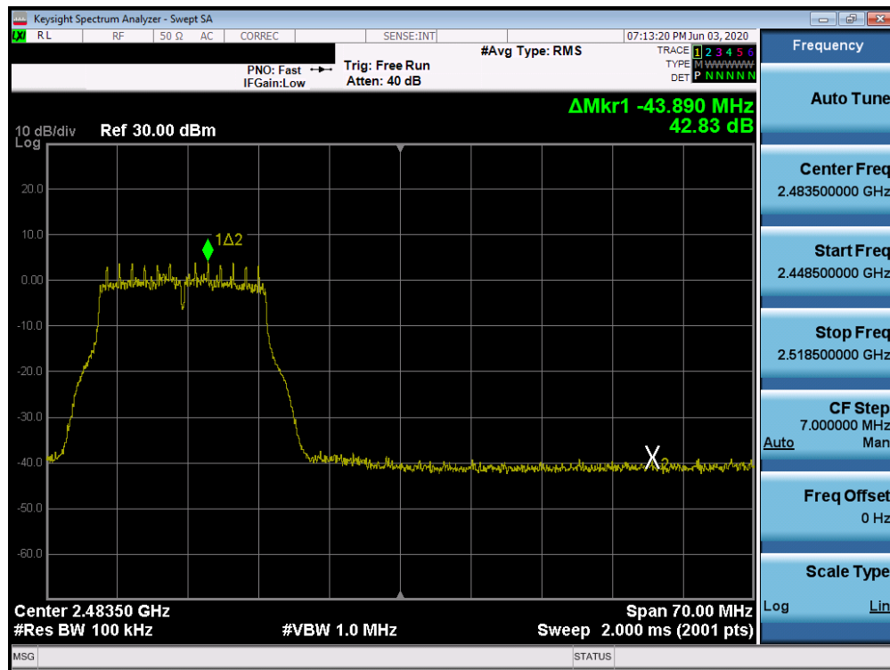
Plot 7-56. Band Edge Plot SISO CORE 0 (802.11g – Ch. 11)
