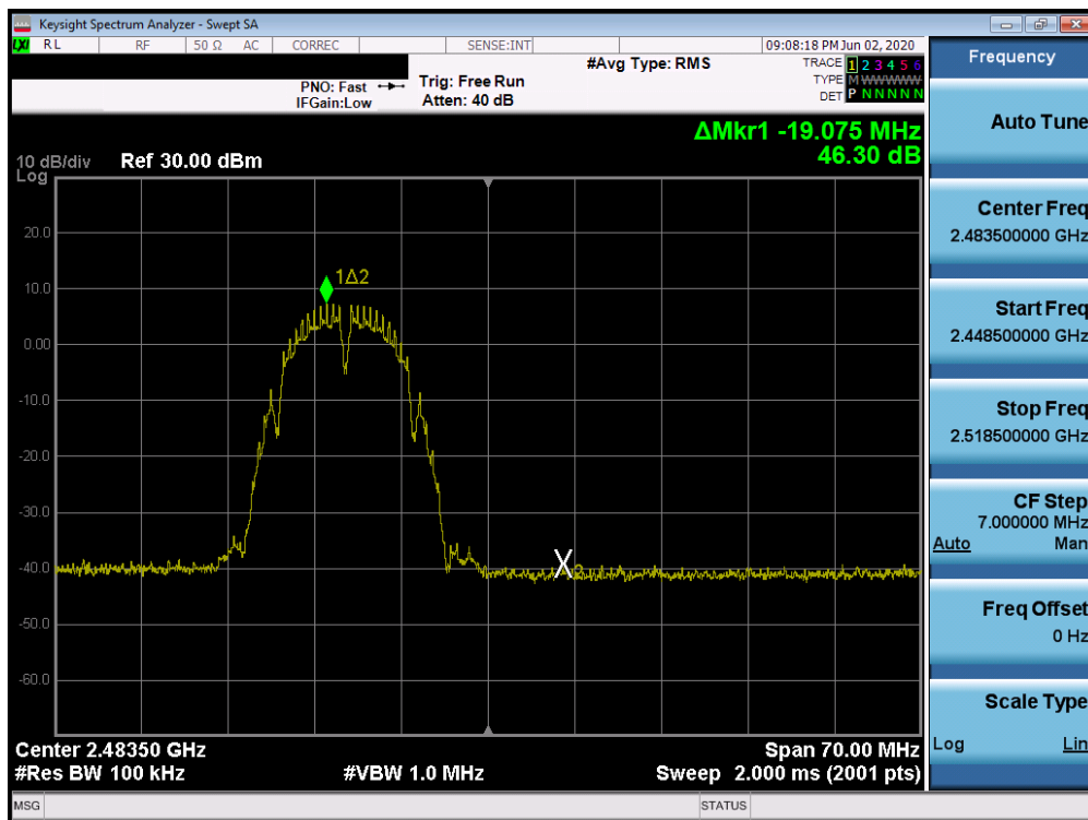
Plot 7-68. Band Edge Plot SISO CORE 1 (802.11b – Ch. 13)
