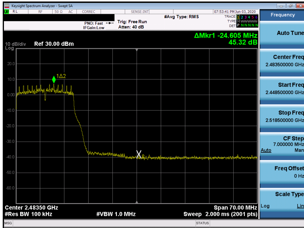
Plot 7-71. Band Edge Plot SISO CORE 1 (802.11g – Ch. 10)
