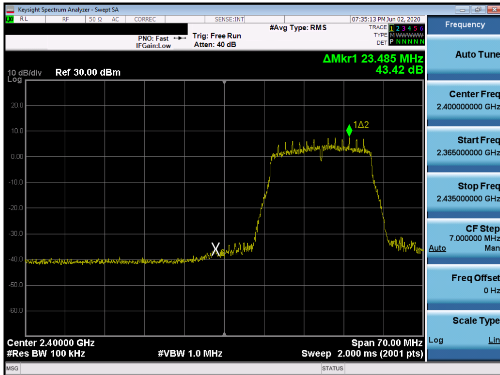
Plot 7-60. Band Edge Plot SISO CORE 0 (802.11n (2.4GHz) – Ch. 2)
