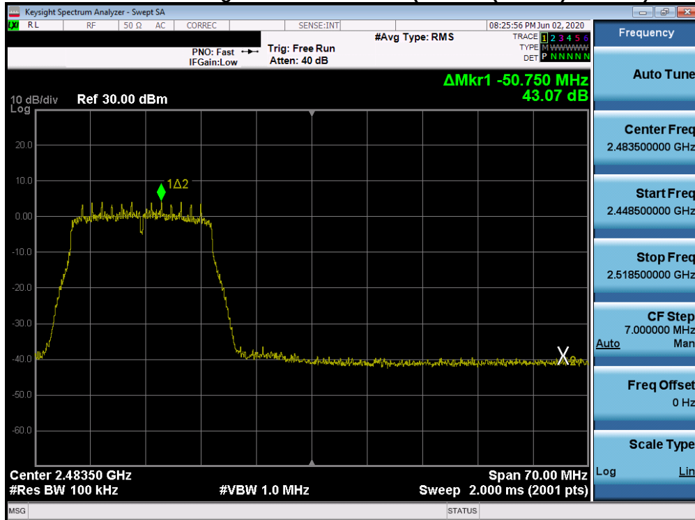
Plot 7-62. Band Edge Plot SISO CORE 0 (802.11n (2.4GHz) – Ch. 11)
