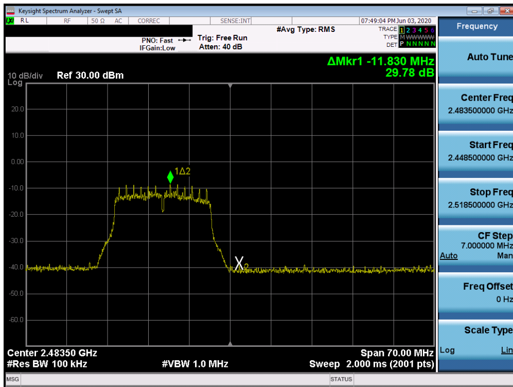
Plot 7-74. Band Edge Plot SISO CORE 1 (802.11g – Ch. 13)
