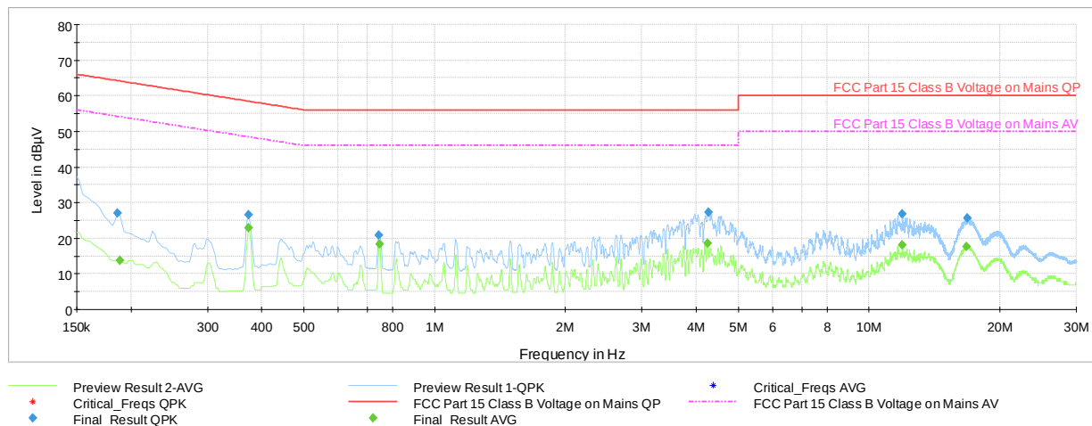
Plot 7-129. Line Conducted Plot with 802.11n Ch.6 (L1, with Laptop)
