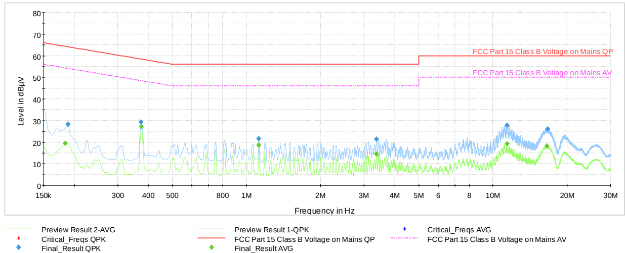
Plot 7-130. Line Conducted Plot with 802.11n Ch.6 (N, with Laptop)
