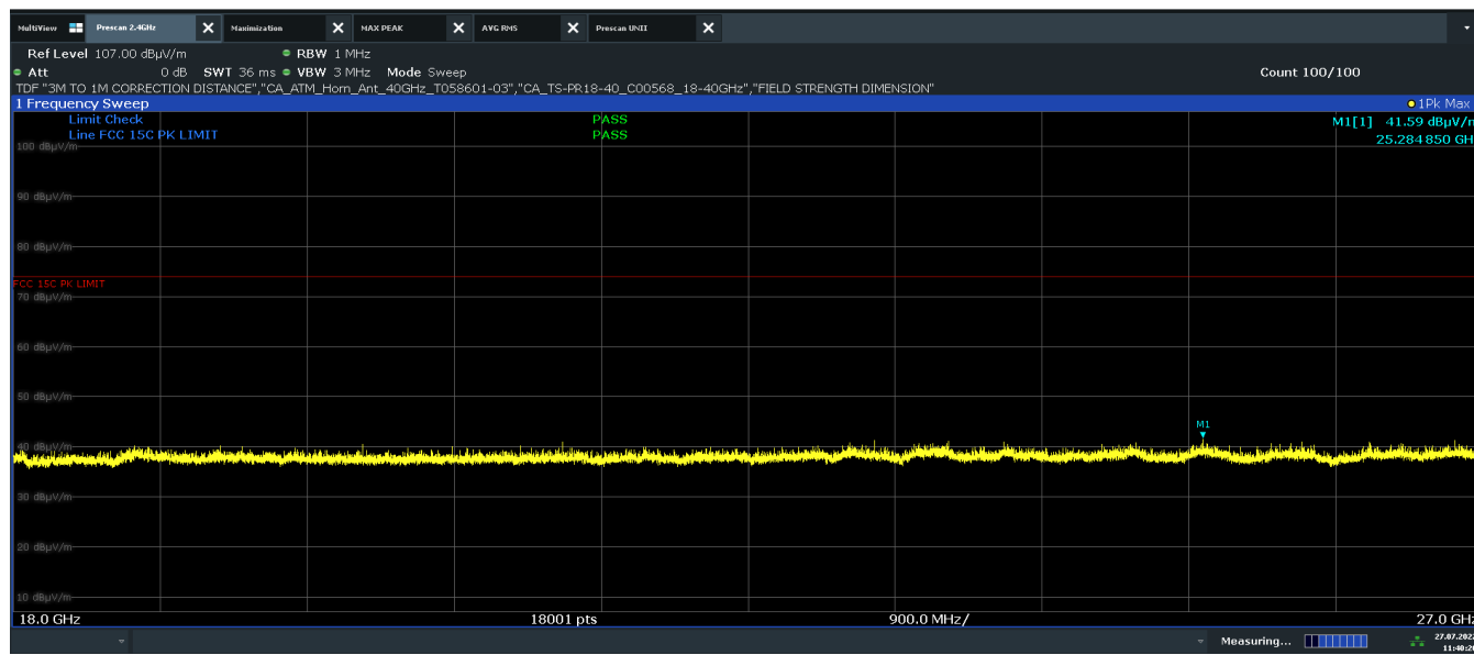
Plot 7-454. Radiated Spurious Emissions above 18GHz CDD (802.11n – Ch.6, Pol V)
