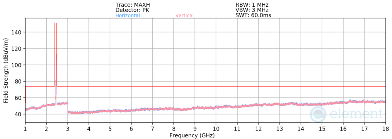
Plot 7-444. Radiated Spurious Emissions above 1GHz Antenna 4a (802.11ax(SU) – Ch. 11)
