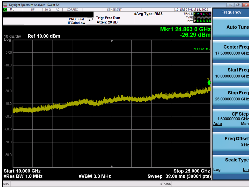
Plot 7-430. Conducted Spurious Plot Antenna 4a (802.11b – Ch. 6)
