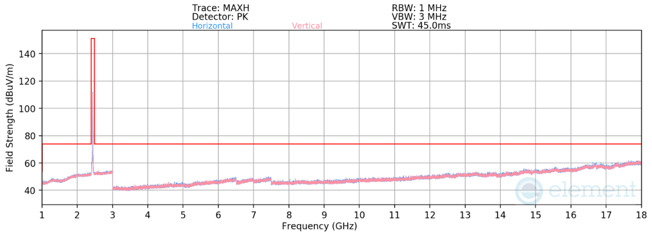
Plot 7-440. Radiated Spurious Emissions above 1GHz Antenna 4a (802.11b – Ch. 6)
