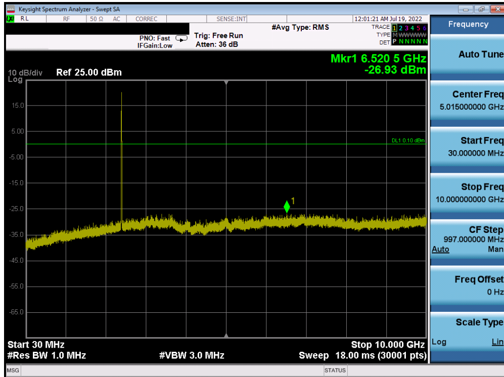
Plot 7-433. Conducted Spurious Plot Antenna 2a (802.11b – Ch. 1)
