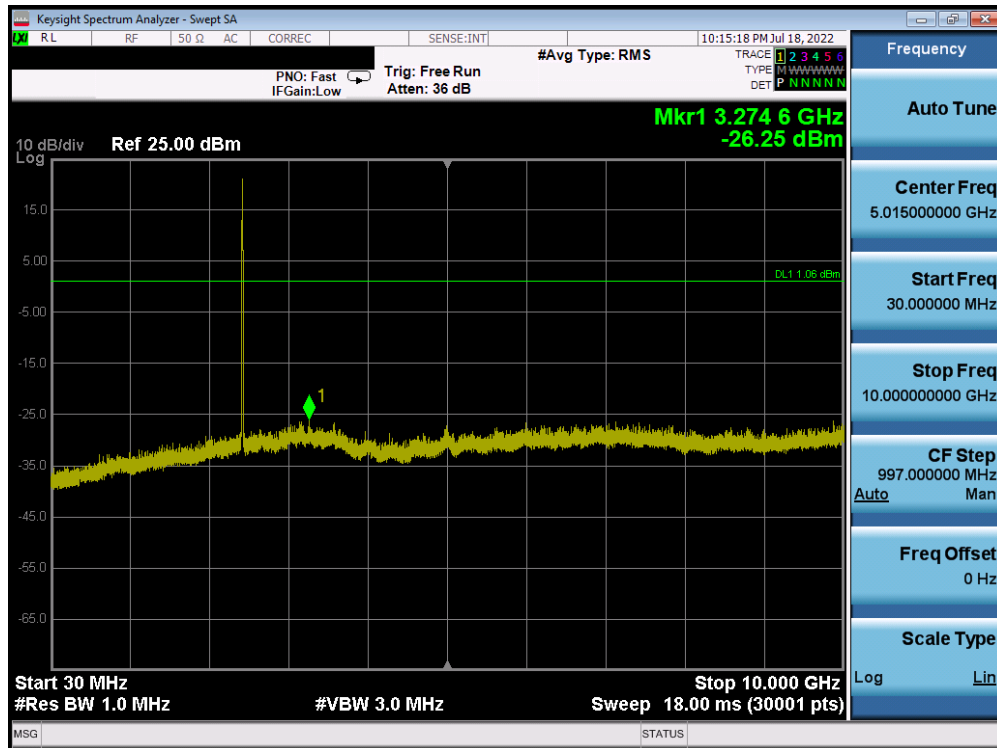
Plot 7-429. Conducted Spurious Plot Antenna 4a (802.11b – Ch. 6)
