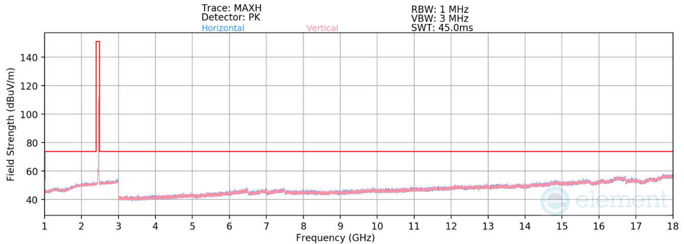
Plot 7-441. Radiated Spurious Emissions above 1GHz Antenna 4a (802.11b – Ch. 11)
