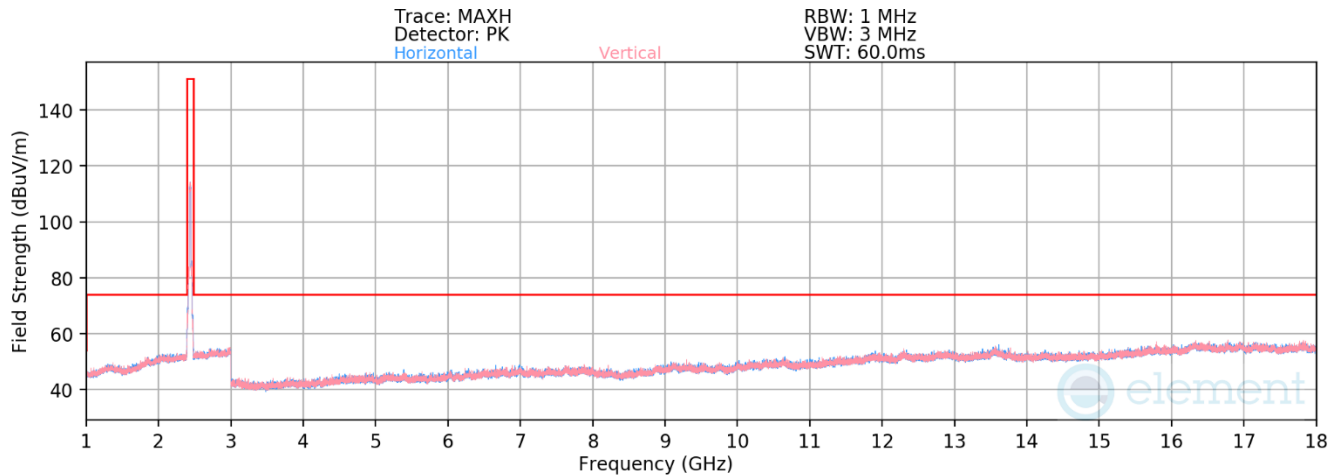
Plot 7-443. Radiated Spurious Emissions above 1GHz Antenna 4a (802.11ax(SU) – Ch. 6)
