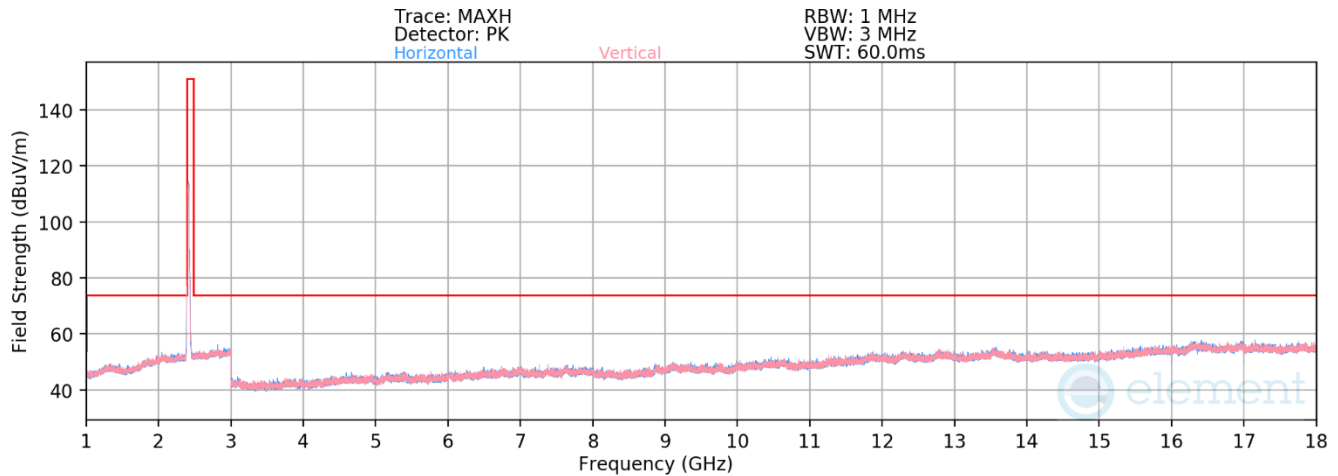
Plot 7-448. Radiated Spurious Emissions above 1GHz Antenna 2a (802.11ax(SU) – Ch. 1)
