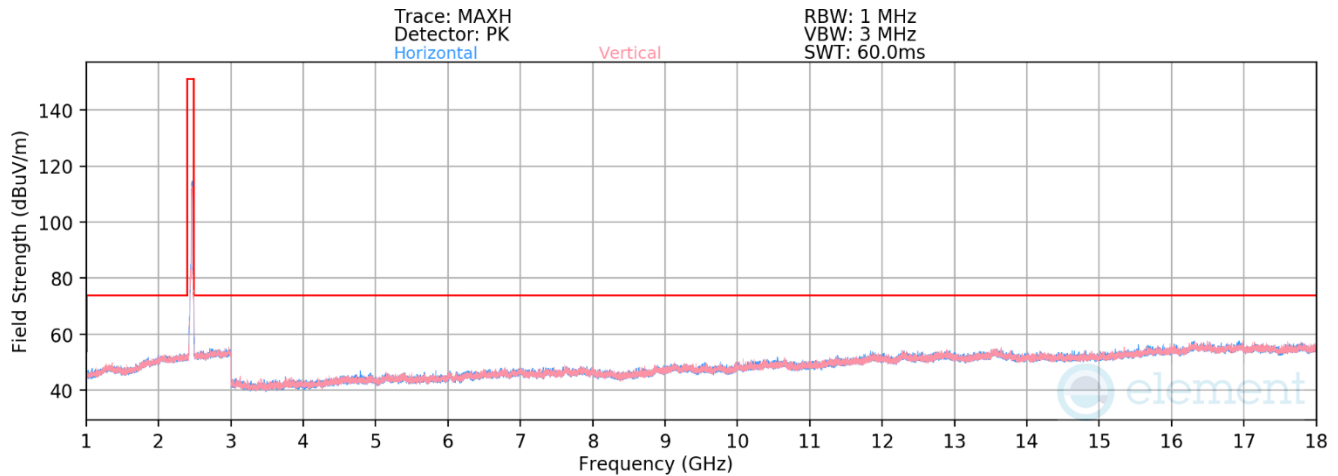
Plot 7-450. Radiated Spurious Emissions above 1GHz Antenna 2a (802.11ax(SU) – Ch. 11)
