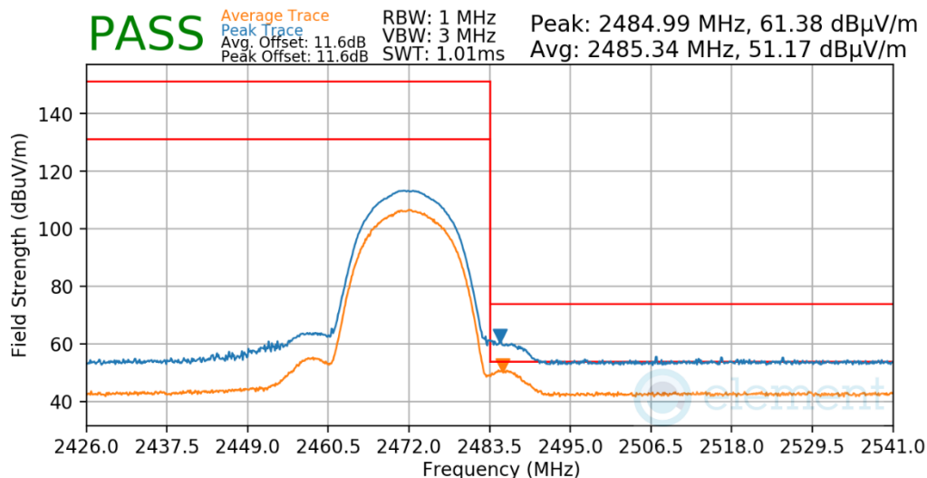
Plot 7-466. Radiated Restricted Upper Band Edge Measurement Antenna 4a
