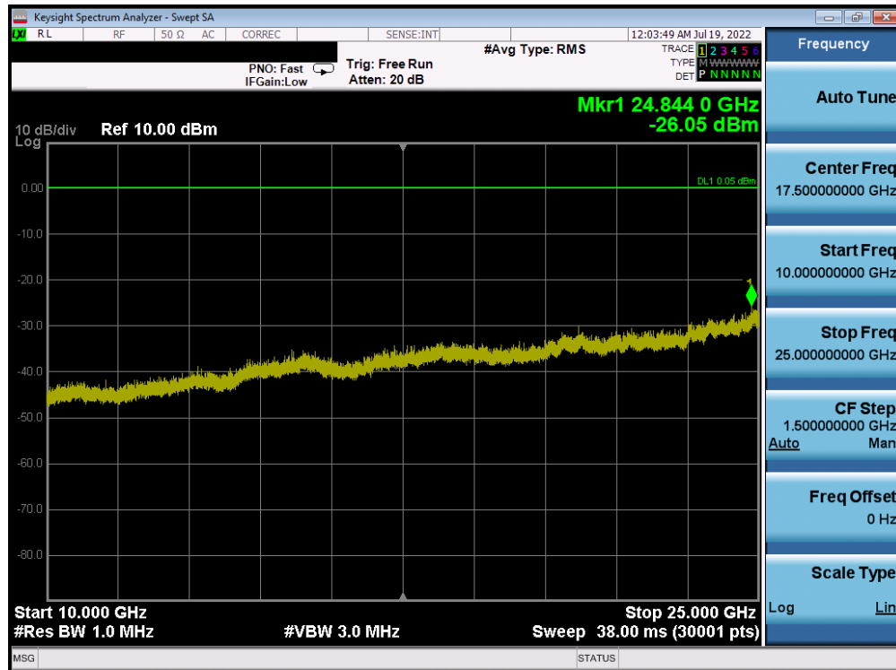
Plot 7-436. Conducted Spurious Plot Antenna 2a (802.11b – Ch. 6)
