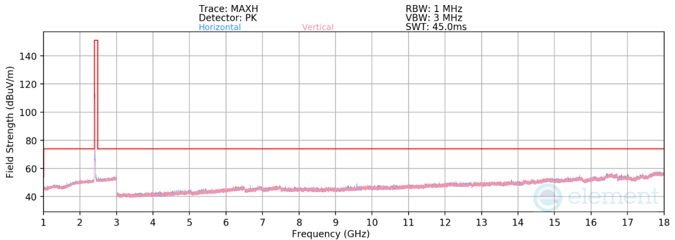
Plot 7-445. Radiated Spurious Emissions above 1GHz Antenna 2a (802.11b – Ch. 1)
