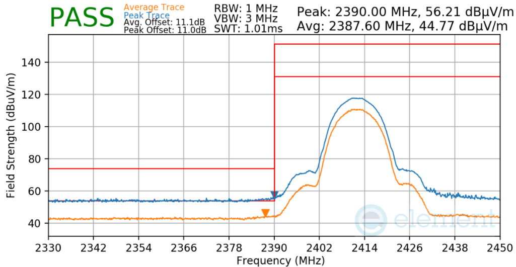
Plot 7-461. Radiated Restricted Lower Band Edge Measurement Antenna 4a
