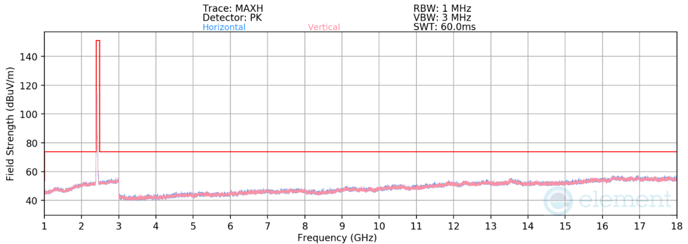
Plot 7-442. Radiated Spurious Emissions above 1GHz Antenna 4a (802.11ax(SU) – Ch. 1)
