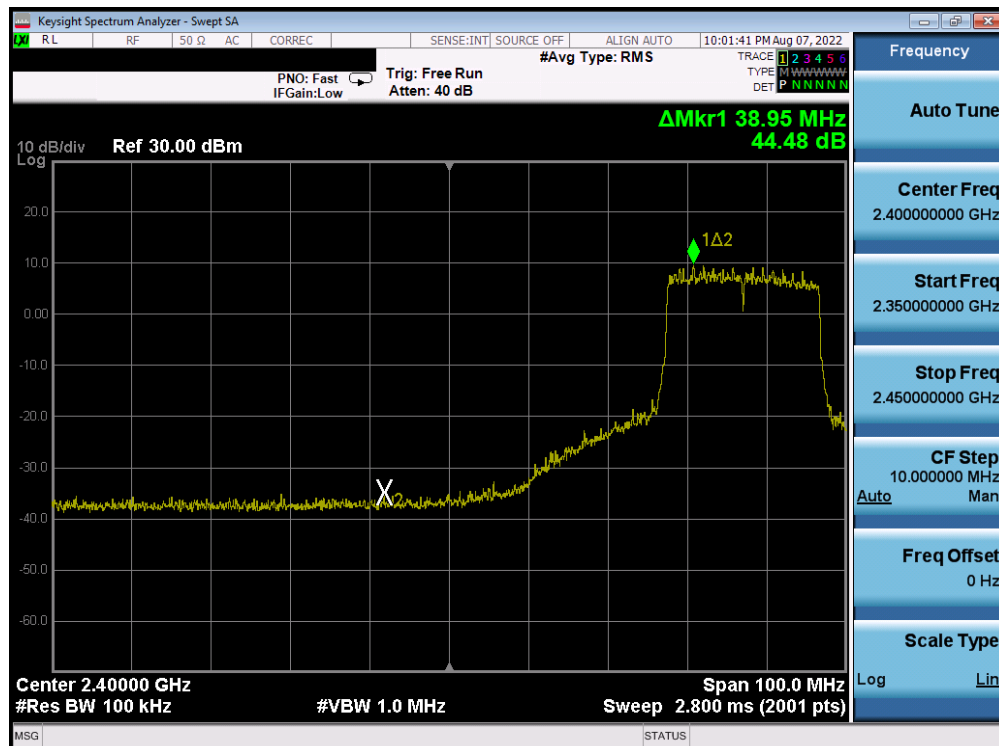
Plot 7-419. Band Edge Plot Antenna 2a (802.11ax (2.4GHz) – Ch. 6 (low)) – MCS5
