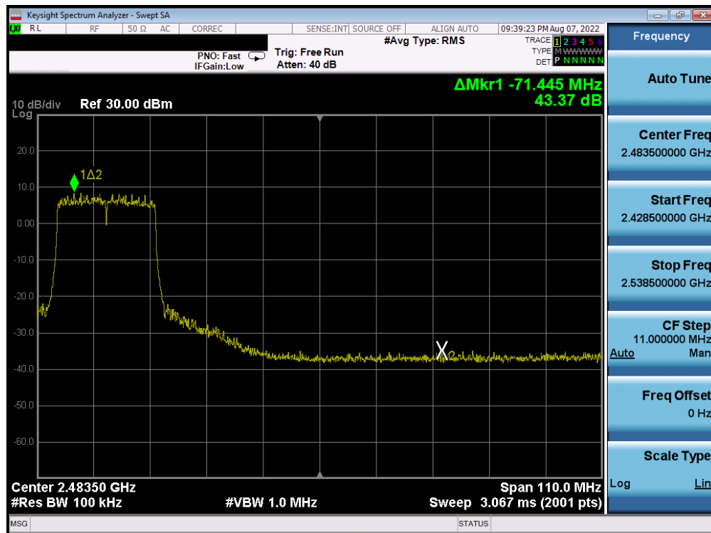
Plot 7-421. Band Edge Plot Antenna 2a (802.11ax (2.4GHz) – Ch. 7) – MCS5
