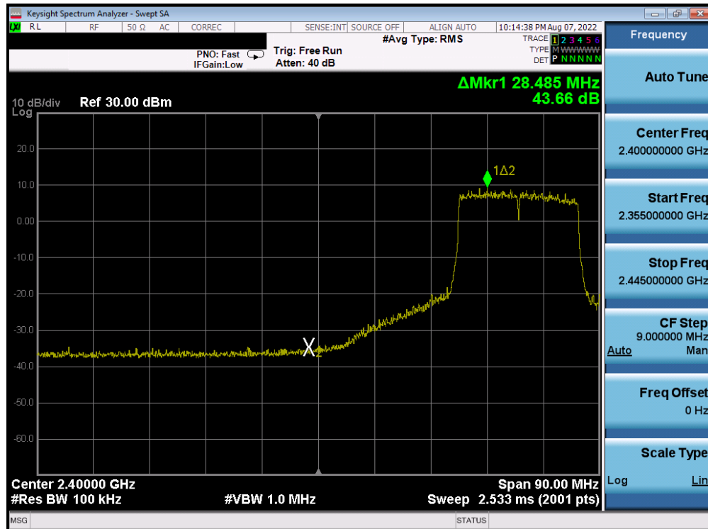
Plot 7-418. Band Edge Plot Antenna 2a (802.11ax (2.4GHz) – Ch. 5) – MCS5
