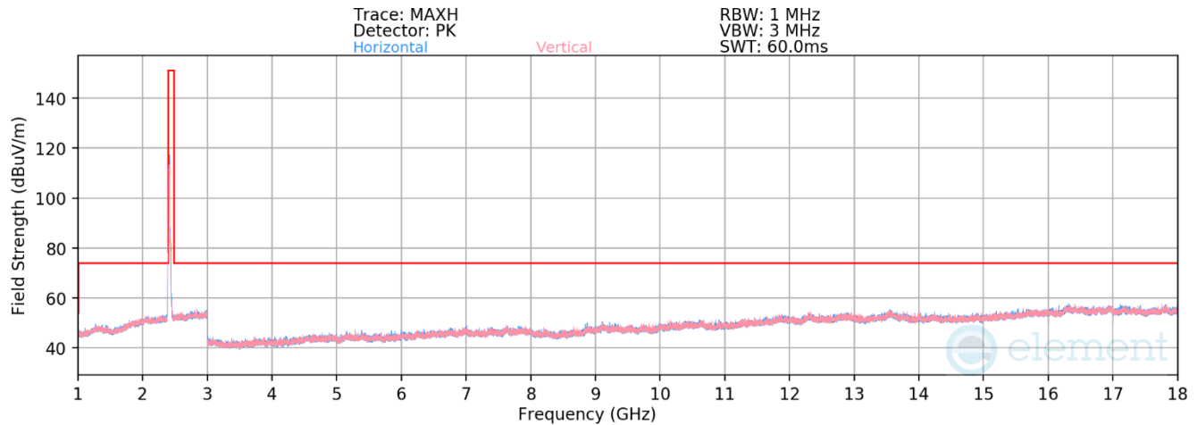
Plot 7-456. Radiated Spurious Emissions above 1GHz CDD (802.11ax (SU) – Ch. 1)
