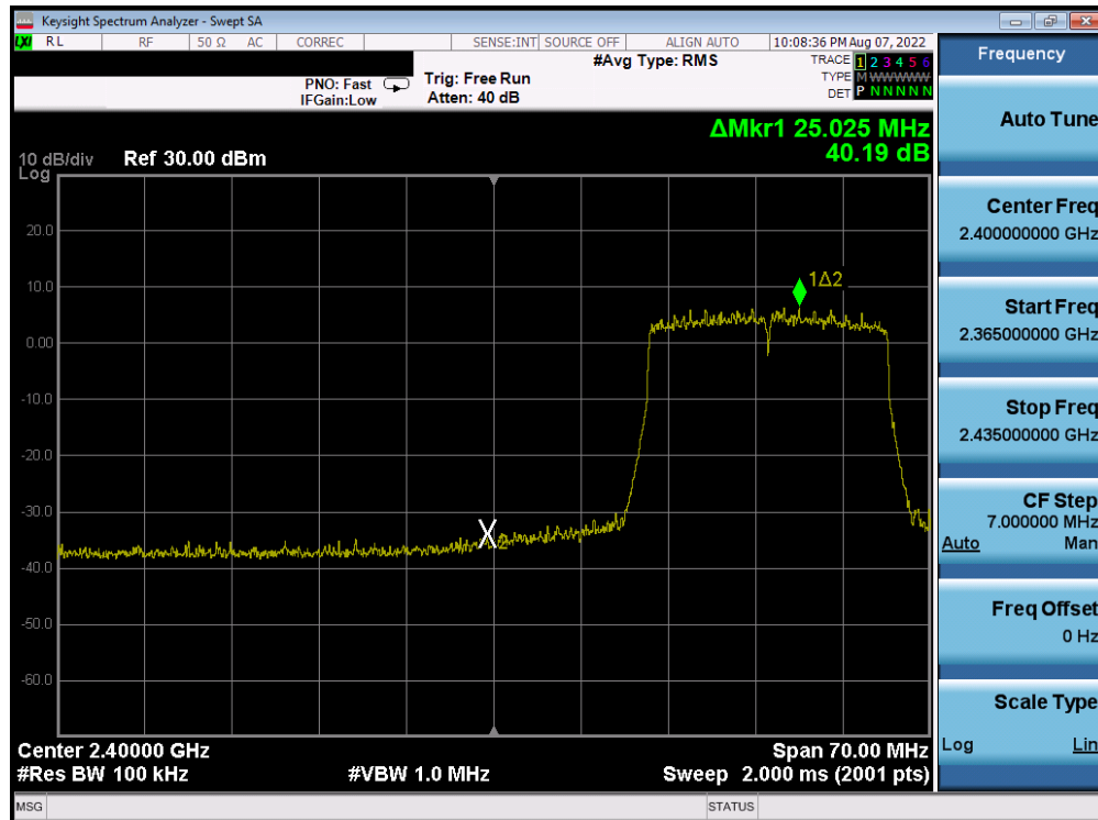
Plot 7-416. Band Edge Plot Antenna 2a (802.11ax (SU - 2.4GHz) – Ch. 3) – MCS5
