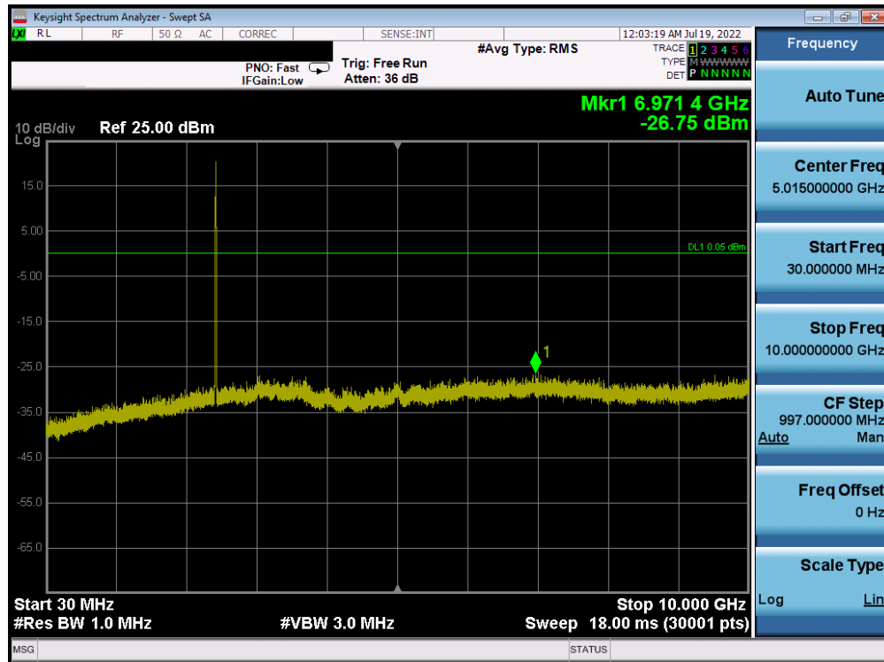
Plot 7-435. Conducted Spurious Plot Antenna 2a (802.11b – Ch. 6)
