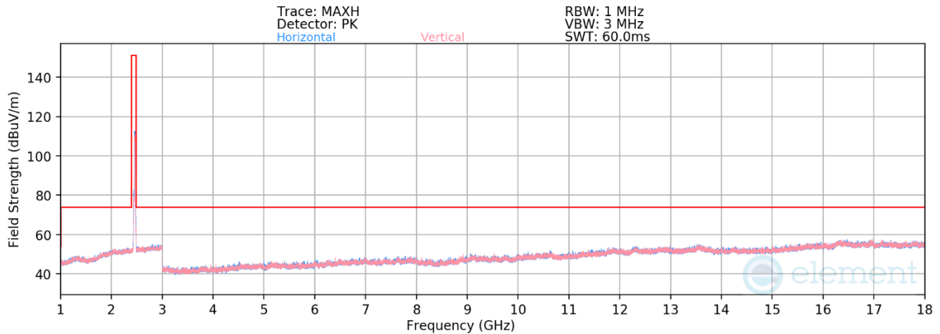
Plot 7-455. Radiated Spurious Emissions above 1GHz CDD (802.11n – Ch. 11)
