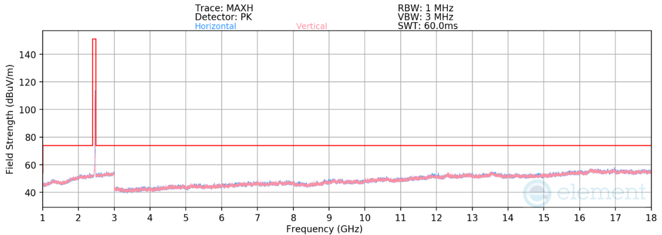
Plot 7-447. Radiated Spurious Emissions above 1GHz Antenna 2a (802.11b – Ch. 11)
