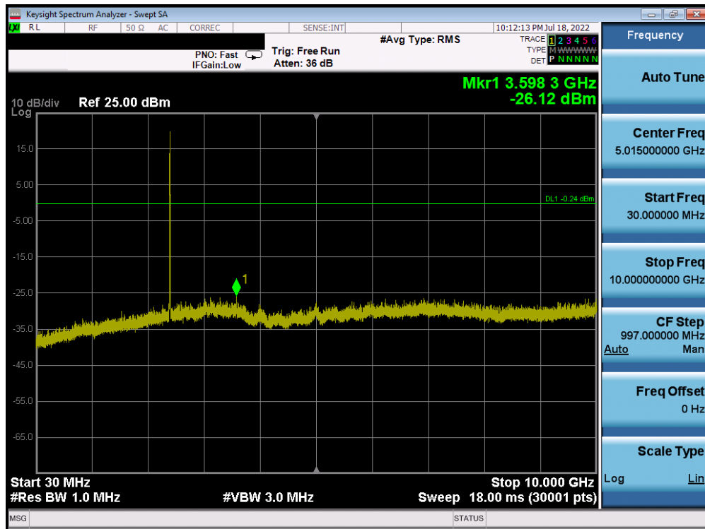
Plot 7-427. Conducted Spurious Plot Antenna 4a (802.11b – Ch. 1)
