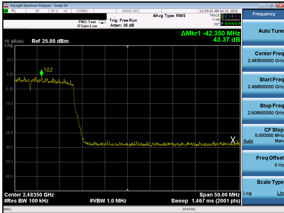
Plot 7-425. Band Edge Plot Antenna 2a (802.11ax (SU - 2.4GHz) – Ch. 11) – MCS5
