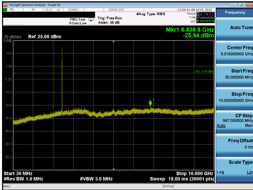
Plot 7-437. Conducted Spurious Plot Antenna 2a (802.11b – Ch. 11)
