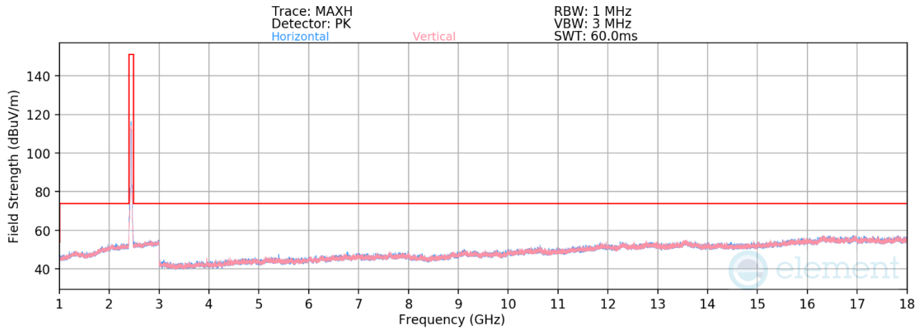
Plot 7-449. Radiated Spurious Emissions above 1GHz Antenna 2a (802.11ax(SU) – Ch. 6)
