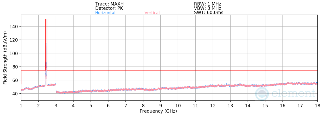
Plot 7-457. Radiated Spurious Emissions above 1GHz CDD (802.11ax (SU) – Ch. 6)
