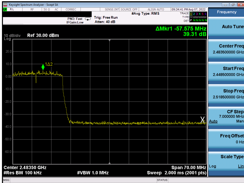
Plot 7-424. Band Edge Plot Antenna 2a (802.11ax (SU - 2.4GHz) – Ch. 10) – MCS5
