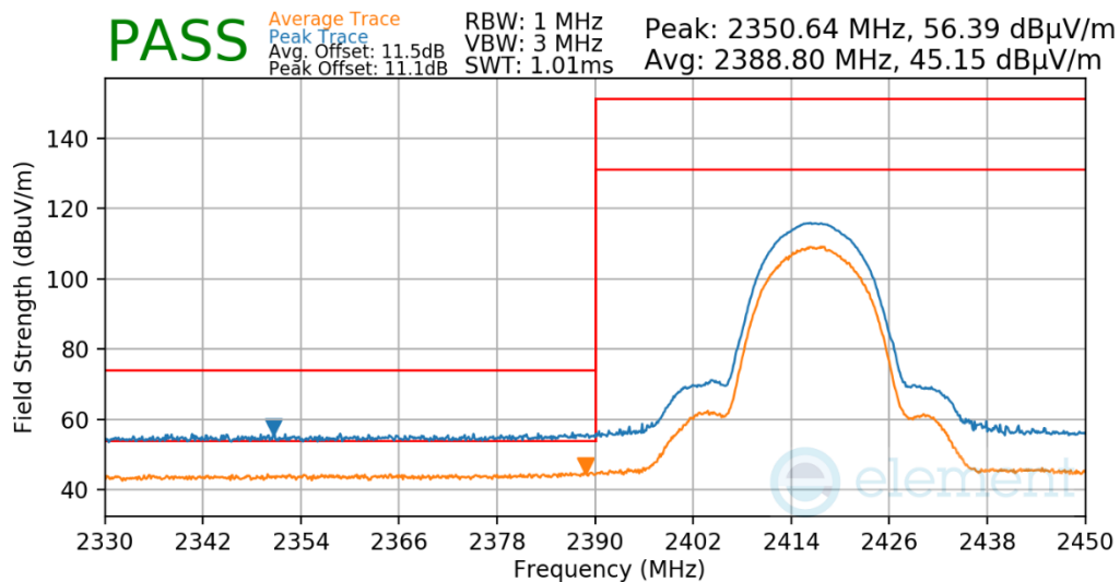
Plot 7-462. Radiated Restricted Lower Band Edge Measurement Antenna 4a
