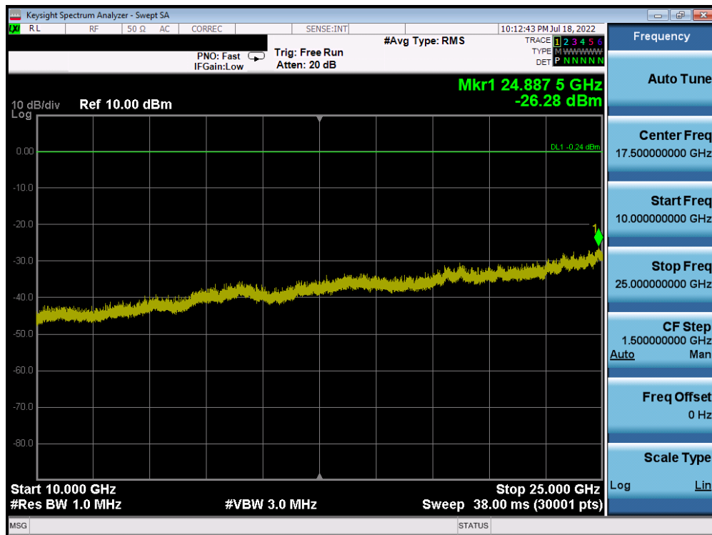
Plot 7-428. Conducted Spurious Plot Antenna 4a (802.11b – Ch. 1)
