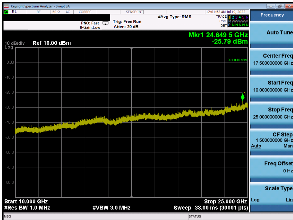
Plot 7-434. Conducted Spurious Plot Antenna 2a (802.11b – Ch. 1)
