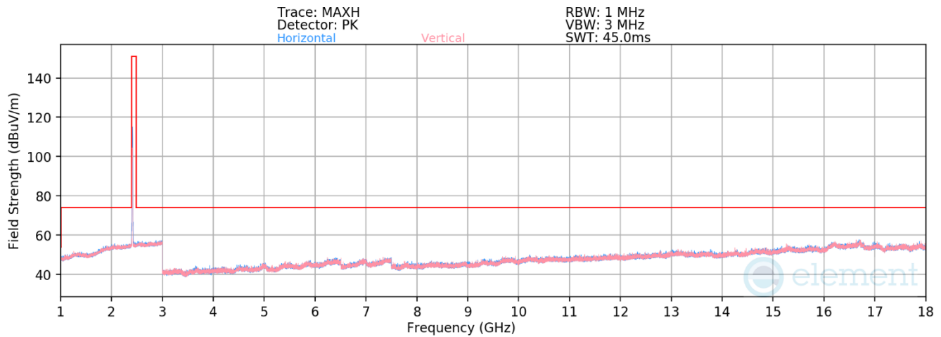
Plot 7-439. Radiated Spurious Emissions above 1GHz Antenna 4a (802.11b – Ch. 1)
