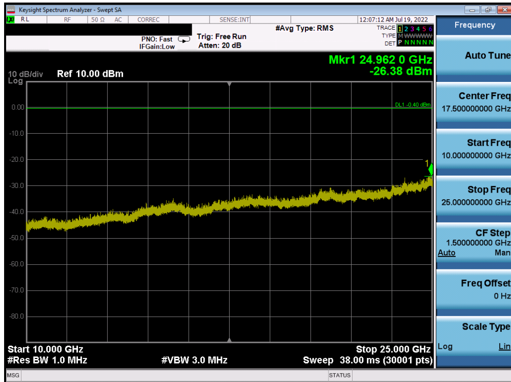
Plot 7-438. Conducted Spurious Plot Antenna 2a (802.11b – Ch. 11)
