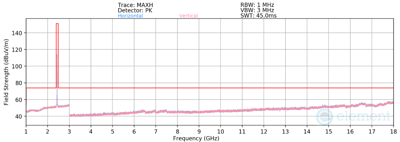
Plot 7-446. Radiated Spurious Emissions above 1GHz Antenna 2a (802.11b – Ch. 6)
