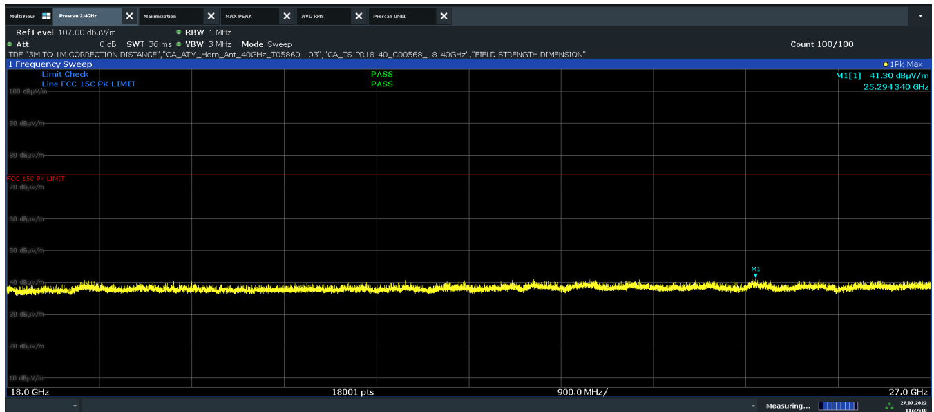
Plot 7-453. Radiated Spurious Emissions above 18GHz CDD (802.11n – Ch.6, Pol H)
