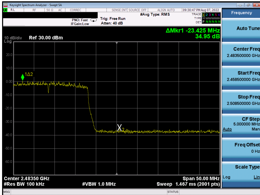
Plot 7-426. Band Edge Plot Antenna 2a (802.11ax (SU - 2.4GHz) – Ch. 12) – MCS5
