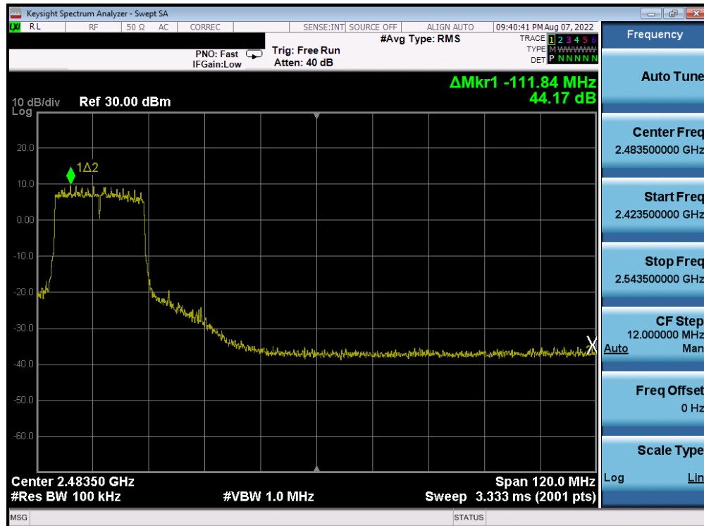
Plot 7-420. Band Edge Plot Antenna 2a (802.11ax (2.4GHz) – Ch. 6 (high)) – MCS5
