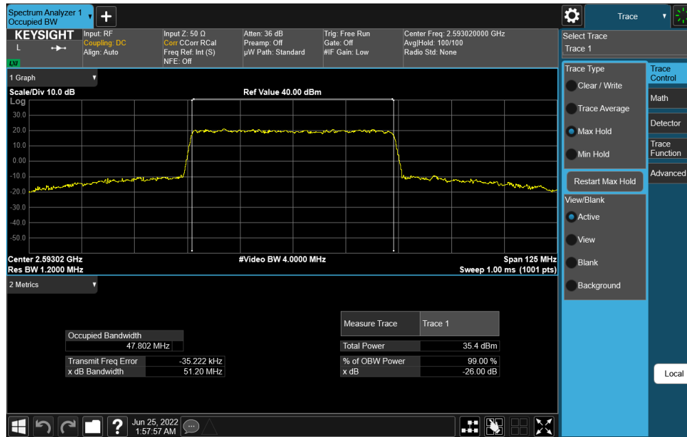
Plot 7-102. Occupied Bandwidth Plot (NR Band n41 - 50MHz CP-OFDM QPSK - Full RB)
