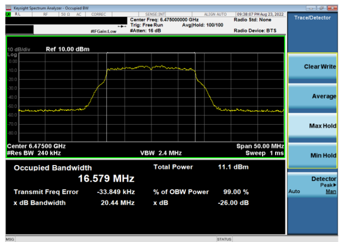
Plot 7-6. 26dB & 99% Bandwidth Plot Antenna 5b (20MHz 802.11a (UNII Band 6) – Ch. 105, 12Mbps)
