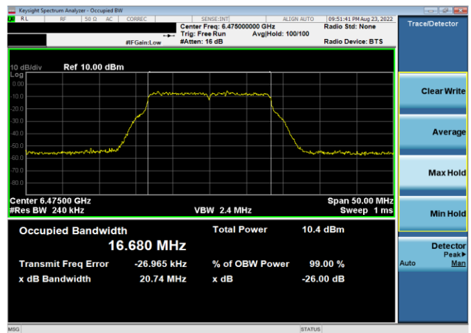
Plot 7-46. 26dB & 99% Bandwidth Plot Antenna 5b (20MHz 802.11a (UNII Band 6) – Ch. 105, 54Mbps)
