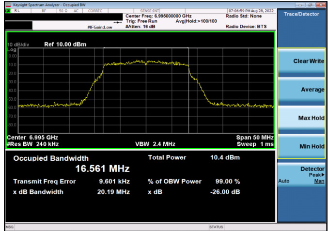
Plot 7-36. 26dB & 99% Bandwidth Plot Antenna 5b (20MHz 802.11a (UNII Band 8) – Ch. 209, 24Mbps)
