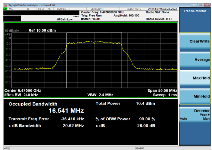
Plot 7-26. 26dB & 99% Bandwidth Plot Antenna 5b (20MHz 802.11a (UNII Band 6) – Ch. 105, 24Mbps)
