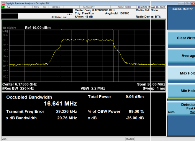
Plot 7-41. 26dB & 99% Bandwidth Plot Antenna 5b (20MHz 802.11a (UNII Band 5) – Ch. 45, 54Mbps)
