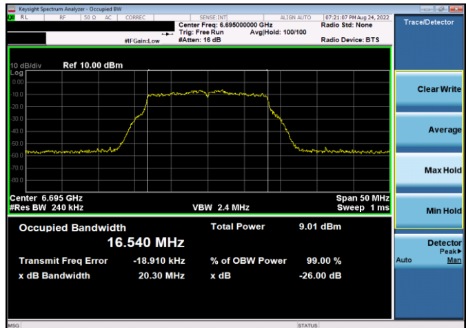
Plot 7-31. 26dB & 99% Bandwidth Plot Antenna 5b (20MHz 802.11a (UNII Band 7) – Ch. 149, 24Mbps)
