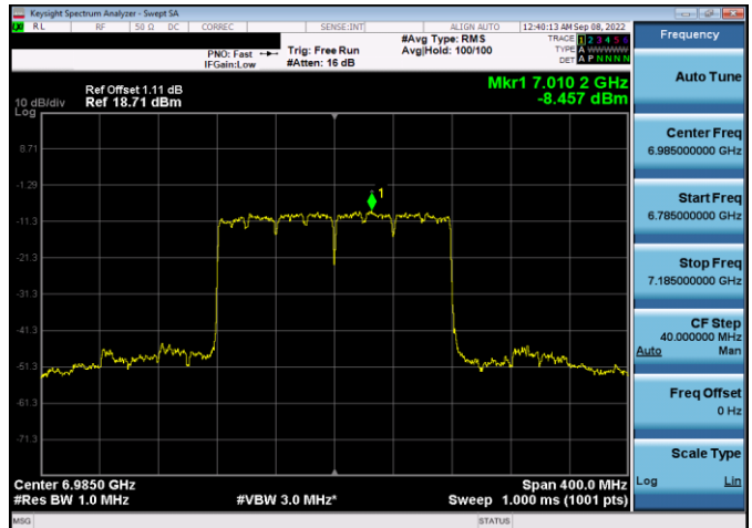
Plot 7-336. Power Spectral Density Plot SDM Antenna 4a (160MHz 802.11ax (UNII Band 8) – Ch. 207, MCS11)
