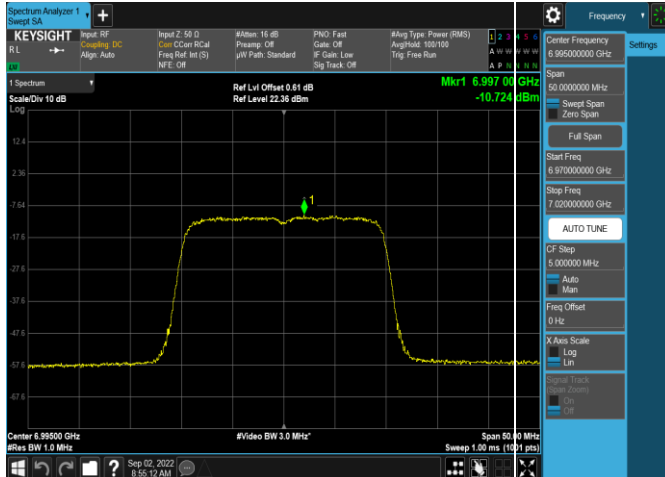
Plot 7-329. Power Spectral Density Plot SDM Antenna 5b (20MHz 802.11ax (UNII Band 8) – Ch. 209, MCS11)
