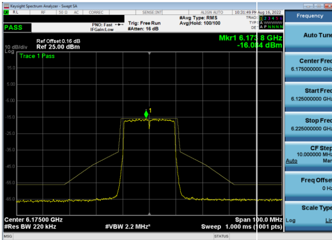
Plot 7-338. In-Band Emission Plot Antenna 5b (20MHz 802.11ax (UNII Band 5) – Ch. 45, MCS2)
