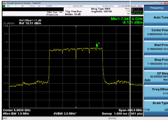
Plot 7-335. Power Spectral Density Plot SDM Antenna 5b (160MHz 802.11ax (UNII Band 8) – Ch. 207, MCS11)
