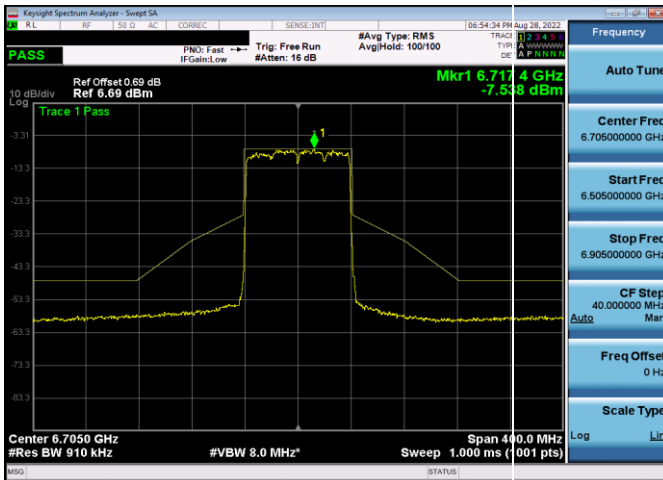
Plot 7-370. In-Band Emission Plot Antenna 5b (80MHz 802.11ax (UNII Band 7) – Ch. 151, MCS4)
