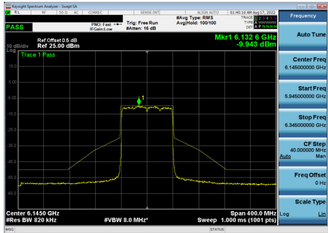
Plot 7-340. In-Band Emission Plot Antenna 5b (80MHz 802.11ax (UNII Band 5) – Ch. 39, MCS2)
