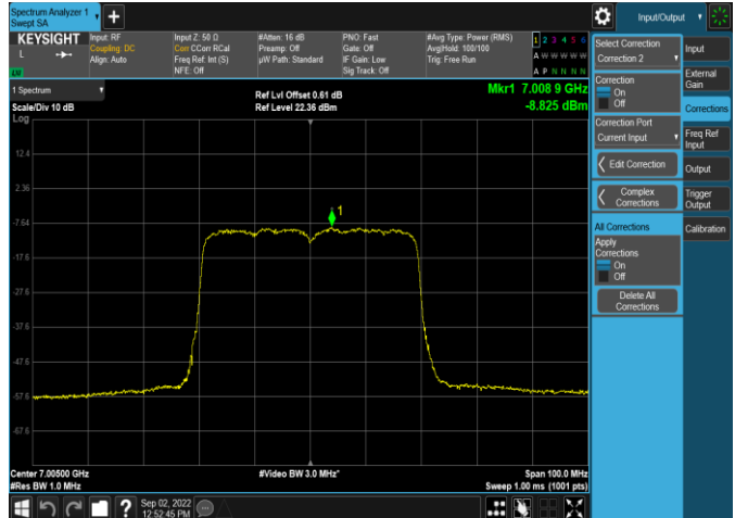
Plot 7-332. Power Spectral Density Plot SDM Antenna 4a (40MHz 802.11ax (UNII Band 8) – Ch. 211, MCS11)
