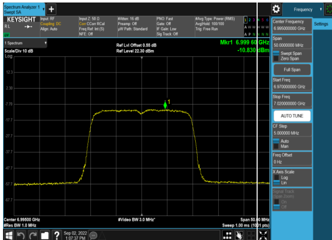
Plot 7-330. Power Spectral Density Plot SDM Antenna 4a (20MHz 802.11ax (UNII Band 8) – Ch. 209, MCS11)
