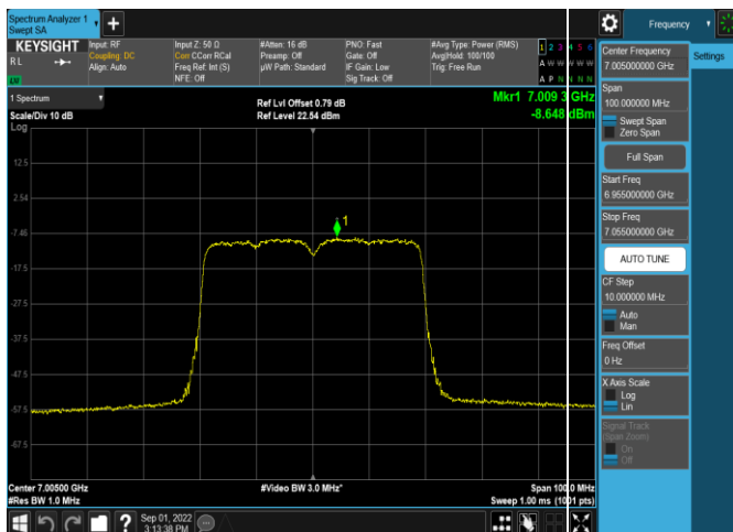
Plot 7-331. Power Spectral Density Plot SDM Antenna 5b (40MHz 802.11ax (UNII Band 8) – Ch. 211, MCS11)
