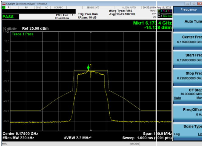
Plot 7-337. In-Band Emission Plot Antenna 5b (20MHz 802.11a (UNII Band 5) – Ch. 45, 12Mbps)
