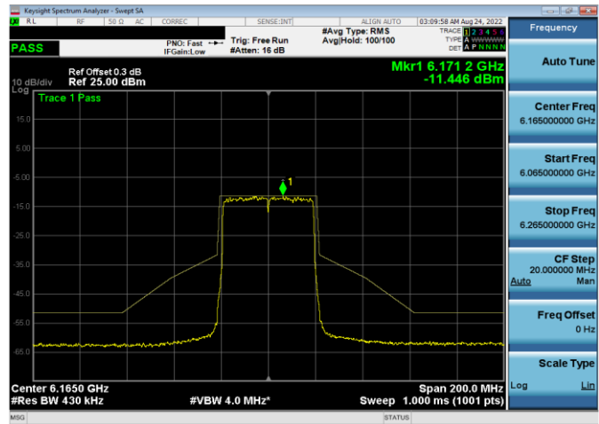
Plot 7-339. In-Band Emission Plot Antenna 5b (40MHz 802.11ax (UNII Band 5) – Ch. 43, MCS2)
