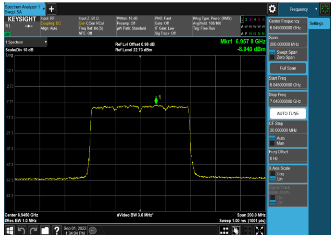
Plot 7-333. Power Spectral Density Plot SDM Antenna 5b (80MHz 802.11ax (UNII Band 8) – Ch. 199, MCS11)
