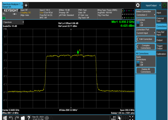
Plot 7-334. Power Spectral Density Plot SDM Antenna 4a (80MHz 802.11ax (UNII Band 8) – Ch. 199, MCS11)
