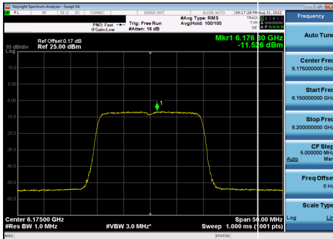
Plot 7-264. Power Spectral Density Plot SDM Antenna 5b (20MHz 802.11ax RU242 (UNII Band 5) – Ch. 45)
