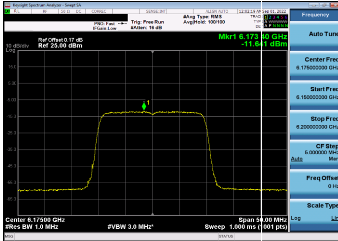
Plot 7-263. Power Spectral Density Plot SDM Antenna 4a (20MHz 802.11ax RU242 (UNII Band 5) – Ch. 45)
