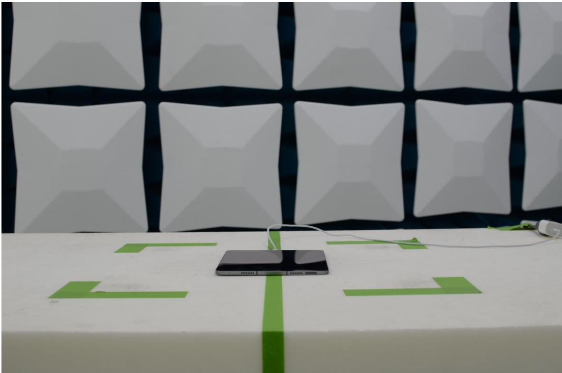
Figure 12: 30MHz-1GHz Test Setup (Front View)
