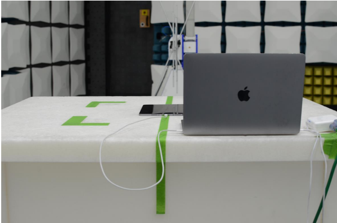
Figure 19: 30MHz-1GHz Test Setup (Rear View)
