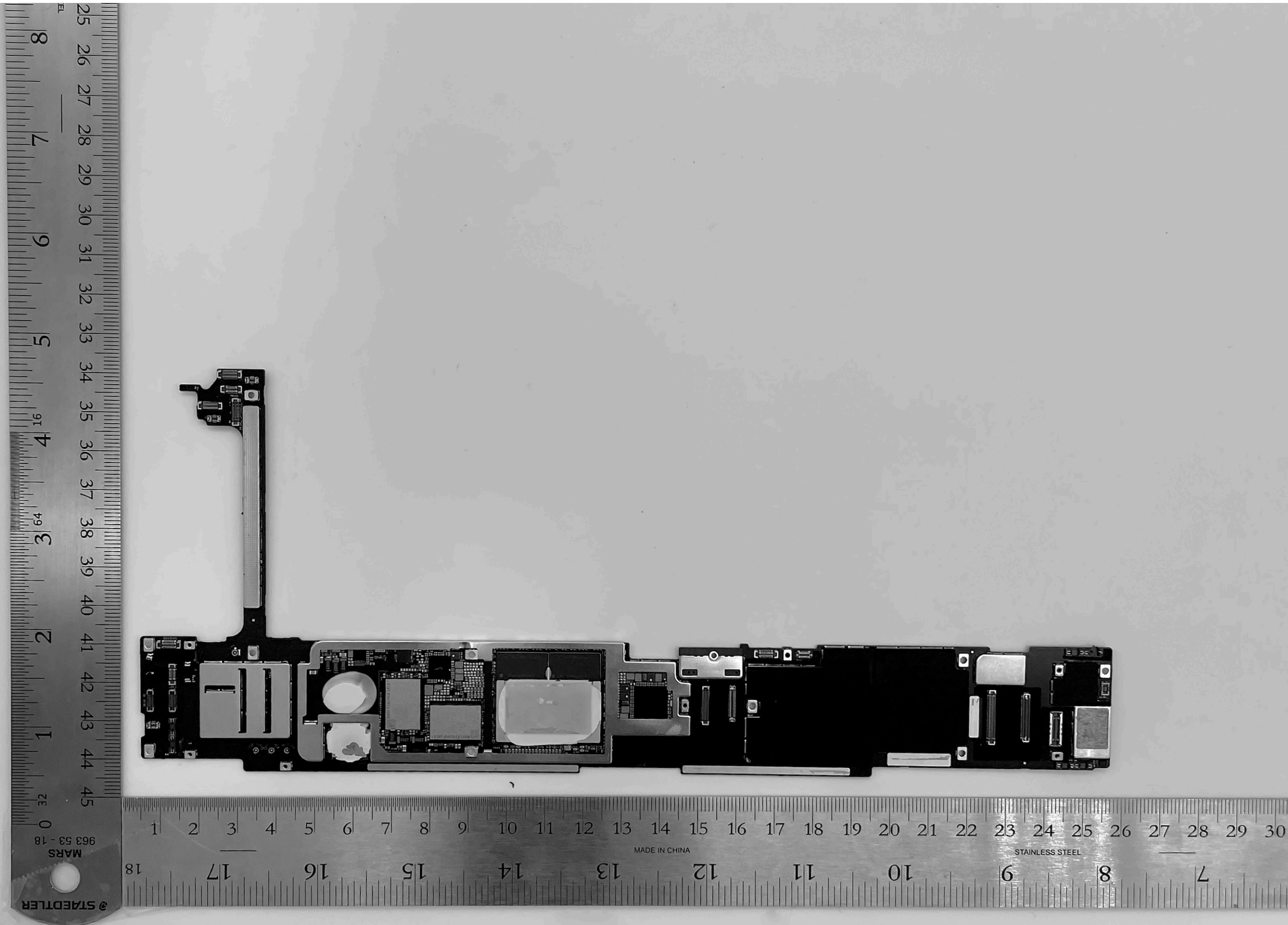
A2436 MLB with Shield - Front
