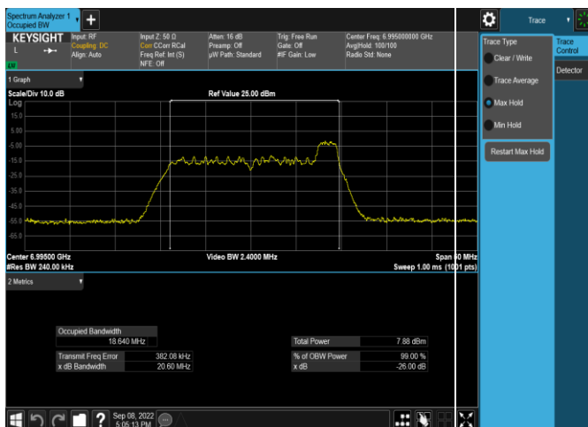
Plot 7-51. 26dB & 99% Bandwidth Plot Antenna WF5t (20MHz 802.11ax RU26 (UNII Band 8) - Ch. 209)
