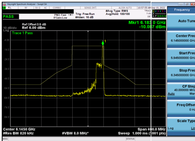
Plot 7-532. In-Band Emission Plot SDM Antenna WF5t (80MHz 802.11ax RU26 (UNII Band 5) – Ch. 39)
