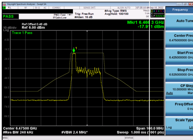
Plot 7-544. In-Band Emission Plot SDM Antenna WF5t (20MHz 802.11ax RU26 (UNII Band 6) – Ch. 105)
