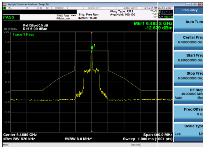
Plot 7-562. In-Band Emission Plot SDM Antenna WF5t (80MHz 802.11ax RU26 (UNII Band 6) – Ch. 103)
