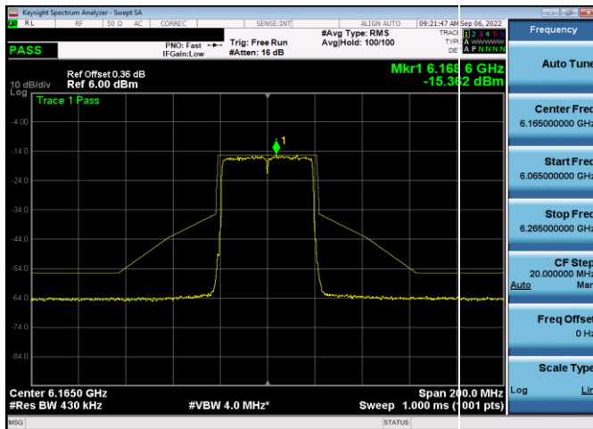
Plot 7-526. In-Band Emission Plot SDM Antenna WF5t (40MHz 802.11ax RU484 (UNII Band 5) – Ch. 43)
