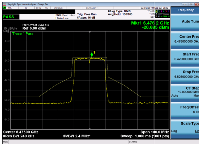
Plot 7-550. In-Band Emission Plot SDM Antenna WF5t (20MHz 802.11ax RU242 (UNII Band 6) – Ch. 105)
