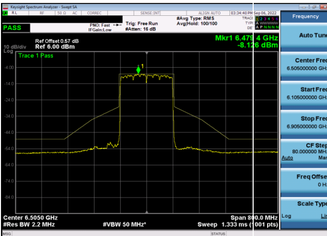
Plot 7-574. In-Band Emission Plot SDM Antenna WF5t (160MHz 802.11ax RU484 (UNII Band 6) – Ch. 111)
