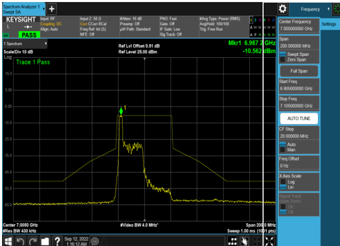
Plot 7-615. In-Band Emission Plot SDM Antenna WF5t (40MHz 802.11ax RU26 (UNII Band 8) - Ch. 211)
