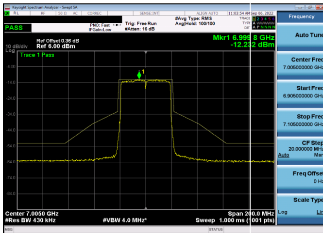
Plot 7-622. In-Band Emission Plot SDM Antenna WF5b (40MHz 802.11ax RU484 (UNII Band 8) - Ch. 211)
