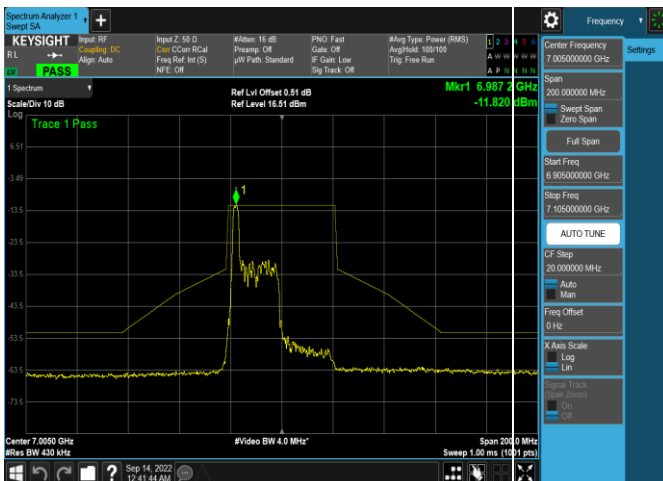
Plot 7-616. In-Band Emission Plot SDM Antenna WF5b (40MHz 802.11ax RU26 (UNII Band 8) - Ch. 211)
