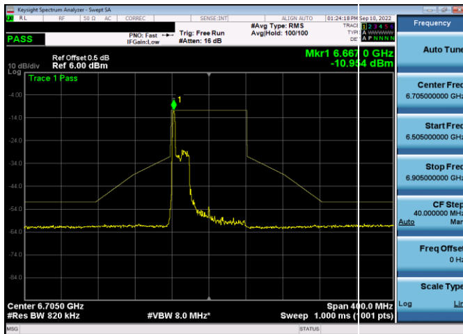
Plot 7-592. In-Band Emission Plot SDM Antenna WF5t (80MHz 802.11ax RU26 (UNII Band 7) – Ch. 151)
