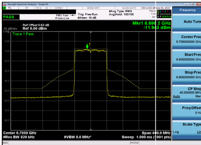
Plot 7-598. In-Band Emission Plot SDM Antenna WF5t (80MHz 802.11ax RU996 (UNII Band 7) – Ch. 151)
