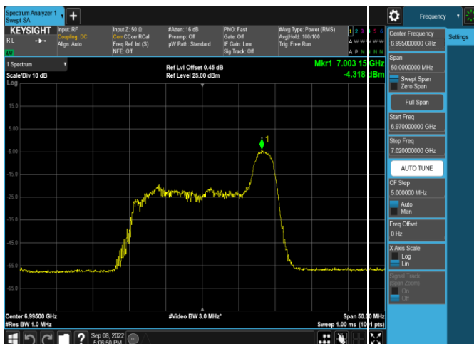
Plot 7-179. Power Spectral Density Plot Antenna WF5t (20MHz 802.11ax RU26 (UNII Band 8) – Ch. 209)
