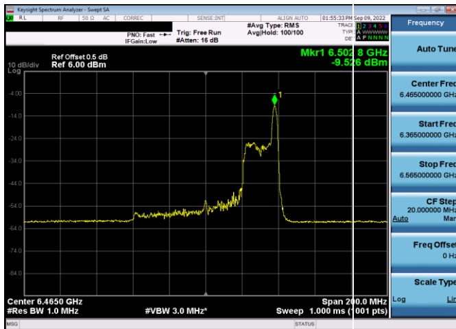
Plot 7-219. Power Spectral Density Plot Antenna WF5b (80MHz 802.11ax RU26 (UNII Band 6) – Ch. 103)
