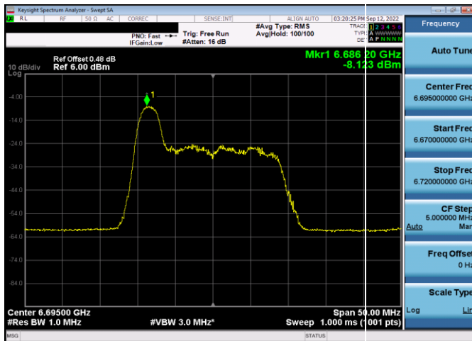
Plot 7-225. Power Spectral Density Plot Antenna WF5b (20MHz 802.11ax RU26 (UNII Band 7) – Ch. 149)
