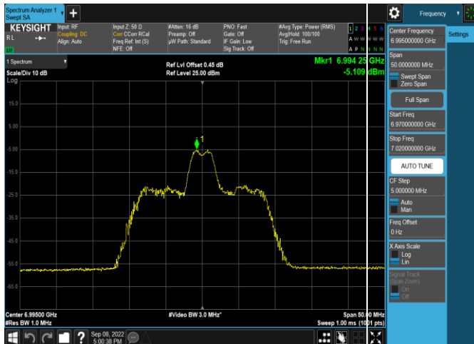
Plot 7-178. Power Spectral Density Plot Antenna WF5t (20MHz 802.11ax RU26 (UNII Band 8) – Ch. 209)
