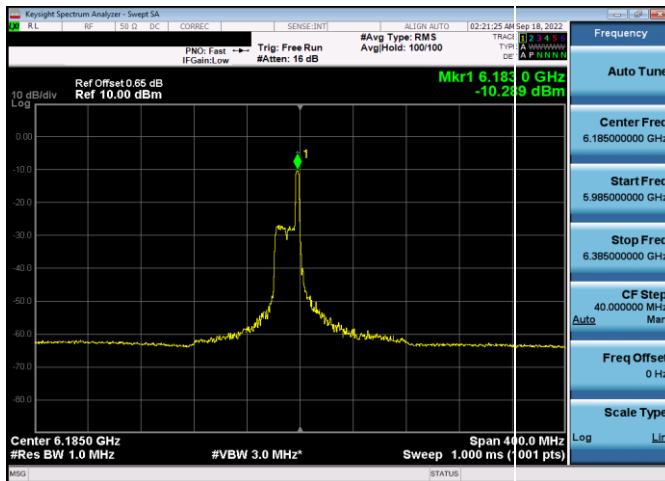
Plot 7-283. Power Spectral Density Plot SDM Antenna WF5t (160MHz 802.11ax RU26 (UNII Band 5) – Ch. 47)
