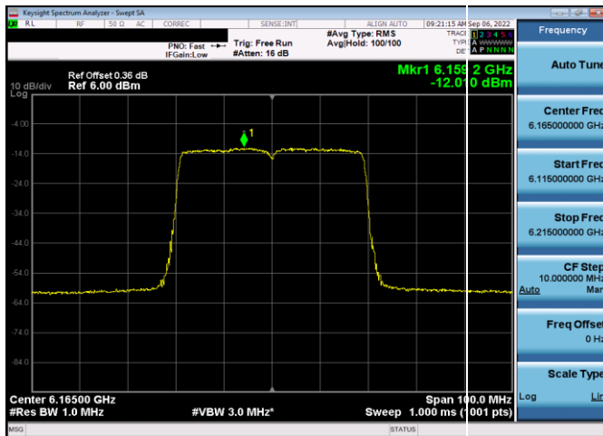
Plot 7-271. Power Spectral Density Plot SDM Antenna WF5t (40MHz 802.11ax RU484 (UNII Band 5) – Ch. 43)
