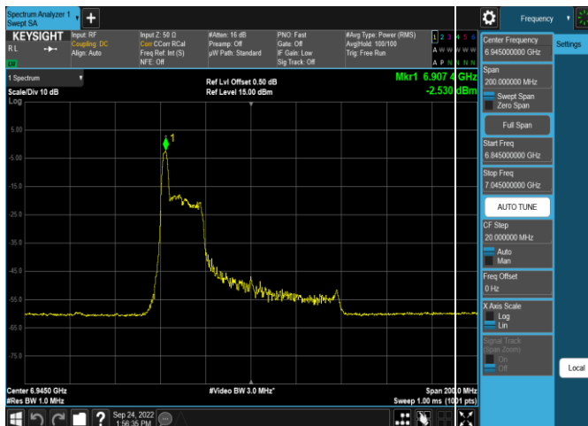
Plot 7-249. Power Spectral Density Plot Antenna WF5b (80MHz 802.11ax RU26 (UNII Band 8) – Ch. 199)
