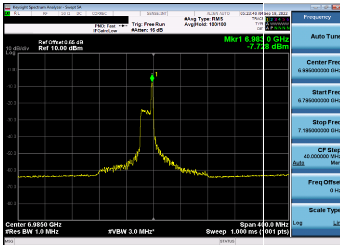
Plot 7-379. Power Spectral Density Plot SDM Antenna WF5b (160MHz 802.11ax RU26 (UNII Band 8) – Ch. 207)
