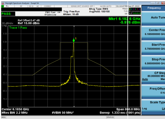
Plot 7-397. In-Band Emission Plot Antenna WF5t (160MHz 802.11ax RU26 (UNII Band 5) – Ch. 47)
