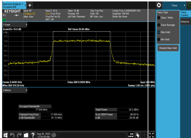
Plot 7-59. 26dB & 99% Bandwidth Plot Antenna WF5t (80MHz 802.11ax (UNII Band 8) – Ch. 199, MCS11)
