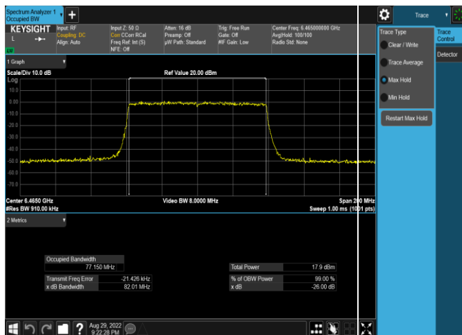
Plot 7-9. 26dB & 99% Bandwidth Plot Antenna WF5t (80MHz 802.11ax (UNII Band 6) – Ch. 103, MCS2)
