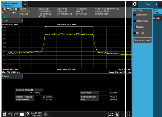
Plot 7-39. 26dB & 99% Bandwidth Plot Antenna WF5t (80MHz 802.11ax (UNII Band 8) – Ch. 199, MCS4)
