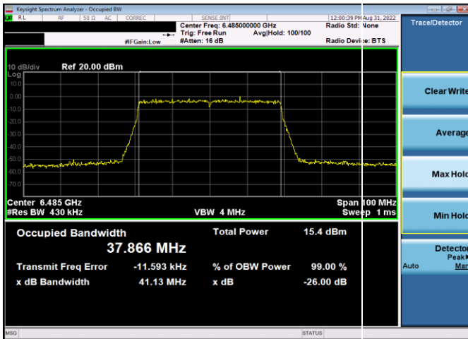
Plot 7-28. 26dB & 99% Bandwidth Plot Antenna WF5t (40MHz 802.11ax (UNII Band 6) – Ch. 107, MCS4)
