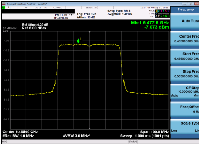
Plot 7-148. Power Spectral Density Plot Antenna WF5t (40MHz 802.11ax (UNII Band 6) – Ch. 107, MCS4)
