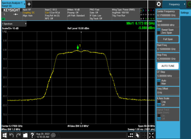
Plot 7-121. Power Spectral Density Plot Antenna WF5t (20MHz 802.11a (UNII Band 5) – Ch. 45, MCS2)
