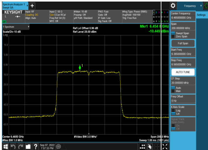
Plot 7-318. Power Spectral Density Plot SDM Antenna WF5b (80MHz 802.11ax (UNII Band 6) – Ch. 103, MCS11)
