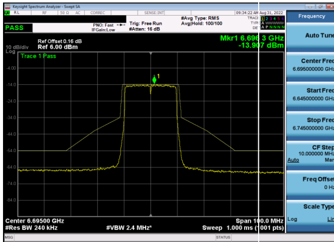
Plot 7-348. In-Band Emission Plot Antenna WF5t (20MHz 802.11ax (UNII Band 7) – Ch. 149, MCS2)
