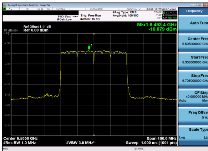
Plot 7-319. Power Spectral Density Plot SDM Antenna WF5t (160MHz 802.11ax (UNII Band 6) – Ch. 111, MCS11)
