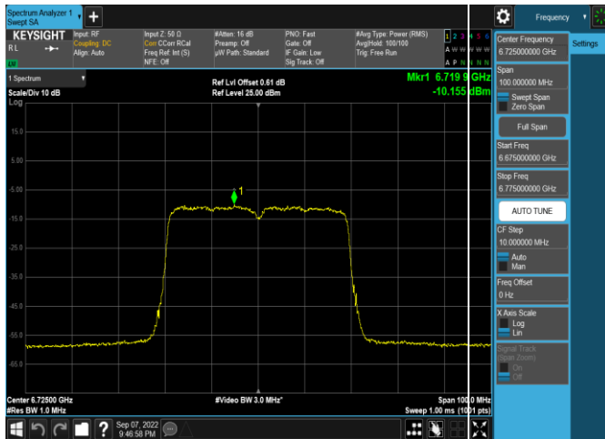
Plot 7-324. Power Spectral Density Plot SDM Antenna WF5b (40MHz 802.11ax (UNII Band 7) – Ch. 155, MCS11)
